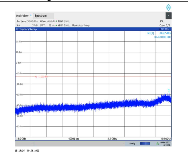
1-N78-3450-3550-PC1-30-100-L-1-DFT-PI2BPSK- Inner_1RB_Left-1@1-18000-40000-Ant0-18000.00-- 61.97--13-PASS
