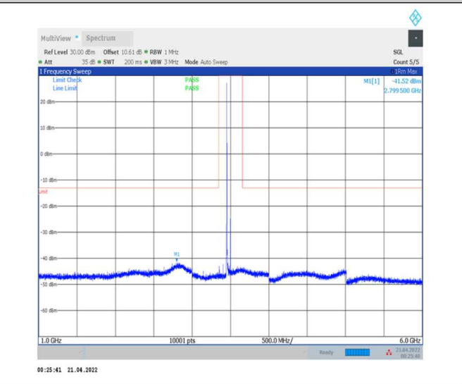
1-N78-3450-3550--30-100-H-1-DFT-PI2BPSK- Inner_1RB_Left-1@1-1000-6000-Ant0--41.52--13- PASS
