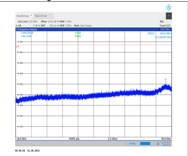
1-N78-3450-3550--30-100-L-1-DFT-PI2BPSK- Inner_1RB_Left-1@1-18000-40000-Ant0--48.67--13- PASS
