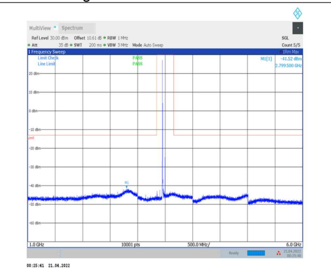
1-N78-3450-3550--30-100-M-1-DFT-PI2BPSK- Inner_1RB_Left-1@1-1000-6000-Ant0--41.68--13- PASS
