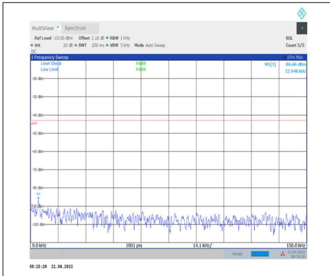
1-N78-3450-3550--30-100-H-1-DFT-PI2BPSK- Inner_1RB_Left-1@1-0.009-0.15-Ant0--86.66--43- PASS
