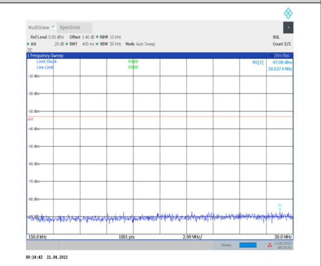
1-N78-3450-3550--30-100-M-1-DFT-PI2BPSK- Inner_1RB_Left-1@1-0.15-30-Ant0--87.00--33-PASS
