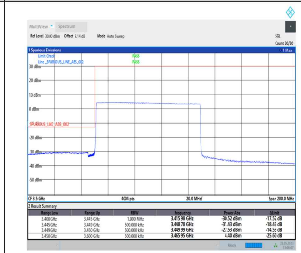
1-N78-3450-3550-PC1-30-80-L-3-DFT-PI2BPSK-Outer_Full-216@0-Ant0-1--PASS-see graph
