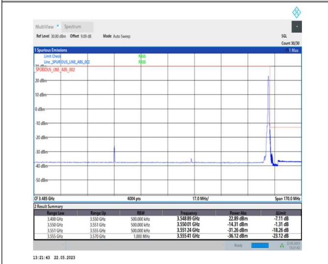
1-N78-3450-3550-PC1-30-100-H-5-CP-QPSK-Edge_1RB_Right-1@272-Ant0-1--PASS-see graph
