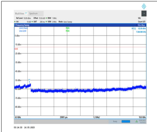
1-N78-3450-3550-PC1-30-100-L-1-DFT-PI2BPSK- Inner_1RB_Left-1@1-6000-18000-Ant0-7366.08-- 52.90--13-PASS
