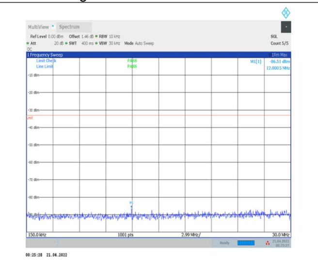
1-N78-3450-3550--30-100-H-1-DFT-PI2BPSK- Inner_1RB_Left-1@1-0.15-30-Ant0--86.51--33-PASS
