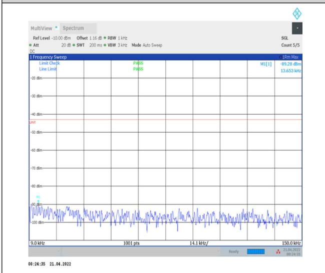
1-N78-3450-3550--30-100-M-1-DFT-PI2BPSK- Inner_1RB_Left-1@1-0.009-0.15-Ant0--89.28--43- PASS
