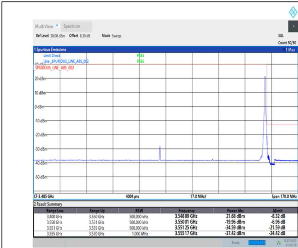
1-N78-3450-3550-PC1-30-70-H-2-DFT-PI2BPSK-Edge_1RB_Right-1@188-Ant0-1--PASS-see graph
