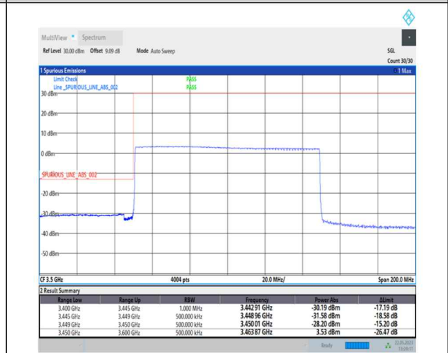
1-N78-3450-3550-PC1-30-100-L-3-DFT-PI2BPSK-Outer_Full-270@0-Ant0-1--PASS-see graph
