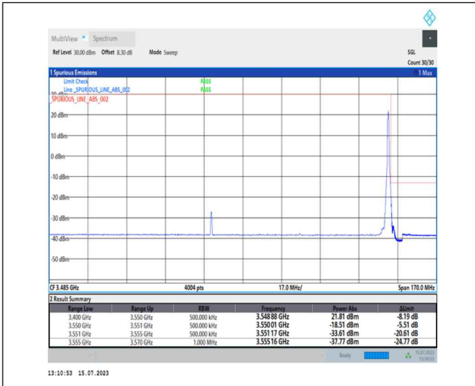
1-N78-3450-3550-PC1-30-80-H-2-DFT-PI2BPSK-Edge_1RB_Right-1@216-Ant0-1--PASS-see graph
