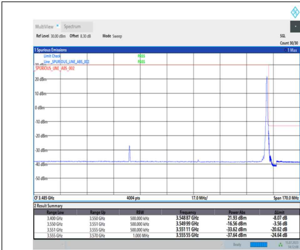
1-N78-3450-3550-PC1-30-90-H-2-DFT-PI2BPSK-Edge_1RB_Right-1@244-Ant0-1--PASS-see graph
