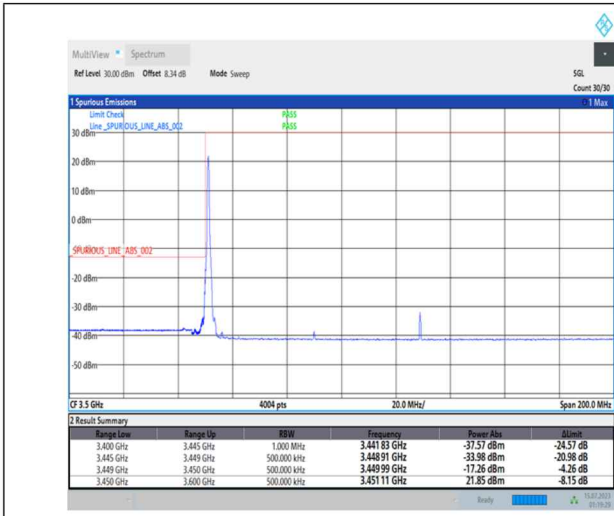
1-N78-3450-3550-PC1-30-80-L-1-DFT-PI2BPSK-Edge_1RB_Left-1@0-Ant0-1--PASS-see graph
