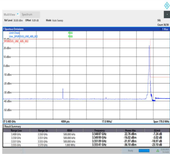
1-N78-3450-3550-PC1-30-90-H-2-DFT-PI2BPSK-Edge_1RB_Right-1@244-Ant0-1--PASS-see graph
