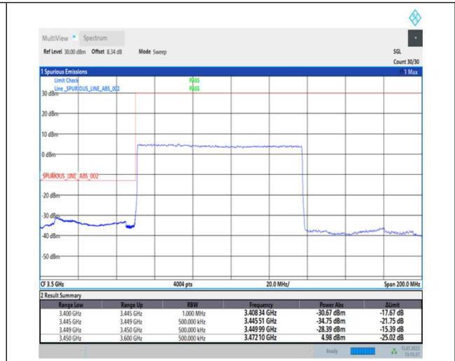
1-N78-3450-3550-PC1-30-90-L-3-DFT-PI2BPSK-Outer_Full-240@0-Ant0-1--PASS-see graph
