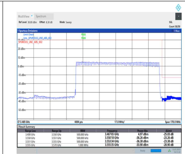
1-N78-3450-3550-PC1-30-90-H-3-DFT-PI2BPSK-Outer_Full-240@0-Ant0-1--PASS-see graph
