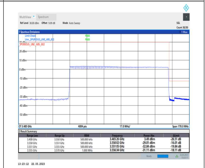
1-N78-3450-3550-PC1-30-100-H-6-CP-QPSK-Outer_Full-273@0-Ant0-1--PASS-see graph
