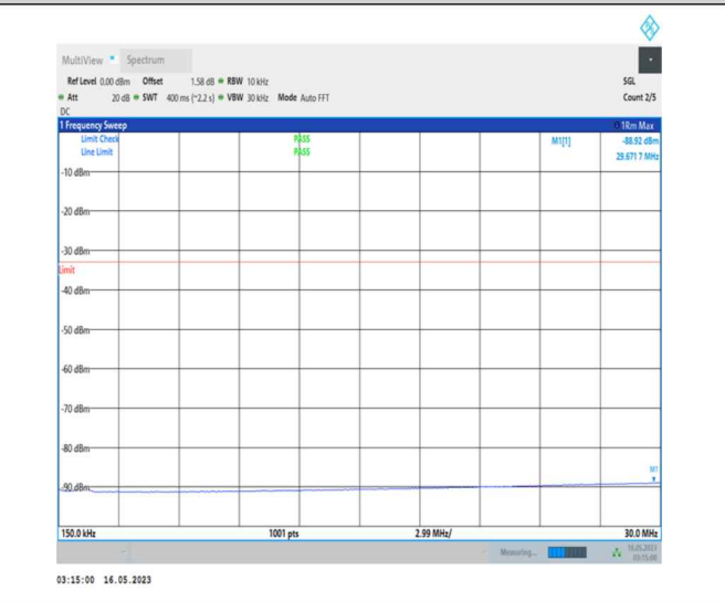
1-N78-3450-3550-PC1-30-100-M-1-DFT-PI2BPSK- Inner_1RB_Left-1@1-0.15-30-Ant0-29.67--88.92--33- PASS
