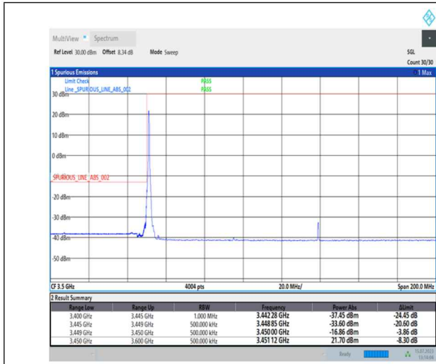
1-N78-3450-3550-PC1-30-90-L-1-DFT-PI2BPSK-Edge_1RB_Left-1@0-Ant0-1--PASS-see graph
