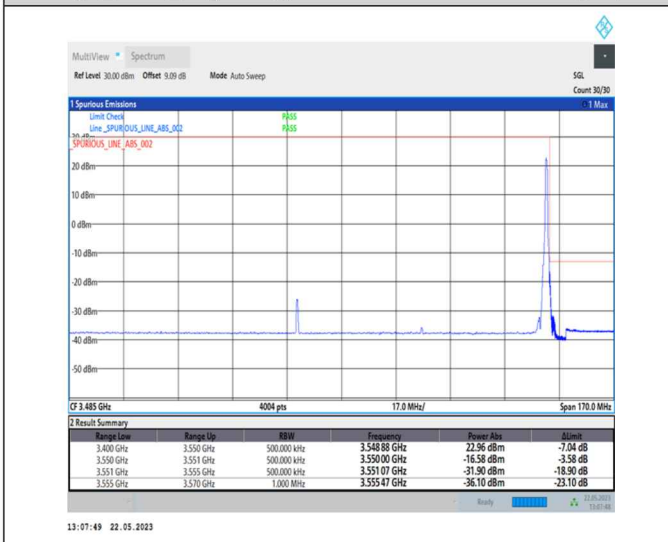
1-N78-3450-3550-PC1-30-80-H-5-CP-QPSK-Edge_1RB_Right-1@216-Ant0-1--PASS-see graph
