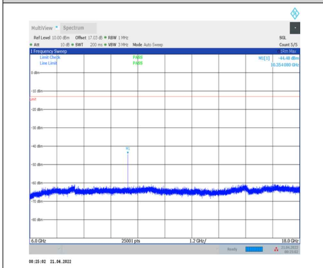
1-N78-3450-3550--30-100-M-1-DFT-PI2BPSK- Inner_1RB_Left-1@1-6000-18000-Ant0--44.48--13- PASS
