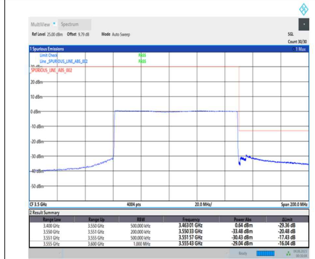
1-N78-3450-3550-PC1-30-90-H-3-DFT-PI2BPSK-Outer_Full-240@0-Ant0-1--PASS-see graph
