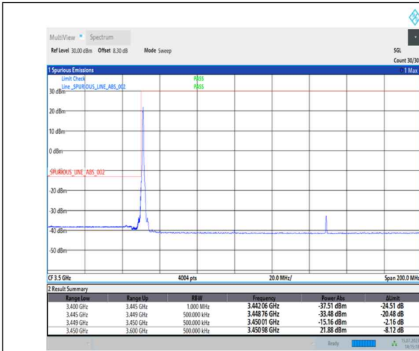
1-N78-3450-3550-PC1-30-100-L-1-DFT-PI2BPSK-Edge_1RB_Left-1@0-Ant0-1--PASS-see graph
