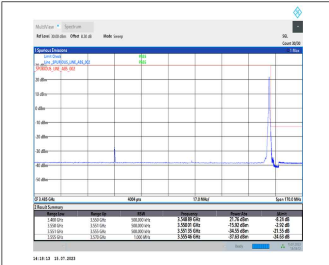
1-N78-3450-3550-PC1-30-100-H-2-DFT-PI2BPSK-Edge_1RB_Right-1@272-Ant0-1--PASS-see graph
