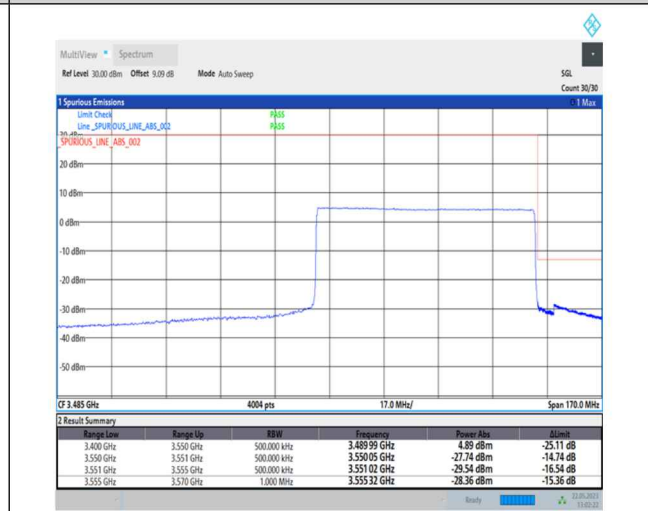
1-N78-3450-3550-PC1-30-70-H-3-DFT-PI2BPSK-Outer_Full-180@0-Ant0-1--PASS-see graph
