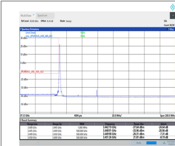
1-N78-3450-3550-PC1-30-50-L-1-DFT-PI2BPSK-Edge_1RB_Left-1@0-Ant0-1--PASS-see graph
