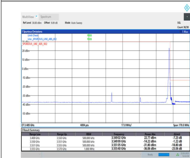
1-N78-3450-3550-PC1-30-60-H-2-DFT-PI2BPSK-Edge_1RB_Right-1@161-Ant0-1--PASS-see graph
