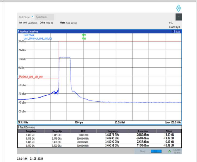
1-N78-3450-3550-PC1-30-15-L-6-CP-QPSK-Outer_Full-38@0-Ant0-1--PASS-see graph
