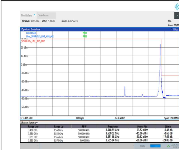
1-N78-3450-3550-PC1-30-40-H-2-DFT-PI2BPSK-Edge_1RB_Right-1@105-Ant0-1--PASS-see graph
