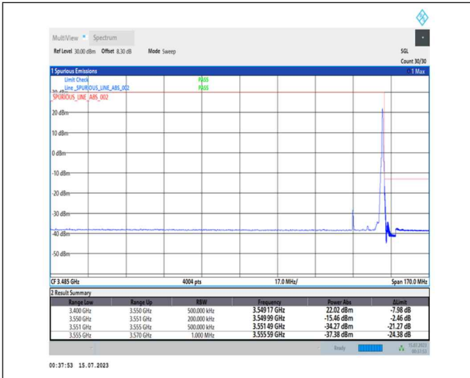
1-N78-3450-3550-PC1-30-15-H-2-DFT-PI2BPSK-Edge_1RB_Right-1@37-Ant0-1--PASS-see graph
