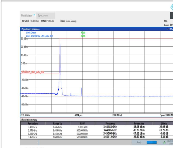
1-N78-3450-3550-PC1-30-30-L-1-DFT-PI2BPSK-Edge_1RB_Left-1@0-Ant0-1--PASS-see graph
