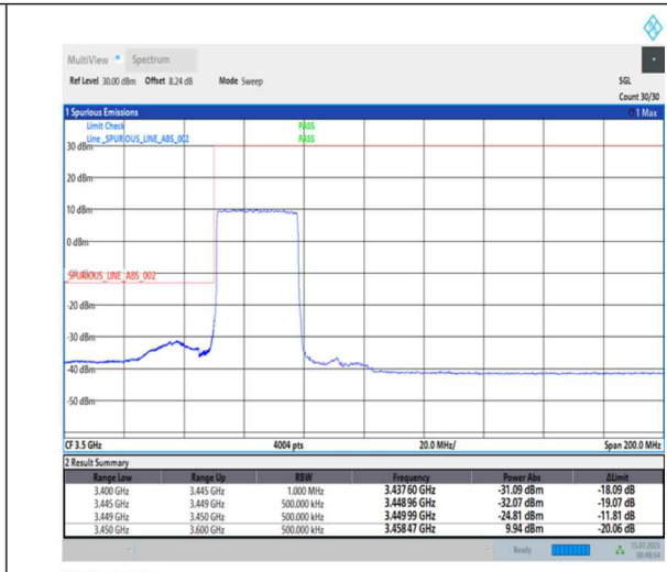
1-N78-3450-3550-PC1-30-30-L-3-DFT-PI2BPSK-Outer_Full-75@0-Ant0-1--PASS-see graph
