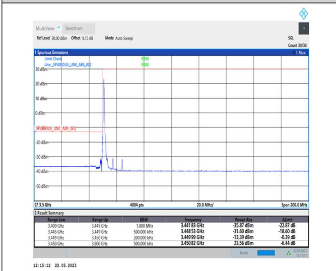
1-N78-3450-3550-PC1-30-15-L-4-CP-QPSK-Edge_1RB_Left-1@0-Ant0-1--PASS-see graph
