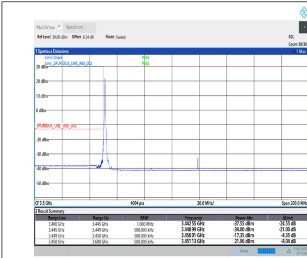
1-N78-3450-3550-PC1-30-70-L-1-DFT-PI2BPSK-Edge_1RB_Left-1@0-Ant0-1--PASS-see graph
