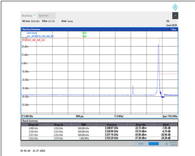
1-N78-3450-3550-PC1-30-30-H-2-DFT-PI2BPSK-Edge_1RB_Right-1@77-Ant0-1--PASS-see graph
