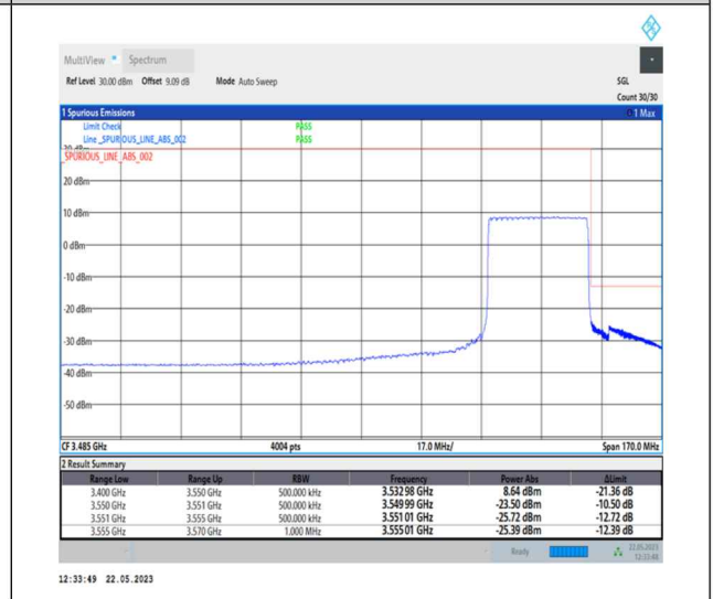
1-N78-3450-3550-PC1-30-30-H-6-CP-QPSK-Outer_Full-78@0-Ant0-1--PASS-see graph
