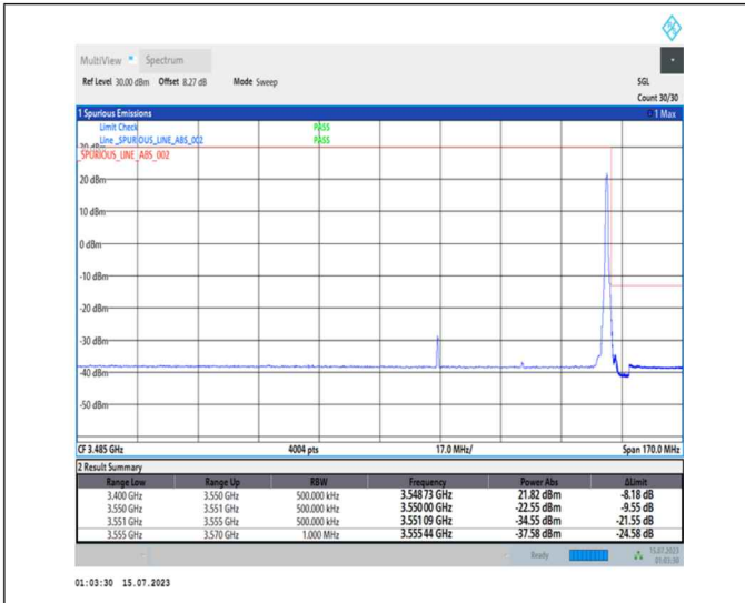
1-N78-3450-3550-PC1-30-50-H-2-DFT-PI2BPSK-Edge_1RB_Right-1@132-Ant0-1--PASS-see graph
