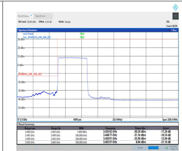
1-N78-3450-3550-PC1-30-40-L-3-DFT-PI2BPSK-Outer_Full-100@0-Ant0-1--PASS-see graph
