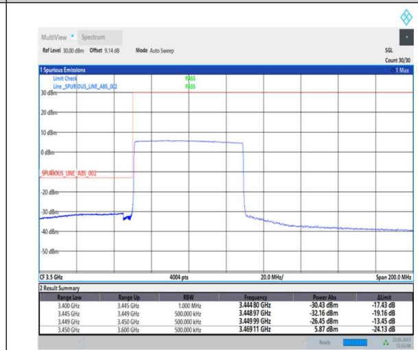
1-N78-3450-3550-PC1-30-60-L-3-DFT-PI2BPSK-Outer_Full-162@0-Ant0-1--PASS-see graph
