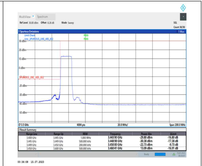
1-N78-3450-3550-PC1-30-15-L-3-DFT-PI2BPSK-Outer_Full-36@0-Ant0-1--PASS-see graph
