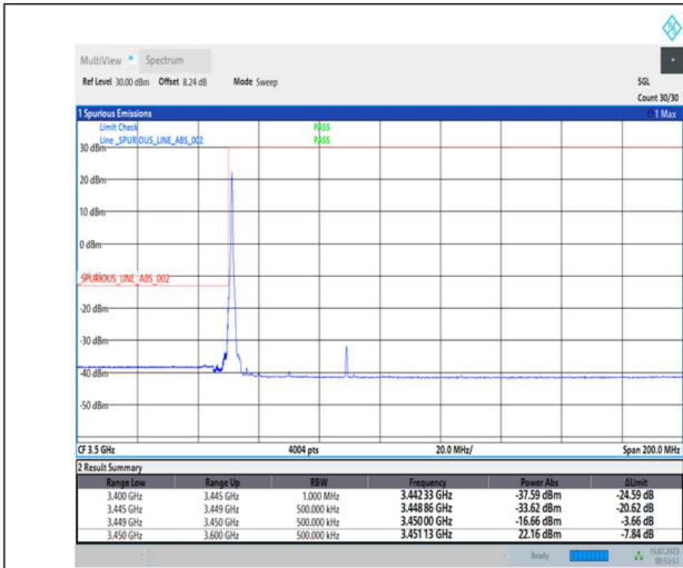
1-N78-3450-3550-PC1-30-40-L-1-DFT-PI2BPSK-Edge_1RB_Left-1@0-Ant0-1--PASS-see graph
