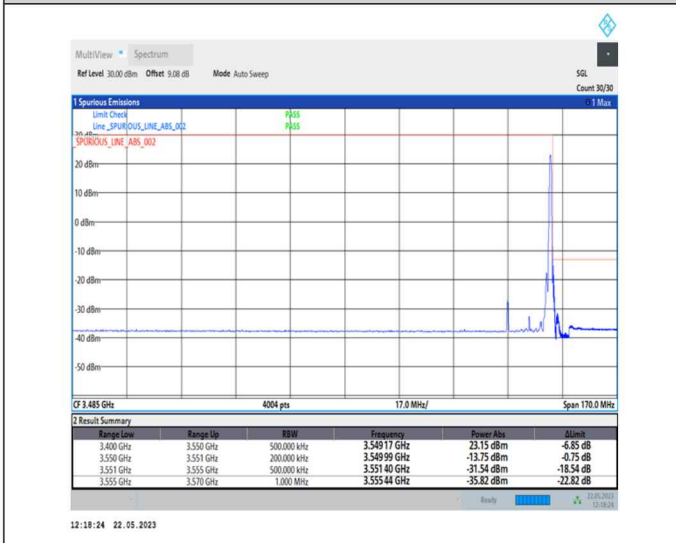
1-N78-3450-3550-PC1-30-15-H-5-CP-QPSK-Edge_1RB_Right-1@37-Ant0-1--PASS-see graph
