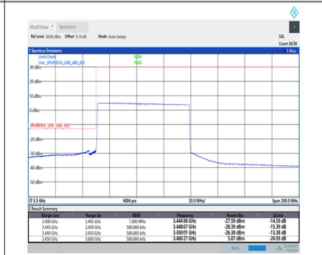
1-N78-3450-3550-PC1-30-70-L-3-DFT-PI2BPSK-Outer_Full-180@0-Ant0-1--PASS-see graph
