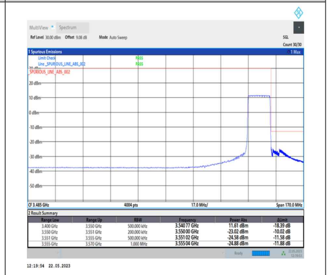
1-N78-3450-3550-PC1-30-15-H-6-CP-QPSK-Outer_Full-38@0-Ant0-1--PASS-see graph
