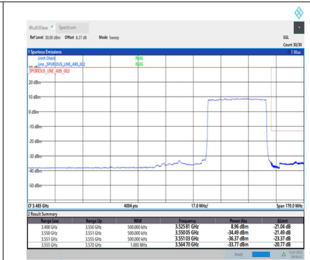
1-N78-3450-3550-PC1-30-40-H-3-DFT-PI2BPSK-Outer_Full-100@0-Ant0-1--PASS-see graph
