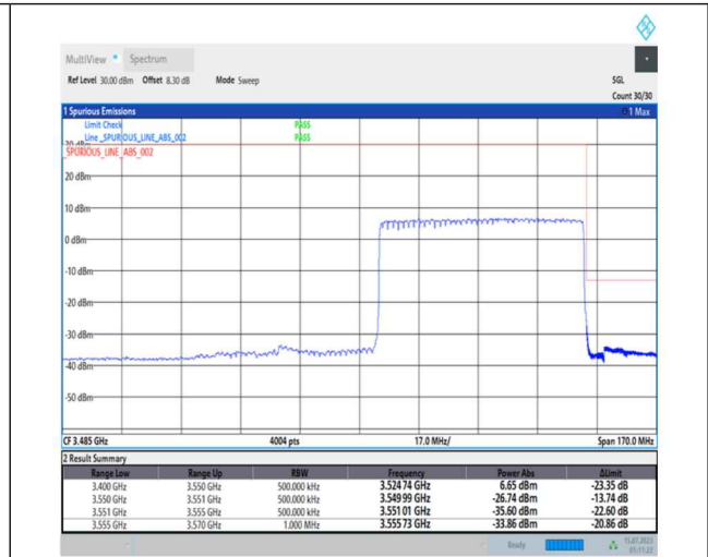
1-N78-3450-3550-PC1-30-60-H-3-DFT-PI2BPSK-Outer_Full-162@0-Ant0-1--PASS-see graph
