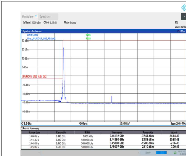
1-N78-3450-3550-PC1-30-60-L-1-DFT-PI2BPSK-Edge_1RB_Left-1@0-Ant0-1--PASS-see graph
