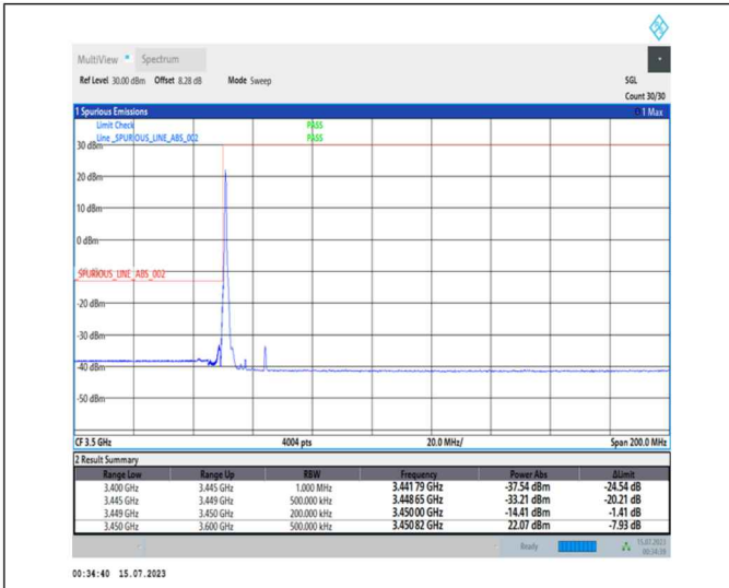
1-N78-3450-3550-PC1-30-15-L-1-DFT-PI2BPSK-Edge_1RB_Left-1@0-Ant0-1--PASS-see graph
