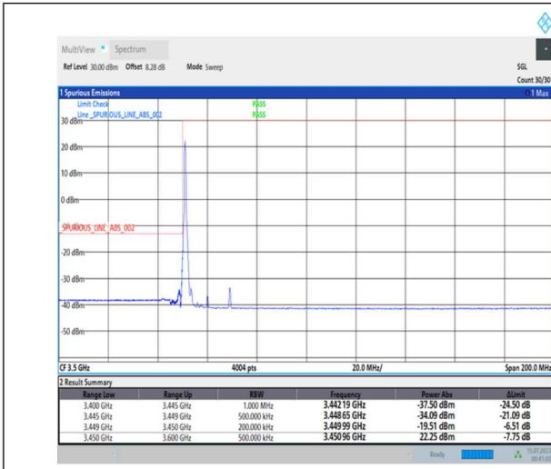
1-N78-3450-3550-PC1-30-20-L-1-DFT-PI2BPSK-Edge_1RB_Left-1@0-Ant0-1--PASS-see graph
