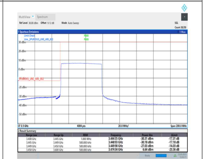
1-N78-3450-3550-PC1-30-50-L-3-DFT-PI2BPSK-Outer_Full-128@0-Ant0-1--PASS-see graph
