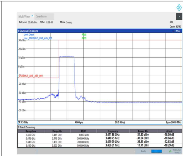
1-N78-3450-3550-PC1-30-20-L-3-DFT-PI2BPSK-Outer_Full-50@0-Ant0-1--PASS-see graph
