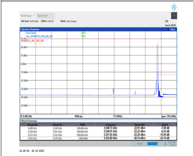
1-N78-3450-3550-PC1-30-50-H-5-CP-QPSK-Edge_1RB_Right-1@132-Ant0-1--PASS-see graph
