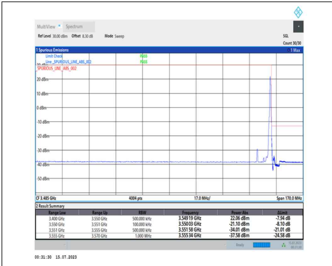
1-N78-3450-3550-PC1-30-10-H-2-DFT-PI2BPSK-Edge_1RB_Right-1@23-Ant0-1--PASS-see graph
