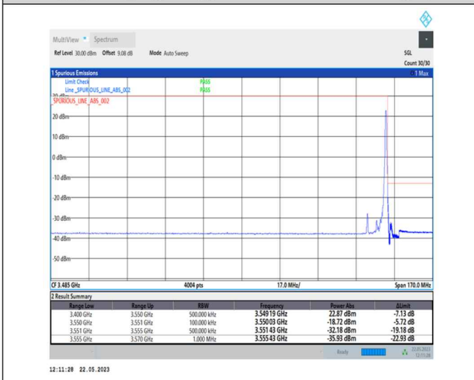
1-N78-3450-3550-PC1-30-10-H-5-CP-QPSK-Edge_1RB_Right-1@23-Ant0-1--PASS-see graph
