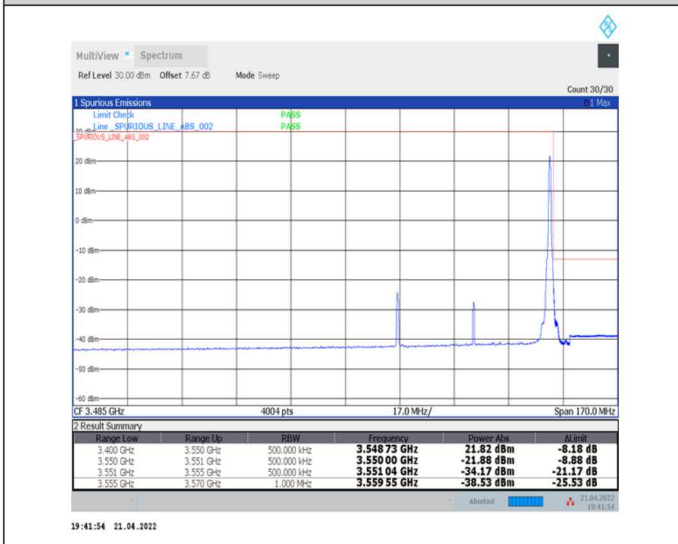
1-N78-3450-3550-30-50-H-5-CP-QPSK-Edge_1RB_Right-1@132-Ant0-PASS-see graph
