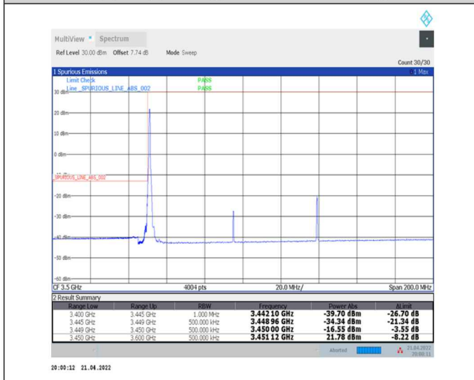
1-N78-3450-3550--30-90-L-4-CP-QPSK-Edge_1RB_Left-1@0-Ant0-PASS-see graph
