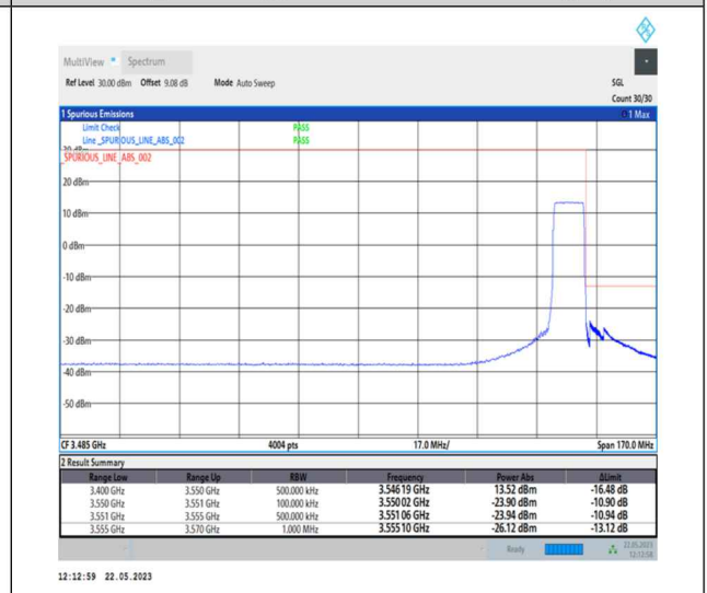
1-N78-3450-3550-PC1-30-10-H-6-CP-QPSK-Outer_Full-24@0-Ant0-1--PASS-see graph
