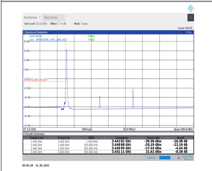
1-N78-3450-3550--30-80-L-4-CP-QPSK-Edge_1RB_Left-1@0-Ant0-PASS-see graph
