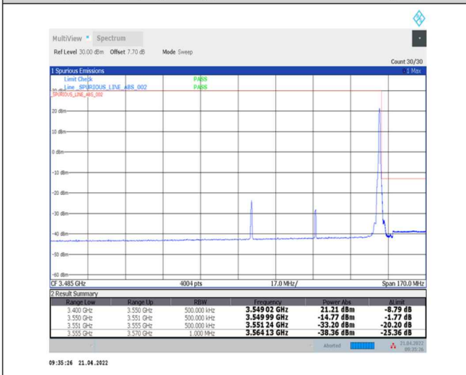
1-N78-3450-3550-30-60-H-5-CP-QPSK-Edge_1RB_Right-1@161-Ant0-PASS-see graph
