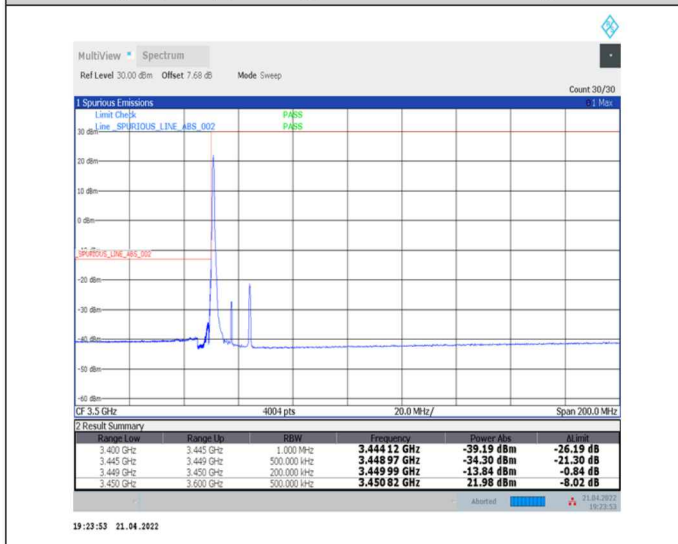
1-N78-3450-3550--30-15-L-4-CP-QPSK-Edge_1RB_Left-1@0-Ant0-PASS-see graph
