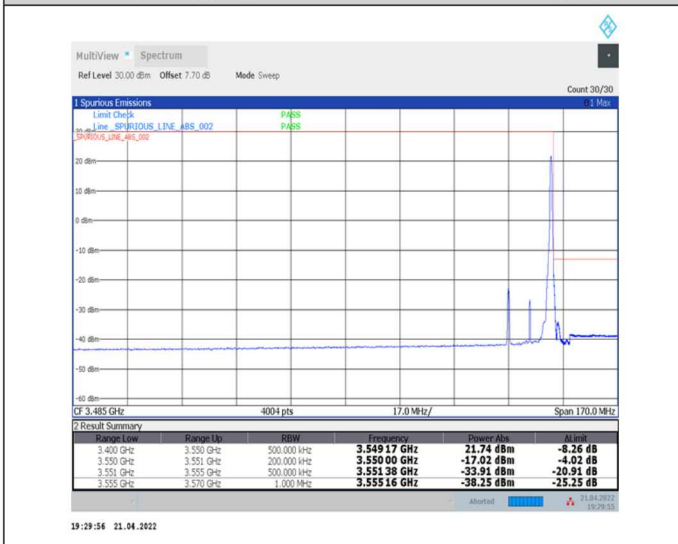
1-N78-3450-3550-30-15-H-5-CP-QPSK-Edge_1RB_Right-1@37-Ant0-PASS-see graph
