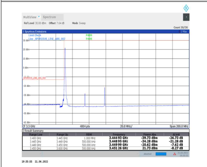
1-N78-3450-3550--30-50-L-4-CP-QPSK-Edge_1RB_Left-1@0-Ant0-PASS-see graph
