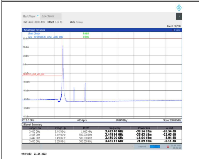
1-N78-3450-3550--30-30-L-4-CP-QPSK-Edge_1RB_Left-1@0-Ant0-PASS-see graph
