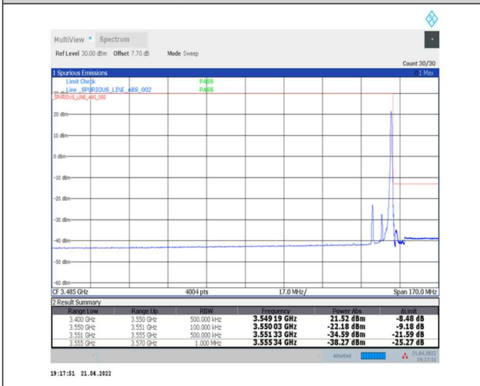
1-N78-3450-3550-30-10-H-5-CP-QPSK-Edge_1RB_Right-1@23-Ant0-PASS-see graph
