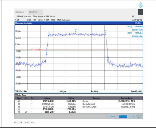
1-N78-3450-3550-PC1-30-40-H-2-DFT-PI2BPSK-Outer_Full-100@0-Ant0-35.783-38.080-≤40-PASS
