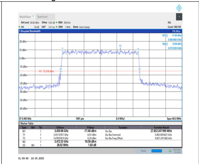
1-N78-3450-3550-PC1-30-30-L-9-CP-256QAM-Outer_Full-78@0-Ant0-27.852-28.920-≤30-PASS
