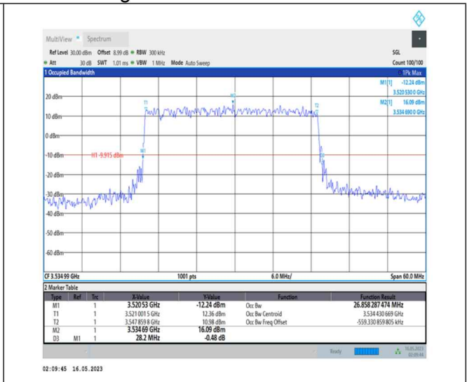
1-N78-3450-3550-PC1-30-30-H-3-DFT-16QAM-Outer_Full-75@0-Ant0-26.858-28.200-≤30-PASS
