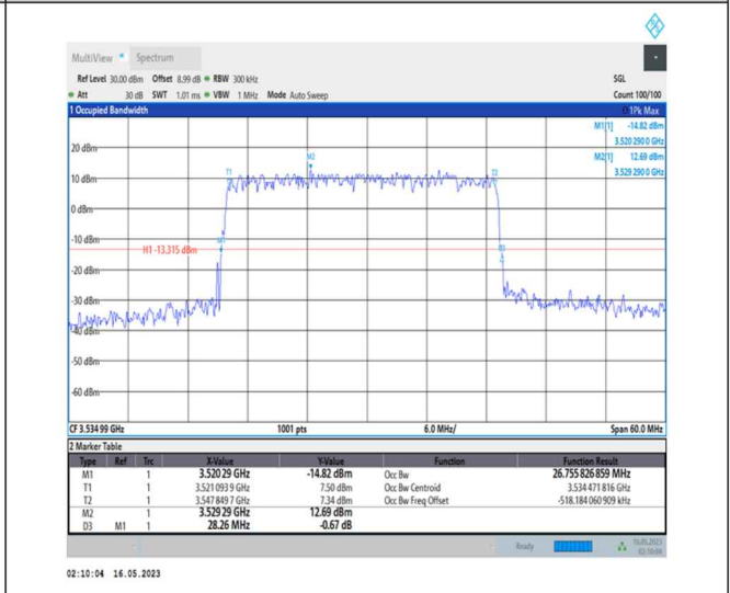
1-N78-3450-3550-PC1-30-30-H-5-DFT-256QAM-Outer_Full-75@0-Ant0-26.756-28.260-≤30-PASS
