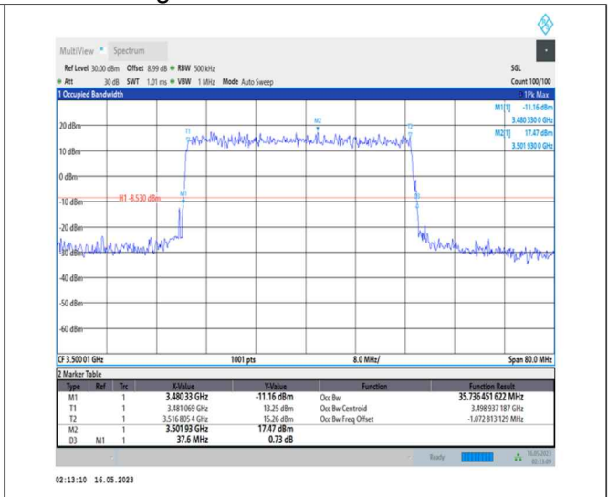
1-N78-3450-3550-PC1-30-40-M-1-DFT-QPSK-Outer_Full-100@0-Ant0-35.736-37.600-≤40-PASS
