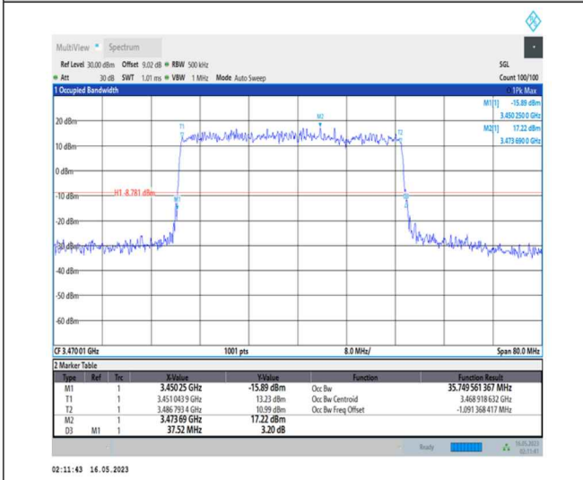
1-N78-3450-3550-PC1-30-40-L-3-DFT-16QAM-Outer_Full-100@0-Ant0-35.75-37.520-≤40-PASS
