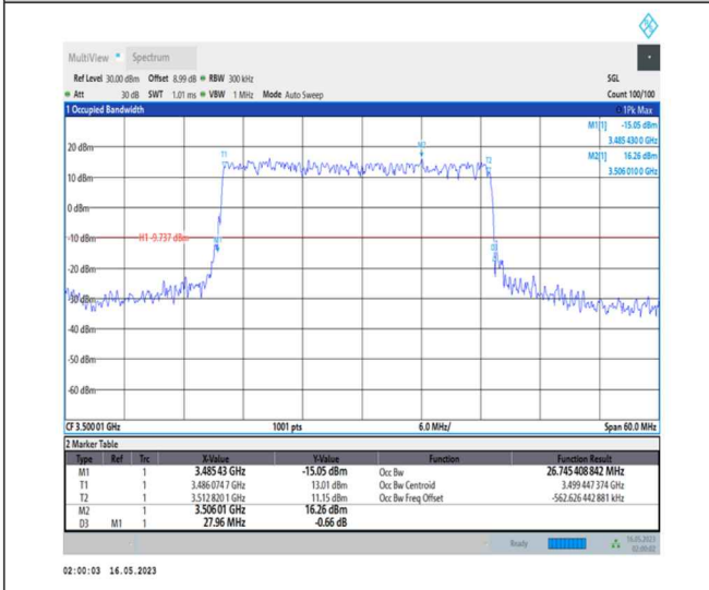
1-N78-3450-3550-PC1-30-30-M-1-DFT-QPSK-Outer_Full-75@0-Ant0-26.745-27.960-≤30-PASS
