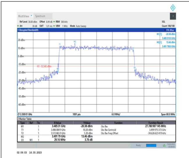
1-N78-3450-3550-PC1-30-30-M-7-CP-16QAM-Outer_Full-78@0-Ant0-27.781-29.160-≤30-PASS
