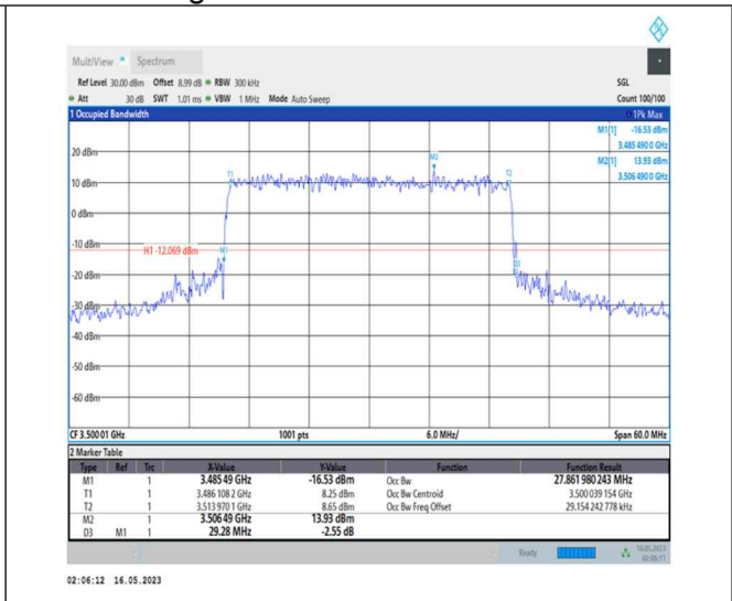
1-N78-3450-3550-PC1-30-30-M-8-CP-64QAM-Outer_Full-78@0-Ant0-27.862-29.280-≤30-PASS
