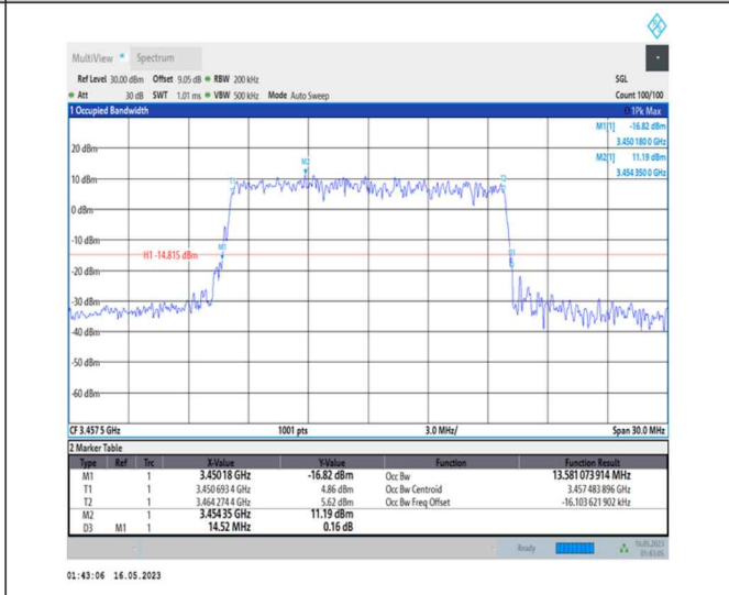
1-N78-3450-3550-PC1-30-15-L-9-CP-256QAM-Outer_Full-38@0-Ant0-13.581-14.520-≤15-PASS
