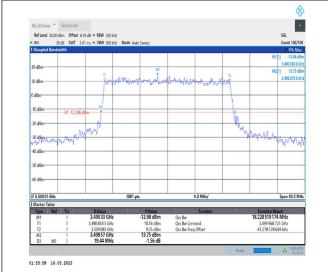
1-N78-3450-3550-PC1-30-20-M-8-CP-64QAM-Outer_Full-51@0-Ant0-18.229-19.440-≤20-PASS
