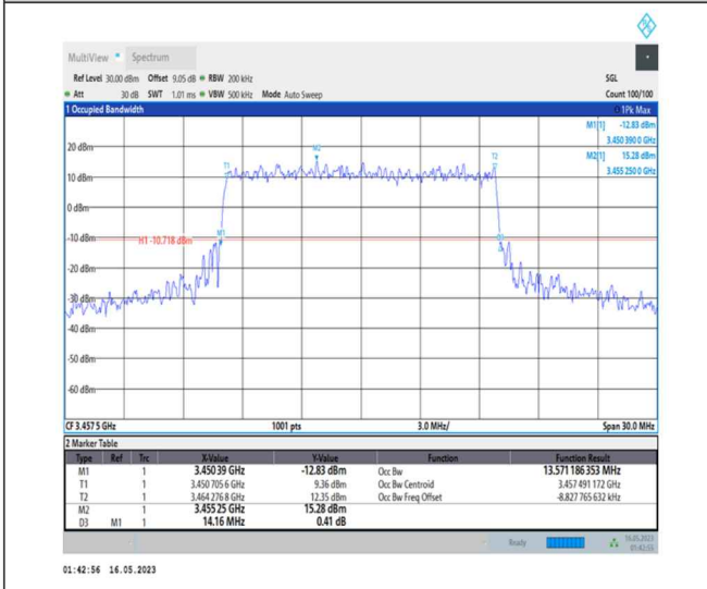
1-N78-3450-3550-PC1-30-15-L-8-CP-64QAM-Outer_Full-38@0-Ant0-13.571-14.160-≤15-PASS
