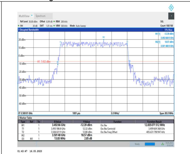
1-N78-3450-3550-PC1-30-15-M-2-DFT-PI2BPSK-Outer_Full-36@0-Ant0-12.835-13.830-≤15-PASS
