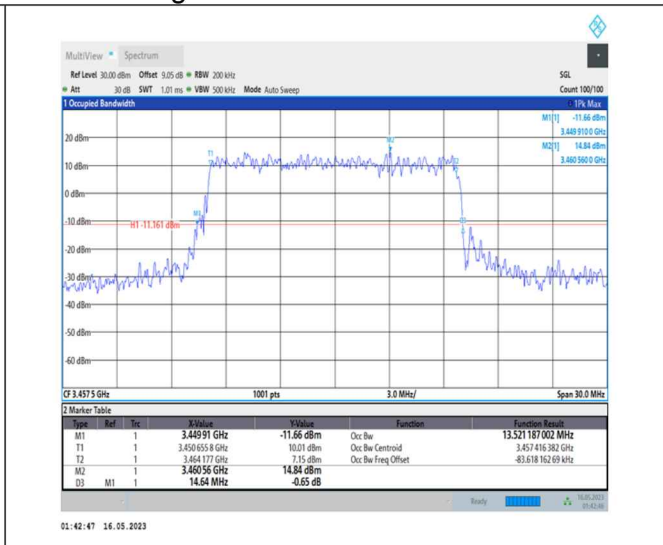
1-N78-3450-3550-PC1-30-15-L-7-CP-16QAM-Outer_Full-38@0-Ant0-13.521-14.640-≤15-PASS
