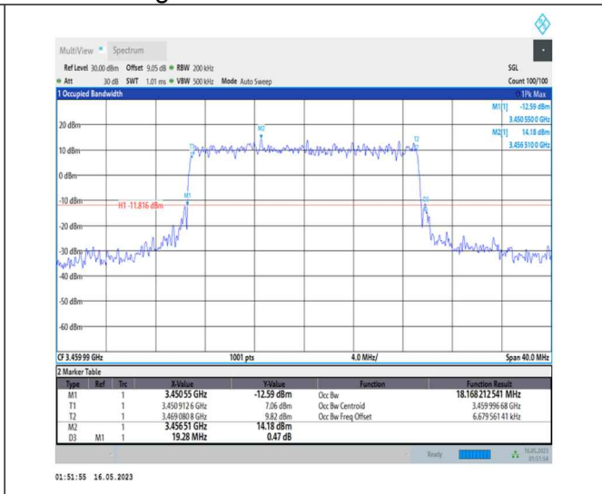
1-N78-3450-3550-PC1-30-20-L-8-CP-64QAM-Outer_Full-51@0-Ant0-18.168-19.280-≤20-PASS
