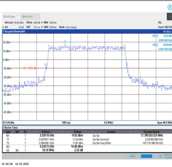
1-N78-3450-3550-PC1-30-20-H-1-DFT-QPSK-Outer_Full-50@0-Ant0-17.79-19.160-≤20-PASS
