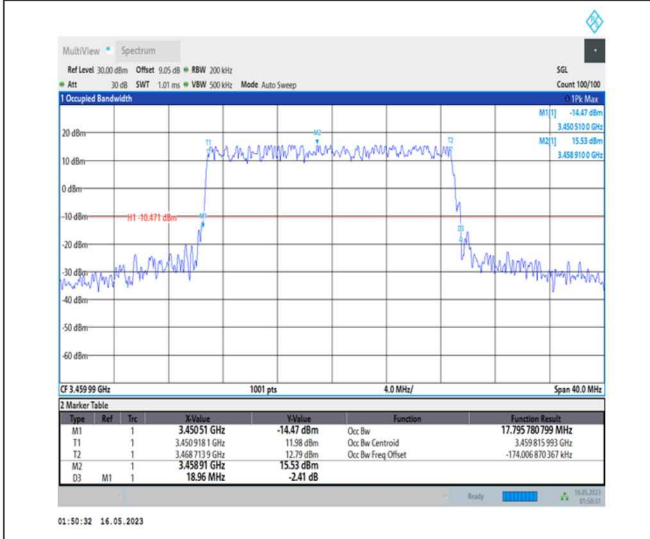
1-N78-3450-3550-PC1-30-20-L-1-DFT-QPSK-Outer_Full-50@0-Ant0-17.796-18.960-≤20-PASS
