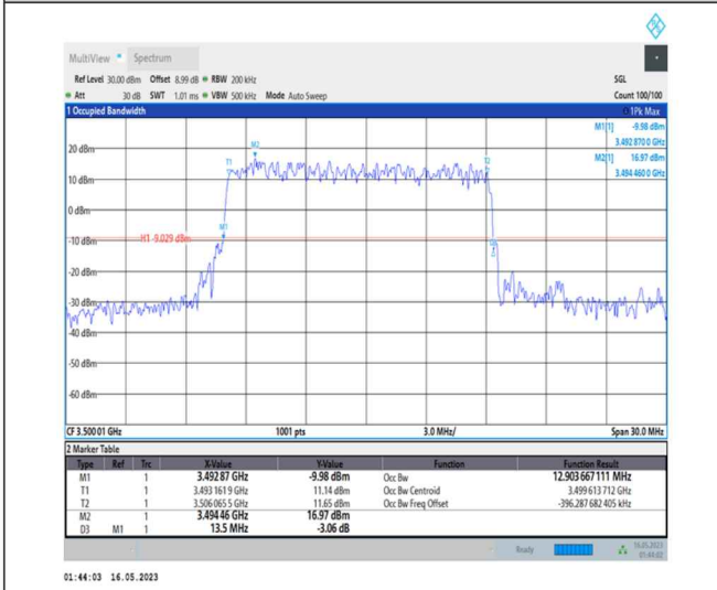
1-N78-3450-3550-PC1-30-15-M-3-DFT-16QAM-Outer_Full-36@0-Ant0-12.904-13.500-≤15-PASS
