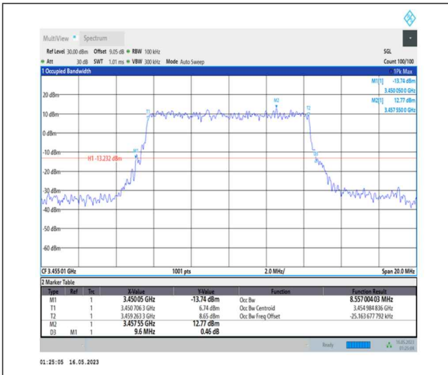
1-N78-3450-3550-PC1-30-10-L-5-DFT-256QAM-Outer_Full-24@0-Ant0-8.557-9.600-≤10-PASS
