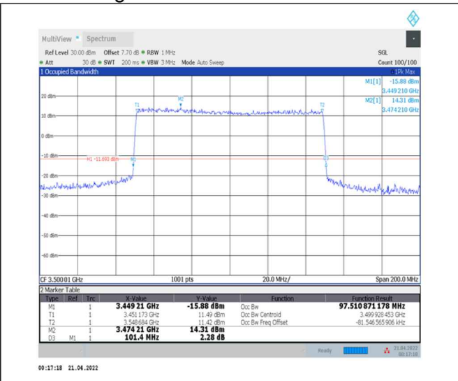
1-N78-3450-3550--30-100-M-7-CP-16QAM- Outer_Full-273@0-Ant0-97.511-101.400-≤100-PASS
