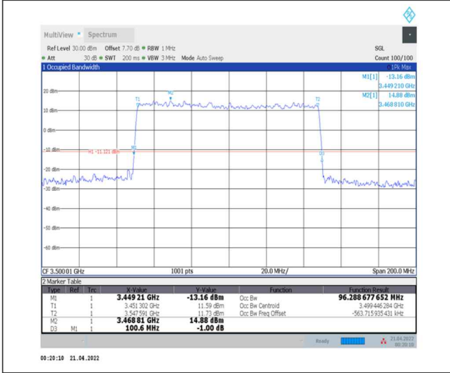
1-N78-3450-3550--30-100-H-3-DFT-16QAM-Outer_Full-270@0-Ant0-96.289-100.600-≤100-PASS
