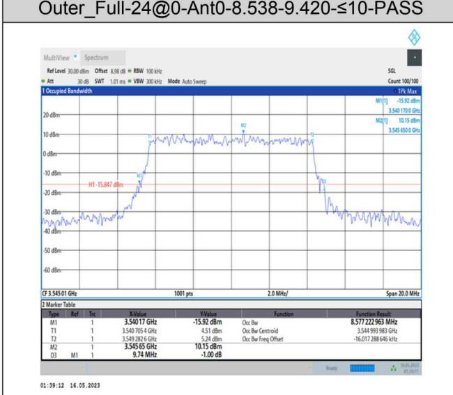
1-N78-3450-3550-PC1-30-10-H-9-CP-256QAM-Outer_Full-24@0-Ant0-8.577-9.740-≤10-PASS
