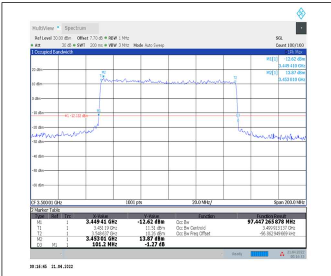
1-N78-3450-3550--30-100-M-6-CP-QPSK- Outer_Full-273@0-Ant0-97.447-101.200-≤100-PASS
