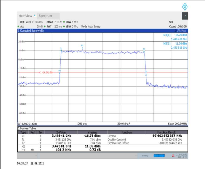
1-N78-3450-3550--30-100-M-9-CP-256QAM- Outer_Full-273@0-Ant0-97.404-101.200-≤100-PASS
