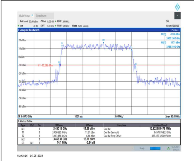
1-N78-3450-3550-PC1-30-15-L-4-DFT-64QAM-Outer_Full-36@0-Ant0-12.823-14.100-≤15-PASS
