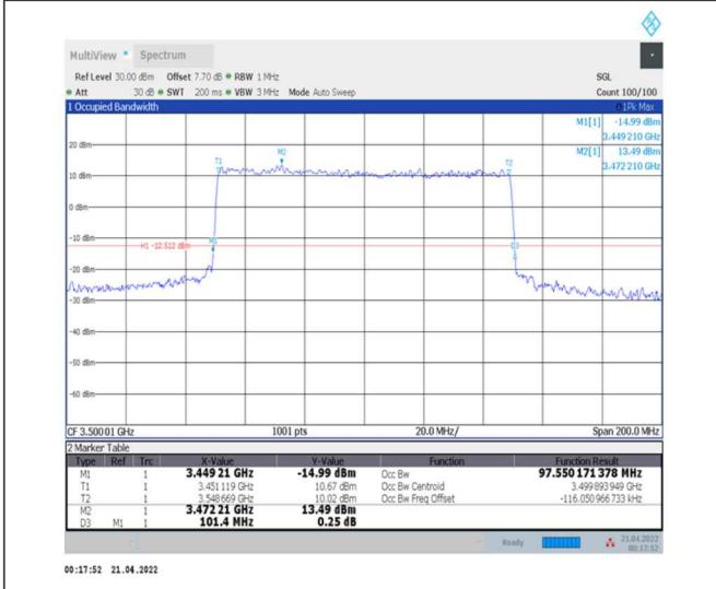
1-N78-3450-3550--30-100-M-8-CP-64QAM- Outer_Full-273@0-Ant0-97.55-101.400-≤100-PASS
