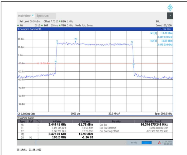
1-N78-3450-3550--30-100-H-1-DFT-QPSK-Outer_Full-270@0-Ant0-96.347-100.200-≤100-PASS
