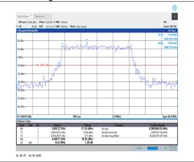
1-N78-3450-3550-PC1-30-10-M-1-DFT-QPSK-Outer_Full-24@0-Ant0-8.59-9.520-≤10-PASS
