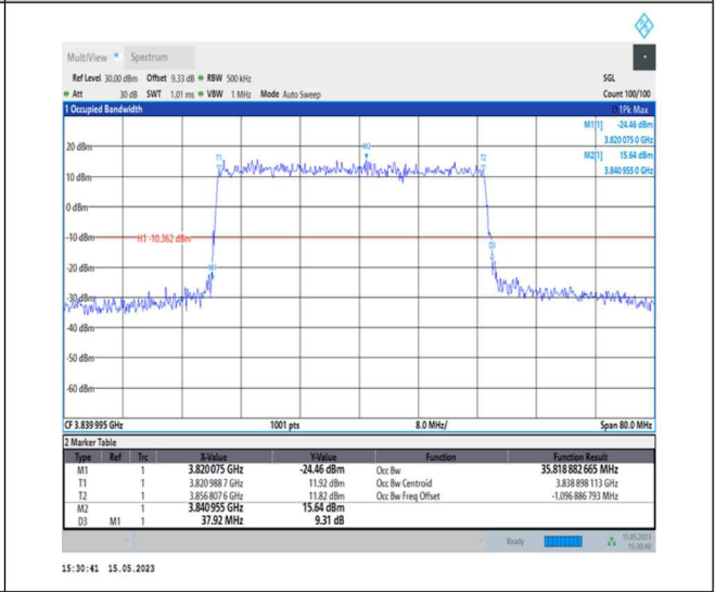
1-N77-3700-3980-PC1-30-40-M-3-DFT-16QAM-Outer_Full-100@0-Ant0-35.819-37.920-≤40-PASS
