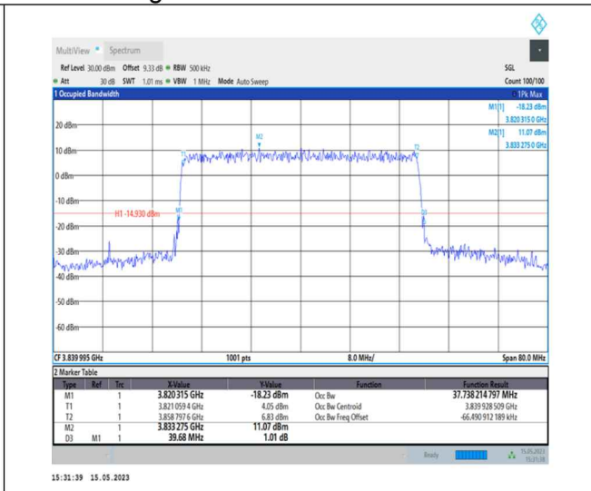
1-N77-3700-3980-PC1-30-40-M-9-CP-256QAM-Outer_Full-106@0-Ant0-37.738-39.680-≤40-PASS
