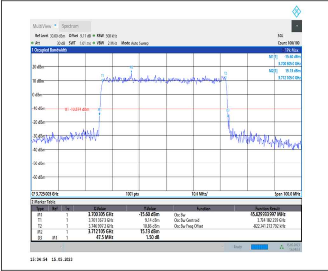
1-N77-3700-3980-PC1-30-50-L-4-DFT-64QAM-Outer_Full-128@0-Ant0-45.63-47.500-≤50-PASS
