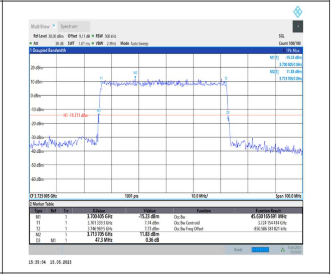
1-N77-3700-3980-PC1-30-50-L-5-DFT-256QAM-Outer_Full-128@0-Ant0-45.63-47.300-≤50-PASS
