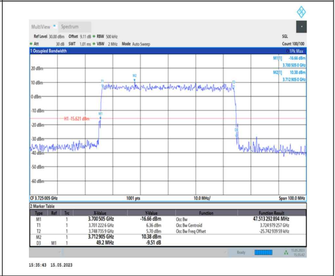
1-N77-3700-3980-PC1-30-50-L-9-CP-256QAM-Outer_Full-133@0-Ant0-47.513-49.200-≤50-PASS
