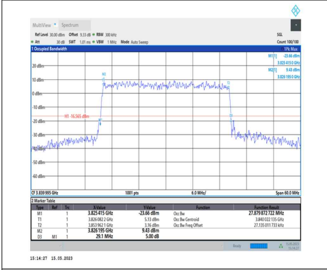
1-N77-3700-3980-PC1-30-30-M-9-CP-256QAM-Outer_Full-78@0-Ant0-27.88-29.100-≤30-PASS
