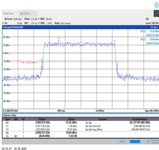
1-N77-3700-3980-PC1-30-30-H-4-DFT-64QAM-Outer_Full-75@0-Ant0-26.727-28.440-≤30-PASS
