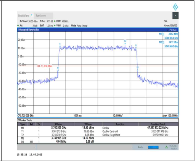
1-N77-3700-3980-PC1-30-50-L-7-CP-16QAM-Outer_Full-133@0-Ant0-47.397-49.400-≤50-PASS
