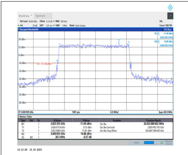
1-N77-3700-3980-PC1-30-30-M-3-DFT-16QAM-Outer_Full-75@0-Ant0-26.833-28.500-≤30-PASS
