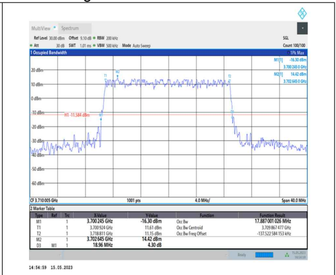
1-N77-3700-3980-PC1-30-20-L-4-DFT-64QAM-Outer_Full-50@0-Ant0-17.887-18.960-≤20-PASS
