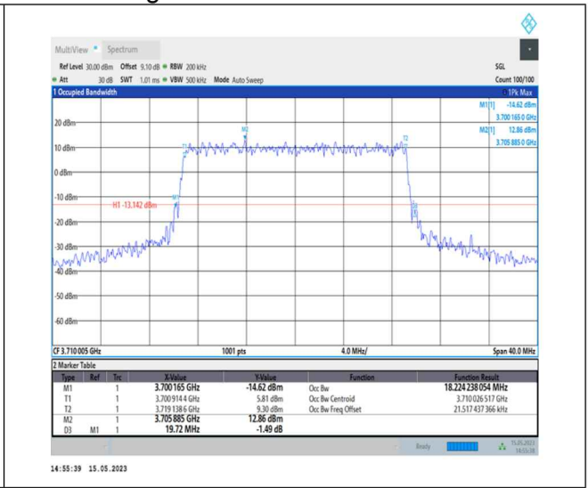
1-N77-3700-3980-PC1-30-20-L-8-CP-64QAM-Outer_Full-51@0-Ant0-18.224-19.720-≤20-PASS
