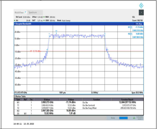
1-N77-3700-3980-PC1-30-15-H-1-DFT-QPSK-Outer_Full-36@0-Ant0-12.844-13.920-≤15-PASS
