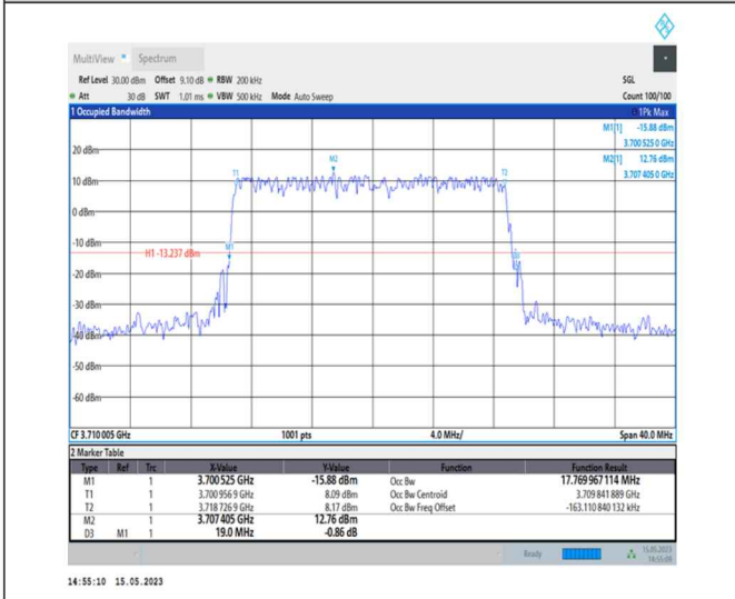
1-N77-3700-3980-PC1-30-20-L-5-DFT-256QAM-Outer_Full-50@0-Ant0-17.77-19.000-≤20-PASS
