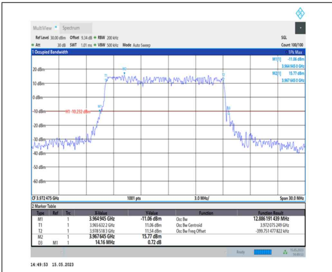
1-N77-3700-3980-PC1-30-15-H-4-DFT-64QAM-Outer_Full-36@0-Ant0-12.886-14.160-≤15-PASS
