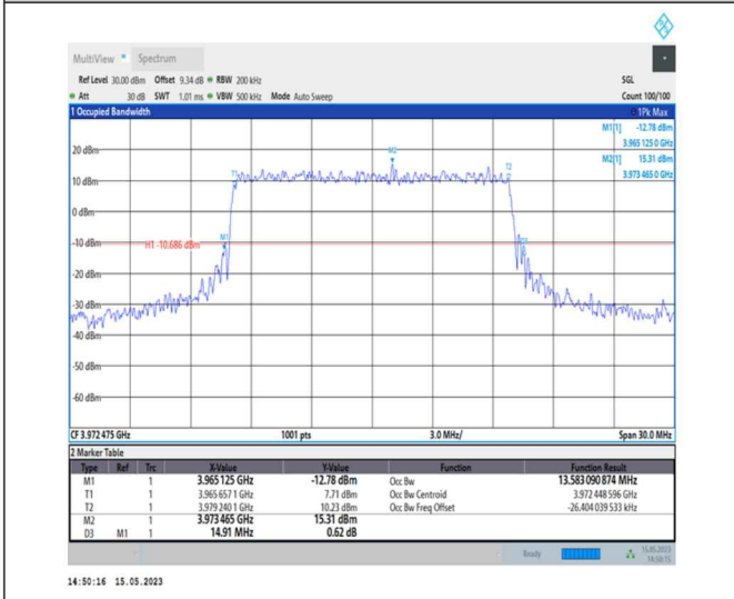
1-N77-3700-3980-PC1-30-15-H-6-CP-QPSK-Outer_Full-38@0-Ant0-13.583-14.910-≤15-PASS
