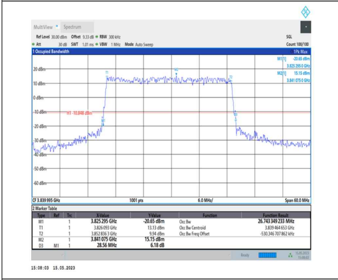
1-N77-3700-3980-PC1-30-30-M-1-DFT-QPSK-Outer_Full-75@0-Ant0-26.743-28.560-≤30-PASS
