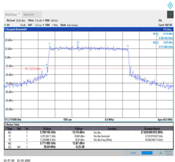
1-N77-3700-3980-PC1-30-30-L-7-CP-16QAM-Outer_Full-78@0-Ant0-27.825-29.640-≤30-PASS
