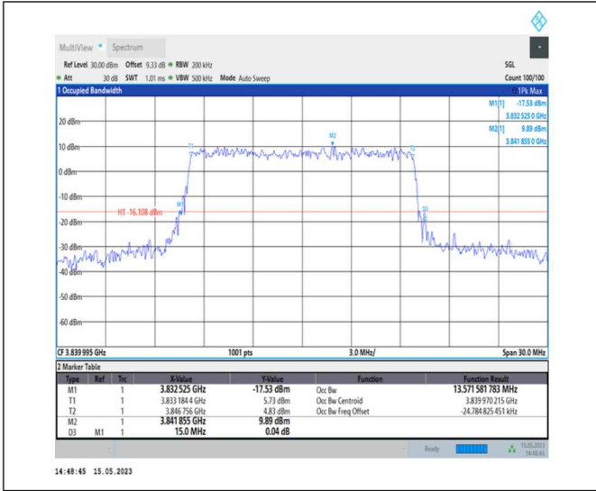
1-N77-3700-3980-PC1-30-15-M-9-CP-256QAM-Outer_Full-38@0-Ant0-13.572-15.000-≤15-PASS
