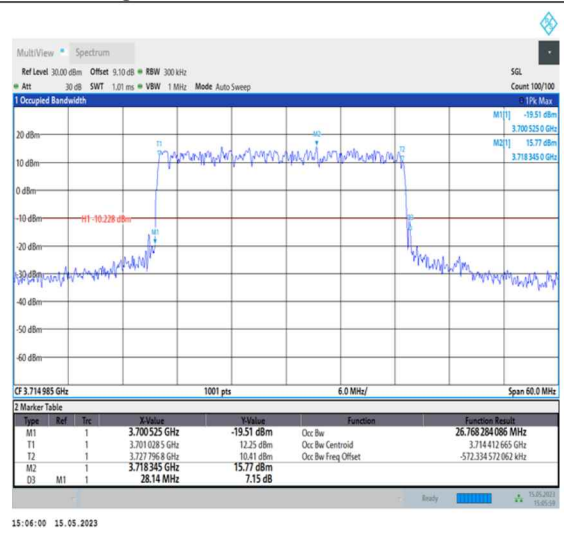
1-N77-3700-3980-PC1-30-30-L-1-DFT-QPSK-Outer_Full-75@0-Ant0-26.768-28.140-≤30-PASS
