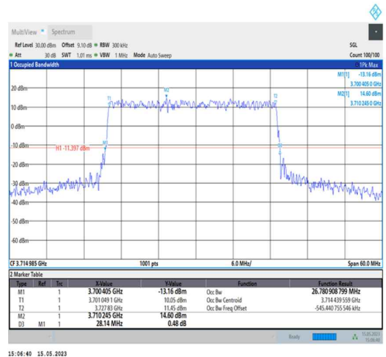
1-N77-3700-3980-PC1-30-30-L-3-DFT-16QAM-Outer_Full-75@0-Ant0-26.781-28.140-≤30-PASS
