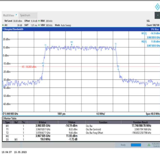
1-N77-3700-3980-PC1-30-20-H-5-DFT-256QAM-Outer_Full-50@0-Ant0-17.747-19.000-≤20-PASS
