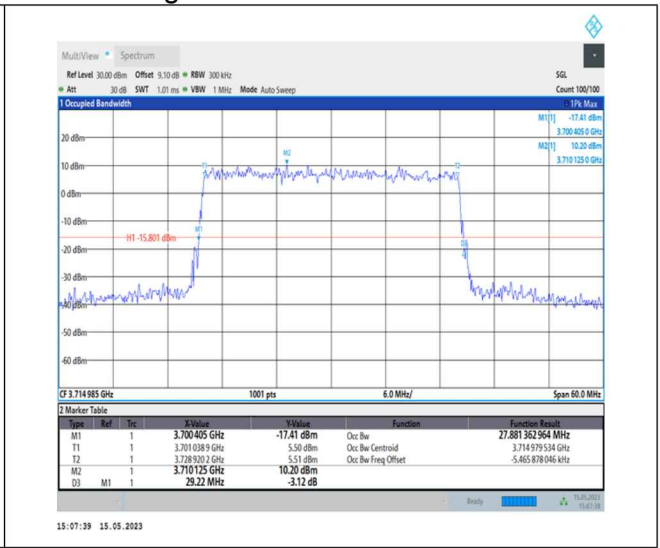
1-N77-3700-3980-PC1-30-30-L-9-CP-256QAM-Outer_Full-78@0-Ant0-27.881-29.220-≤30-PASS
