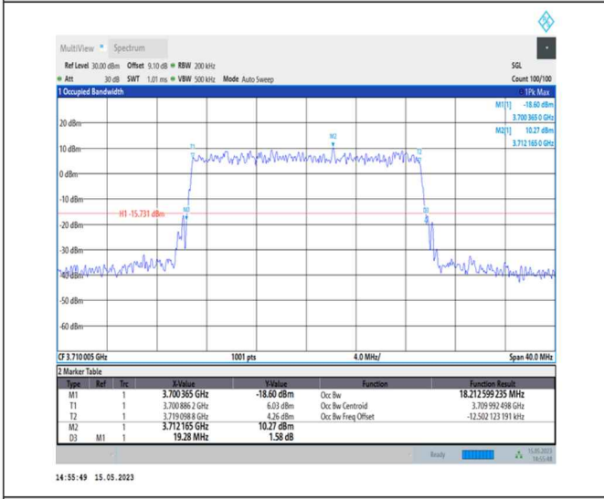
1-N77-3700-3980-PC1-30-20-L-9-CP-256QAM-Outer_Full-51@0-Ant0-18.213-19.280-≤20-PASS
