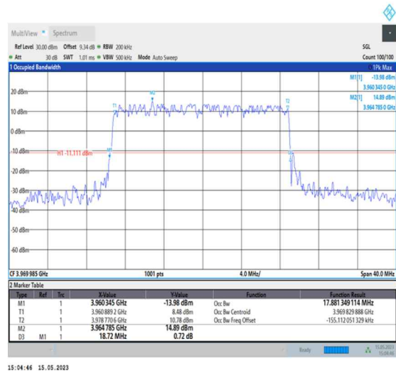
1-N77-3700-3980-PC1-30-20-H-4-DFT-64QAM-Outer_Full-50@0-Ant0-17.881-18.720-≤20-PASS
