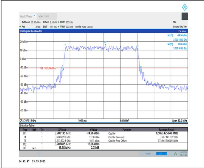
1-N77-3700-3980-PC1-30-15-L-4-DFT-64QAM-Outer_Full-36@0-Ant0-12.863-13.980-≤15-PASS
