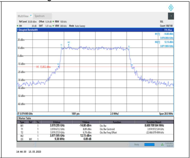
1-N77-3700-3980-PC1-30-10-H-8-CP-64QAM-Outer_Full-24@0-Ant0-8.601-9.380-≤10-PASS
