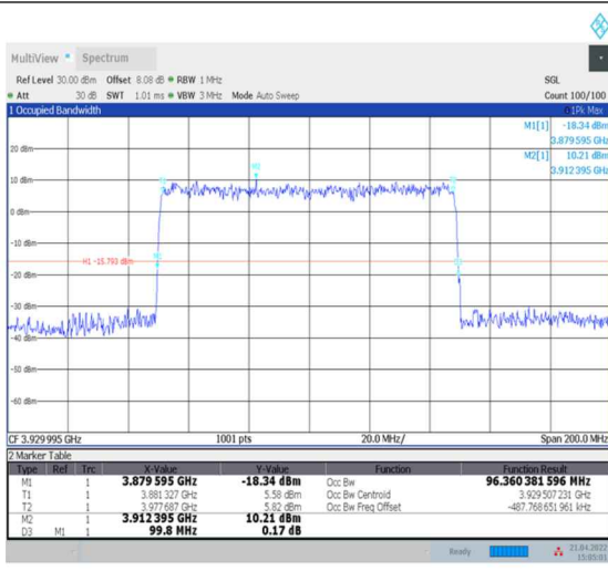
1-N77-3700-3980--30-100-H-5-DFT-256QAM-Outer_Full-270@0-Ant0-96.36-99.800-≤100-PASS
