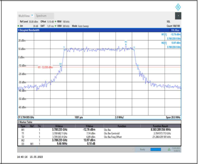
1-N77-3700-3980-PC1-30-10-L-8-CP-64QAM-Outer_Full-24@0-Ant0-8.583-9.460-≤10-PASS
