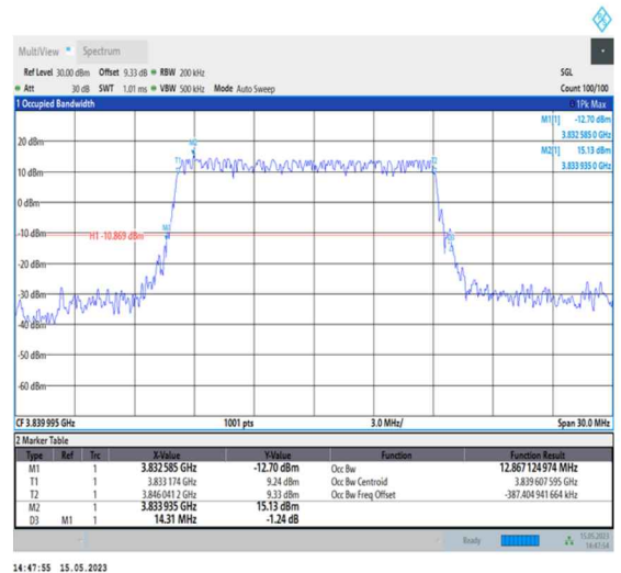
1-N77-3700-3980-PC1-30-15-M-4-DFT-64QAM-Outer_Full-36@0-Ant0-12.867-14.310-≤15-PASS
