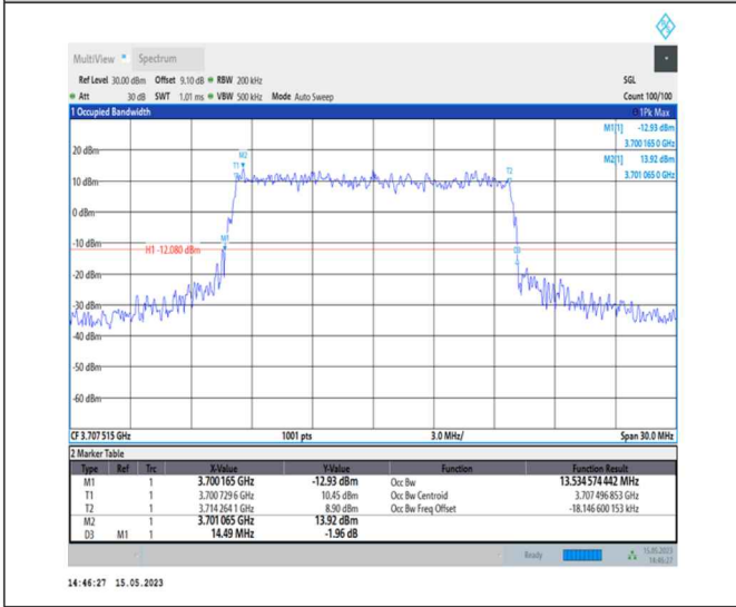
1-N77-3700-3980-PC1-30-15-L-8-CP-64QAM-Outer_Full-38@0-Ant0-13.535-14.490-≤15-PASS
