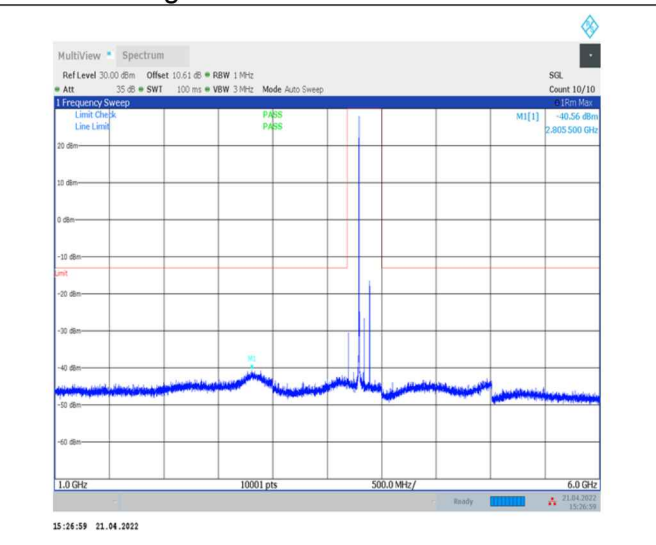
1-N77-3700-3980--30-100-M-1-DFT-PI2BPSK- Inner_1RB_Left-1@1-1000-6000-Ant0--40.56--13- PASS
