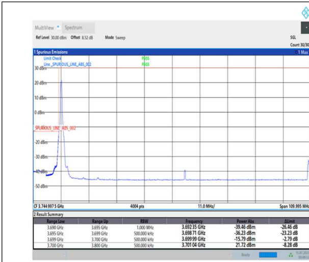
1-N77-3700-3980-PC1-30-100-L-1-DFT-PI2BPSK-Edge_1RB_Left-1@0-Ant0-1--PASS-see graph
