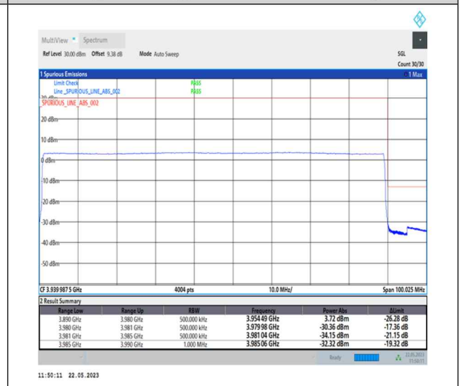
1-N77-3700-3980-PC1-30-90-H-6-CP-QPSK-Outer_Full-245@0-Ant0-1--PASS-see graph
