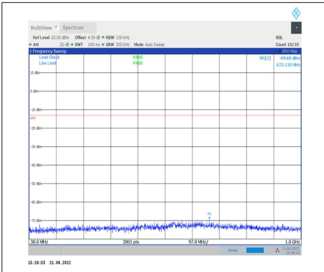
1-N77-3700-3980--30-100-M-1-DFT-PI2BPSK- Inner_1RB_Left-1@1-30-1000-Ant0--69.60--13- PASS
