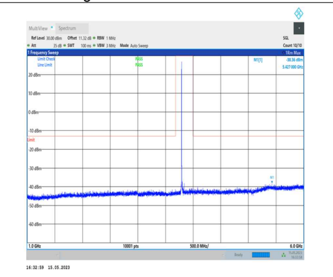
1-N77-3700-3980-PC1-30-100-M-1-DFT-PI2BPSK- Inner_1RB_Left-1@1-1000-6000-Ant0-5427.00--38.36--13-PASS
