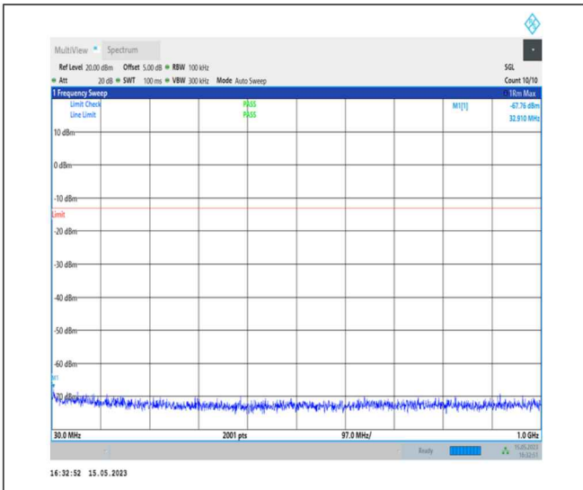
1-N77-3700-3980-PC1-30-100-M-1-DFT-PI2BPSK- Inner_1RB_Left-1@1-30-1000-Ant0-32.91--67.76--13-PASS
