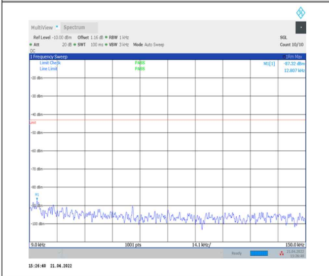
1-N77-3700-3980--30-100-M-1-DFT-PI2BPSK- Inner_1RB_Left-1@1-0.009-0.15-Ant0--87.32--43- PASS
