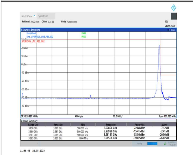
1-N77-3700-3980-PC1-30-90-H-5-CP-QPSK-Edge_1RB_Right-1@244-Ant0-1--PASS-see graph
