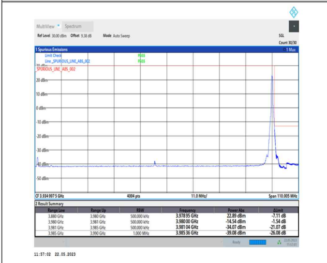
1-N77-3700-3980-PC1-30-100-H-5-CP-QPSK-Edge_1RB_Right-1@272-Ant0-1--PASS-see graph
