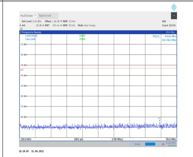
1-N77-3700-3980--30-100-M-1-DFT-PI2BPSK- Inner_1RB_Left-1@1-0.15-30-Ant0--84.63--33-PASS
