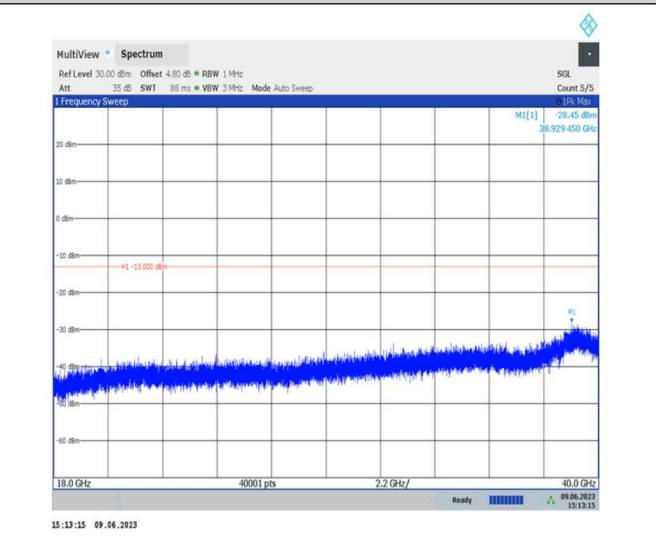
1-N77-3700-3980-PC1-30-100-M-1-DFT-PI2BPSK- Inner_1RB_Left-1@1-18000-40000-Ant0-18000.00--60.70--13-PASS
