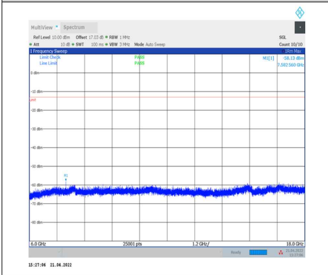
1-N77-3700-3980--30-100-M-1-DFT-PI2BPSK- Inner_1RB_Left-1@1-6000-18000-Ant0--58.13--13- PASS
