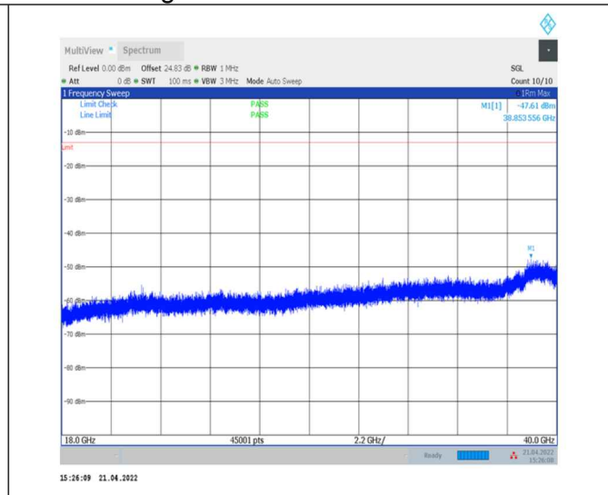
1-N77-3700-3980--30-100-L-1-DFT-PI2BPSK- Inner_1RB_Left-1@1-18000-40000-Ant0--47.61--13- PASS
