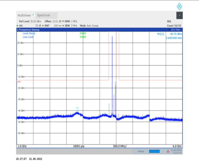
1-N77-3700-3980--30-100-H-1-DFT-PI2BPSK- Inner_1RB_Left-1@1-1000-6000-Ant0--40.75--13- PASS
