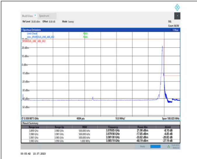
1-N77-3700-3980-PC1-30-90-H-2-DFT-PI2BPSK-Edge_1RB_Right-1@244-Ant0-1--PASS-see graph
