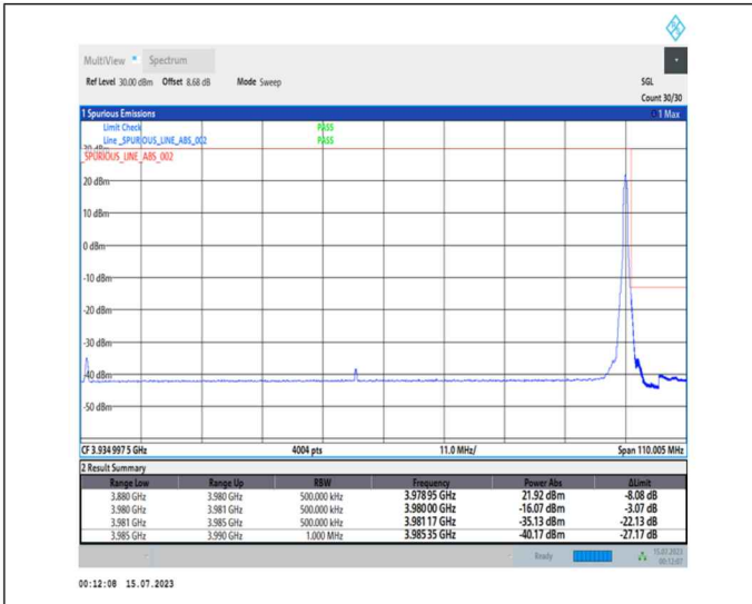
1-N77-3700-3980-PC1-30-100-H-2-DFT-PI2BPSK-Edge_1RB_Right-1@272-Ant0-1--PASS-see graph
