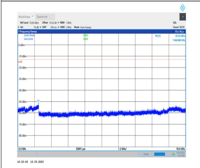
1-N77-3700-3980-PC1-30-100-M-1-DFT-PI2BPSK- Inner_1RB_Left-1@1-6000-18000-Ant0-7466.88--52.52--13-PASS
