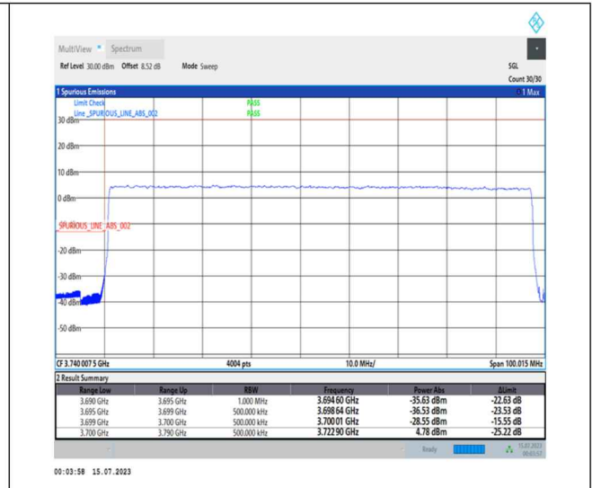
1-N77-3700-3980-PC1-30-90-L-3-DFT-PI2BPSK-Outer_Full-240@0-Ant0-1--PASS-see graph
