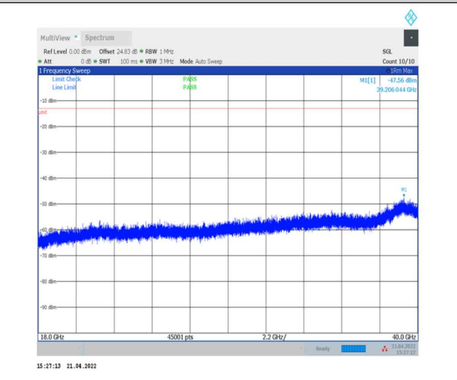
1-N77-3700-3980--30-100-M-1-DFT-PI2BPSK- Inner_1RB_Left-1@1-18000-40000-Ant0--47.56--13- PASS
