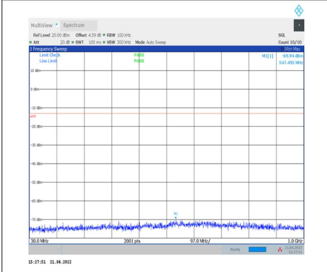
1-N77-3700-3980--30-100-H-1-DFT-PI2BPSK- Inner_1RB_Left-1@1-30-1000-Ant0--69.94--13- PASS
