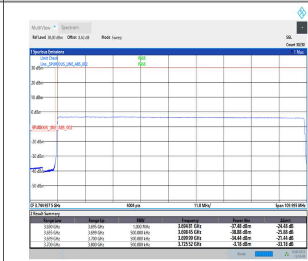
1-N77-3700-3980-PC1-30-100-L-3-DFT-PI2BPSK-Outer_Full-270@0-Ant0-1--PASS-see graph
