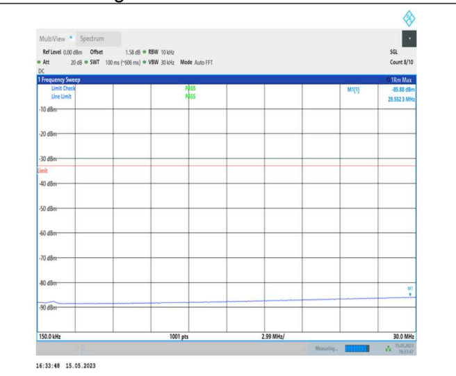
1-N77-3700-3980-PC1-30-100-H-1-DFT-PI2BPSK- Inner_1RB_Left-1@1-0.15-30-Ant0-29.55--85.88--33- PASS
