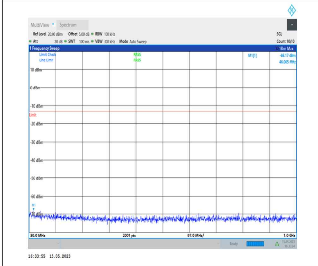
1-N77-3700-3980-PC1-30-100-H-1-DFT-PI2BPSK- Inner_1RB_Left-1@1-30-1000-Ant0-46.01--68.17-- 13-PASS
