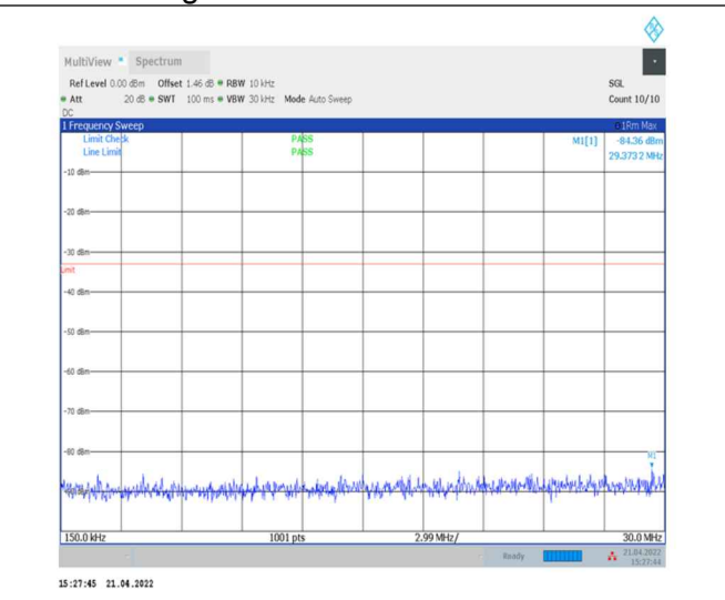
1-N77-3700-3980--30-100-H-1-DFT-PI2BPSK- Inner_1RB_Left-1@1-0.15-30-Ant0--84.36--33-PASS
