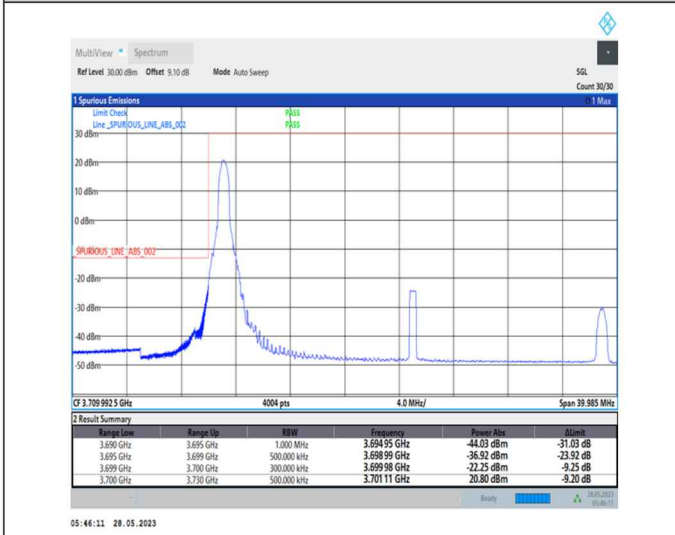
1-N77-3700-3980-PC1-30-30-L-4-CP-QPSK-Edge_1RB_Left-1@0-Ant0-1--PASS-see graph
