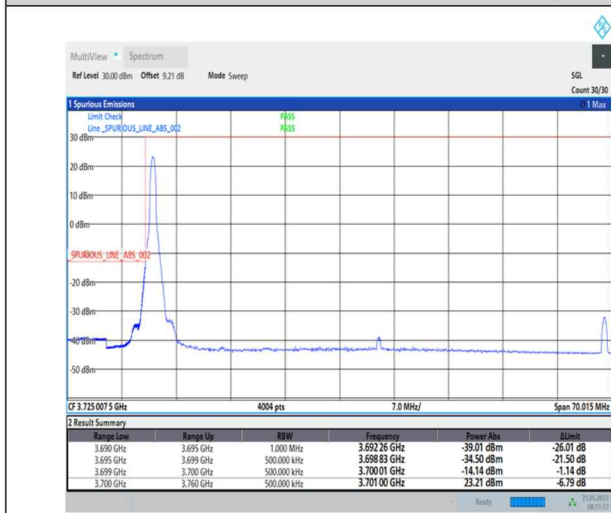
1-N77-3700-3980-PC1-30-60-L-1-DFT-PI2BPSK-Edge_1RB_Left-1@0-Ant0-1--PASS-see graph
