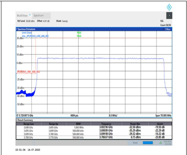
1-N77-3700-3980-PC1-30-70-L-3-DFT-PI2BPSK-Outer_Full-180@0-Ant0-1--PASS-see graph
