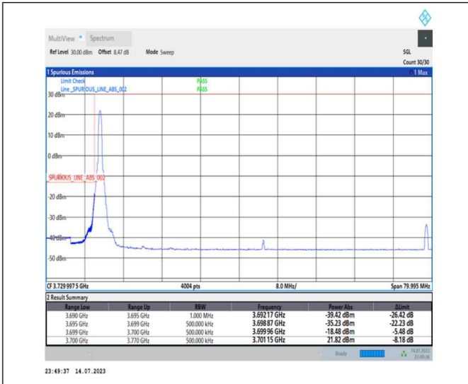
1-N77-3700-3980-PC1-30-70-L-1-DFT-PI2BPSK-Edge_1RB_Left-1@0-Ant0-1--PASS-see graph
