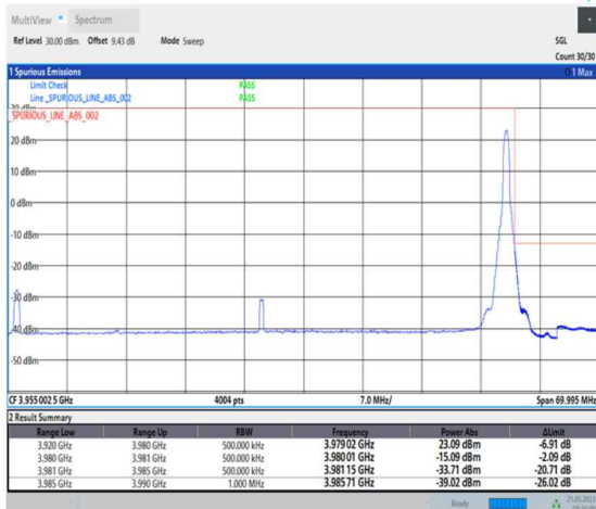
1-N77-3700-3980-PC1-30-60-H-5-CP-QPSK-Edge_1RB_Right-1@161-Ant0-1--PASS-see graph
