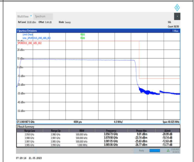
1-N77-3700-3980-PC1-30-30-H-6-CP-QPSK-Outer_Full-78@0-Ant0-1--PASS-see graph
