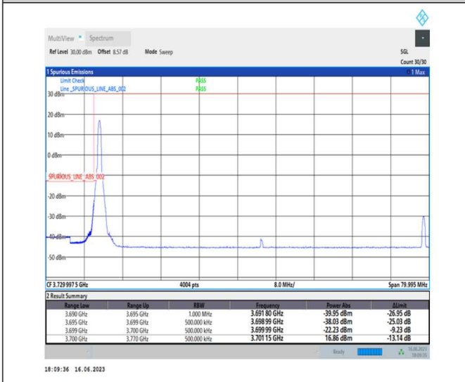
1-N77-3700-3980-PC1-30-70-L-4-CP-QPSK-Edge_1RB_Left-1@0-Ant0-1--PASS-see graph
