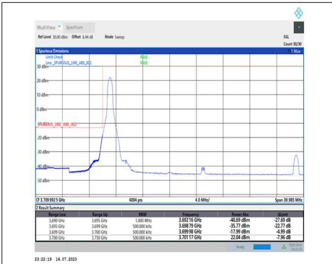
1-N77-3700-3980-PC1-30-30-L-1-DFT-PI2BPSK-Edge_1RB_Left-1@0-Ant0-1--PASS-see graph
