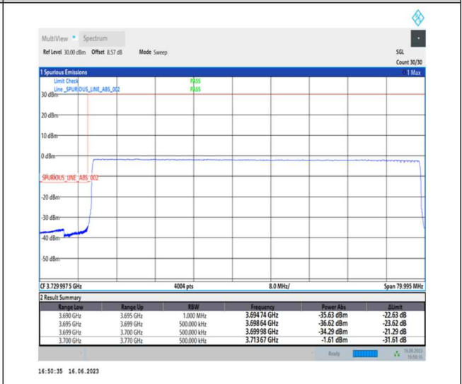
1-N77-3700-3980-PC1-30-70-L-6-CP-QPSK-Outer_Full-189@0-Ant0-1--PASS-see graph
