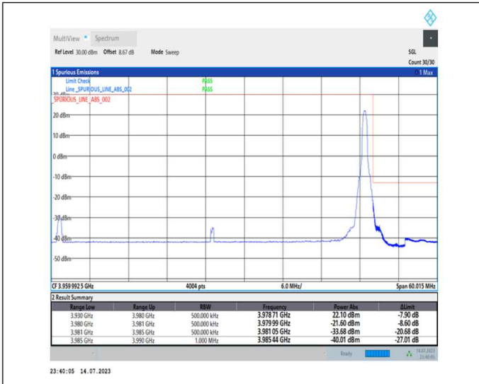
1-N77-3700-3980-PC1-30-50-H-2-DFT-PI2BPSK-Edge_1RB_Right-1@132-Ant0-1--PASS-see graph
