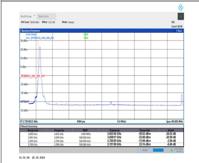
1-N77-3700-3980-PC1-30-80-L-4-CP-QPSK-Edge_1RB_Left-1@0-Ant0-1--PASS-see graph
