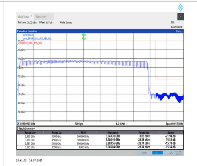
1-N77-3700-3980-PC1-30-50-H-3-DFT-PI2BPSK-Outer_Full-128@0-Ant0-1--PASS-see graph
