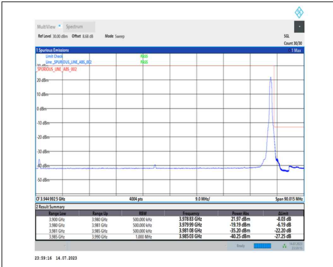
1-N77-3700-3980-PC1-30-80-H-2-DFT-PI2BPSK-Edge_1RB_Right-1@216-Ant0-1--PASS-see graph
