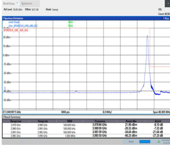
1-N77-3700-3980-PC1-30-70-H-2-DFT-PI2BPSK-Edge_1RB_Right-1@188-Ant0-1--PASS-see graph
