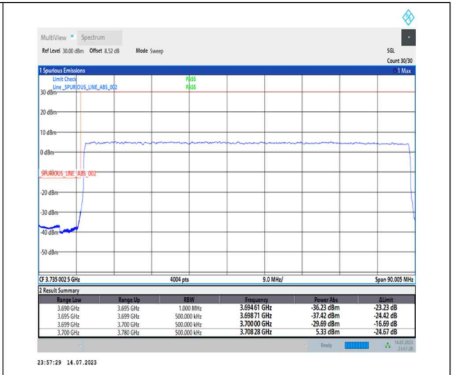
1-N77-3700-3980-PC1-30-80-L-3-DFT-PI2BPSK-Outer_Full-216@0-Ant0-1--PASS-see graph
