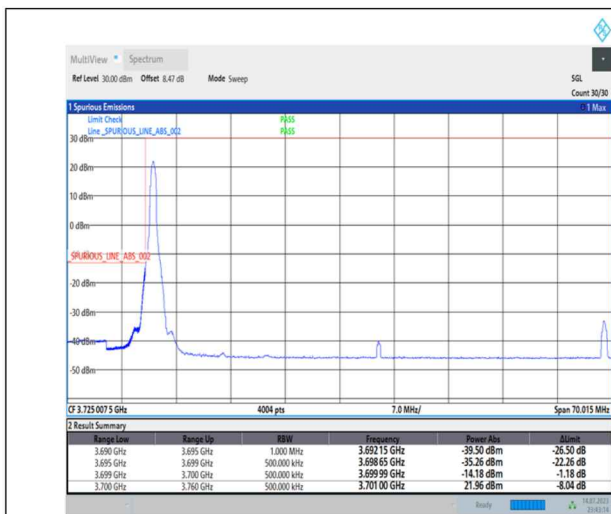
1-N77-3700-3980-PC1-30-60-L-1-DFT-PI2BPSK-Edge_1RB_Left-1@0-Ant0-1--PASS-see graph
