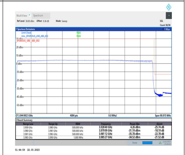
1-N77-3700-3980-PC1-30-80-H-6-CP-QPSK-Outer_Full-217@0-Ant0-1--PASS-see graph
