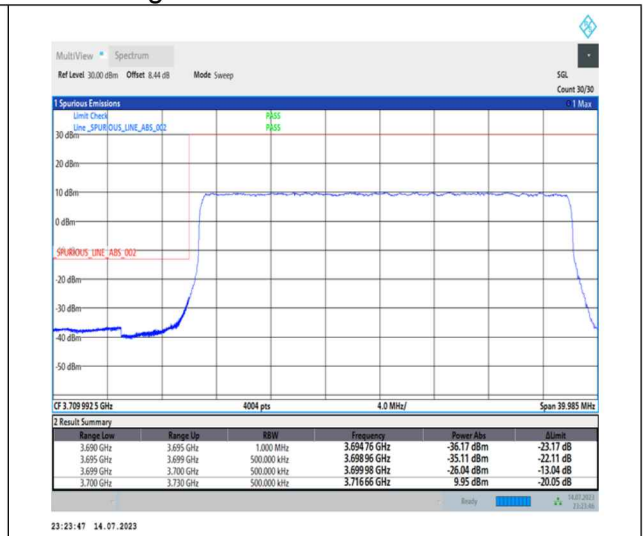
1-N77-3700-3980-PC1-30-30-L-3-DFT-PI2BPSK-Outer_Full-75@0-Ant0-1--PASS-see graph
