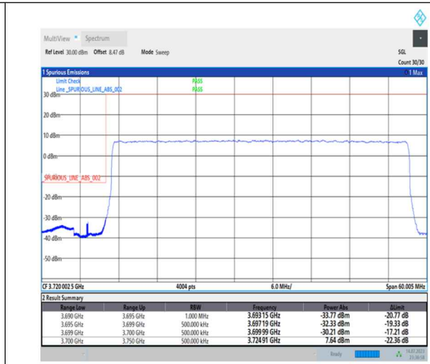
1-N77-3700-3980-PC1-30-50-L-3-DFT-PI2BPSK-Outer_Full-128@0-Ant0-1--PASS-see graph
