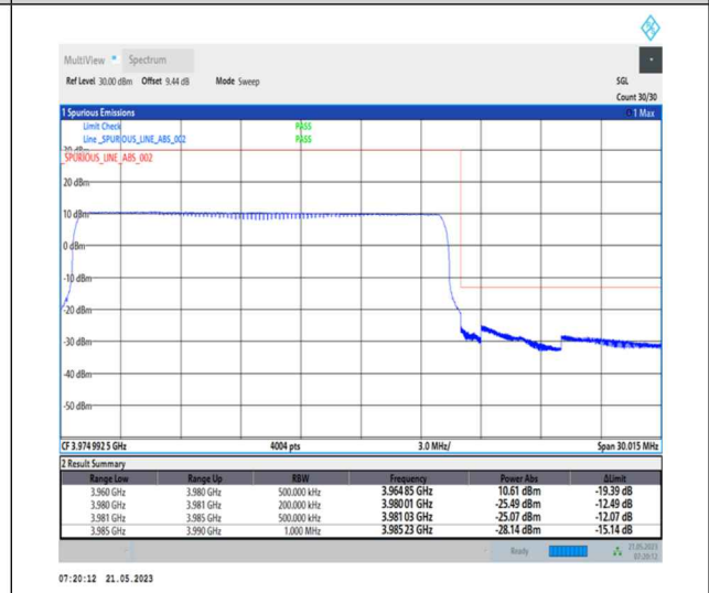
1-N77-3700-3980-PC1-30-20-H-6-CP-QPSK-Outer_Full-51@0-Ant0-1--PASS-see graph
