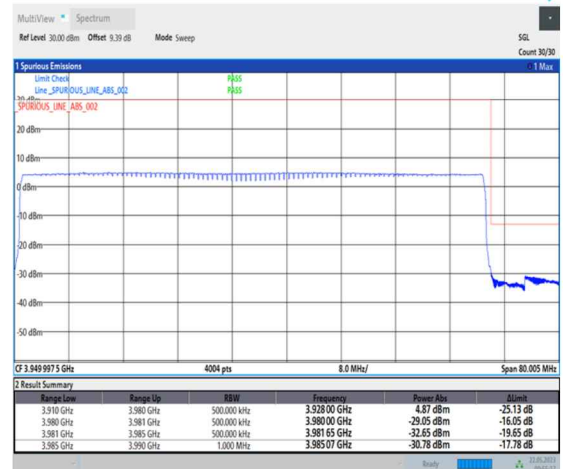
1-N77-3700-3980-PC1-30-70-H-6-CP-QPSK-Outer_Full-189@0-Ant0-1--PASS-see graph
