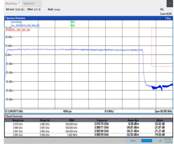
1-N77-3700-3980-PC1-30-70-H-3-DFT-PI2BPSK-Outer_Full-180@0-Ant0-1--PASS-see graph
