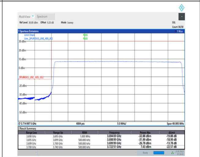
1-N77-3700-3980-PC1-30-40-L-3-DFT-PI2BPSK-Outer_Full-100@0-Ant0-1--PASS-see graph
