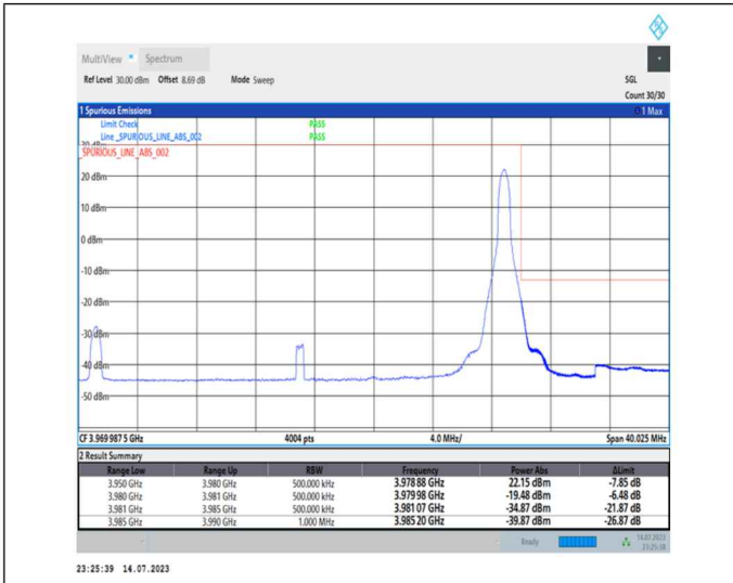
1-N77-3700-3980-PC1-30-30-H-2-DFT-PI2BPSK-Edge_1RB_Right-1@77-Ant0-1--PASS-see graph
