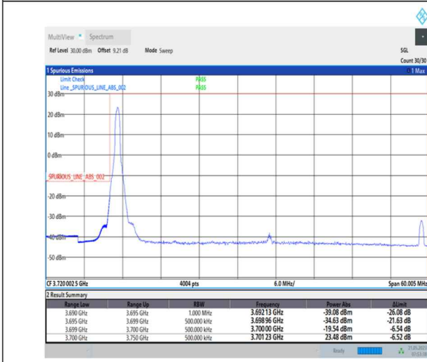
1-N77-3700-3980-PC1-30-50-L-1-DFT-PI2BPSK-Edge_1RB_Left-1@0-Ant0-1--PASS-see graph
