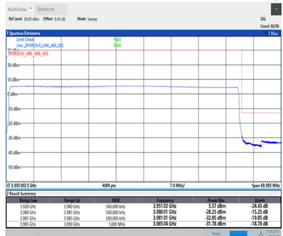
1-N77-3700-3980-PC1-30-60-H-6-CP-QPSK-Outer_Full-162@0-Ant0-1--PASS-see graph
