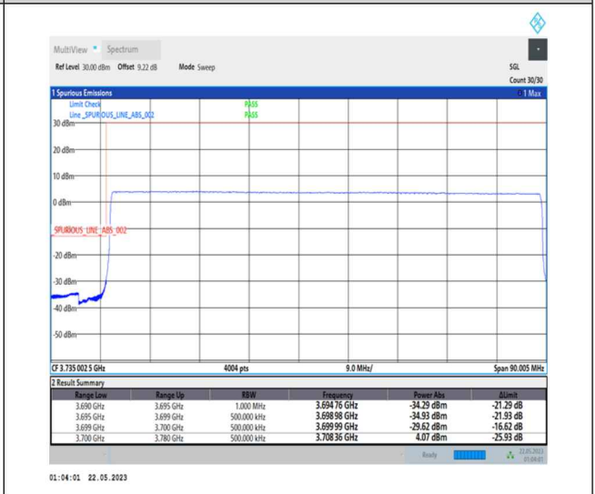
1-N77-3700-3980-PC1-30-80-L-6-CP-QPSK-Outer_Full-217@0-Ant0-1--PASS-see graph
