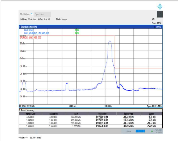
1-N77-3700-3980-PC1-30-20-H-5-CP-QPSK-Edge_1RB_Right-1@50-Ant0-1--PASS-see graph
