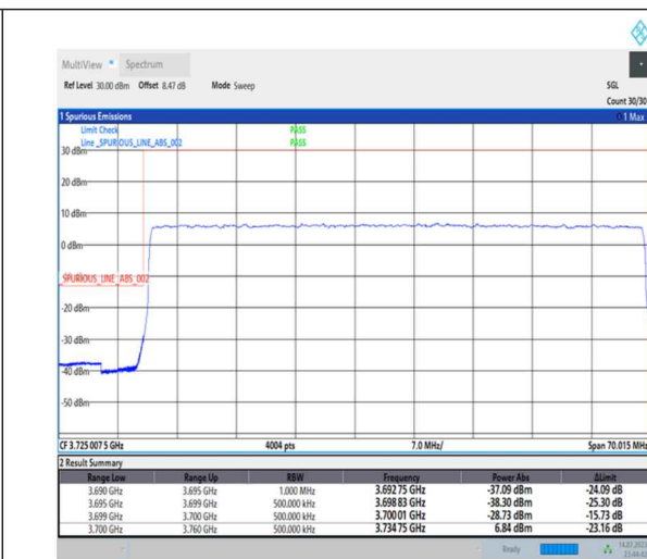
1-N77-3700-3980-PC1-30-60-L-3-DFT-PI2BPSK-Outer_Full-162@0-Ant0-1--PASS-see graph
