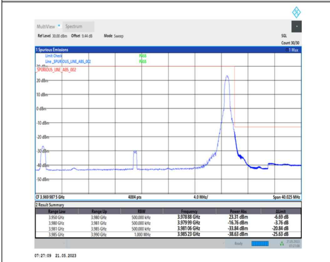
1-N77-3700-3980-PC1-30-30-H-5-CP-QPSK-Edge_1RB_Right-1@77-Ant0-1--PASS-see graph
