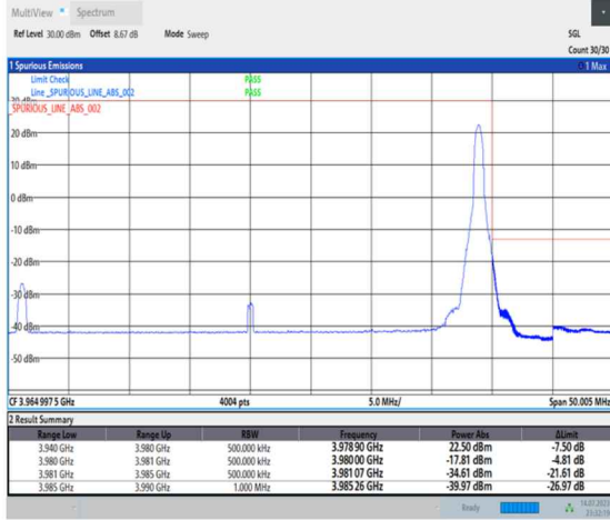
1-N77-3700-3980-PC1-30-40-H-2-DFT-PI2BPSK-Edge_1RB_Right-1@105-Ant0-1--PASS-see graph
