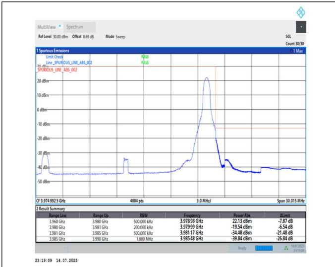
1-N77-3700-3980-PC1-30-20-H-2-DFT-PI2BPSK-Edge_1RB_Right-1@50-Ant0-1--PASS-see graph
