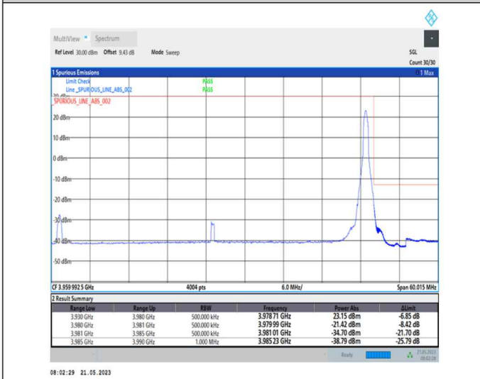
1-N77-3700-3980-PC1-30-50-H-5-CP-QPSK-Edge_1RB_Right-1@132-Ant0-1--PASS-see graph
