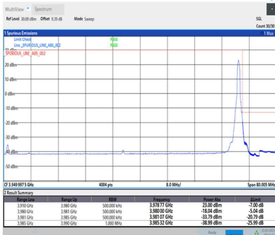
1-N77-3700-3980-PC1-30-70-H-5-CP-QPSK-Edge_1RB_Right-1@188-Ant0-1--PASS-see graph
