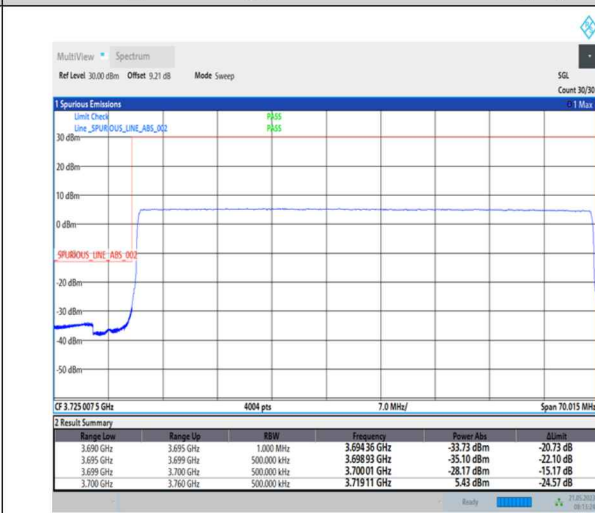
1-N77-3700-3980-PC1-30-60-L-3-DFT-PI2BPSK-Outer_Full-162@0-Ant0-1--PASS-see graph
