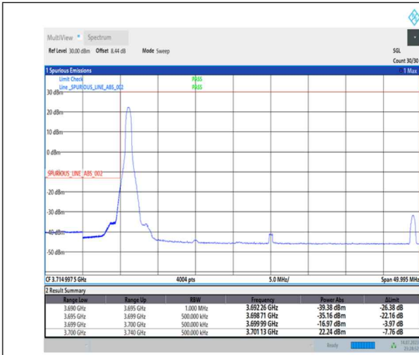
1-N77-3700-3980-PC1-30-40-L-1-DFT-PI2BPSK-Edge_1RB_Left-1@0-Ant0-1--PASS-see graph
