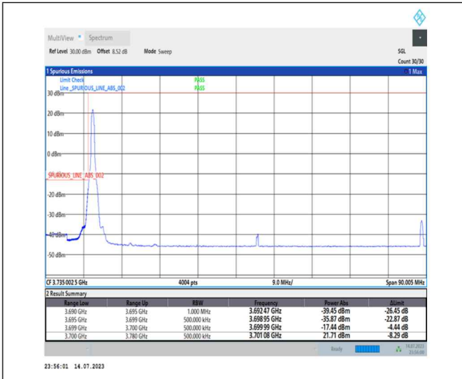
1-N77-3700-3980-PC1-30-80-L-1-DFT-PI2BPSK-Edge_1RB_Left-1@0-Ant0-1--PASS-see graph
