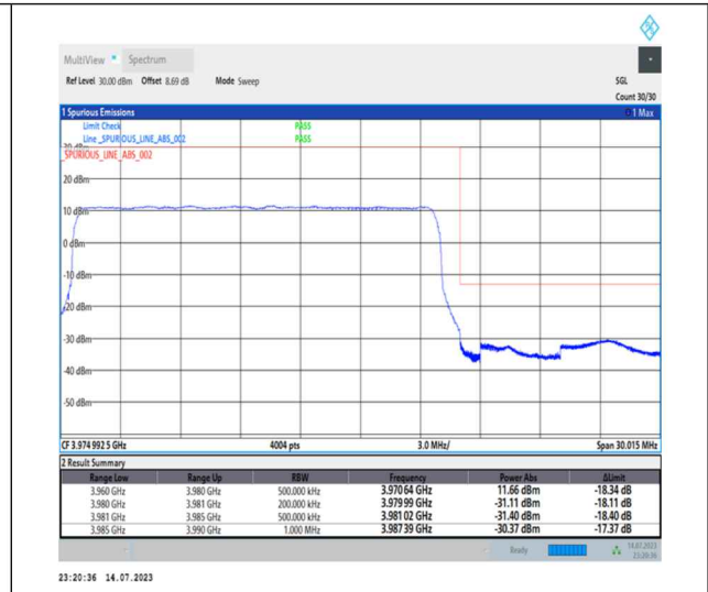
1-N77-3700-3980-PC1-30-20-H-3-DFT-PI2BPSK-Outer_Full-50@0-Ant0-1--PASS-see graph
