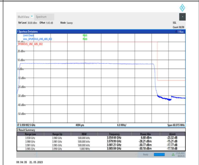
1-N77-3700-3980-PC1-30-50-H-6-CP-QPSK-Outer_Full-133@0-Ant0-1--PASS-see graph
