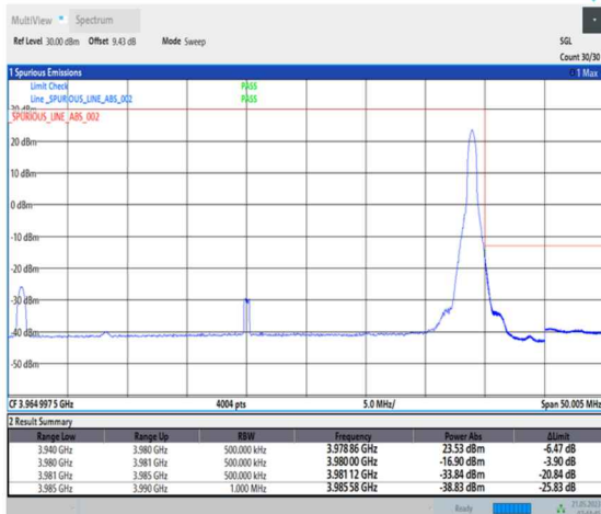
1-N77-3700-3980-PC1-30-40-H-5-CP-QPSK-Edge_1RB_Right-1@105-Ant0-1--PASS-see graph
