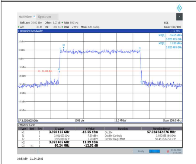
1-N77-3700-3980--30-60-H-3-DFT-16QAM- Outer_Full-162@0-Ant0-57.925-60.240-≤60-PASS
