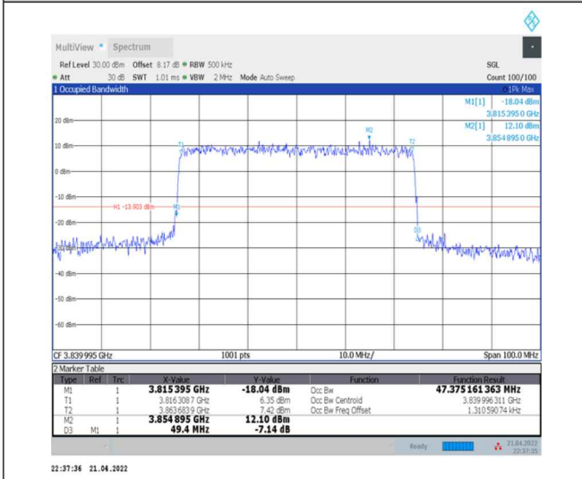
1-N77-3700-3980--30-50-M-7-CP-16QAM-Outer_Full-133@0-Ant0-47.375-49.400-≤50-PASS
