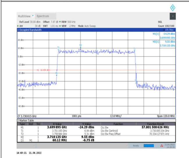
1-N77-3700-3980--30-60-L-5-DFT-256QAM-Outer_Full-162@0-Ant0-57.802-60.120-≤60-PASS
