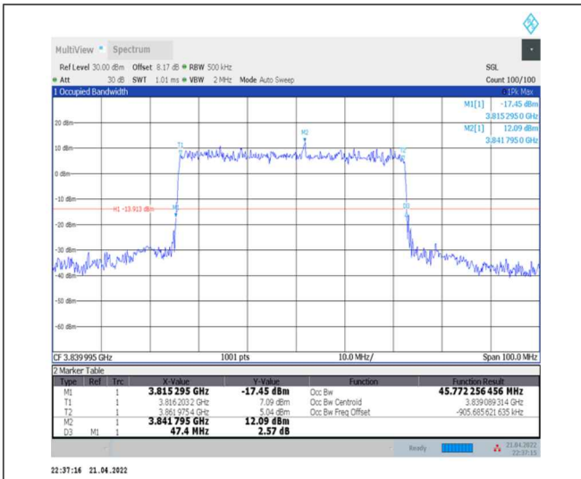
1-N77-3700-3980--30-50-M-5-DFT-256QAM-Outer_Full-128@0-Ant0-45.772-47.400-≤50-PASS
