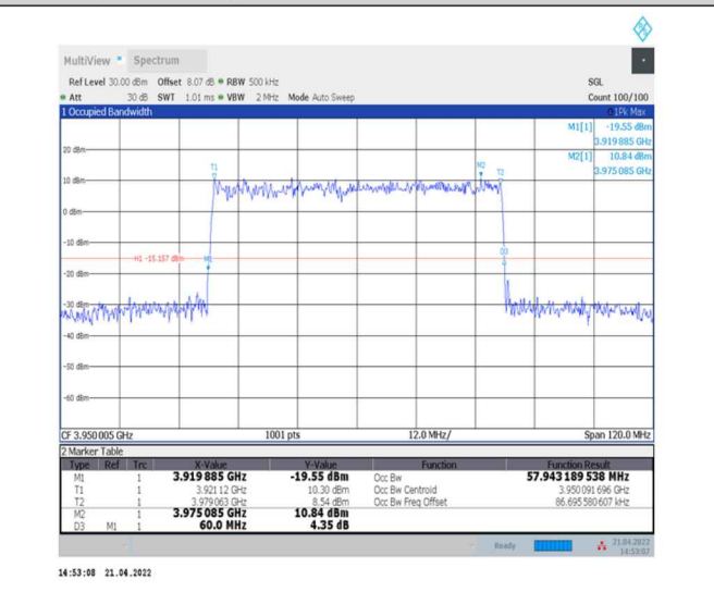
1-N77-3700-3980--30-60-H-4-DFT-64QAM- Outer_Full-162@0-Ant0-57.943-60.000-≤60-PASS
