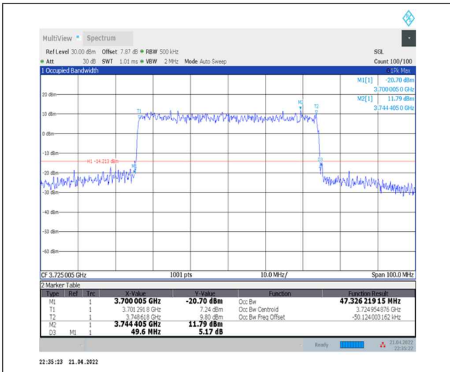
1-N77-3700-3980--30-50-L-6-CP-QPSK-Outer_Full-133@0-Ant0-47.326-49.600-≤50-PASS
