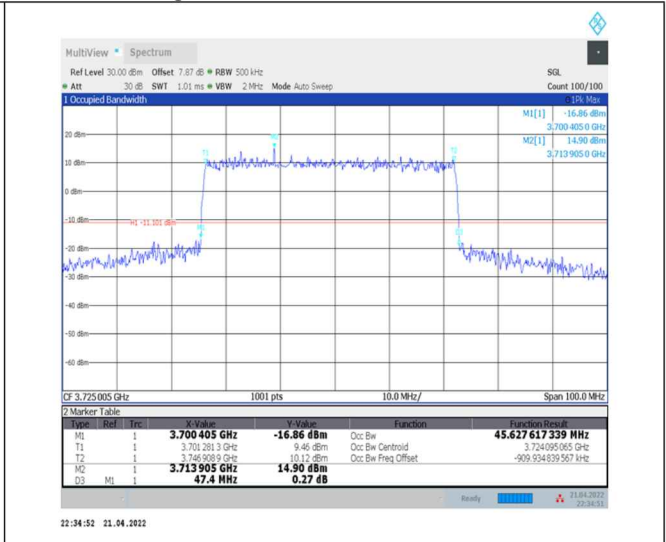
1-N77-3700-3980--30-50-L-3-DFT-16QAM-Outer_Full-128@0-Ant0-45.628-47.400-≤50-PASS
