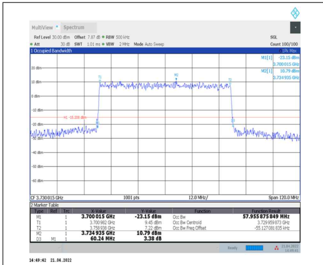
1-N77-3700-3980--30-60-L-7-CP-16QAM-Outer_Full-162@0-Ant0-57.956-60.240-≤60-PASS
