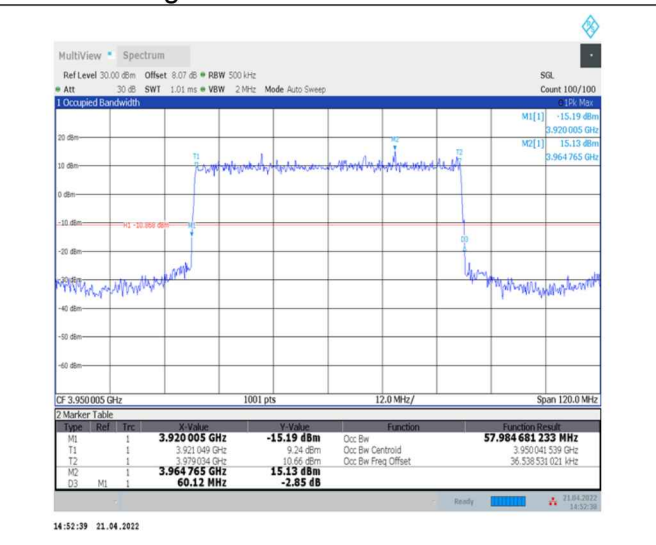
1-N77-3700-3980--30-60-H-2-DFT-PI2BPSK- Outer_Full-162@0-Ant0-57.985-60.120-≤60-PASS
