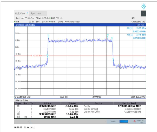
1-N77-3700-3980--30-60-H-1-DFT-QPSK- Outer_Full-162@0-Ant0-57.938-59.880-≤60-PASS
