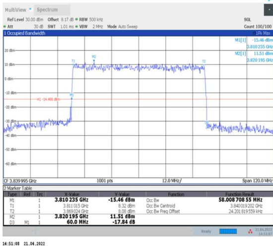
1-N77-3700-3980--30-60-M-4-DFT-64QAM-Outer_Full-162@0-Ant0-58.009-60.000-≤60-PASS
