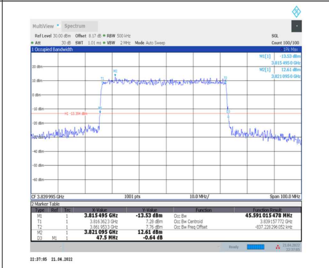
1-N77-3700-3980--30-50-M-4-DFT-64QAM-Outer_Full-128@0-Ant0-45.591-47.500-≤50-PASS
