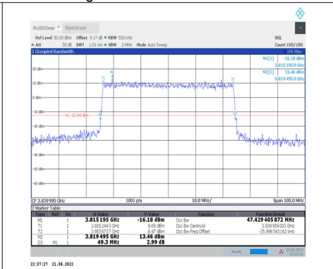
1-N77-3700-3980--30-50-M-6-CP-QPSK-Outer_Full-133@0-Ant0-47.429-49.300-≤50-PASS
