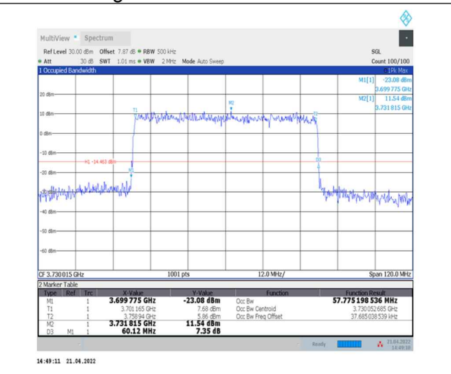
1-N77-3700-3980--30-60-L-4-DFT-64QAM-Outer_Full-162@0-Ant0-57.775-60.120-≤60-PASS
