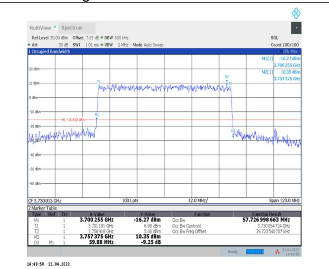
1-N77-3700-3980--30-60-L-8-CP-64QAM-Outer_Full-162@0-Ant0-57.727-59.880-≤60-PASS
