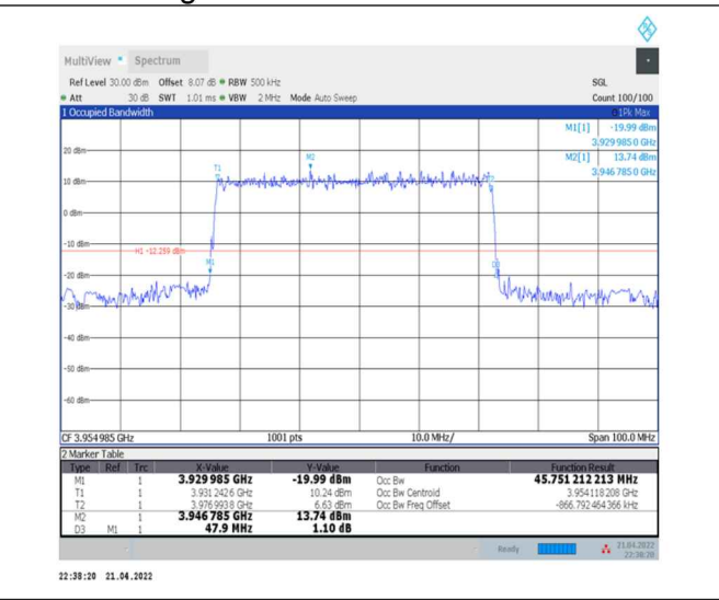
1-N77-3700-3980--30-50-H-1-DFT-QPSK-Outer_Full-128@0-Ant0-45.751-47.900-≤50-PASS
