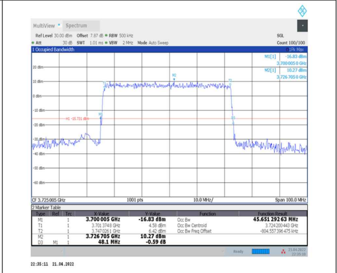
1-N77-3700-3980--30-50-L-5-DFT-256QAM-Outer_Full-128@0-Ant0-45.651-48.100-≤50-PASS
