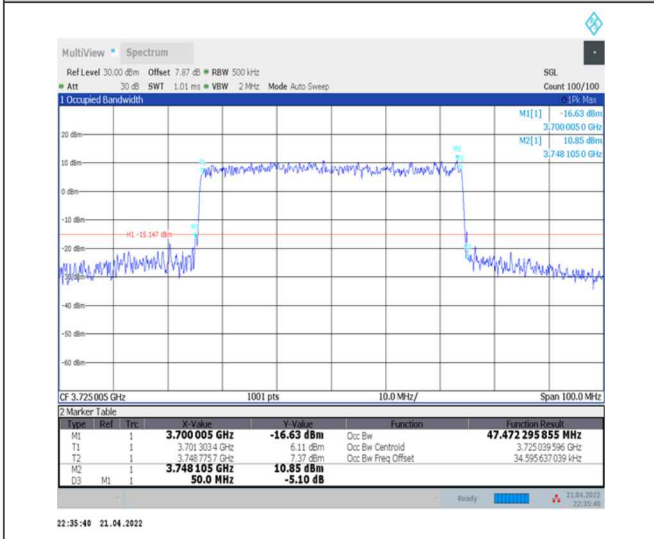
1-N77-3700-3980--30-50-L-8-CP-64QAM-Outer_Full-133@0-Ant0-47.472-50.000-≤50-PASS
