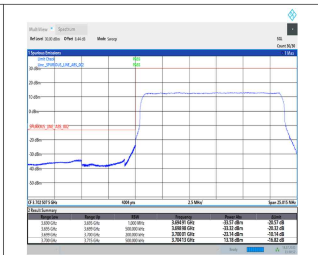
1-N77-3700-3980-PC1-30-15-L-3-DFT-PI2BPSK-Outer_Full-36@0-Ant0-1--PASS-see graph
