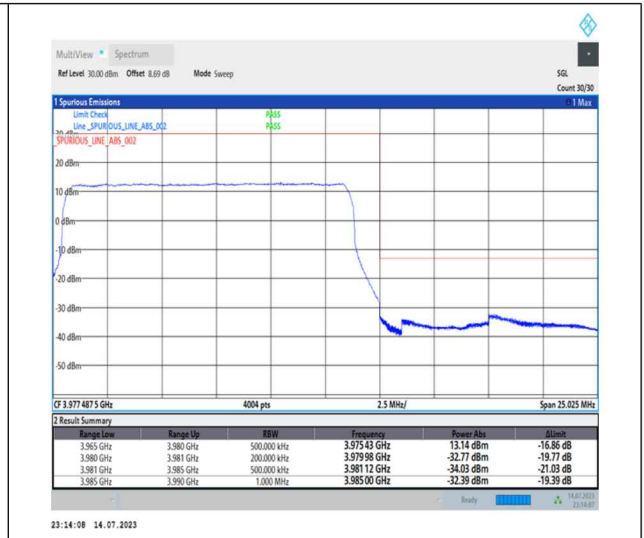
1-N77-3700-3980-PC1-30-15-H-3-DFT-PI2BPSK-Outer_Full-36@0-Ant0-1--PASS-see graph
