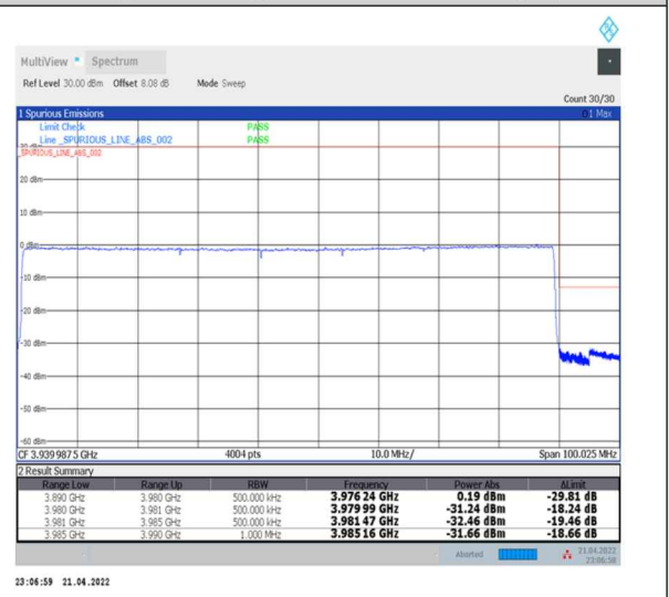
1-N77-3700-3980--30-90-H-6-CP-QPSK-Outer_Full-245@0-Ant0-PASS-see graph
