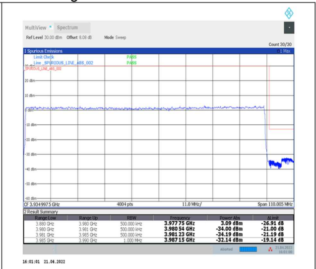
1-N77-3700-3980--30-100-H-3-DFT-PI2BPSK-Outer_Full-270@0-Ant0-PASS-see graph
