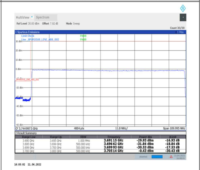
1-N77-3700-3980--30-100-L-6-CP-QPSK-Outer_Full-273@0-Ant0-PASS-see graph
