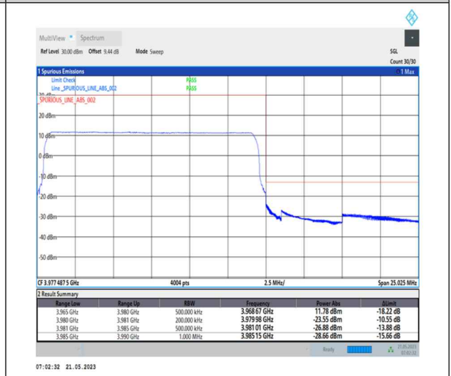
1-N77-3700-3980-PC1-30-15-H-6-CP-QPSK-Outer_Full-38@0-Ant0-1--PASS-see graph
