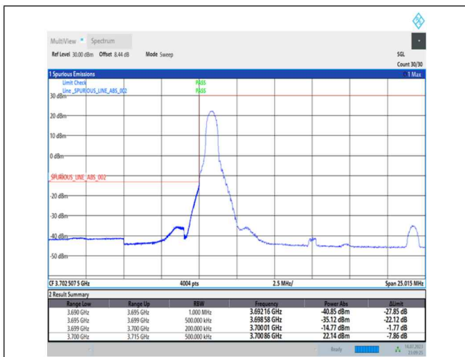
1-N77-3700-3980-PC1-30-15-L-1-DFT-PI2BPSK-Edge_1RB_Left-1@0-Ant0-1--PASS-see graph
