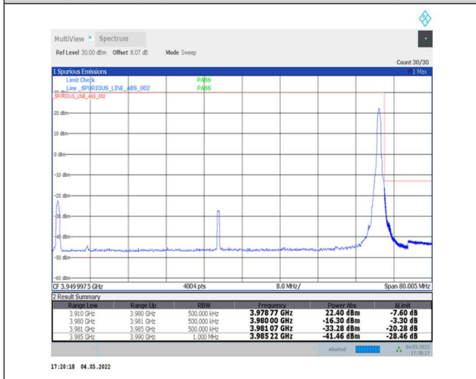
1-N77-3700-3980-30-70-H-5-CP-QPSK-Edge_1RB_Right-1@188-Ant0-PASS-see graph
