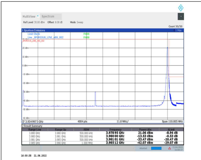
1-N77-3700-3980--30-100-H-2-DFT-PI2BPSK-Edge_1RB_Right-1@272-Ant0-PASS-see graph
