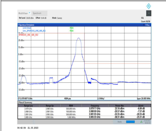
1-N77-3700-3980-PC1-30-10-H-5-CP-QPSK-Edge_1RB_Right-1@23-Ant0-1--PASS-see graph
