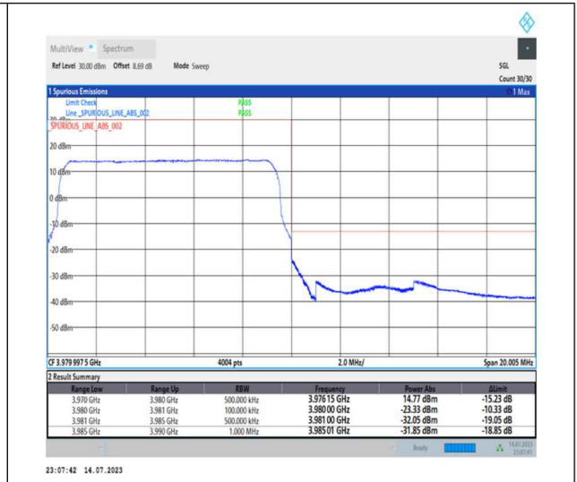
1-N77-3700-3980-PC1-30-10-H-3-DFT-PI2BPSK-Outer_Full-24@0-Ant0-1--PASS-see graph
