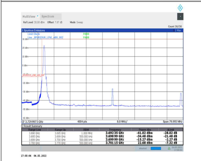
1-N77-3700-3980--30-70-L-4-CP-QPSK-Edge_1RB_Left-1@0-Ant0-PASS-see graph
