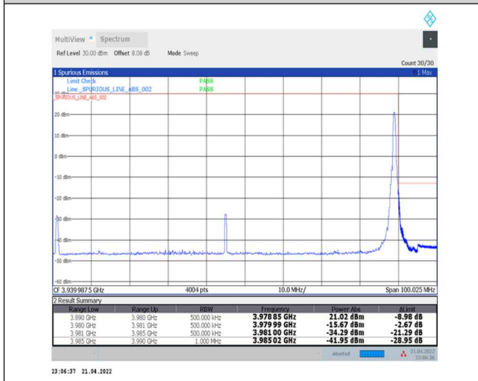
1-N77-3700-3980--30-90-H-5-CP-QPSK-Edge_1RB_Right-1@244-Ant0-PASS-see graph
