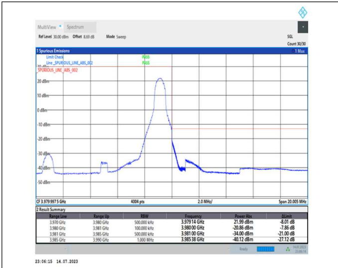
1-N77-3700-3980-PC1-30-10-H-2-DFT-PI2BPSK-Edge_1RB_Right-1@23-Ant0-1--PASS-see graph
