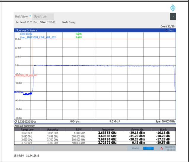
1-N77-3700-3980--30-80-L-6-CP-QPSK-Outer_Full-217@0-Ant0-PASS-see graph
