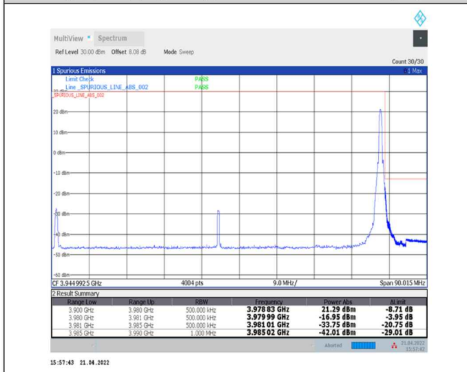
1-N77-3700-3980--30-80-H-5-CP-QPSK-Edge_1RB_Right-1@216-Ant0-PASS-see graph
