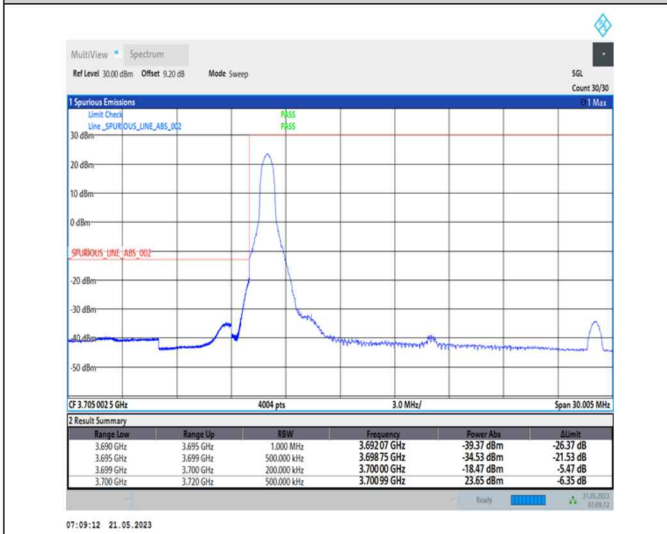
1-N77-3700-3980-PC1-30-20-L-4-CP-QPSK-Edge_1RB_Left-1@0-Ant0-1--PASS-see graph
