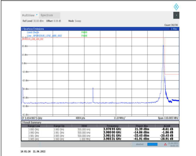
1-N77-3700-3980--30-100-H-5-CP-QPSK-Edge_1RB_Right-1@272-Ant0-PASS-see graph
