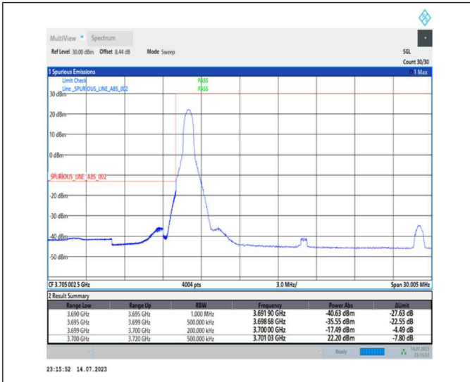
1-N77-3700-3980-PC1-30-20-L-1-DFT-PI2BPSK-Edge_1RB_Left-1@0-Ant0-1--PASS-see graph
