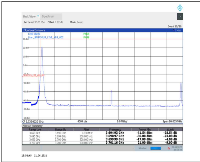
1-N77-3700-3980--30-80-L-1-DFT-PI2BPSK-Edge_1RB_Left-1@0-Ant0-PASS-see graph
