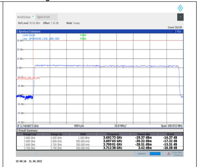
1-N77-3700-3980--30-90-L-3-DFT-PI2BPSK-Outer_Full-240@0-Ant0-PASS-see graph
