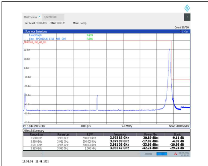
1-N77-3700-3980--30-80-H-2-DFT-PI2BPSK-Edge_1RB_Right-1@216-Ant0-PASS-see graph
