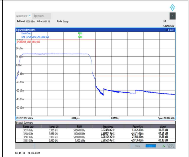
1-N77-3700-3980-PC1-30-10-H-6-CP-QPSK-Outer_Full-24@0-Ant0-1--PASS-see graph
