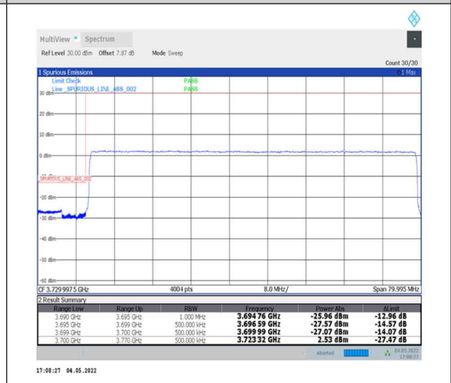
1-N77-3700-3980--30-70-L-6-CP-QPSK-Outer_Full-189@0-Ant0-PASS-see graph
