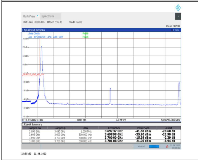
1-N77-3700-3980--30-80-L-4-CP-QPSK-Edge_1RB_Left-1@0-Ant0-PASS-see graph
