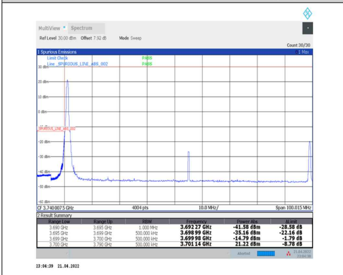
1-N77-3700-3980--30-90-L-4-CP-QPSK-Edge_1RB_Left-1@0-Ant0-PASS-see graph
