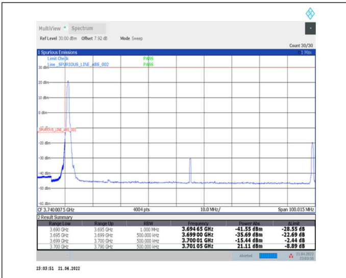
1-N77-3700-3980--30-90-L-1-DFT-PI2BPSK-Edge_1RB_Left-1@0-Ant0-PASS-see graph
