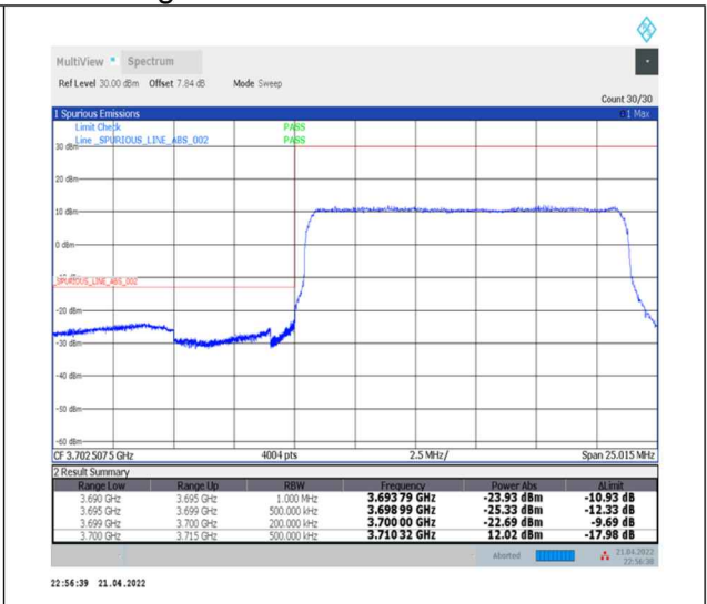
1-N77-3700-3980--30-15-L-3-DFT-PI2BPSK-Outer_Full-36@0-Ant0-PASS-see graph
