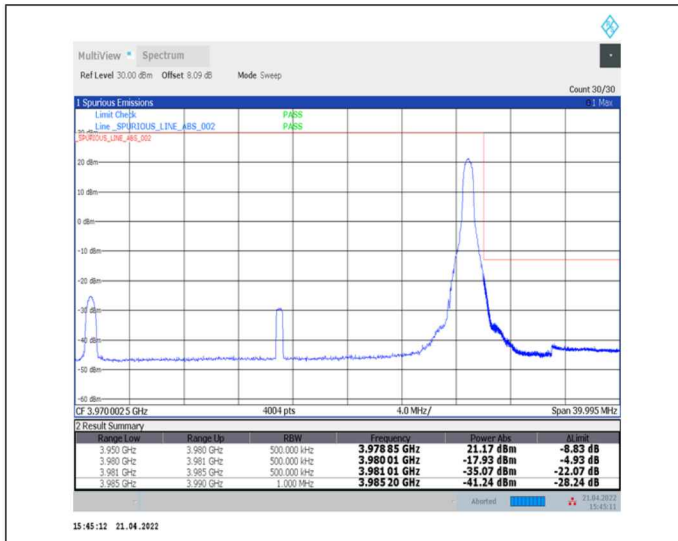
1-N77-3700-3980-30-30-H-2-DFT-PI2BPSK-Edge_1RB_Right-1@77-Ant0-PASS-see graph
