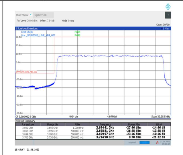
1-N77-3700-3980--30-30-L-3-DFT-PI2BPSK-Outer_Full-75@0-Ant0-PASS-see graph
