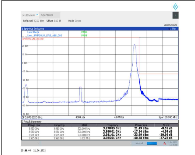
1-N77-3700-3980-30-30-H-5-CP-QPSK-Edge_1RB_Right-1@77-Ant0-PASS-see graph
