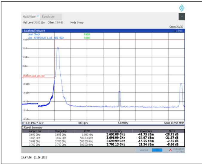
1-N77-3700-3980--30-40-L-1-DFT-PI2BPSK-Edge_1RB_Left-1@0-Ant0-PASS-see graph
