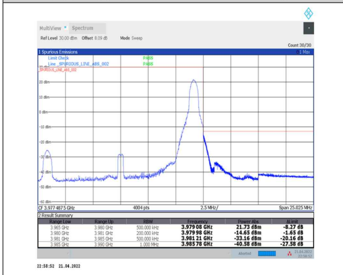
1-N77-3700-3980-30-15-H-5-CP-QPSK-Edge_1RB_Right-1@37-Ant0-PASS-see graph
