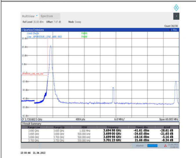
1-N77-3700-3980--30-50-L-4-CP-QPSK-Edge_1RB_Left-1@0-Ant0-PASS-see graph
