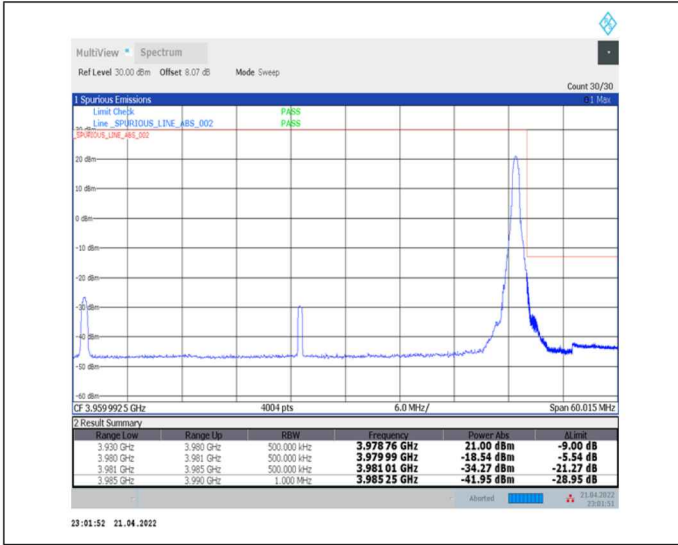
1-N77-3700-3980--30-50-H-2-DFT-PI2BPSK-Edge_1RB_Right-1@132-Ant0-PASS-see graph
