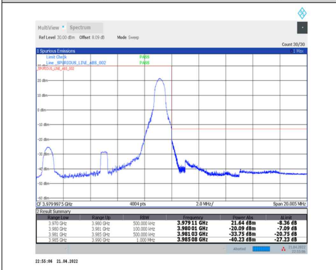
1-N77-3700-3980-30-10-H-5-CP-QPSK-Edge_1RB_Right-1@23-Ant0-PASS-see graph
