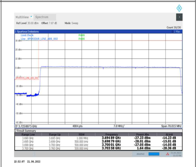
1-N77-3700-3980--30-60-L-6-CP-QPSK-Outer_Full-162@0-Ant0-PASS-see graph
