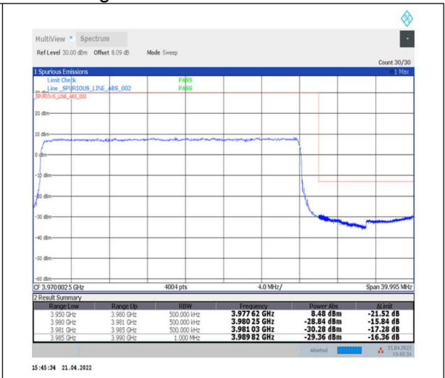
1-N77-3700-3980-30-30-H-3-DFT-PI2BPSK-Outer_Full-75@0-Ant0-PASS-see graph
