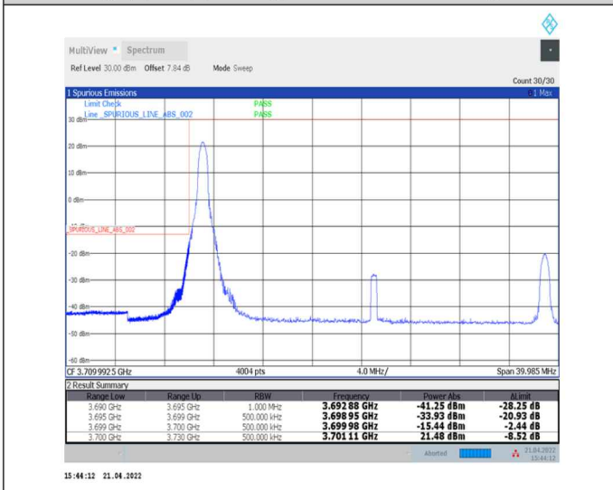
1-N77-3700-3980--30-30-L-4-CP-QPSK-Edge_1RB_Left-1@0-Ant0-PASS-see graph
