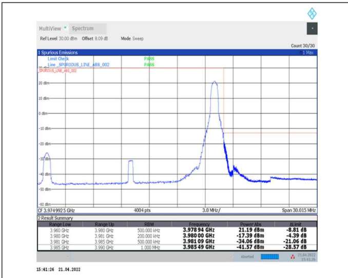
1-N77-3700-3980-30-20-H-2-DFT-PI2BPSK-Edge_1RB_Right-1@50-Ant0-PASS-see graph
