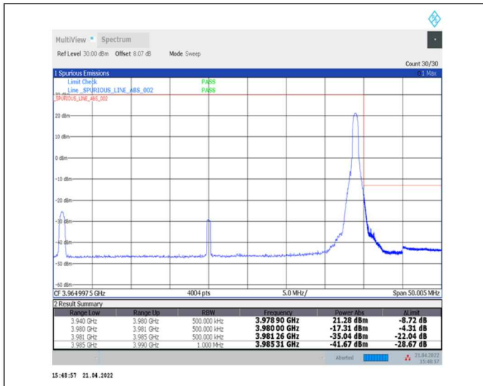
1-N77-3700-3980--30-40-H-2-DFT-PI2BPSK-Edge_1RB_Right-1@105-Ant0-PASS-see graph
