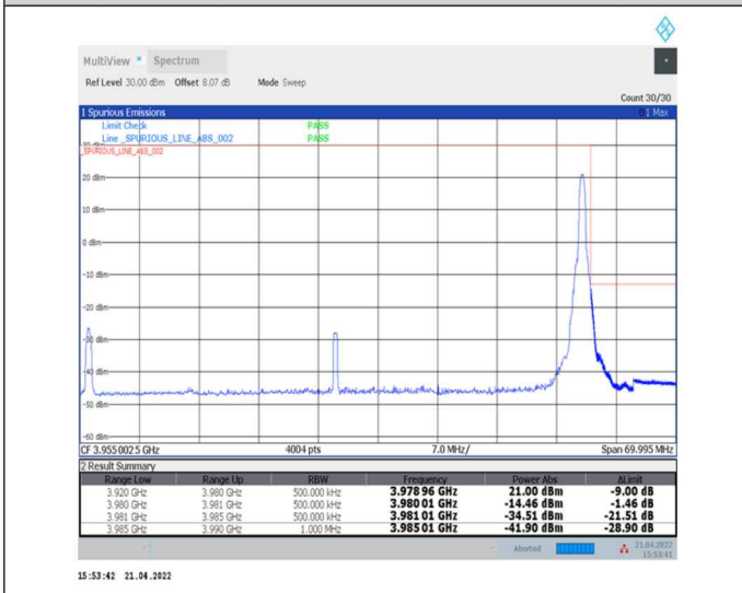
1-N77-3700-3980--30-60-H-5-CP-QPSK-Edge_1RB_Right-1@161-Ant0-PASS-see graph
