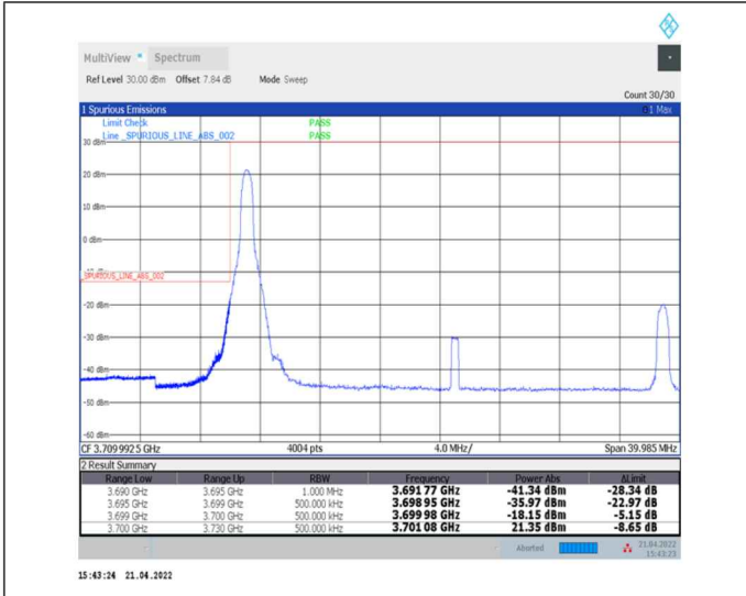
1-N77-3700-3980--30-30-L-1-DFT-PI2BPSK-Edge_1RB_Left-1@0-Ant0-PASS-see graph
