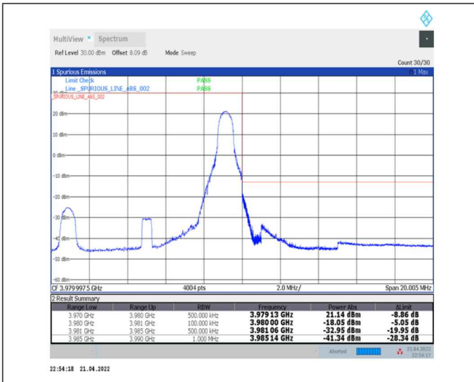
1-N77-3700-3980-30-10-H-2-DFT-PI2BPSK-Edge_1RB_Right-1@23-Ant0-PASS-see graph
