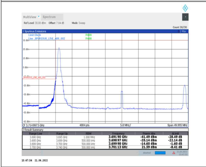
1-N77-3700-3980--30-40-L-4-CP-QPSK-Edge_1RB_Left-1@0-Ant0-PASS-see graph
