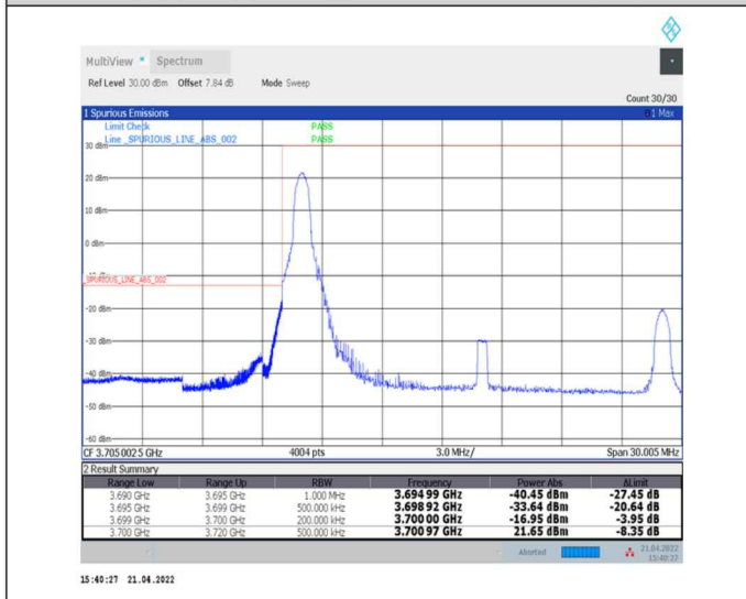
1-N77-3700-3980--30-20-L-4-CP-QPSK-Edge_1RB_Left-1@0-Ant0-PASS-see graph
