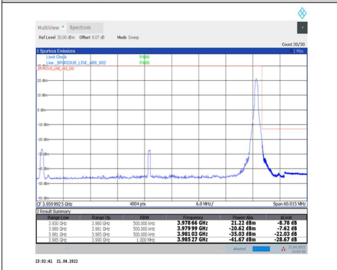
1-N77-3700-3980--30-50-H-5-CP-QPSK-Edge_1RB_Right-1@132-Ant0-PASS-see graph
