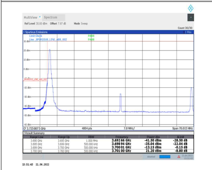
1-N77-3700-3980--30-60-L-4-CP-QPSK-Edge_1RB_Left-1@0-Ant0-PASS-see graph
