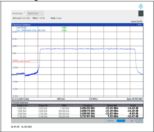
1-N77-3700-3980--30-40-L-3-DFT-PI2BPSK-Outer_Full-100@0-Ant0-PASS-see graph
