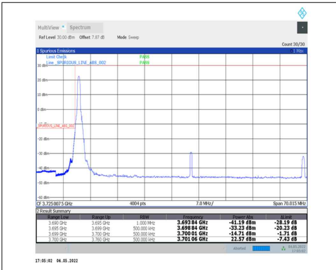
1-N77-3700-3980--30-60-L-1-DFT-PI2BPSK-Edge_1RB_Left-1@0-Ant0-PASS-see graph
