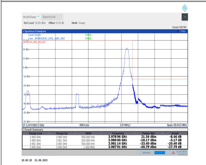
1-N77-3700-3980-30-20-H-5-CP-QPSK-Edge_1RB_Right-1@50-Ant0-PASS-see graph
