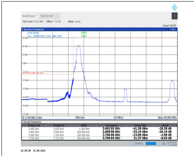
1-N77-3700-3980--30-20-L-1-DFT-PI2BPSK-Edge_1RB_Left-1@0-Ant0-PASS-see graph
