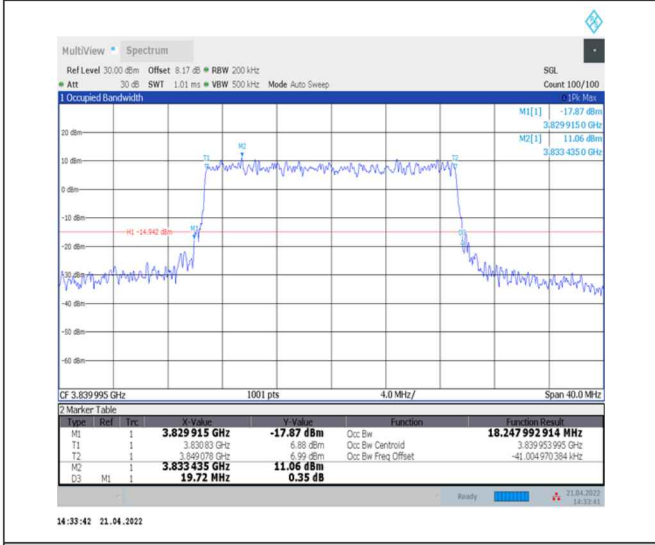
1-N77-3700-3980--30-20-M-8-CP-64QAM-Outer_Full-51@0-Ant0-18.248-19.720-≤20-PASS
