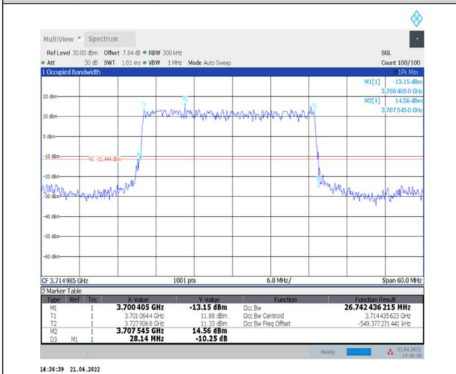
1-N77-3700-3980--30-30-L-2-DFT-PI2BPSK-Outer_Full-75@0-Ant0-26.744-28.140-<=30-PASS
