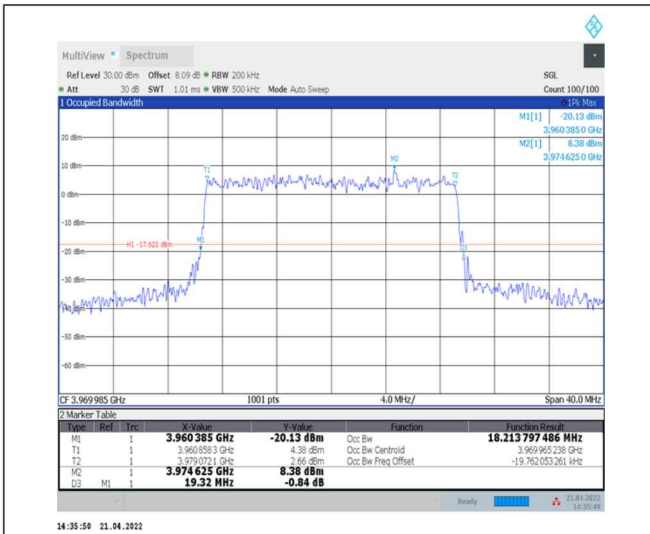
1-N77-3700-3980--30-20-H-9-CP-256QAM-Outer_Full-51@0-Ant0-18.214-19.320-<=30-PASS
