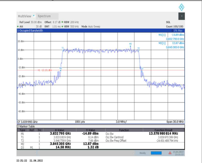
1-N77-3700-3980--30-15-M-6-CP-QPSK-Outer_Full-38@0-Ant0-13.579-14.580-≤15-PASS
