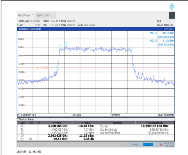
1-N77-3700-3980--30-20-H-7-CP-16QAM-Outer_Full-51@0-Ant0-18.19-19.520-≤20-PASS
