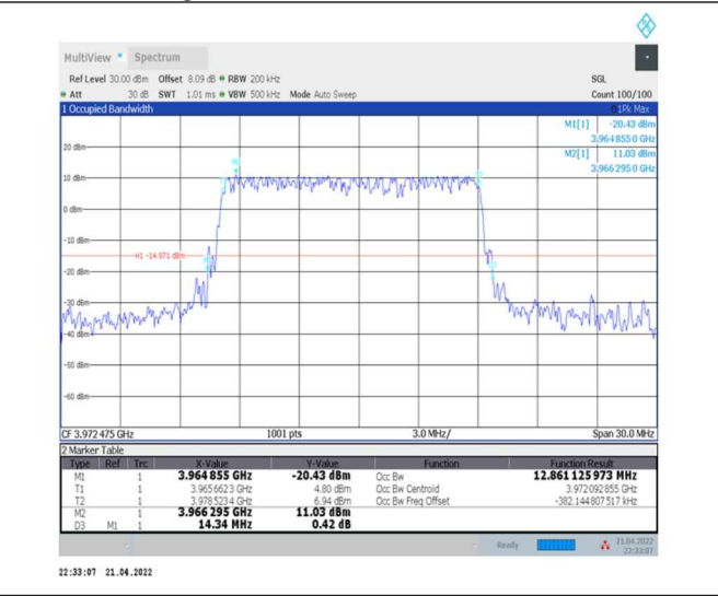
1-N77-3700-3980--30-15-H-5-DFT-256QAM-Outer_Full-36@0-Ant0-12.861-14.340-≤15-PASS
