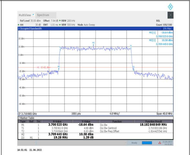
1-N77-3700-3980--30-20-L-6-CP-QPSK-Outer_Full-51@0-Ant0-18.183-19.280-<=20-PASS
