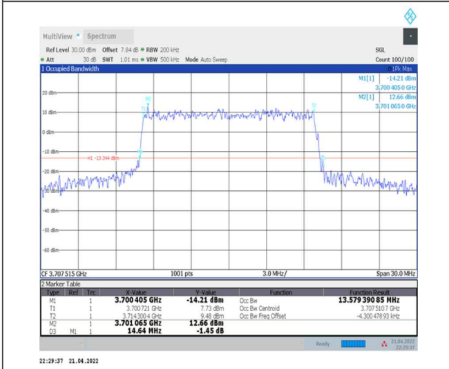
1-N77-3700-3980--30-15-L-8-CP-64QAM-Outer_Full-38@0-Ant0-13.579-14.640-≤15-PASS
