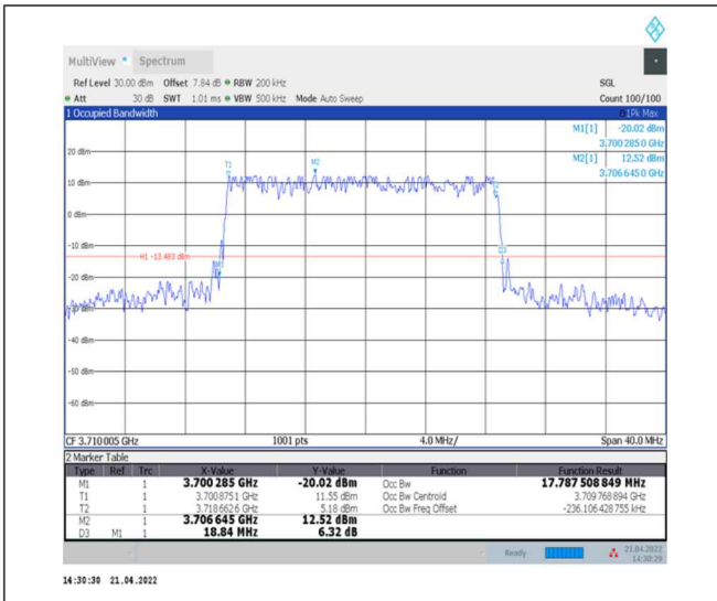
1-N77-3700-3980--30-20-L-3-DFT-16QAM-Outer_Full-50@0-Ant0-17.788-18.840-<=20-PASS
