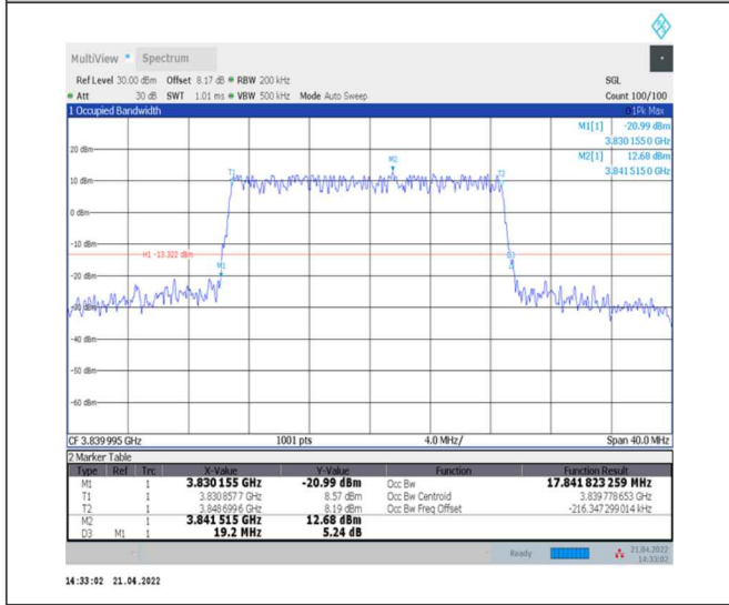
1-N77-3700-3980--30-20-M-4-DFT-64QAM-Outer_Full-50@0-Ant0-17.842-19.200-<=20-PASS
