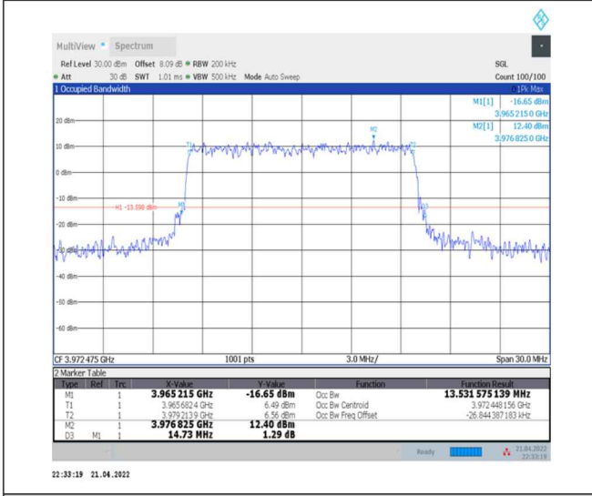
1-N77-3700-3980--30-15-H-6-CP-QPSK-Outer_Full-38@0-Ant0-13.532-14.730-≤15-PASS
