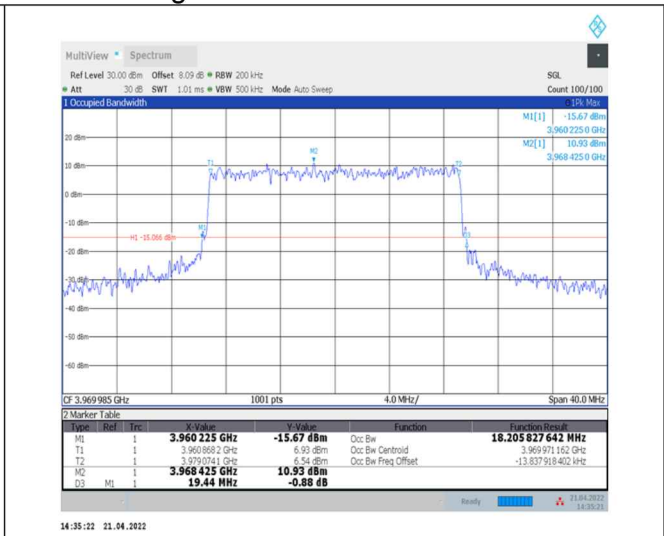
1-N77-3700-3980--30-20-H-6-CP-QPSK-Outer_Full-51@0-Ant0-18.206-19.440-≤20-PASS
