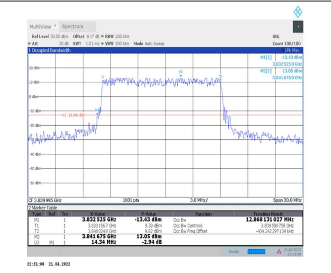
1-N77-3700-3980--30-15-M-4-DFT-64QAM-Outer_Full-36@0-Ant0-12.868-14.340-≤15-PASS
