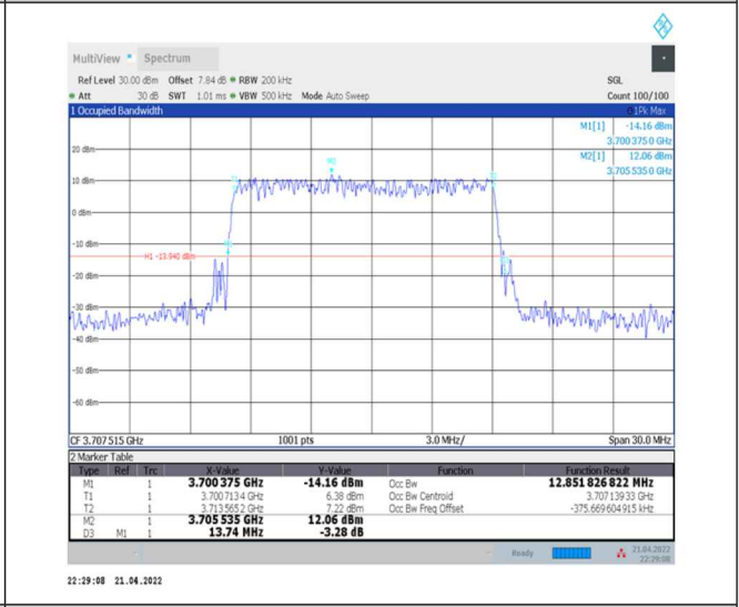
1-N77-3700-3980--30-15-L-5-DFT-256QAM-Outer_Full-36@0-Ant0-12.852-13.740-≤15-PASS
