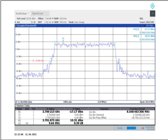
1-N77-3700-3980--30-10-L-5-DFT-256QAM-Outer_Full-24@0-Ant0-8.548-9.640-≤10-PASS
