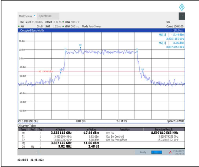
1-N77-3700-3980--30-10-M-6-CP-QPSK-Outer_Full-24@0-Ant0-8.598-9.820-≤10-PASS
