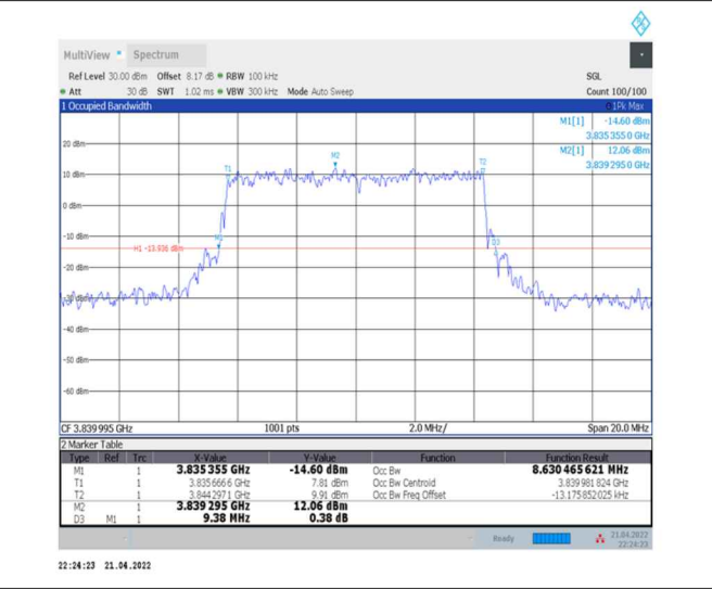
1-N77-3700-3980--30-10-M-3-DFT-16QAM-Outer_Full-24@0-Ant0-8.63-9.380-≤10-PASS
