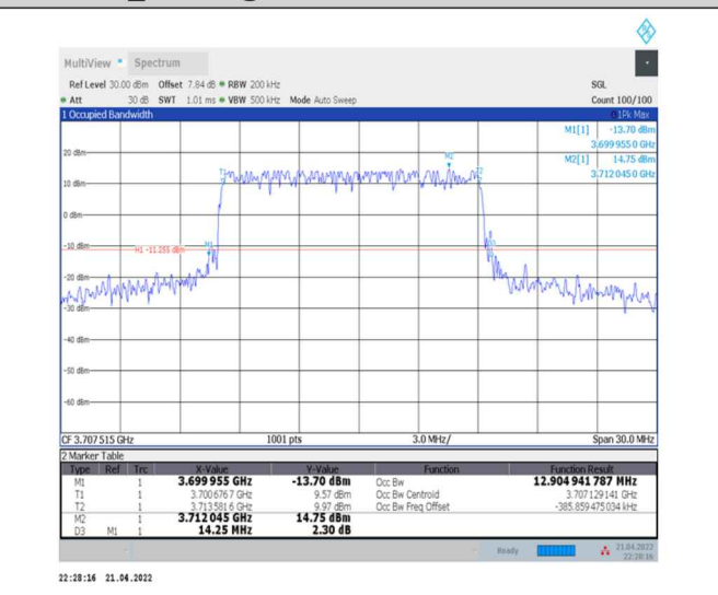
1-N77-3700-3980--30-15-L-1-DFT-QPSK-Outer_Full-36@0-Ant0-12.905-14.250-≤15-PASS
