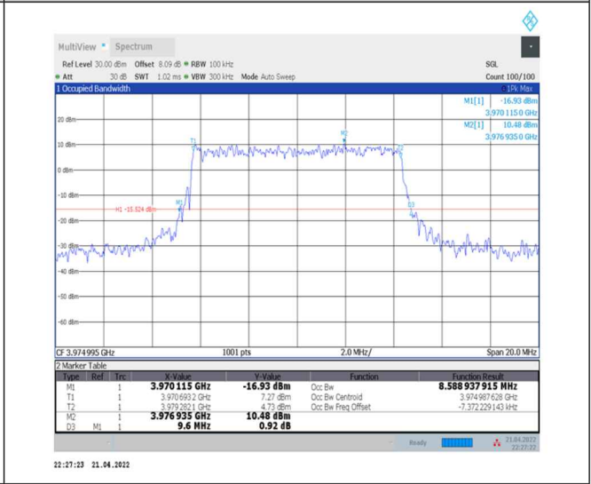
1-N77-3700-3980--30-10-H-6-CP-QPSK-Outer_Full-24@0-Ant0-8.589-9.600-≤10-PASS
