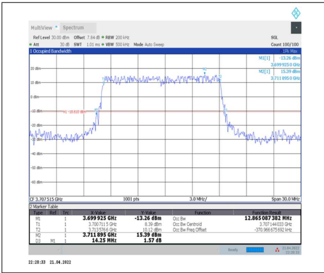
1-N77-3700-3980--30-15-L-2-DFT-PI2BPSK-Outer_Full-36@0-Ant0-12.865-14.250-≤15-PASS
