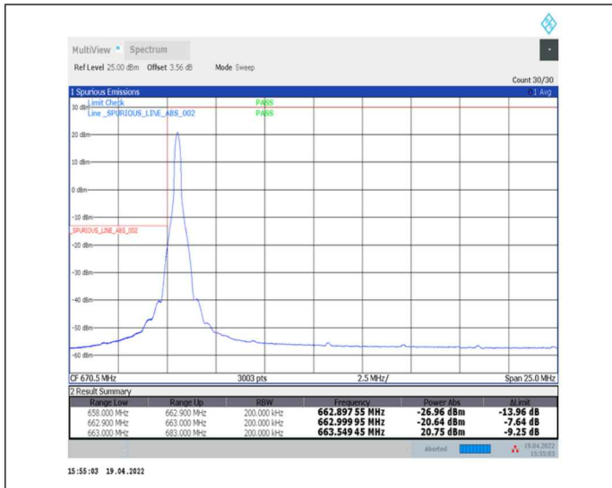
1-N71--15-20-L-1-DFT-PI2BPSK-Edge_1RB_Left-1@0-Ant0-PASS-see graph
