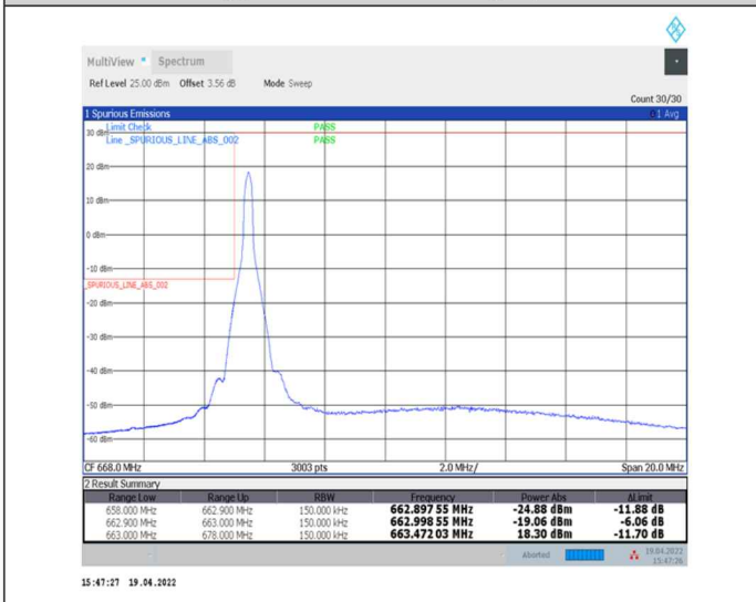
1-N71--15-15-L-4-CP-QPSK-Edge_1RB_Left-1@0-Ant0-PASS-see graph
