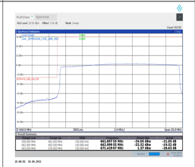
1-N71--15-15-L-6-CP-QPSK-Outer_Full-79@0-Ant0-PASS-see graph
