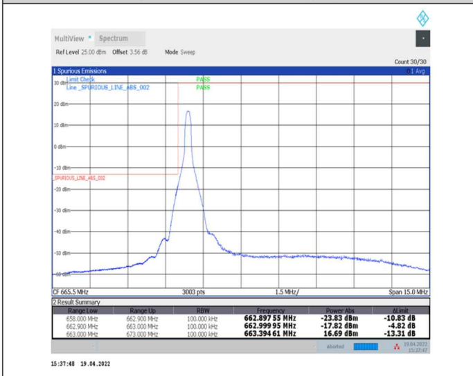
1-N71--15-10-L-4-CP-QPSK-Edge_1RB_Left-1@0-Ant0-PASS-see graph
