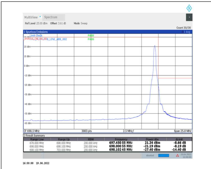
1-N71--15-20-H-2-DFT-PI2BPSK-Edge_1RB_Right-1@105-Ant0-PASS-see graph
