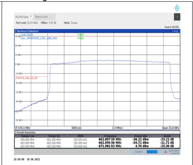
1-N71--15-20-L-3-DFT-PI2BPSK-Outer_Full-100@0-Ant0-PASS-see graph
