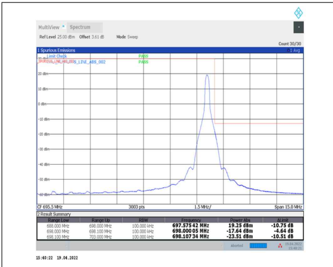
1-N71--15-10-H-2-DFT-PI2BPSK-Edge_1RB_Right-1@51-Ant0-PASS-see graph
