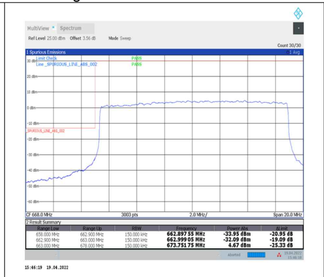
1-N71--15-15-L-3-DFT-PI2BPSK-Outer_Full-75@0-Ant0-PASS-see graph
