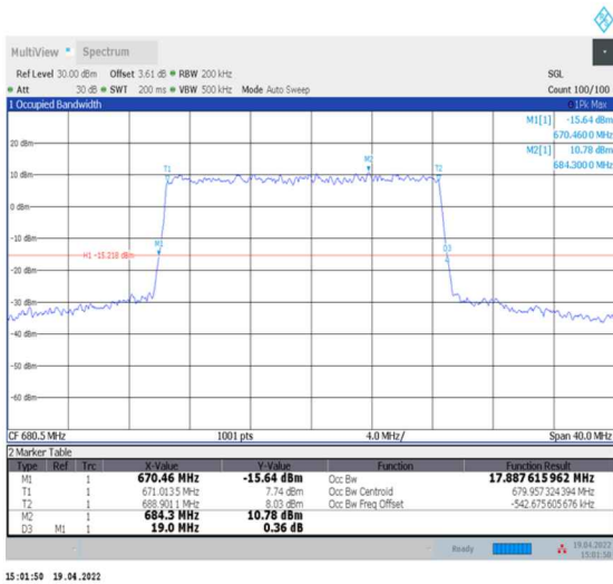
1-N71--15-20-M-5-DFT-256QAM-Outer_Full-100@0-Ant0-17.888-19.000-≤20-PASS
