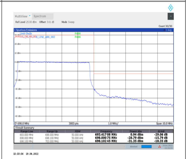
1-N71--15-5-H-6-CP-QPSK-Outer_Full-25@0-Ant0-PASS-see graph
