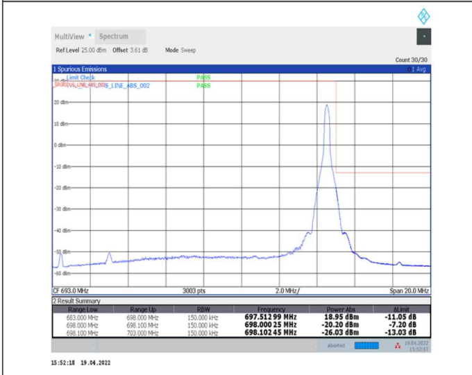
1-N71--15-15-H-5-CP-QPSK-Edge_1RB_Right-1@78-Ant0-PASS-see graph
