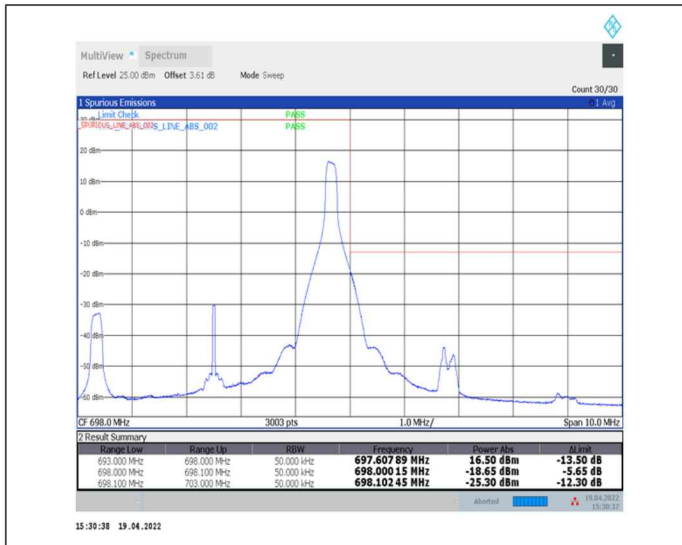
1-N71--15-5-H-2-DFT-PI2BPSK-Edge_1RB_Right-1@24-Ant0-PASS-see graph
