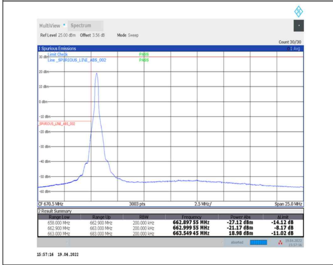
1-N71--15-20-L-4-CP-QPSK-Edge_1RB_Left-1@0-Ant0-PASS-see graph
