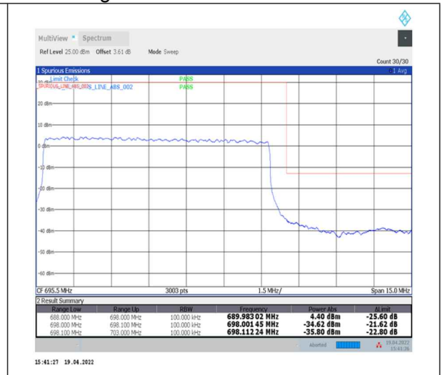
1-N71--15-10-H-3-DFT-PI2BPSK-Outer_Full-50@0-Ant0-PASS-see graph
