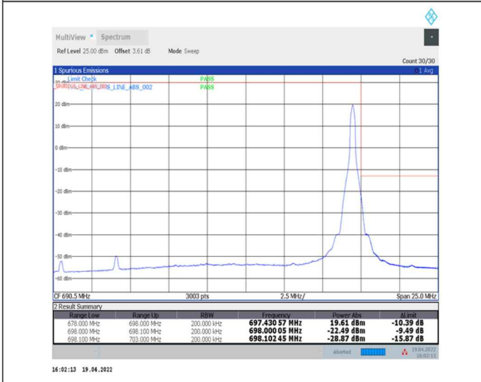
1-N71--15-20-H-5-CP-QPSK-Edge_1RB_Right-1@105-Ant0-PASS-see graph
