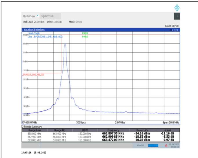
1-N71--15-15-L-1-DFT-PI2BPSK-Edge_1RB_Left-1@0-Ant0-PASS-see graph
