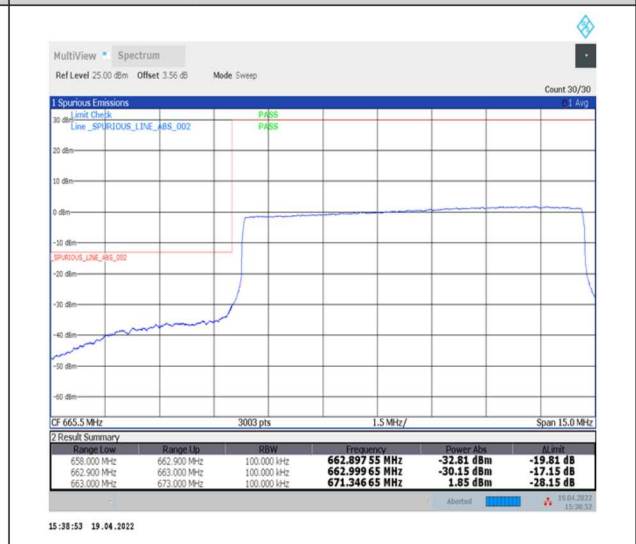
1-N71--15-10-L-6-CP-QPSK-Outer_Full-52@0-Ant0-PASS-see graph
