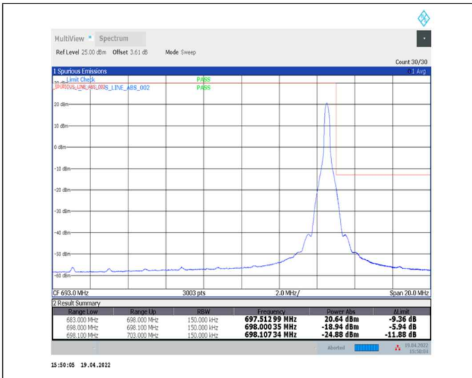
1-N71--15-15-H-2-DFT-PI2BPSK-Edge_1RB_Right-1@78-Ant0-PASS-see graph
