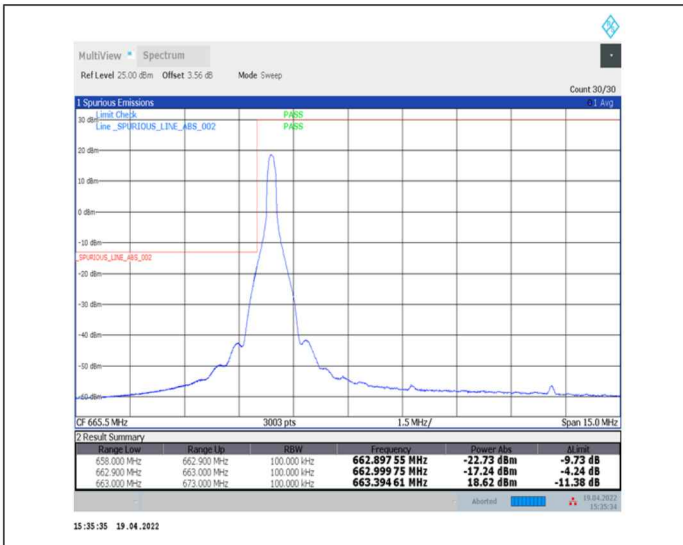
1-N71--15-10-L-1-DFT-PI2BPSK-Edge_1RB_Left-1@0-Ant0-PASS-see graph
