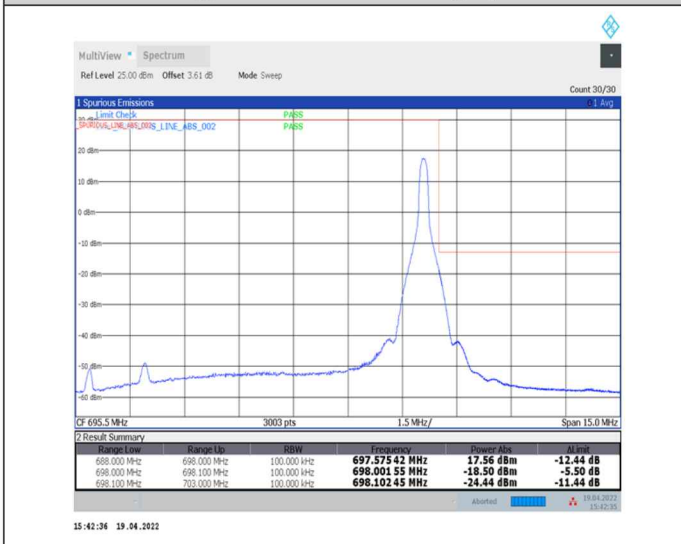
1-N71--15-10-H-5-CP-QPSK-Edge_1RB_Right-1@51-Ant0-PASS-see graph
