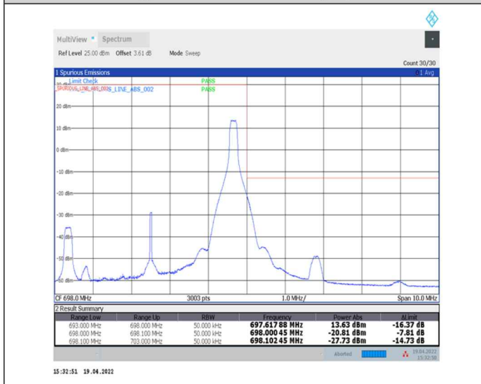
1-N71--15-5-H-5-CP-QPSK-Edge_1RB_Right-1@24-Ant0-PASS-see graph
