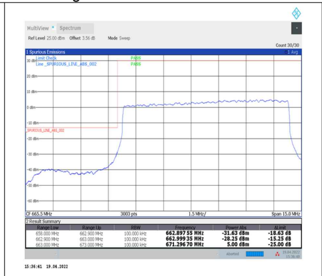
1-N71--15-10-L-3-DFT-PI2BPSK-Outer_Full-50@0-Ant0-PASS-see graph
