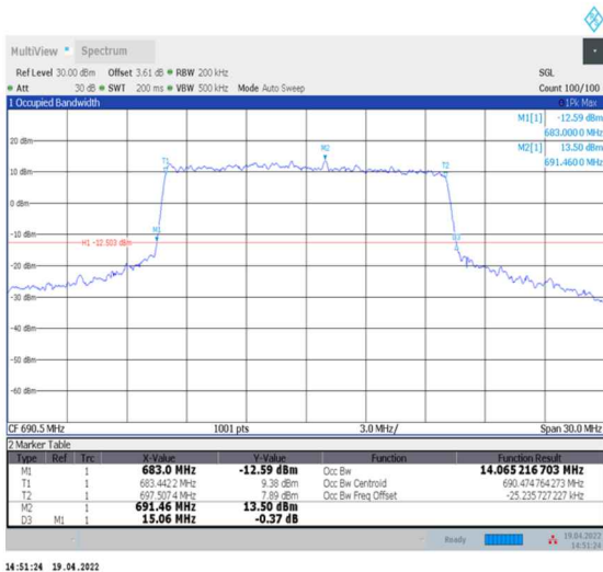
1-N71--15-15-H-7-CP-16QAM-Outer_Full-79@0-Ant0-14.065-15.060-≤15-PASS
