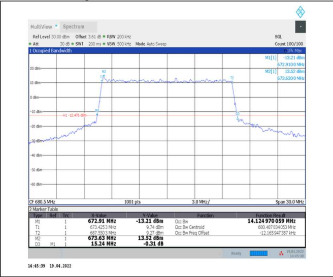
1-N71--15-15-M-7-CP-16QAM-Outer_Full-79@0-Ant0-14.125-15.240-≤15-PASS
