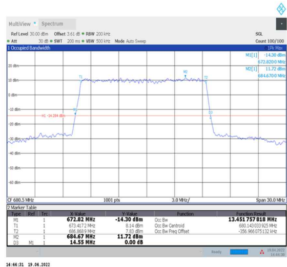
1-N71--15-15-M-5-DFT-256QAM-Outer_Full-75@0-Ant0-13.452-14.550-≤15-PASS
