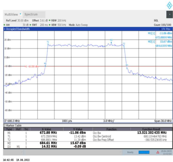
1-N71--15-15-M-1-DFT-QPSK-Outer_Full-75@0-Ant0-13.521-14.520-≤15-PASS
