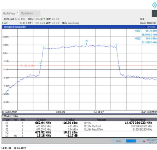
1-N71--15-15-L-9-CP-256QAM-Outer_Full-79@0-Ant0-14.079-15.180-≤15-PASS
