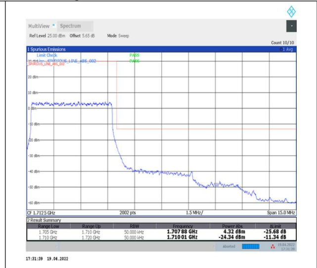
1-N70--15-5-H-3-DFT-PI2BPSK-Outer_Full-25@0-Ant2-seegraph-PASS-see graph
