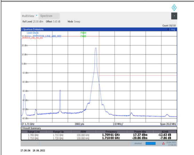
1-N70--15-10-H-5-CP-QPSK-Edge_1RB_Right-1@51-Ant2-seegraph-PASS-see graph
