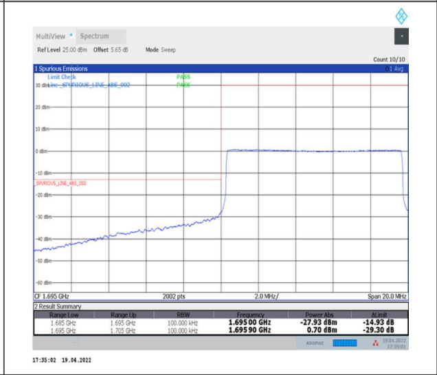
1-N70--15-10-L-6-CP-QPSK-Outer_Full-52@0-Ant2-seegraph-PASS-see graph
