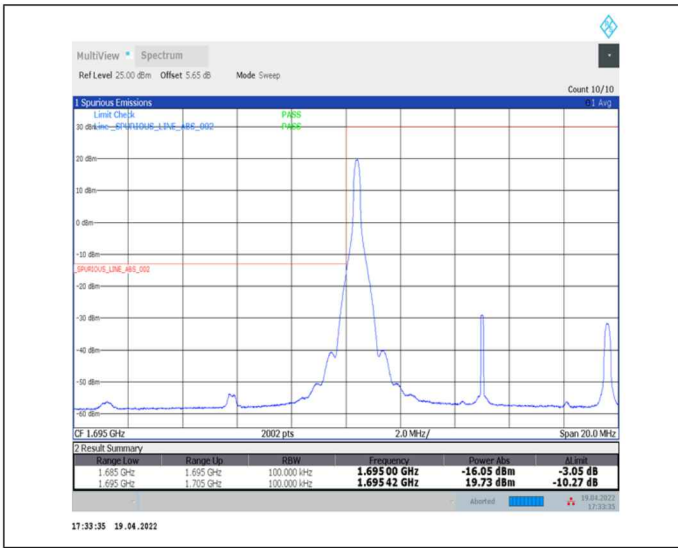
1-N70--15-10-L-1-DFT-PI2BPSK-Edge_1RB_Left-1@0-Ant2-seegraph-PASS-see graph
