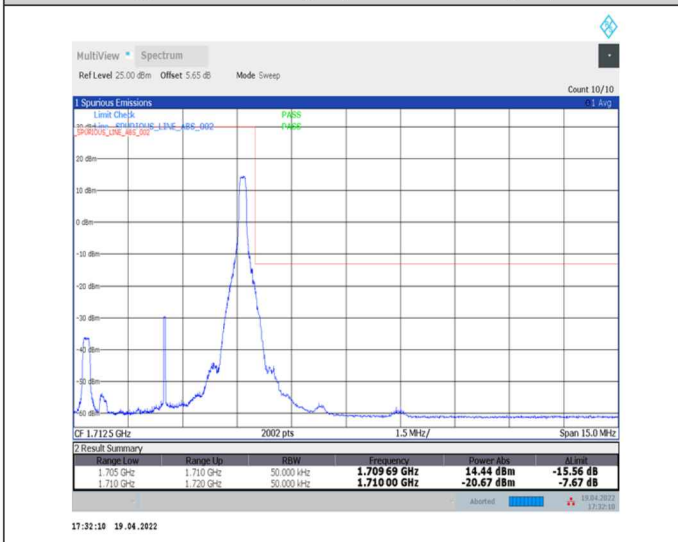
1-N70--15-5-H-5-CP-QPSK-Edge_1RB_Right-1@24-Ant2-seegraph-PASS-see graph
