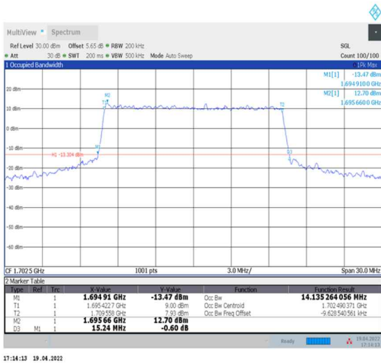
1-N70--15-15-H-7-CP-16QAM-Outer_Full-79@0-Ant2-14.135-15.240-≤15-PASS
