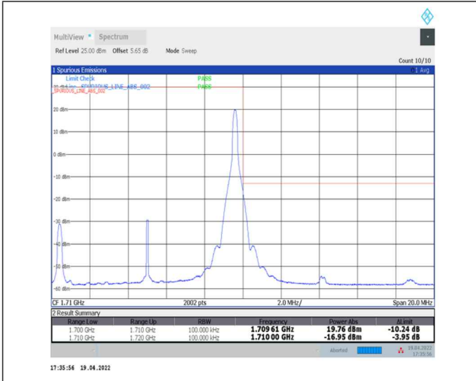
1-N70--15-10-H-2-DFT-PI2BPSK-Edge_1RB_Right-1@51-Ant2-seegraph-PASS-see graph
