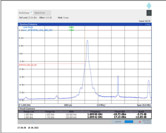
1-N70--15-10-L-4-CP-QPSK-Edge_1RB_Left-1@0-Ant2-seegraph-PASS-see graph
