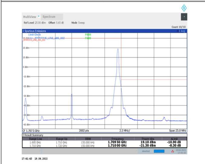
1-N70--15-15-H-5-CP-QPSK-Edge_1RB_Right-1@78-Ant2-seegraph-PASS-see graph
