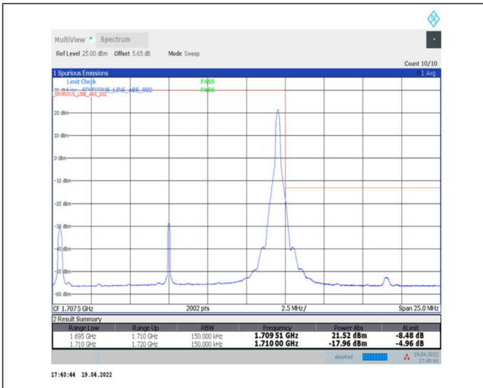
1-N70--15-15-H-2-DFT-PI2BPSK-Edge_1RB_Right-1@78-Ant2-seegraph-PASS-see graph
