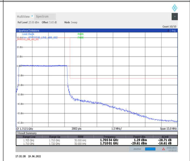
1-N70--15-5-H-6-CP-QPSK-Outer_Full-25@0-Ant2-seegraph-PASS-see graph
