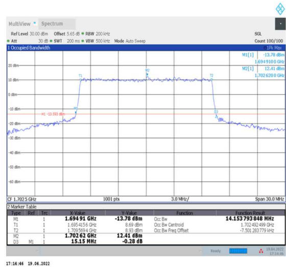
1-N70--15-15-H-8-CP-64QAM-Outer_Full-79@0-Ant2-14.154-15.150-≤15-PASS
