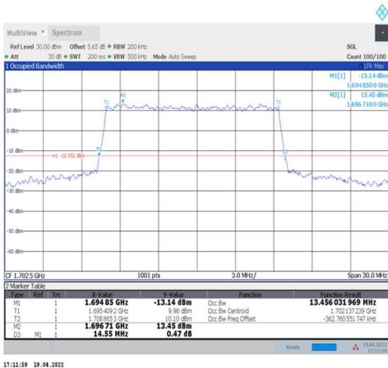
1-N70--15-15-H-3-DFT-16QAM-Outer_Full-75@0-Ant2-13.456-14.550-≤15-PASS
