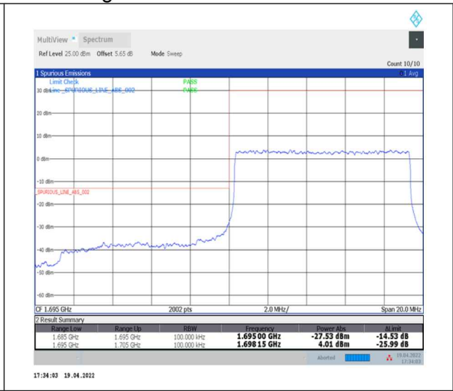
1-N70--15-10-L-3-DFT-PI2BPSK-Outer_Full-50@0-Ant2-seegraph-PASS-see graph
