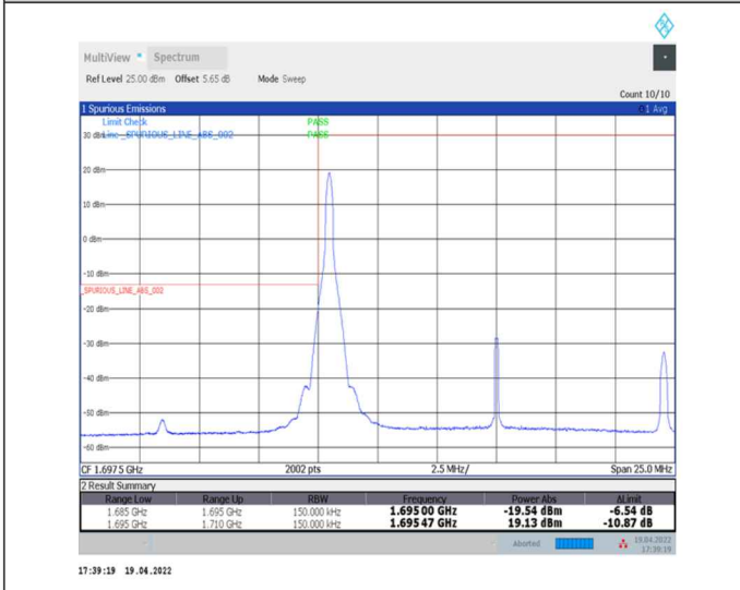
1-N70--15-15-L-4-CP-QPSK-Edge_1RB_Left-1@0-Ant2-seegraph-PASS-see graph
