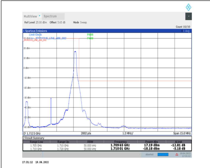
1-N70--15-5-H-2-DFT-PI2BPSK-Edge_1RB_Right-1@24-Ant2-seegraph-PASS-see graph
