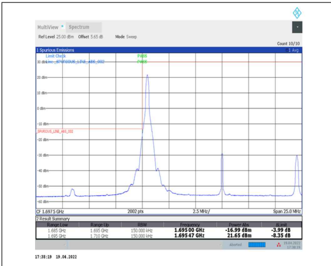
1-N70--15-15-L-1-DFT-PI2BPSK-Edge_1RB_Left-1@0-Ant2-seegraph-PASS-see graph
