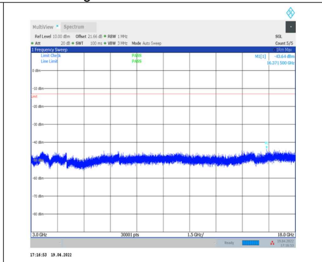
1-N70--15-15-M-1-DFT-PI2BPSK-Inner_1RB_Left-1@1-3000-18000-Ant2--43.64--13-PASS
