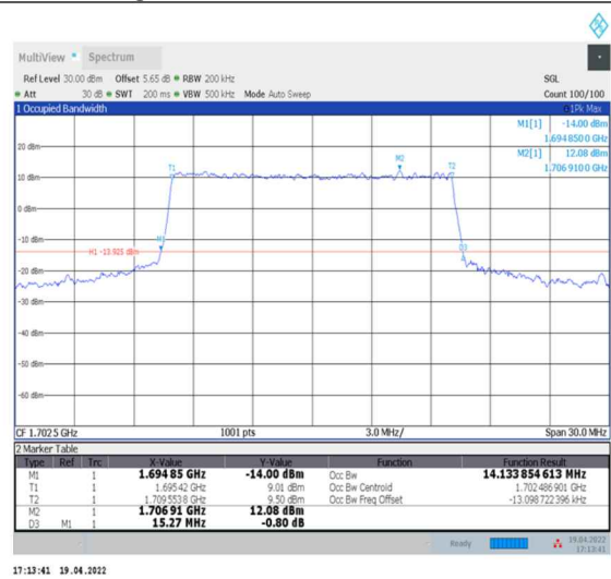
1-N70--15-15-H-6-CP-QPSK-Outer_Full-79@0-Ant2-14.134-15.270-≤15-PASS
