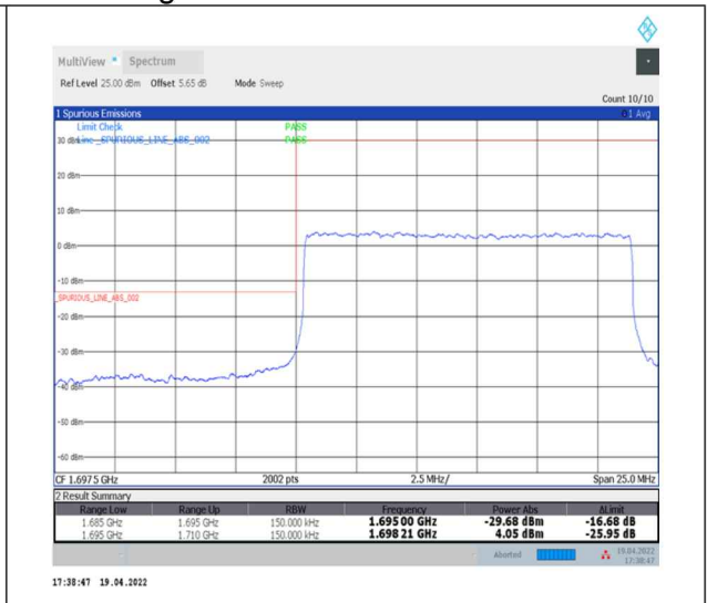
1-N70--15-15-L-3-DFT-PI2BPSK-Outer_Full-75@0-Ant2-seegraph-PASS-see graph
