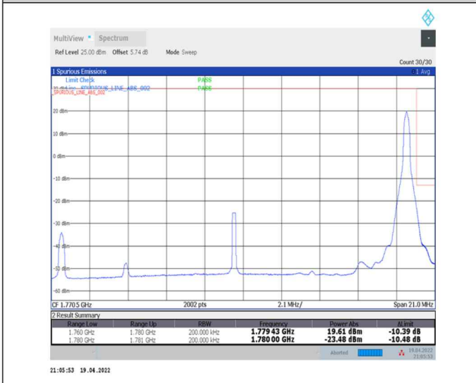
1-N66-PC3-15-20-H-5-CP-QPSK-Edge_1RB_Right-1@105-Ant0-seegraph-PASS-see graph
