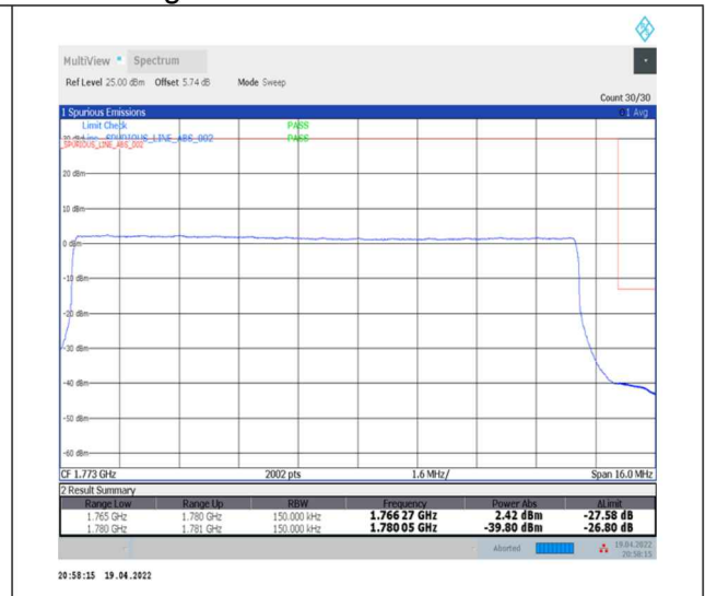
1-N66-PC3-15-15-H-3-DFT-PI2BPSK-Outer_Full-75@0-Ant0-seegraph-PASS-see graph
