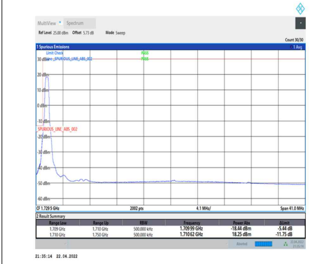
1-N66-PC3-15-40-L-4-CP-QPSK-Edge_1RB_Left-1@0-Ant0-seegraph-PASS-see graph
