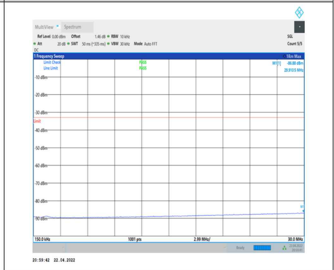
1-N66-PC3-15-40-M-1-DFT-PI2BPSK- Inner_1RB_Left-1@1-0.15-30-Ant0--86.88--33-PASS
