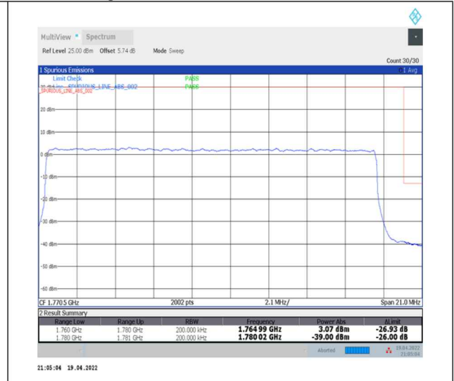
1-N66-PC3-15-20-H-3-DFT-PI2BPSK-Outer_Full-100@0-Ant0-seegraph-PASS-see graph
