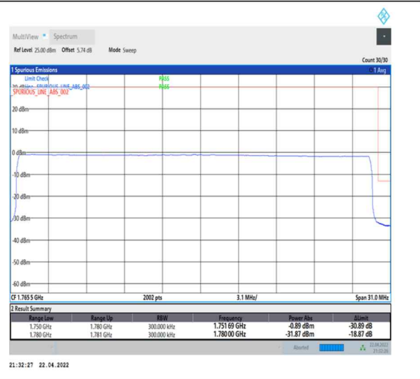
1-N66-PC3-15-30-H-6-CP-QPSK-Outer_Full-160@0-Ant0-seegraph-PASS-see graph
