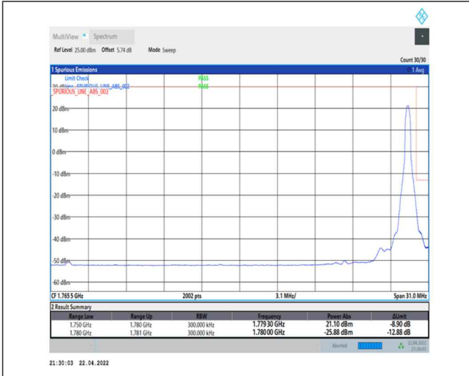
1-N66-PC3-15-30-H-2-DFT-PI2BPSK-Edge_1RB_Right-1@159-Ant0-seegraph-PASS-see graph
