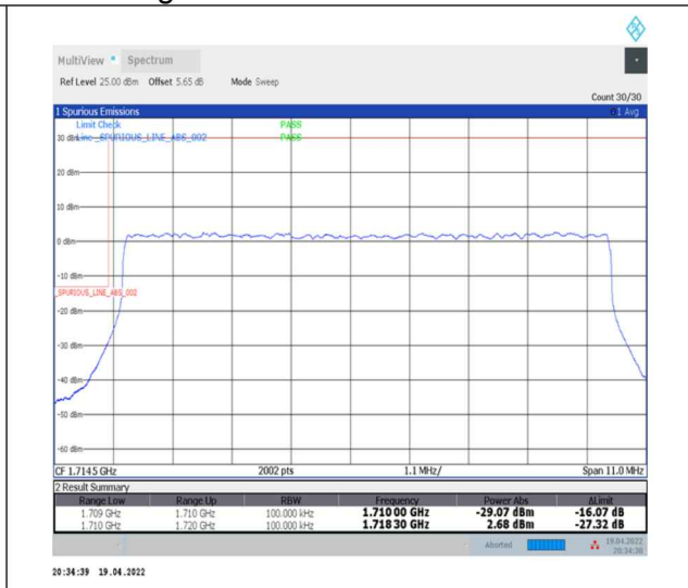
1-N66-PC3-15-10-L-3-DFT-PI2BPSK-Outer_Full-50@0-Ant0-seegraph-PASS-see graph
