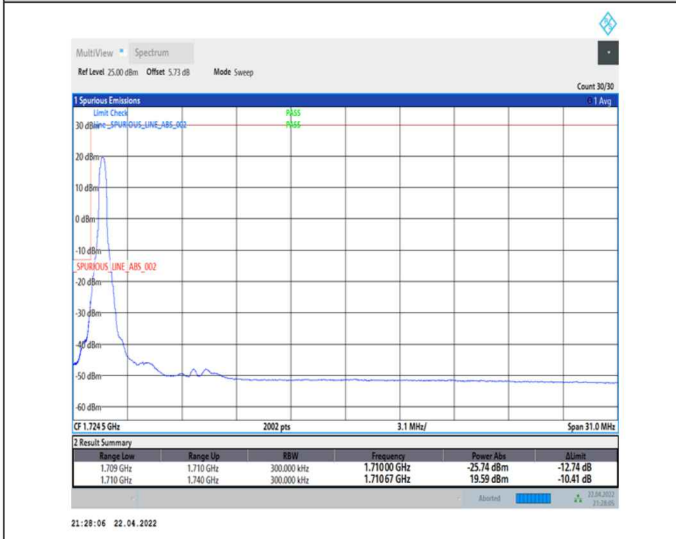
1-N66-PC3-15-30-L-4-CP-QPSK-Edge_1RB_Left-1@0-Ant0-seegraph-PASS-see graph
