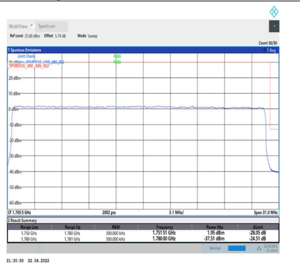
1-N66-PC3-15-30-H-3-DFT-PI2BPSK-Outer_Full-160@0-Ant0-seegraph-PASS-see graph
