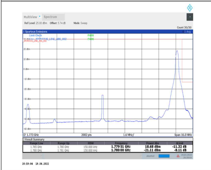
1-N66-PC3-15-15-H-5-CP-QPSK-Edge_1RB_Right-1@78-Ant0-seegraph-PASS-see graph
