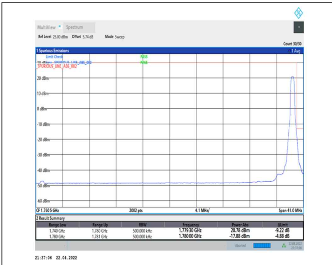
1-N66-PC3-15-40-H-2-DFT-PI2BPSK-Edge_1RB_Right-1@215-Ant0-seegraph-PASS-see graph
