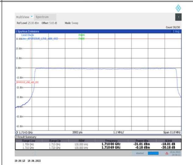
1-N66-PC3-15-10-L-6-CP-QPSK-Outer_Full-52@0-Ant0-seegraph-PASS-see graph
