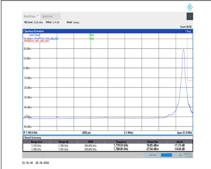
1-N66-PC3-15-30-H-5-CP-QPSK-Edge_1RB_Right-1@159-Ant0-seegraph-PASS-see graph
