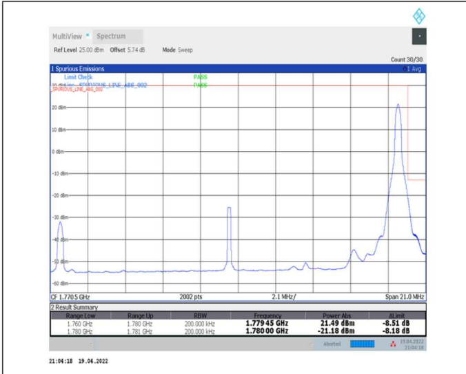
1-N66-PC3-15-20-H-2-DFT-PI2BPSK-Edge_1RB_Right-1@105-Ant0-seegraph-PASS-see graph
