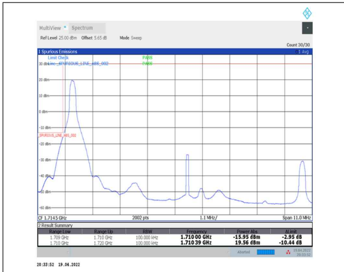
1-N66-PC3-15-10-L-1-DFT-PI2BPSK-Edge_1RB_Left-1@0-Ant0-seegraph-PASS-see graph
