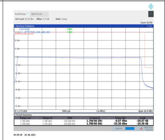
1-N66-PC3-15-15-H-6-CP-QPSK-Outer_Full-79@0-Ant0-seegraph-PASS-see graph
