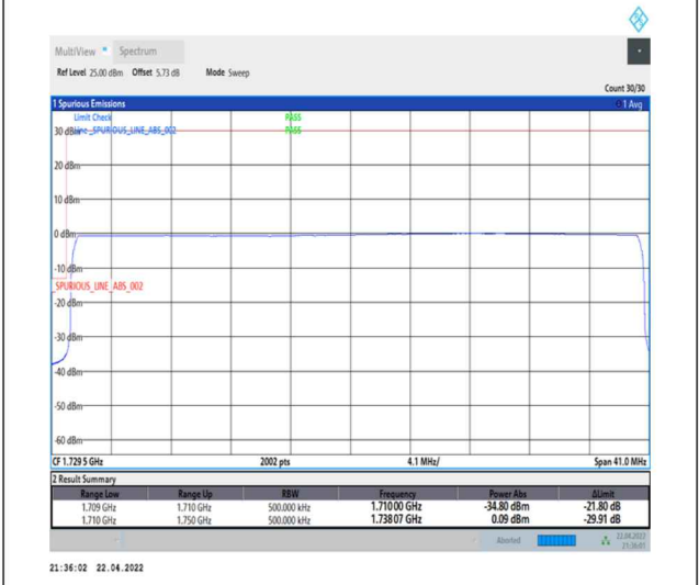
1-N66-PC3-15-40-L-6-CP-QPSK-Outer_Full-216@0-Ant0-seegraph-PASS-see graph
