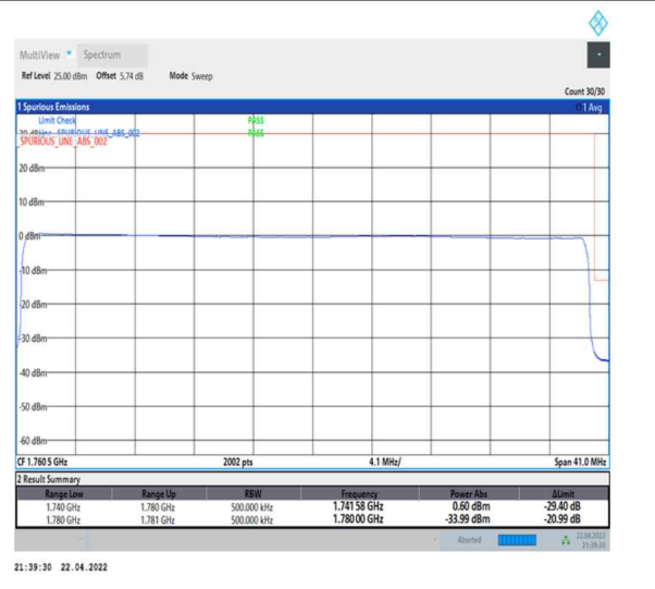
1-N66-PC3-15-40-H-6-CP-QPSK-Outer_Full-216@0-Ant0-seegraph-PASS-see graph
