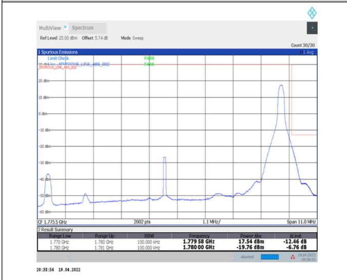
1-N66-PC3-15-10-H-5-CP-QPSK-Edge_1RB_Right-1@51-Ant0-seegraph-PASS-see graph
