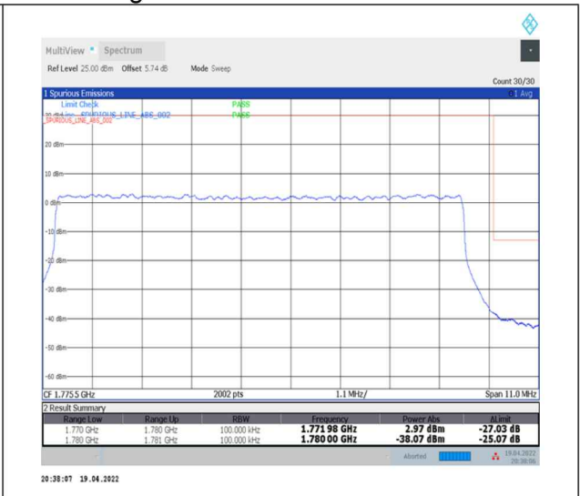
1-N66-PC3-15-10-H-3-DFT-PI2BPSK-Outer_Full-50@0-Ant0-seegraph-PASS-see graph
