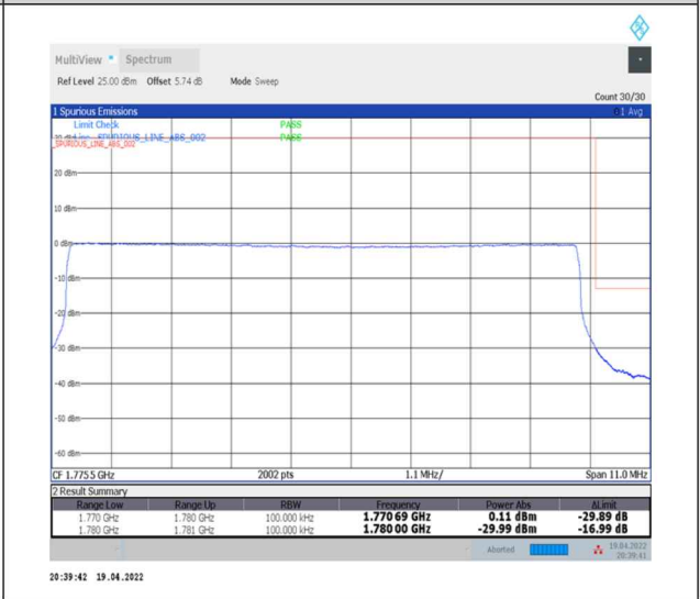
1-N66-PC3-15-10-H-6-CP-QPSK-Outer_Full-52@0-Ant0-seegraph-PASS-see graph
