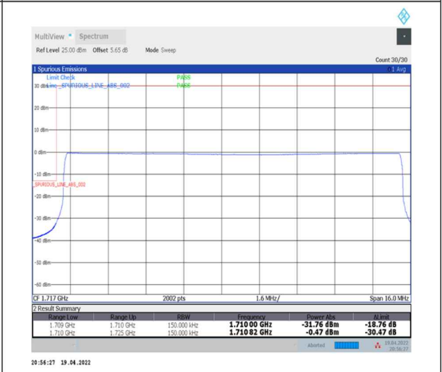
1-N66-PC3-15-15-L-6-CP-QPSK-Outer_Full-79@0-Ant0-seegraph-PASS-see graph
