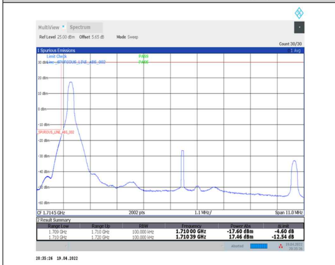
1-N66-PC3-15-10-L-4-CP-QPSK-Edge_1RB_Left-1@0-Ant0-seegraph-PASS-see graph
