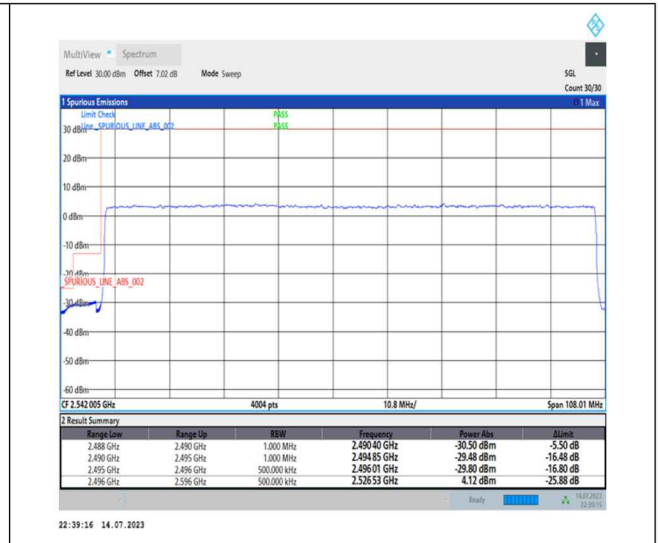
1-N41-PC1-30-100-L-3-DFT-PI2BPSK-Outer_Full-270@0-Ant0-1--PASS-see graph
