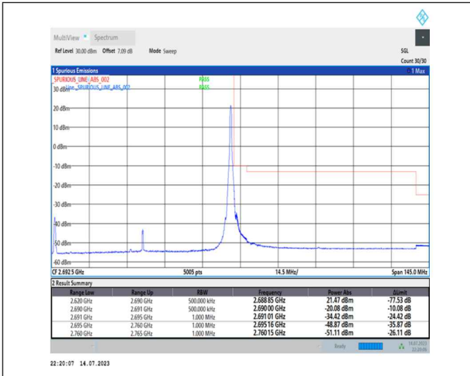
1-N41-PC1-30-70-H-2-DFT-PI2BPSK-Edge_1RB_Right-1@188-Ant0-1--PASS-see graph
