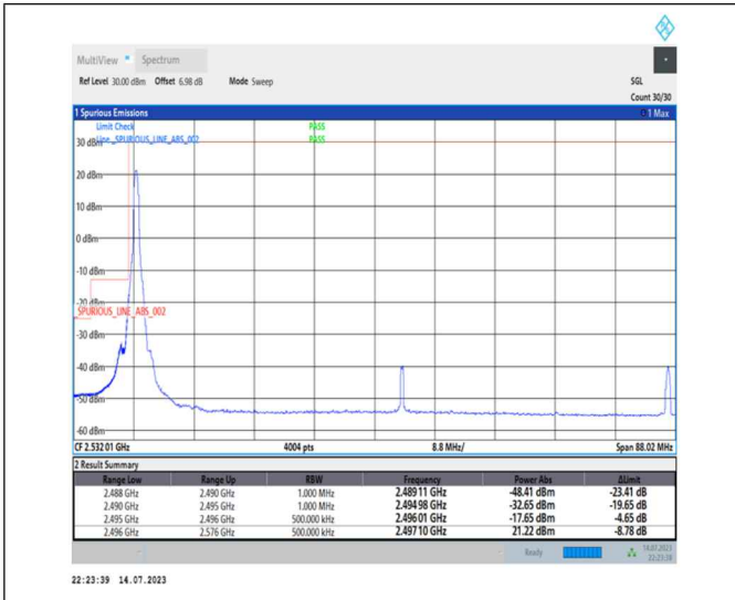
1-N41-PC1-30-80-L-1-DFT-PI2BPSK-Edge_1RB_Left-1@0-Ant0-1--PASS-see graph
