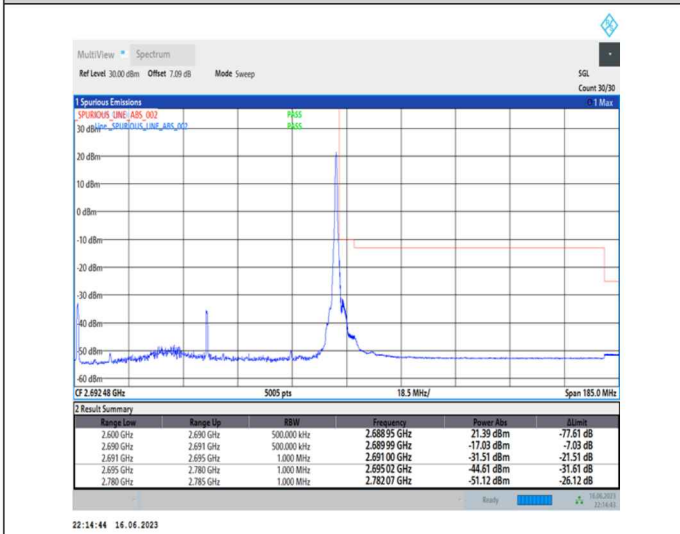
1-N41-PC1-30-90-H-5-CP-QPSK-Edge_1RB_Right-1@244-Ant0-1--PASS-see graph
