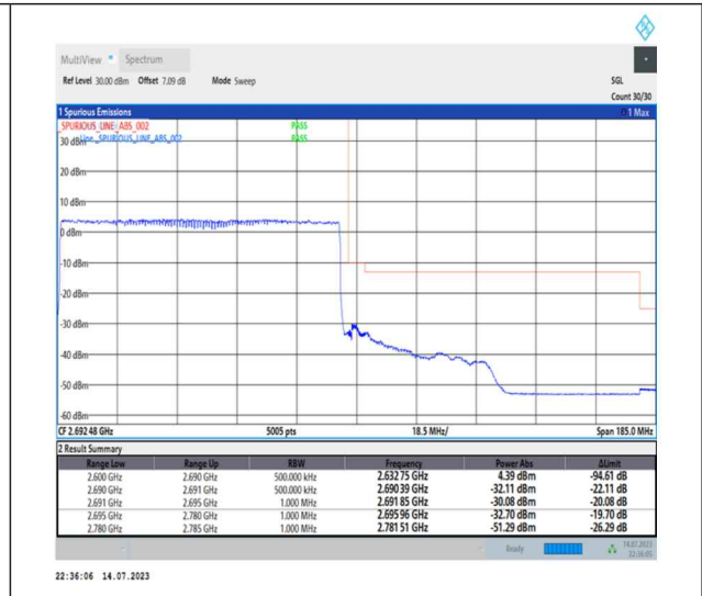
1-N41-PC1-30-90-H-3-DFT-PI2BPSK-Outer_Full-240@0-Ant0-1--PASS-see graph
