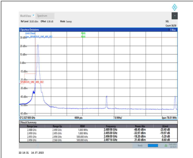
1-N41-PC1-30-70-L-1-DFT-PI2BPSK-Edge_1RB_Left-1@0-Ant0-1--PASS-see graph
