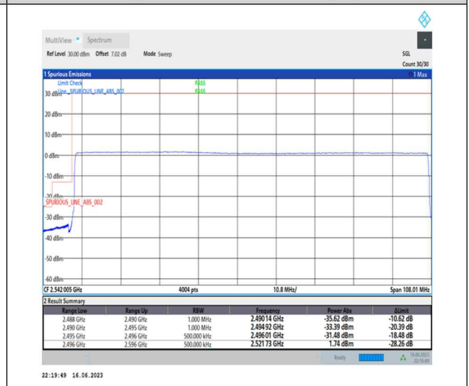
1-N41-PC1-30-100-L-6-CP-QPSK-Outer_Full-273@0-Ant0-1--PASS-see graph
