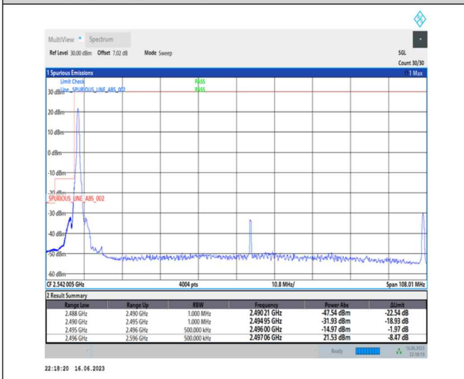
1-N41-PC1-30-100-L-4-CP-QPSK-Edge_1RB_Left-1@0-Ant0-1--PASS-see graph
