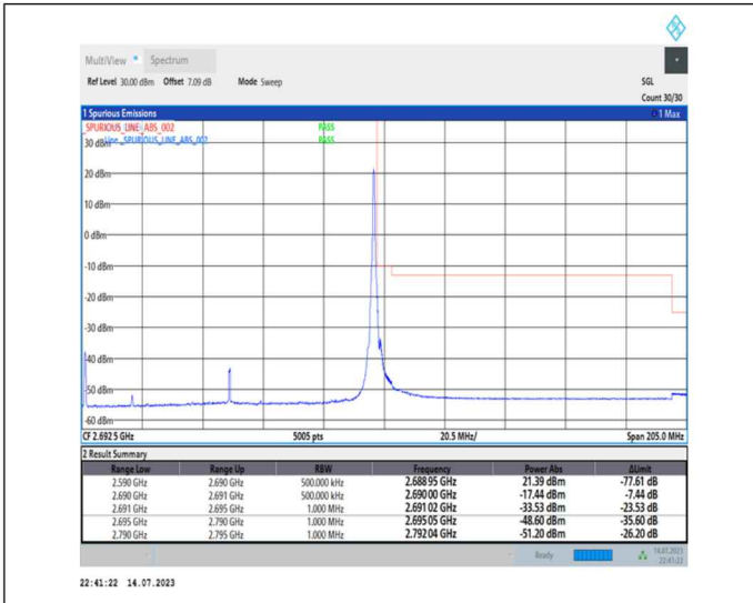
1-N41-PC1-30-100-H-2-DFT-PI2BPSK-Edge_1RB_Right-1@272-Ant0-1--PASS-see graph
