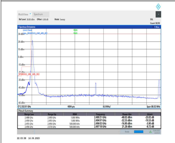
1-N41-PC1-30-80-L-4-CP-QPSK-Edge_1RB_Left-1@0-Ant0-1--PASS-see graph
