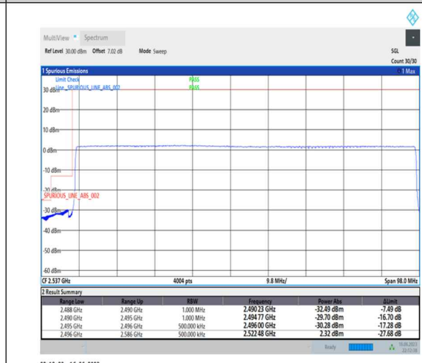
1-N41-PC1-30-90-L-6-CP-QPSK-Outer_Full-245@0-Ant0-1--PASS-see graph
