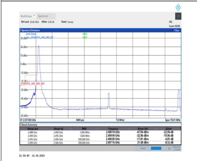
1-N41-PC1-30-70-L-4-CP-QPSK-Edge_1RB_Left-1@0-Ant0-1--PASS-see graph
