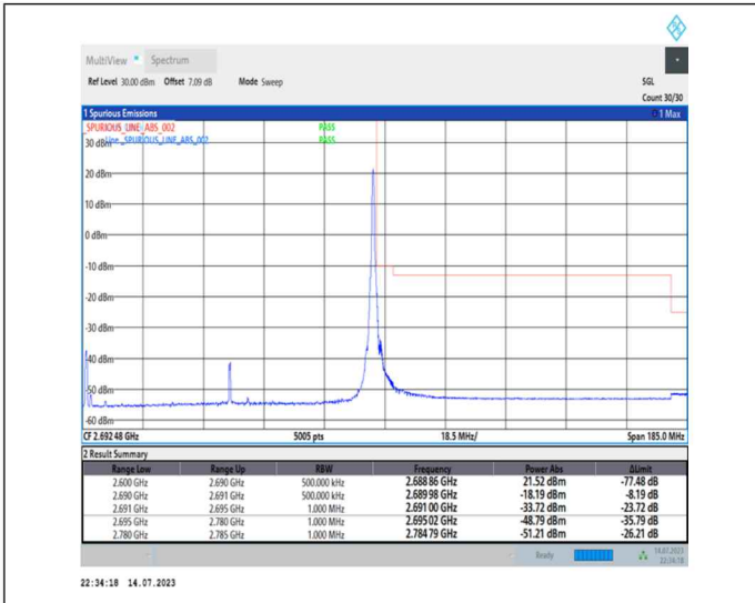
1-N41-PC1-30-90-H-2-DFT-PI2BPSK-Edge_1RB_Right-1@244-Ant0-1--PASS-see graph
