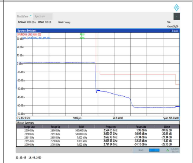
1-N41-PC1-30-100-H-6-CP-QPSK-Outer_Full-273@0-Ant0-1--PASS-see graph
