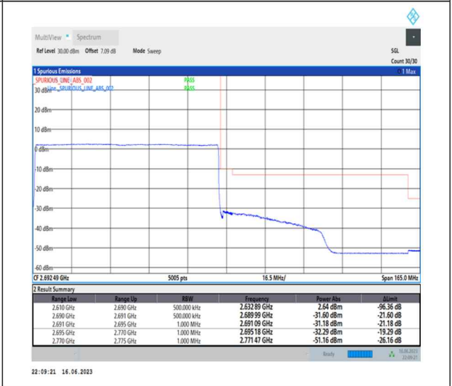
1-N41-PC1-30-80-H-6-CP-QPSK-Outer_Full-217@0-Ant0-1--PASS-see graph
