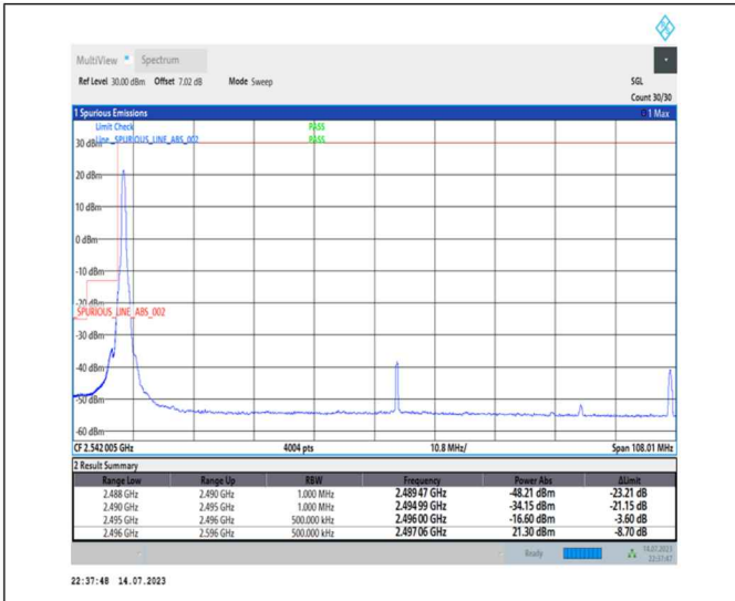
1-N41-PC1-30-100-L-1-DFT-PI2BPSK-Edge_1RB_Left-1@0-Ant0-1--PASS-see graph
