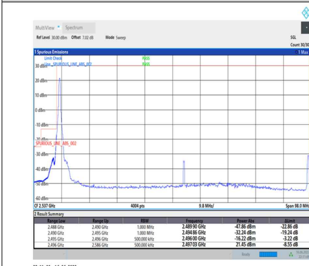
1-N41-PC1-30-90-L-4-CP-QPSK-Edge_1RB_Left-1@0-Ant0-1--PASS-see graph
