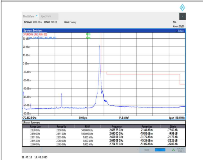
1-N41-PC1-30-70-H-5-CP-QPSK-Edge_1RB_Right-1@188-Ant0-1--PASS-see graph
