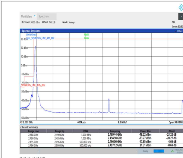
1-N41-PC1-30-90-L-1-DFT-PI2BPSK-Edge_1RB_Left-1@0-Ant0-1--PASS-see graph
