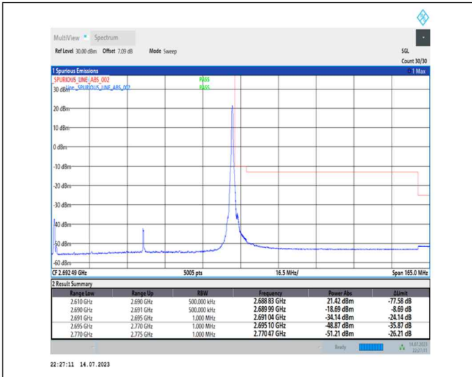
1-N41-PC1-30-80-H-2-DFT-PI2BPSK-Edge_1RB_Right-1@216-Ant0-1--PASS-see graph
