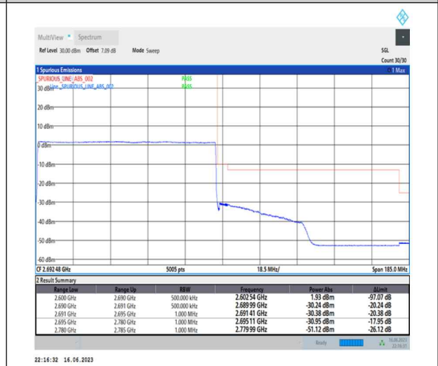
1-N41-PC1-30-90-H-6-CP-QPSK-Outer_Full-245@0-Ant0-1--PASS-see graph
