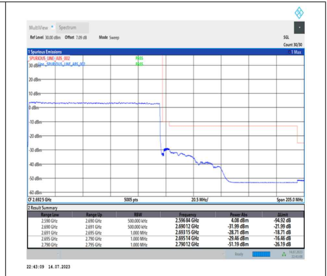
1-N41-PC1-30-100-H-3-DFT-PI2BPSK-Outer_Full-270@0-Ant0-1--PASS-see graph
