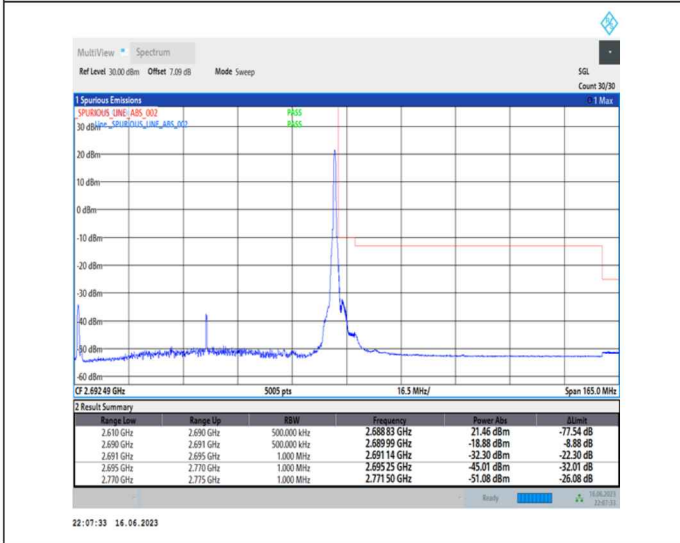
1-N41-PC1-30-80-H-5-CP-QPSK-Edge_1RB_Right-1@216-Ant0-1--PASS-see graph
