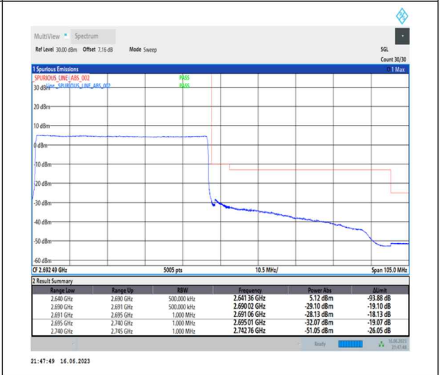
1-N41-PC1-30-50-H-6-CP-QPSK-Outer_Full-133@0-Ant0-1--PASS-see graph
