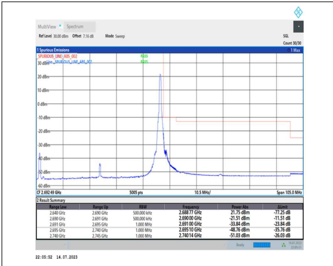
1-N41-PC1-30-50-H-2-DFT-PI2BPSK-Edge_1RB_Right-1@132-Ant0-1--PASS-see graph
