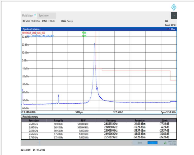
1-N41-PC1-30-60-H-2-DFT-PI2BPSK-Edge_1RB_Right-1@161-Ant0-1--PASS-see graph
