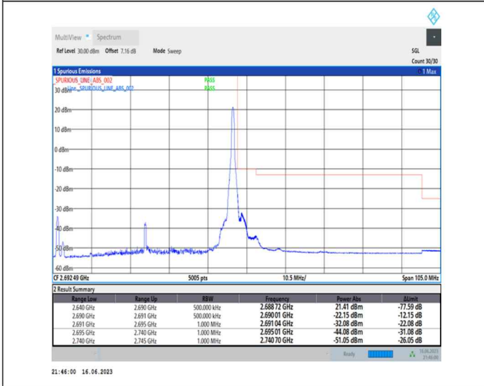
1-N41-PC1-30-50-H-5-CP-QPSK-Edge_1RB_Right-1@132-Ant0-1--PASS-see graph
