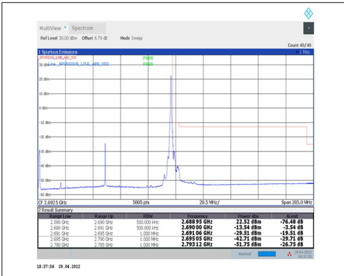
1-N41--30-100-H-2-DFT-PI2BPSK-Edge_1RB_Right-1@272-Ant0-PASS-see graph
