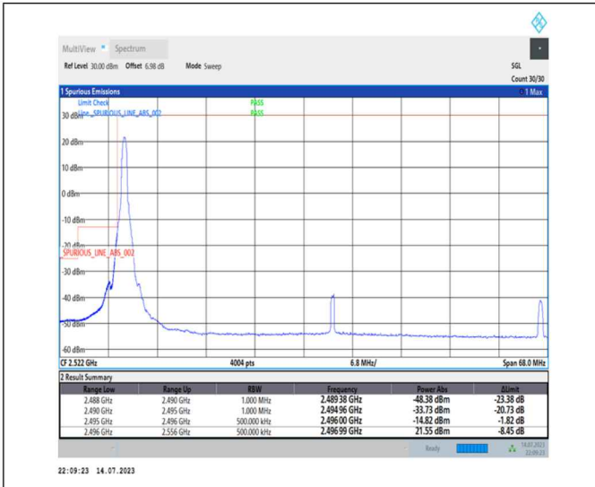
1-N41-PC1-30-60-L-1-DFT-PI2BPSK-Edge_1RB_Left-1@0-Ant0-1--PASS-see graph
