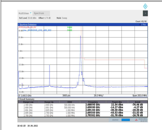
1-N41--30-100-H-5-CP-QPSK-Edge_1RB_Right-1@272-Ant0-PASS-see graph
