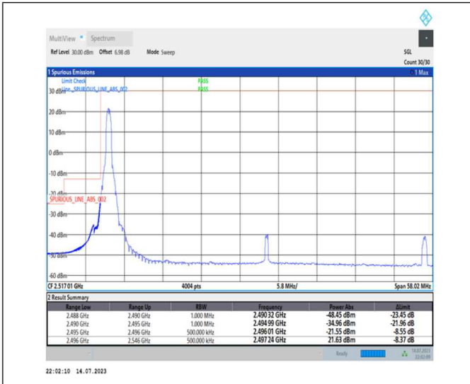
1-N41-PC1-30-50-L-1-DFT-PI2BPSK-Edge_1RB_Left-1@0-Ant0-1--PASS-see graph
