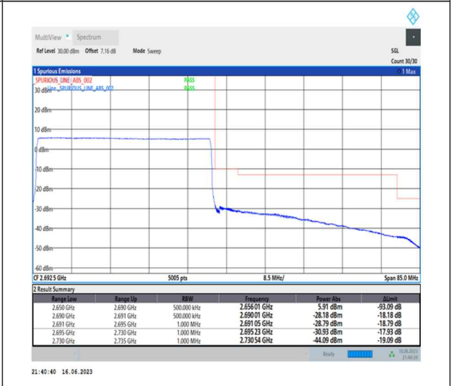
1-N41-PC1-30-40-H-6-CP-QPSK-Outer_Full-106@0-Ant0-1--PASS-see graph
