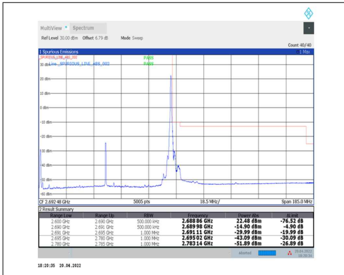
1-N41--30-90-H-2-DFT-PI2BPSK-Edge_1RB_Right-1@244-Ant0-PASS-see graph
