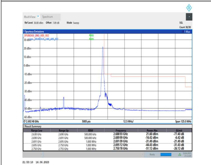
1-N41-PC1-30-60-H-5-CP-QPSK-Edge_1RB_Right-1@161-Ant0-1--PASS-see graph
