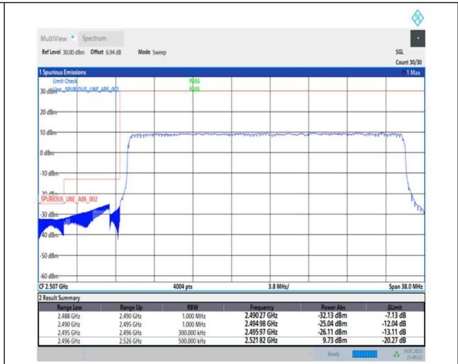
1-N41-PC1-30-30-L-3-DFT-PI2BPSK-Outer_Full-75@0-Ant0-1--PASS-see graph
