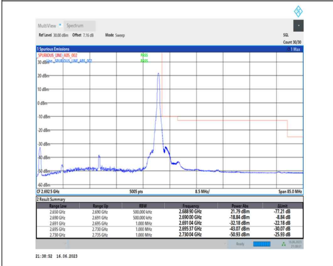
1-N41-PC1-30-40-H-5-CP-QPSK-Edge_1RB_Right-1@105-Ant0-1--PASS-see graph
