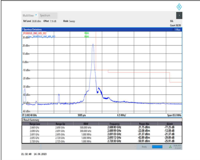
1-N41-PC1-30-30-H-5-CP-QPSK-Edge_1RB_Right-1@77-Ant0-1--PASS-see graph
