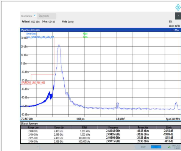
1-N41-PC1-30-30-L-1-DFT-PI2BPSK-Edge_1RB_Left-1@0-Ant0-1--PASS-see graph
