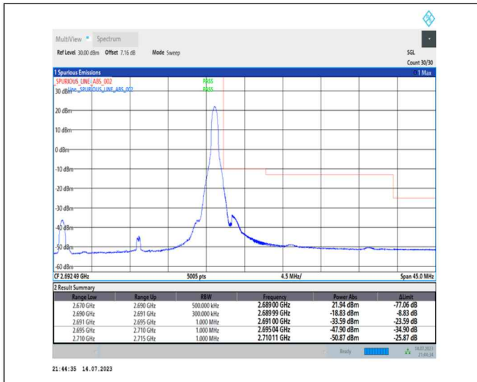
1-N41-PC1-30-20-H-2-DFT-PI2BPSK-Edge_1RB_Right-1@50-Ant0-1--PASS-see graph
