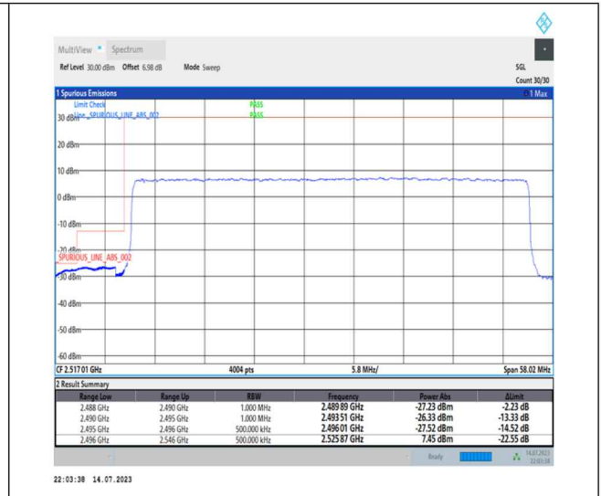
1-N41-PC1-30-50-L-3-DFT-PI2BPSK-Outer_Full-128@0-Ant0-1--PASS-see graph
