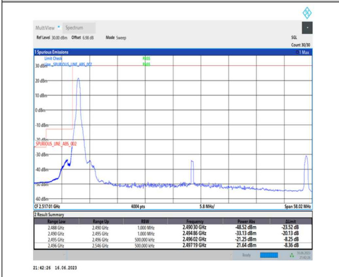
1-N41-PC1-30-50-L-4-CP-QPSK-Edge_1RB_Left-1@0-Ant0-1--PASS-see graph
