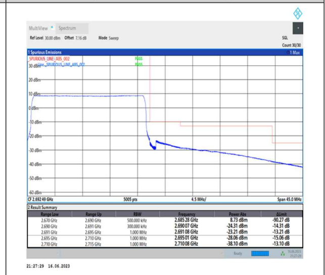
1-N41-PC1-30-20-H-6-CP-QPSK-Outer_Full-51@0-Ant0-1--PASS-see graph
