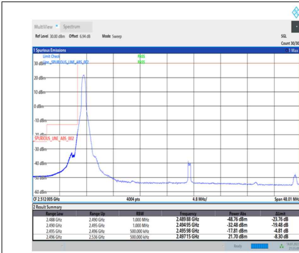
1-N41-PC1-30-40-L-1-DFT-PI2BPSK-Edge_1RB_Left-1@0-Ant0-1--PASS-see graph
