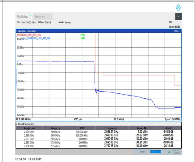
1-N41-PC1-30-60-H-6-CP-QPSK-Outer_Full-162@0-Ant0-1--PASS-see graph
