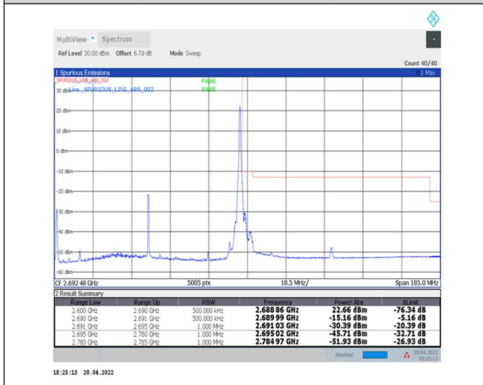
1-N41--30-90-H-5-CP-QPSK-Edge_1RB_Right-1@244-Ant0-PASS-see graph
