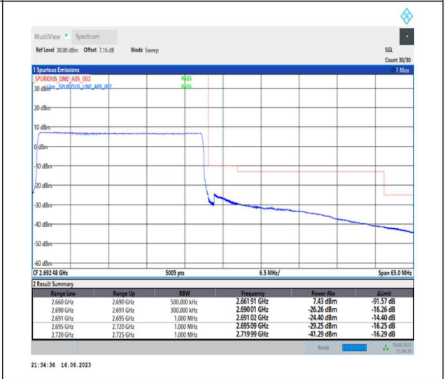
1-N41-PC1-30-30-H-6-CP-QPSK-Outer_Full-78@0-Ant0-1--PASS-see graph
