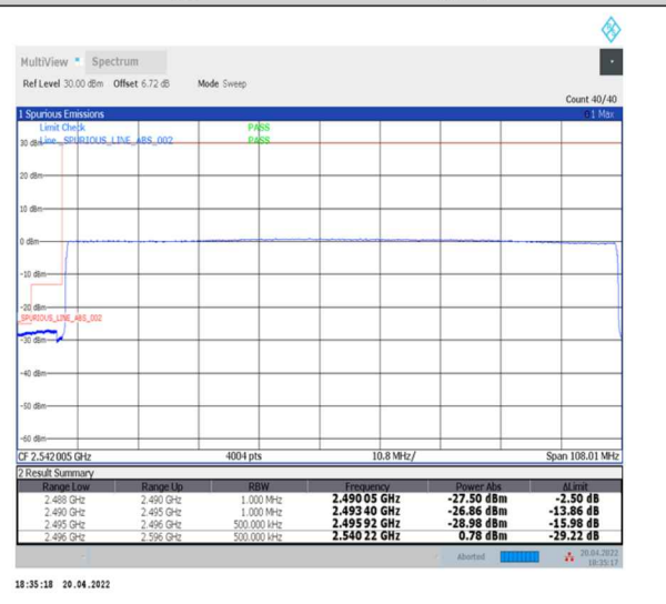
1-N41--30-100-L-6-CP-QPSK-Outer_Full-273@0-Ant0-PASS-see graph
