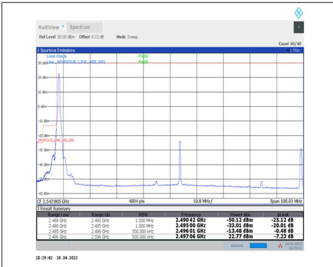
1-N41--30-100-L-1-DFT-PI2BPSK-Edge_1RB_Left-1@0-Ant0-PASS-see graph
