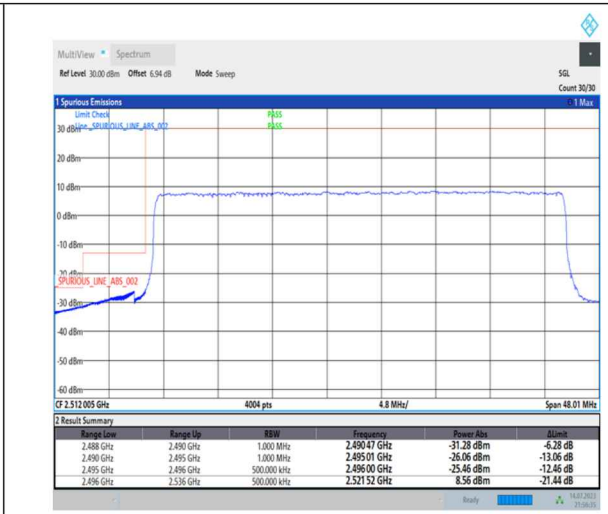
1-N41-PC1-30-40-L-3-DFT-PI2BPSK-Outer_Full-100@0-Ant0-1--PASS-see graph
