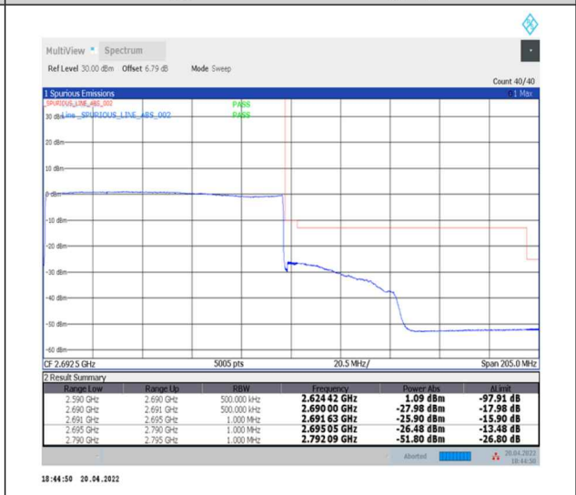
1-N41--30-100-H-6-CP-QPSK-Outer_Full-273@0-Ant0-PASS-see graph
