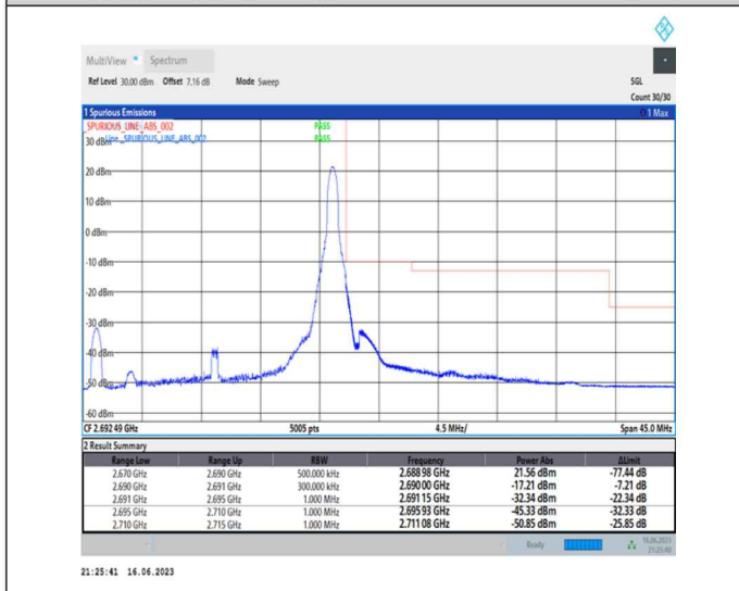
1-N41-PC1-30-20-H-5-CP-QPSK-Edge_1RB_Right-1@50-Ant0-1--PASS-see graph
