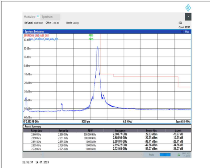
1-N41-PC1-30-30-H-2-DFT-PI2BPSK-Edge_1RB_Right-1@77-Ant0-1--PASS-see graph
