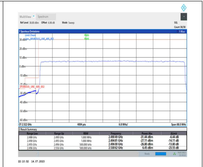
1-N41-PC1-30-60-L-3-DFT-PI2BPSK-Outer_Full-162@0-Ant0-1--PASS-see graph
