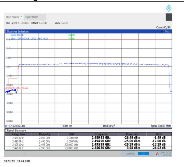
1-N41--30-100-L-3-DFT-PI2BPSK-Outer_Full-270@0-Ant0-PASS-see graph
