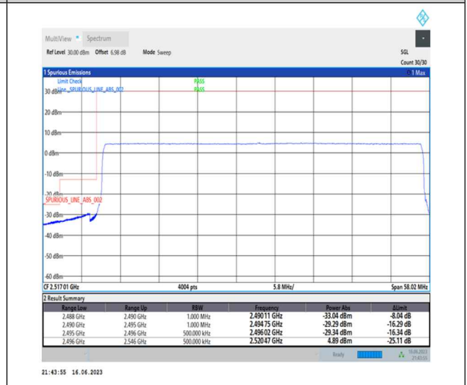
1-N41-PC1-30-50-L-6-CP-QPSK-Outer_Full-133@0-Ant0-1--PASS-see graph
