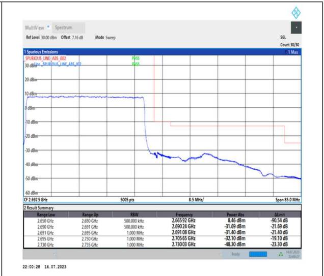
1-N41-PC1-30-40-H-3-DFT-PI2BPSK-Outer_Full-100@0-Ant0-1--PASS-see graph
