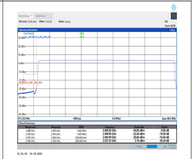
1-N41-PC1-30-60-L-6-CP-QPSK-Outer_Full-162@0-Ant0-1--PASS-see graph
