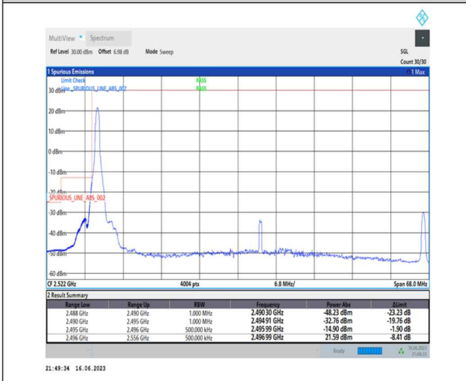
1-N41-PC1-30-60-L-4-CP-QPSK-Edge_1RB_Left-1@0-Ant0-1--PASS-see graph
