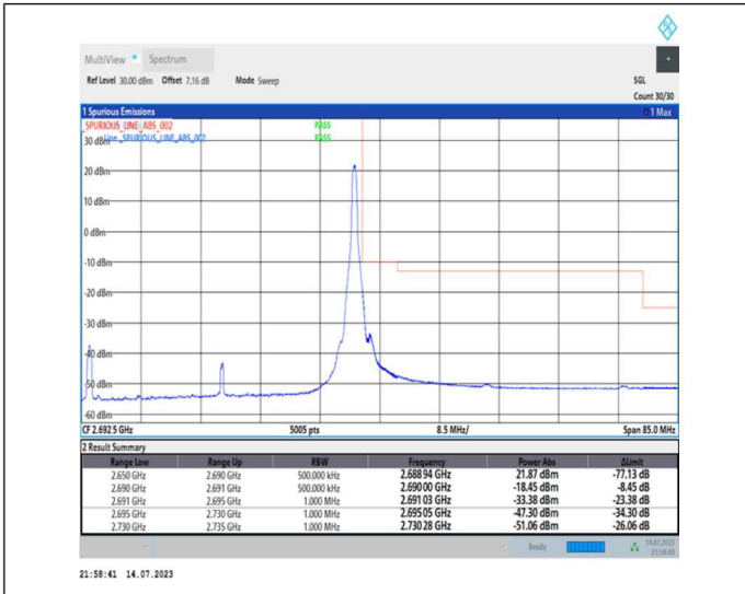
1-N41-PC1-30-40-H-2-DFT-PI2BPSK-Edge_1RB_Right-1@105-Ant0-1--PASS-see graph
