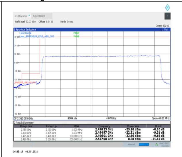
1-N41--30-40-L-3-DFT-PI2BPSK-Outer_Full-100@0-Ant0-PASS-see graph
