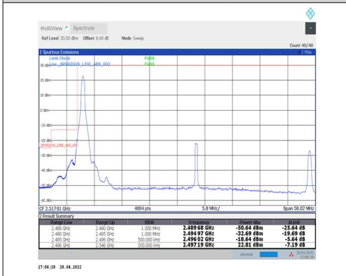
1-N41--30-50-L-4-CP-QPSK-Edge_1RB_Left-1@0-Ant0-PASS-see graph
