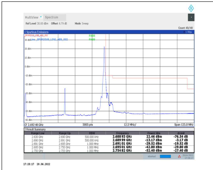
1-N41--30-60-H-2-DFT-PI2BPSK-Edge_1RB_Right-1@161-Ant0-PASS-see graph
