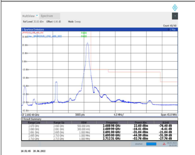
1-N41--30-20-H-5-CP-QPSK-Edge_1RB_Right-1@50-Ant0-PASS-see graph
