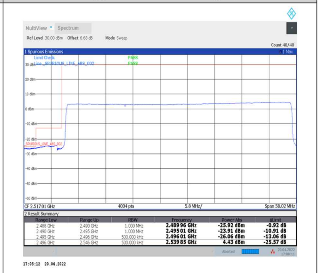
1-N41--30-50-L-6-CP-QPSK-Outer_Full-133@0-Ant0-PASS-see graph
