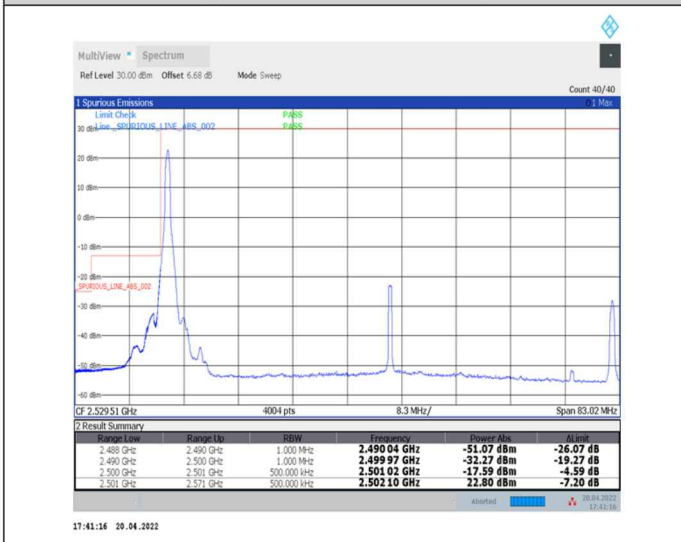
1-N41--30-70-L-4-CP-QPSK-Edge_1RB_Left-1@0-Ant0-PASS-see graph
