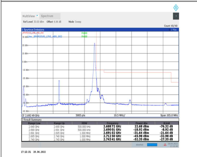
1-N41--30-50-H-5-CP-QPSK-Edge_1RB_Right-1@132-Ant0-PASS-see graph
