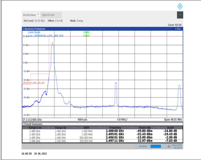
1-N41--30-40-L-4-CP-QPSK-Edge_1RB_Left-1@0-Ant0-PASS-see graph
