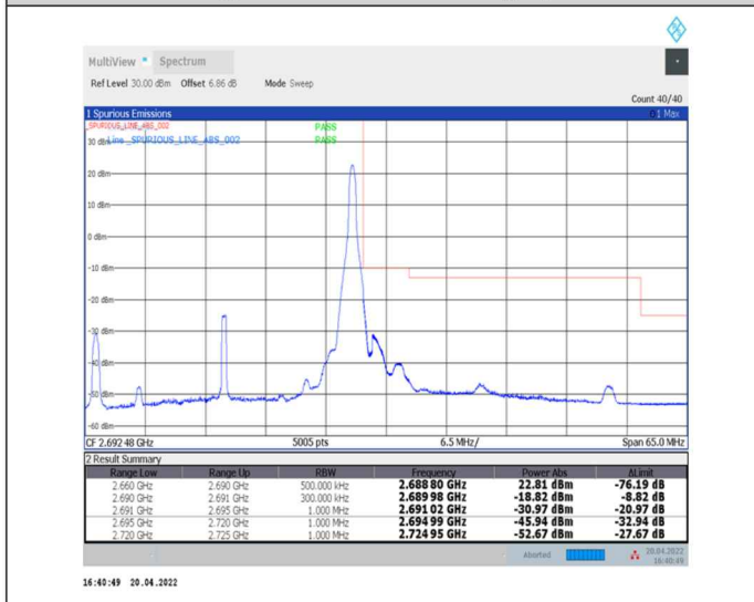
1-N41--30-30-H-5-CP-QPSK-Edge_1RB_Right-1@77-Ant0-PASS-see graph
