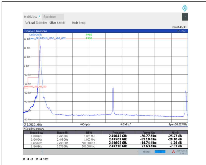
1-N41--30-80-L-1-DFT-PI2BPSK-Edge_1RB_Left-1@0-Ant0-PASS-see graph
