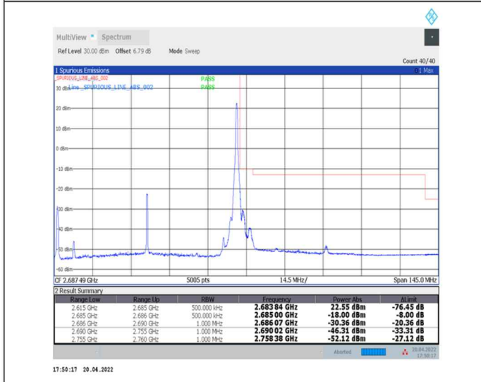
1-N41--30-70-H-5-CP-QPSK-Edge_1RB_Right-1@188-Ant0-PASS-see graph
