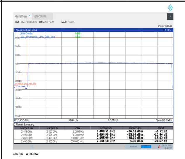
1-N41--30-90-L-6-CP-QPSK-Outer_Full-245@0-Ant0-PASS-see graph
