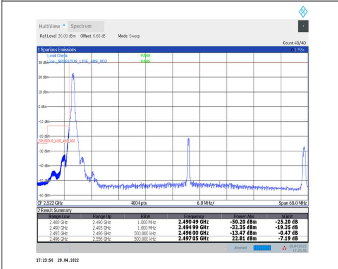
1-N41--30-60-L-4-CP-QPSK-Edge_1RB_Left-1@0-Ant0-PASS-see graph
