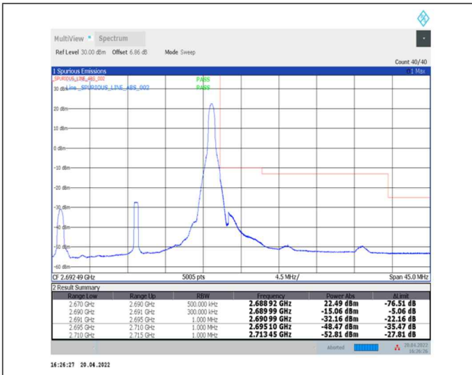
1-N41--30-20-H-2-DFT-PI2BPSK-Edge_1RB_Right-1@50-Ant0-PASS-see graph
