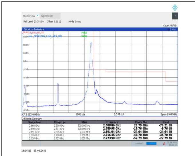
1-N41--30-30-H-2-DFT-PI2BPSK-Edge_1RB_Right-1@77-Ant0-PASS-see graph
