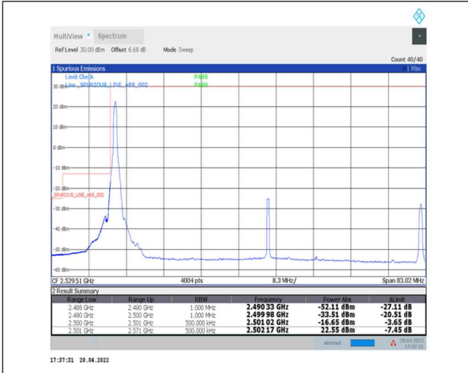
1-N41--30-70-L-1-DFT-PI2BPSK-Edge_1RB_Left-1@0-Ant0-PASS-see graph
