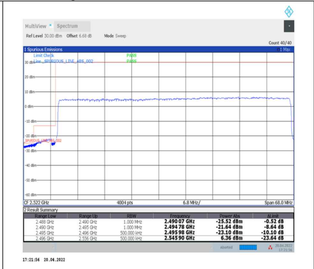
1-N41--30-60-L-3-DFT-PI2BPSK-Outer_Full-162@0-Ant0-PASS-see graph
