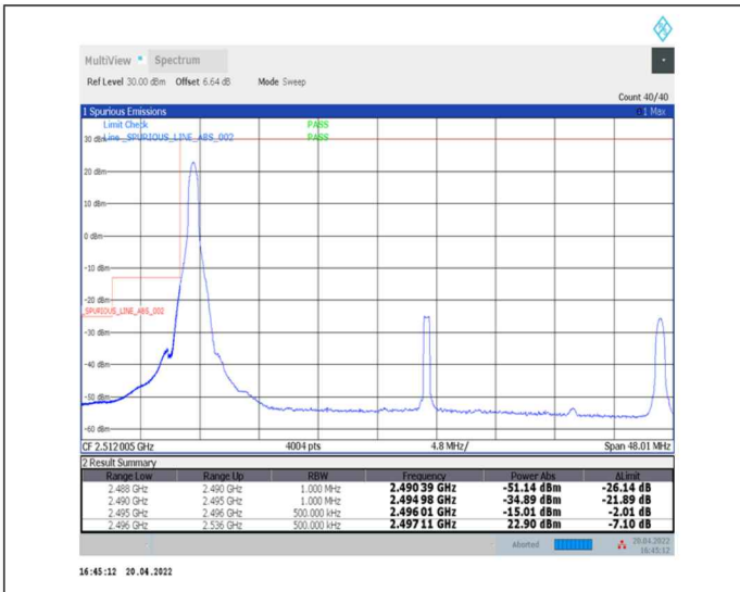
1-N41--30-40-L-1-DFT-PI2BPSK-Edge_1RB_Left-1@0-Ant0-PASS-see graph
