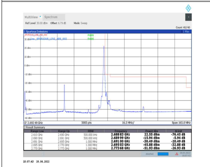
1-N41--30-80-H-5-CP-QPSK-Edge_1RB_Right-1@216-Ant0-PASS-see graph
