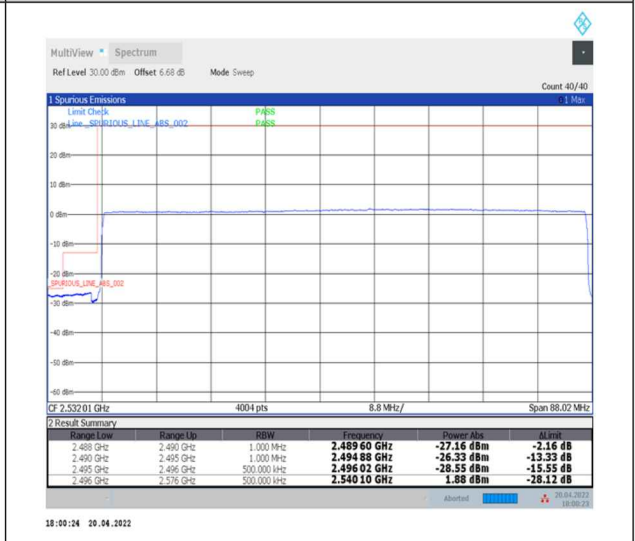
1-N41--30-80-L-6-CP-QPSK-Outer_Full-217@0-Ant0-PASS-see graph
