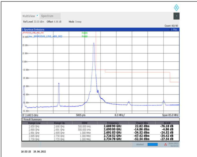
1-N41--30-40-H-2-DFT-PI2BPSK-Edge_1RB_Right-1@105-Ant0-PASS-see graph
