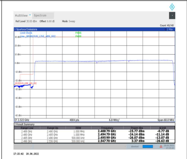
1-N41--30-60-L-6-CP-QPSK-Outer_Full-162@0-Ant0-PASS-see graph
