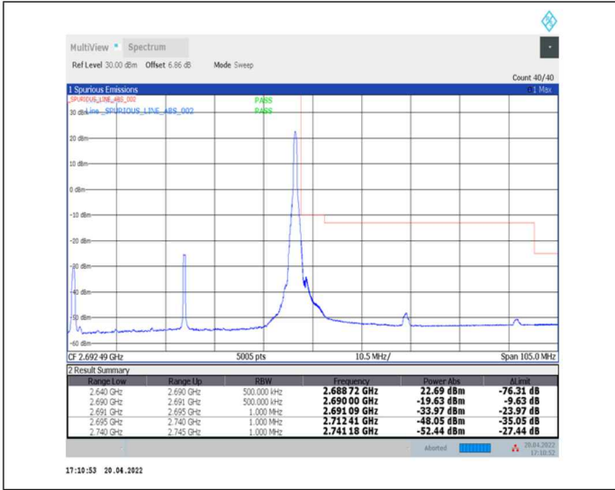
1-N41--30-50-H-2-DFT-PI2BPSK-Edge_1RB_Right-1@132-Ant0-PASS-see graph
