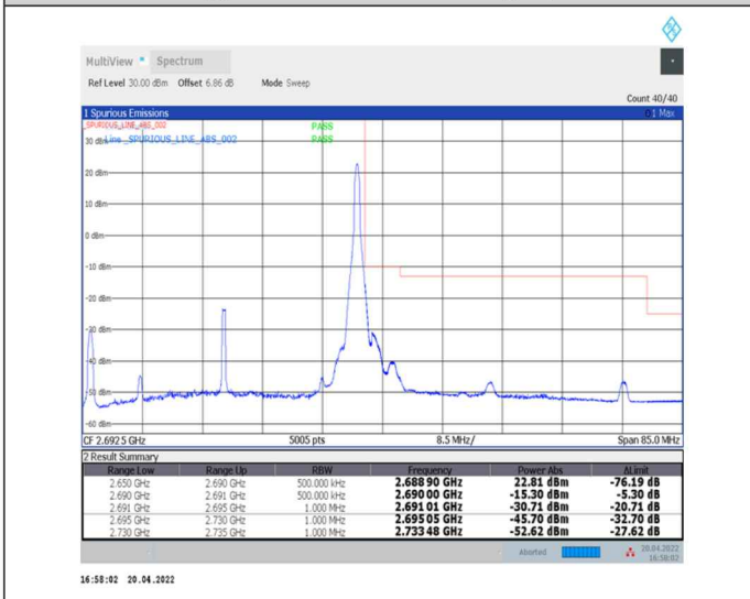
1-N41--30-40-H-5-CP-QPSK-Edge_1RB_Right-1@105-Ant0-PASS-see graph
