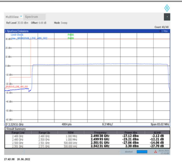
1-N41--30-70-L-6-CP-QPSK-Outer_Full-189@0-Ant0-PASS-see graph
