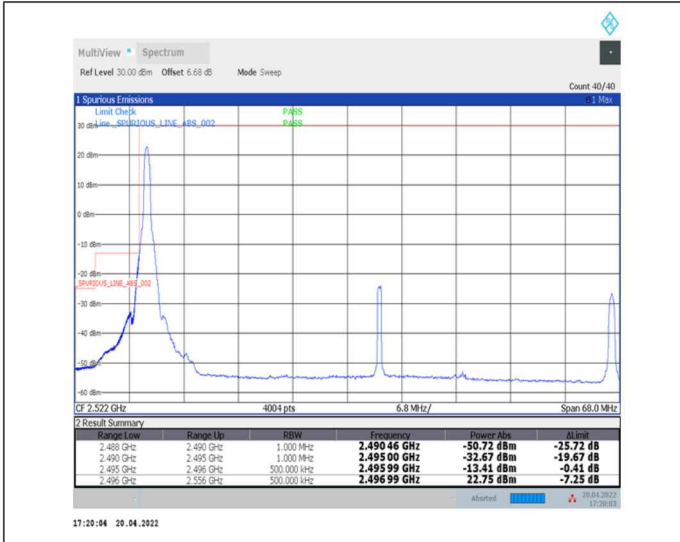
1-N41--30-60-L-1-DFT-PI2BPSK-Edge_1RB_Left-1@0-Ant0-PASS-see graph
