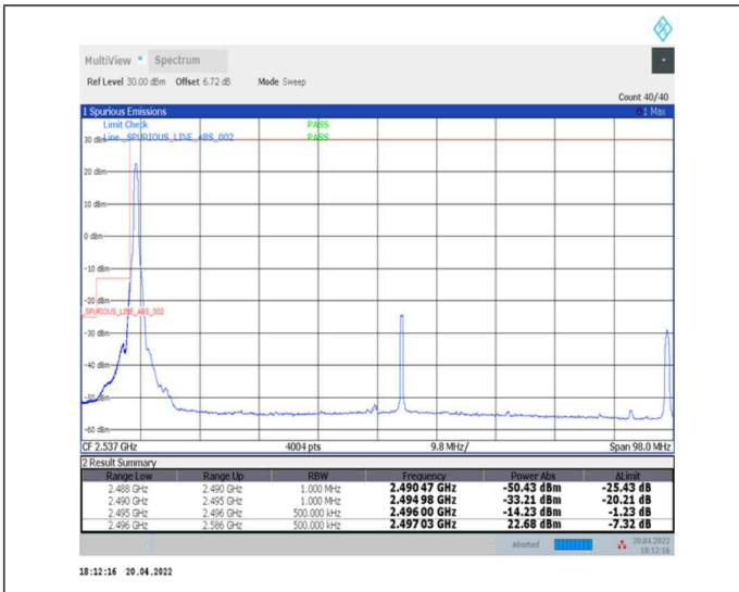
1-N41--30-90-L-1-DFT-PI2BPSK-Edge_1RB_Left-1@0-Ant0-PASS-see graph
