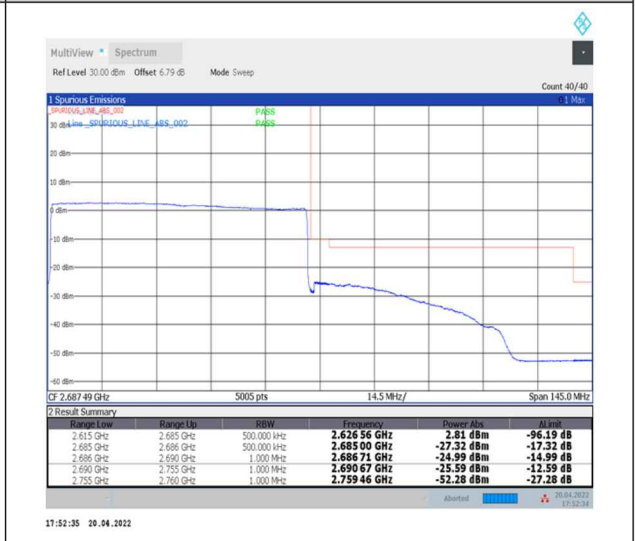
1-N41--30-70-H-6-CP-QPSK-Outer_Full-189@0-Ant0-PASS-see graph
