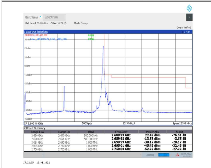
1-N41--30-60-H-5-CP-QPSK-Edge_1RB_Right-1@161-Ant0-PASS-see graph
