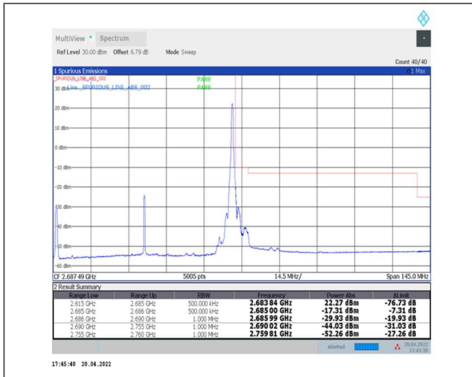
1-N41--30-70-H-2-DFT-PI2BPSK-Edge_1RB_Right-1@188-Ant0-PASS-see graph
