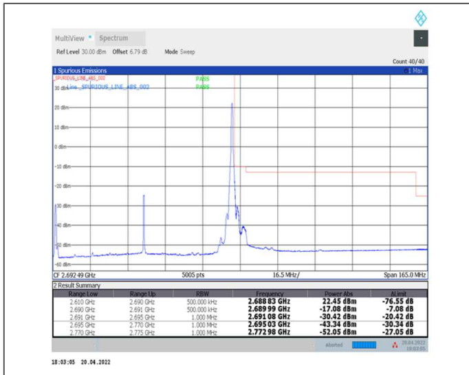
1-N41--30-80-H-2-DFT-PI2BPSK-Edge_1RB_Right-1@216-Ant0-PASS-see graph
