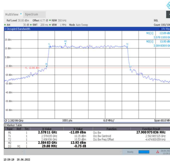
1-N41--30-30-M-8-CP-64QAM-Outer_Full-78@0-Ant0-27.901-29.880-≤30-PASS
