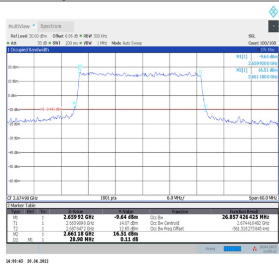
1-N41--30-30-H-1-DFT-QPSK-Outer_Full-75@0-Ant0-26.857-28.980-≤30-PASS
