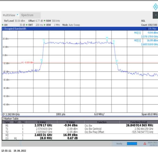
1-N41--30-30-M-1-DFT-QPSK-Outer_Full-75@0-Ant0-26.841-28.800-≤30-PASS
