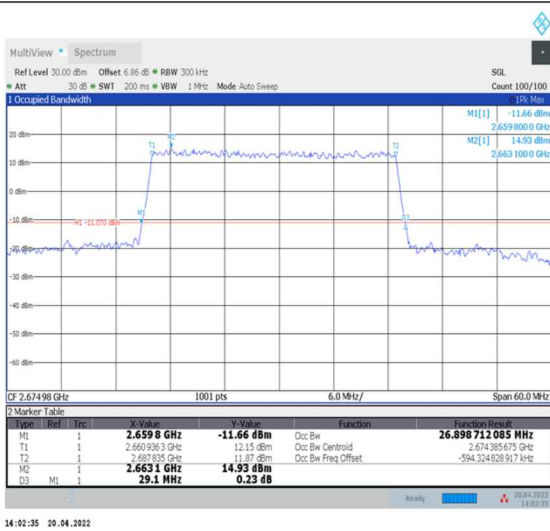
1-N41--30-30-H-4-DFT-64QAM-Outer_Full-75@0-Ant0-26.899-29.100-≤30-PASS
