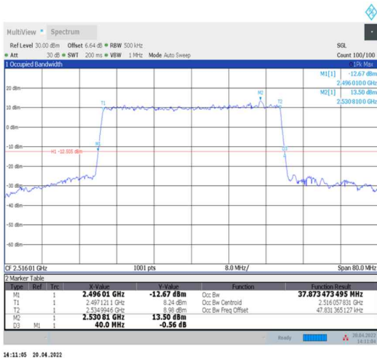
1-N41--30-40-L-9-CP-256QAM-Outer_Full-106@0-Ant0-37.873-40.000-<math>\leq 40</math>-PASS
