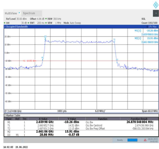
1-N41--30-30-H-3-DFT-16QAM-Outer_Full-75@0-Ant0-26.879-28.860-≤30-PASS
