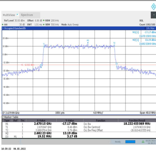
1-N41--30-20-H-7-CP-16QAM-Outer_Full-51@0-Ant0-18.232-19.520-<20-PASS
