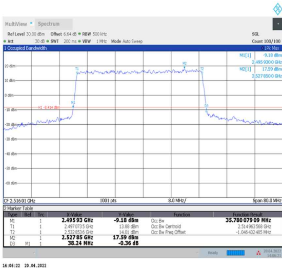
1-N41--30-40-L-1-DFT-QPSK-Outer_Full-100@0-Ant0-35.78-38.240-≤40-PASS
