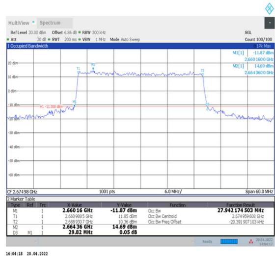
1-N41--30-30-H-7-CP-16QAM-Outer_Full-78@0-Ant0-27.942-29.820-≤30-PASS
