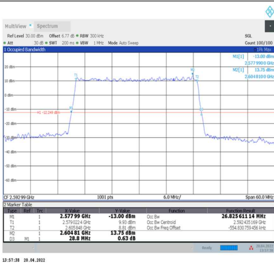
1-N41--30-30-M-5-DFT-256QAM-Outer_Full-75@0-Ant0-26.826-28.800-≤30-PASS
