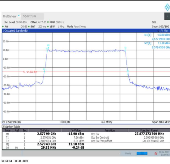
1-N41--30-30-M-9-CP-256QAM-Outer_Full-78@0-Ant0-27.877-29.820-≤30-PASS
