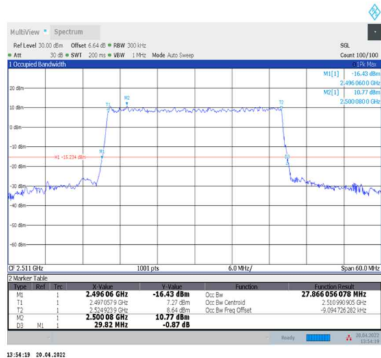
1-N41--30-30-L-9-CP-256QAM-Outer_Full-78@0-Ant0-27.866-29.820-≤30-PASS
