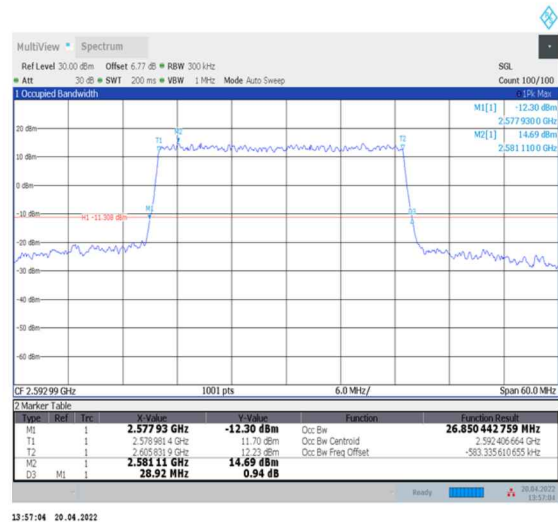
1-N41--30-30-M-4-DFT-64QAM-Outer_Full-75@0-Ant0-26.85-28.920-≤30-PASS
