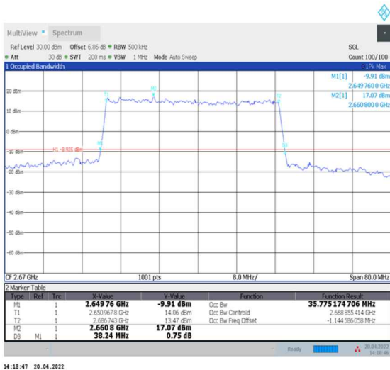
1-N41--30-40-H-3-DFT-16QAM-Outer_Full-100@0-Ant0-35.775-38.240-≤40-PASS
