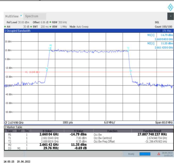
1-N41--30-30-H-9-CP-256QAM-Outer_Full-78@0-Ant0-27.888-29.760-≤30-PASS
