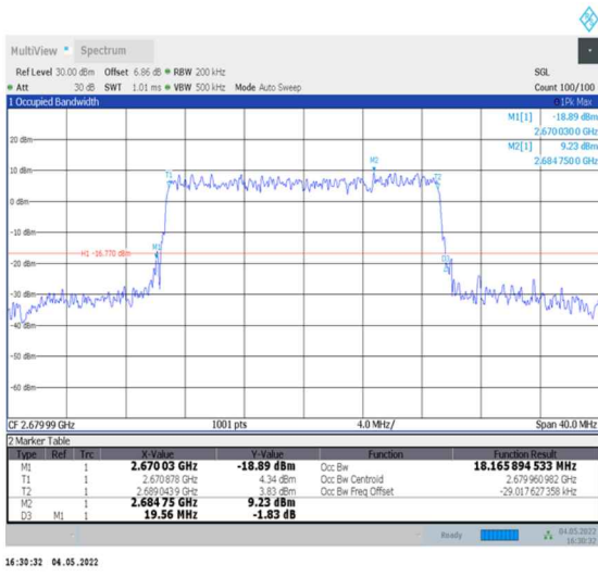
1-N41--30-20-H-9-CP-256QAM-Outer_Full-51@0-Ant0-18.166-19.560-<20-PASS
