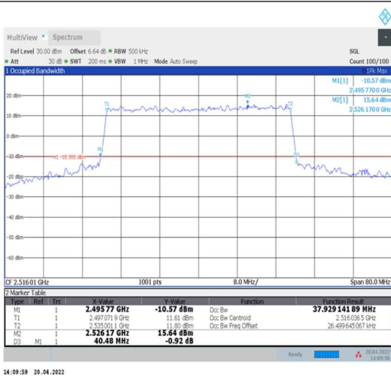
1-N41--30-40-L-7-CP-16QAM-Outer_Full-106@0-Ant0-37.929-40.480-<math>\leq 40</math>-PASS
