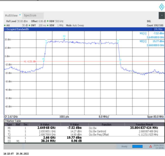
1-N41--30-40-H-2-DFT-PI2BPSK-Outer_Full-100@0-Ant0-35.805-38.240-≤40-PASS
