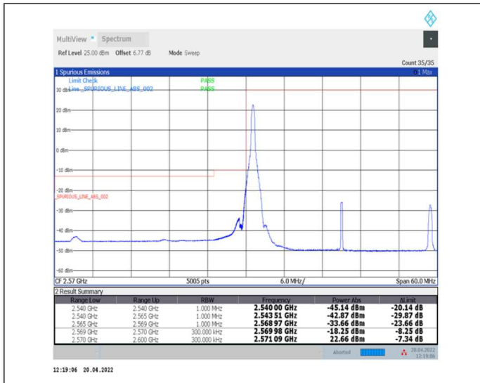
1-N38--30-30-L-1-DFT-PI2BPSK-Edge_1RB_Left-1@0-Ant0-PASS-see graph
