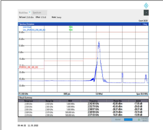
1-N38-PC2-30-20-L-4-CP-QPSK-Edge_1RB_Left-1@0-Ant0-PASS-see graph
