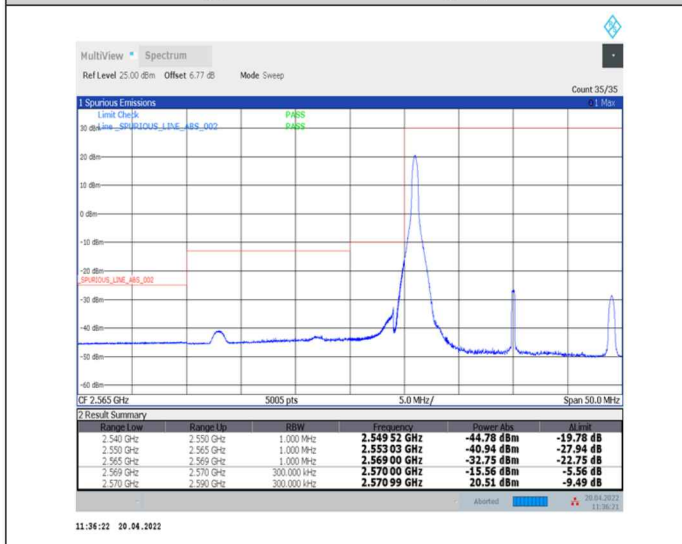
1-N38--30-20-L-4-CP-QPSK-Edge_1RB_Left-1@0-Ant0-PASS-see graph
