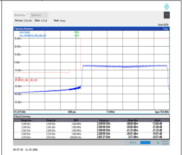
1-N38-PC2-30-40-L-6-CP-QPSK-Outer_Full-106@0-Ant0-PASS-see graph
