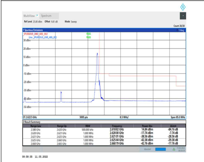
1-N38-PC2-30-40-H-5-CP-QPSK-Edge_1RB_Right-1@105-Ant0-PASS-see graph
