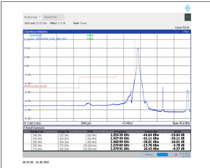
1-N38--30-15-L-1-DFT-PI2BPSK-Edge_1RB_Left-1@0-Ant0-PASS-see graph
