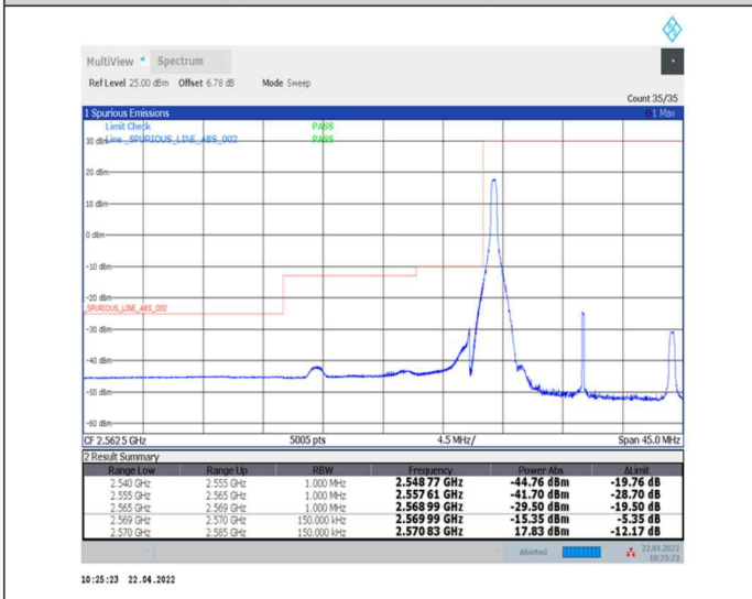
1-N38--30-15-L-4-CP-QPSK-Edge_1RB_Left-1@0-Ant0-PASS-see graph
