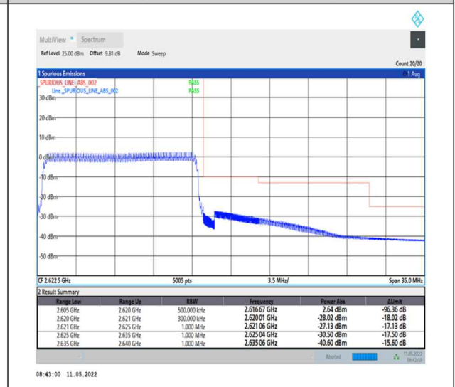
1-N38-PC2-30-15-H-6-CP-QPSK-Outer_Full-38@0-Ant0-PASS-see graph
