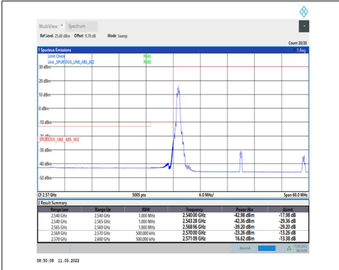
1-N38-PC2-30-30-L-4-CP-QPSK-Edge_1RB_Left-1@0-Ant0-PASS-see graph
