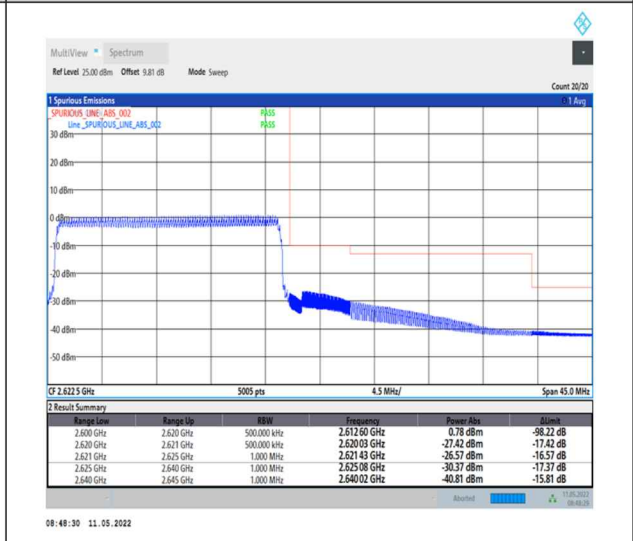
1-N38-PC2-30-20-H-6-CP-QPSK-Outer_Full-51@0-Ant0-PASS-see graph
