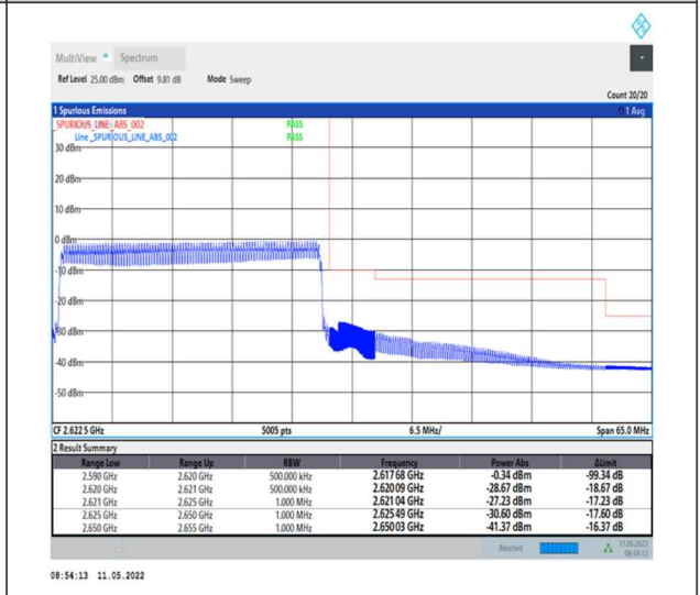
1-N38-PC2-30-30-H-6-CP-QPSK-Outer_Full-78@0-Ant0-PASS-see graph
