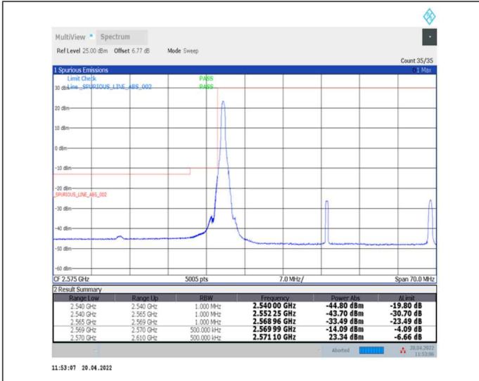
1-N38--30-40-L-1-DFT-PI2BPSK-Edge_1RB_Left-1@0-Ant0-PASS-see graph
