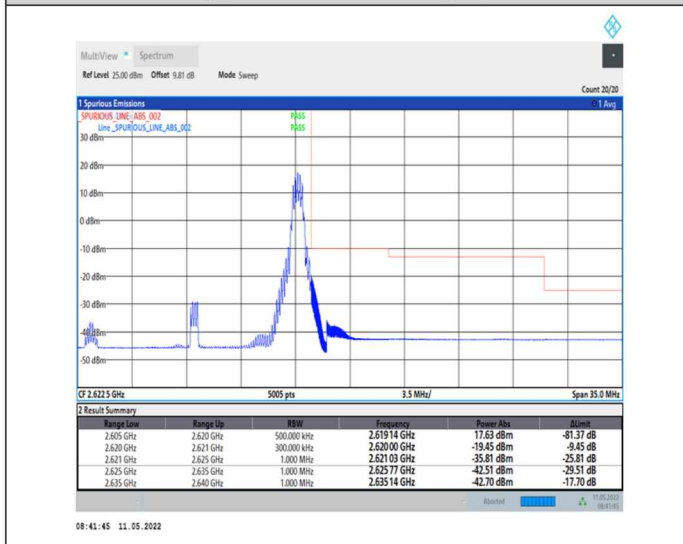
1-N38-PC2-30-15-H-5-CP-QPSK-Edge_1RB_Right-1@37-Ant0-PASS-see graph
