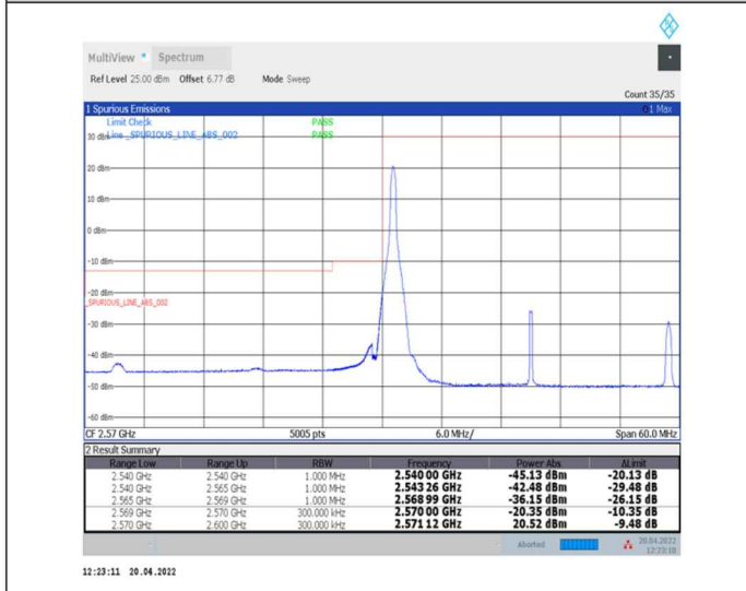
1-N38--30-30-L-4-CP-QPSK-Edge_1RB_Left-1@0-Ant0-PASS-see graph
