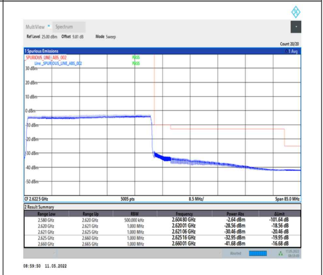
1-N38-PC2-30-40-H-6-CP-QPSK-Outer_Full-106@0-Ant0-PASS-see graph
