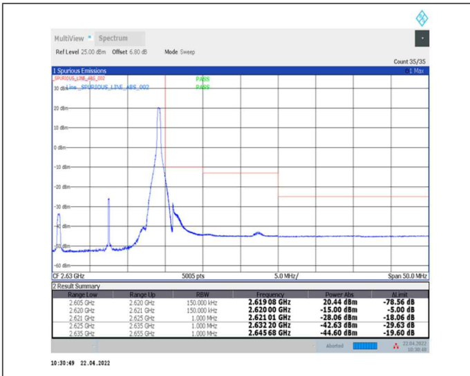
1-N38--30-15-H-2-DFT-PI2BPSK-Edge_1RB_Right-1@37-Ant0-PASS-see graph
