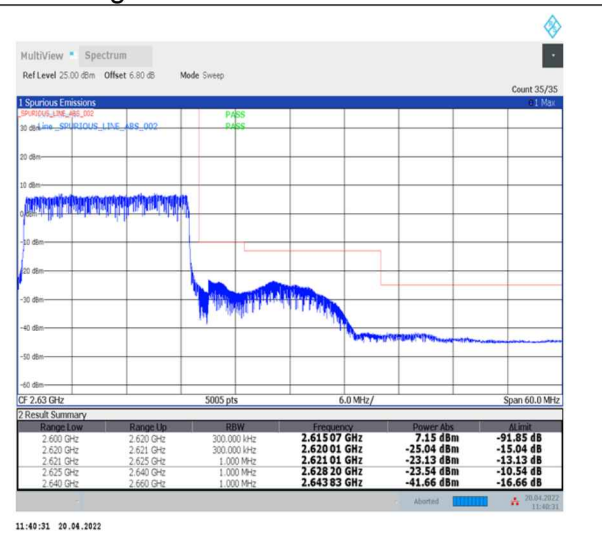
1-N38--30-20-H-3-DFT-PI2BPSK-Outer_Full-50@0-Ant0-PASS-see graph
