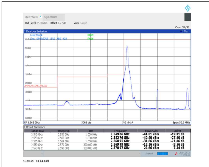
1-N38--30-20-L-1-DFT-PI2BPSK-Edge_1RB_Left-1@0-Ant0-PASS-see graph
