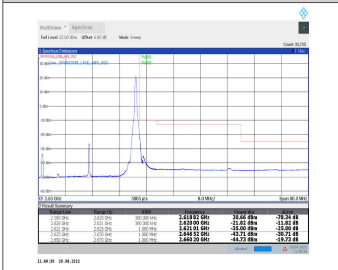
1-N38--30-30-H-5-CP-QPSK-Edge_1RB_Right-1@77-Ant0-PASS-see graph
