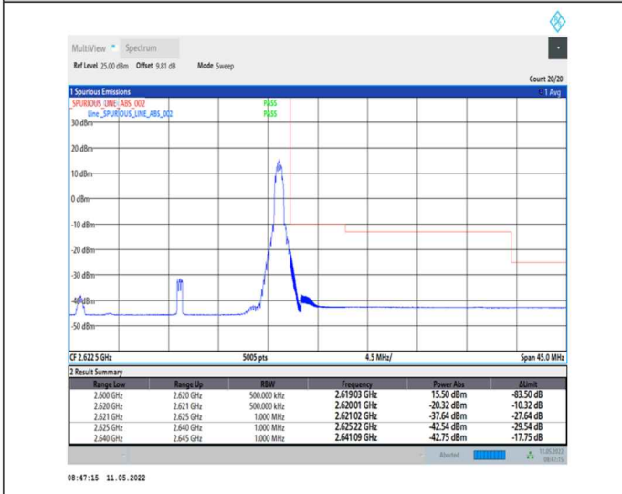
1-N38-PC2-30-20-H-5-CP-QPSK-Edge_1RB_Right-1@50-Ant0-PASS-see graph
