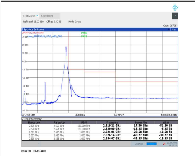
1-N38--30-15-H-5-CP-QPSK-Edge_1RB_Right-1@37-Ant0-PASS-see graph
