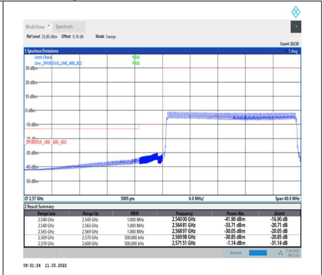
1-N38-PC2-30-30-L-6-CP-QPSK-Outer_Full-78@0-Ant0-PASS-see graph
