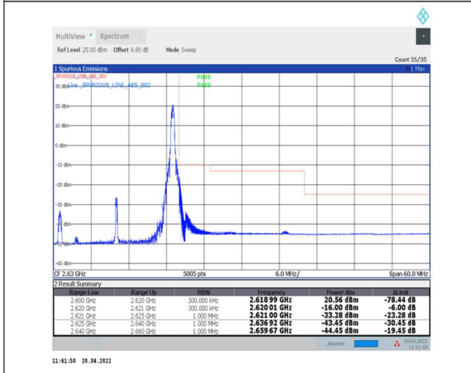
1-N38--30-20-H-5-CP-QPSK-Edge_1RB_Right-1@50-Ant0-PASS-see graph
