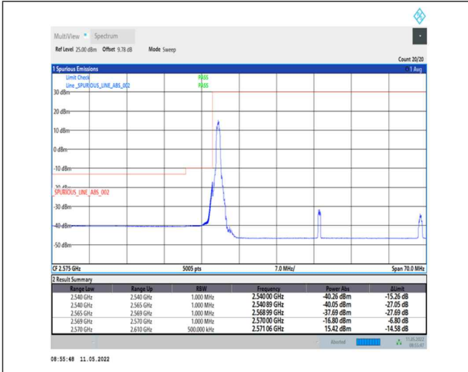
1-N38-PC2-30-40-L-4-CP-QPSK-Edge_1RB_Left-1@0-Ant0-PASS-see graph
