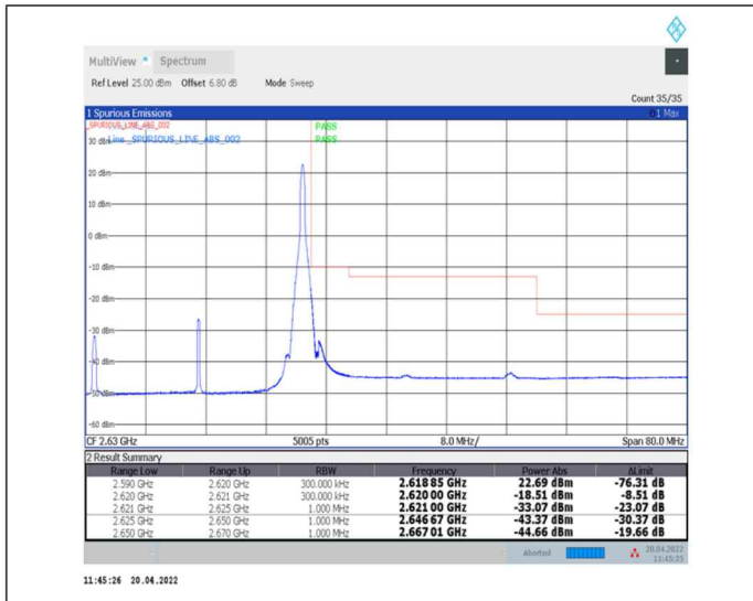
1-N38--30-30-H-2-DFT-PI2BPSK-Edge_1RB_Right-1@77-Ant0-PASS-see graph
