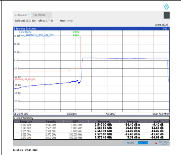
1-N38--30-40-L-6-CP-QPSK-Outer_Full-106@0-Ant0-PASS-see graph
