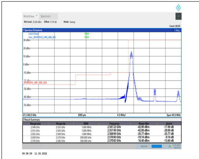
1-N38-PC2-30-15-L-4-CP-QPSK-Edge_1RB_Left-1@0-Ant0-PASS-see graph
