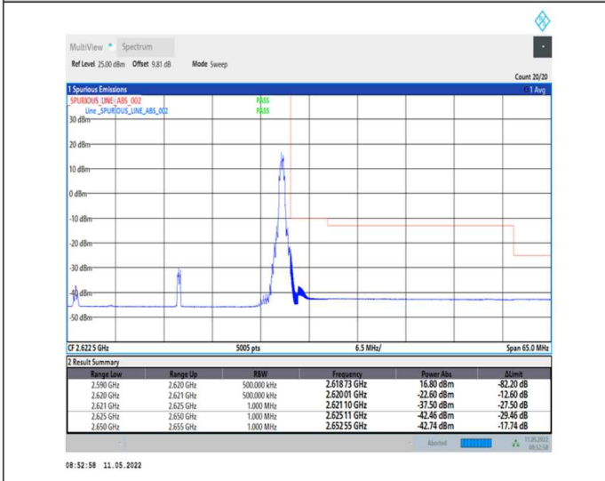
1-N38-PC2-30-30-H-5-CP-QPSK-Edge_1RB_Right-1@77-Ant0-PASS-see graph
