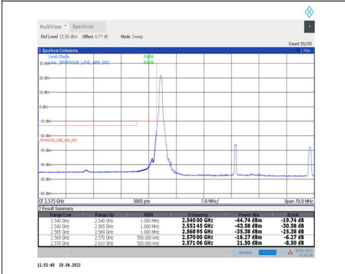
1-N38--30-40-L-4-CP-QPSK-Edge_1RB_Left-1@0-Ant0-PASS-see graph
