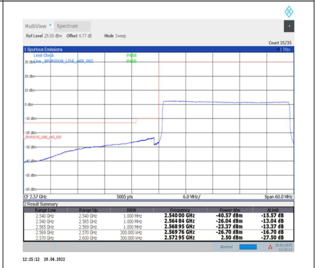
1-N38--30-30-L-6-CP-QPSK-Outer_Full-78@0-Ant0-PASS-see graph
