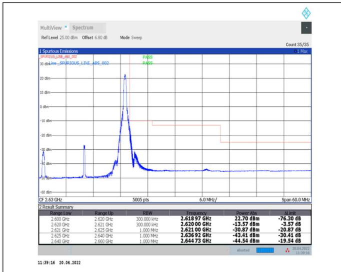
1-N38--30-20-H-2-DFT-PI2BPSK-Edge_1RB_Right-1@50-Ant0-PASS-see graph
