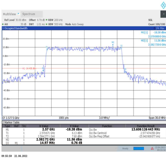
1-N38--30-15-L-8-CP-64QAM-Outer_Full-38@0-Ant0-13.606-14.970-≤15-PASS
