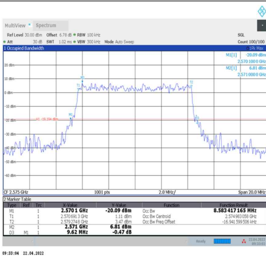
1-N38-30-10-L-9-CP-256QAM-Outer_Full-24@0-Ant0-8.583-9.620-≤10-PASS
