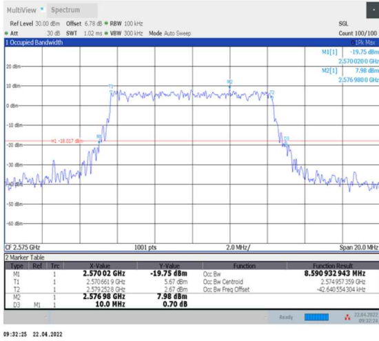
1-N38--30-10-L-5-DFT-256QAM-Outer_Full-24@0-Ant0-8.591-10.000-≤10-PASS
