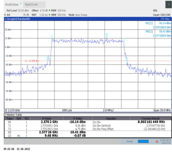
1-N38--30-10-L-6-CP-QPSK-Outer_Full-24@0-Ant0-8.565-9.480-≤10-PASS
