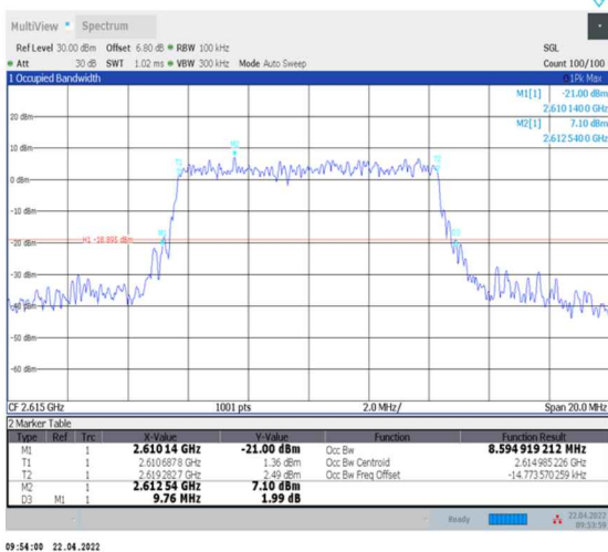
1-N38--30-10-H-9-CP-256QAM-Outer_Full-24@0-Ant0-8.595-9.760-≤10-PASS
