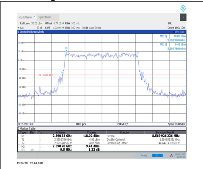
1-N38--30-10-M-5-DFT-256QAM-Outer_Full-24@0-Ant0-8.57-9.500-≤10-PASS
