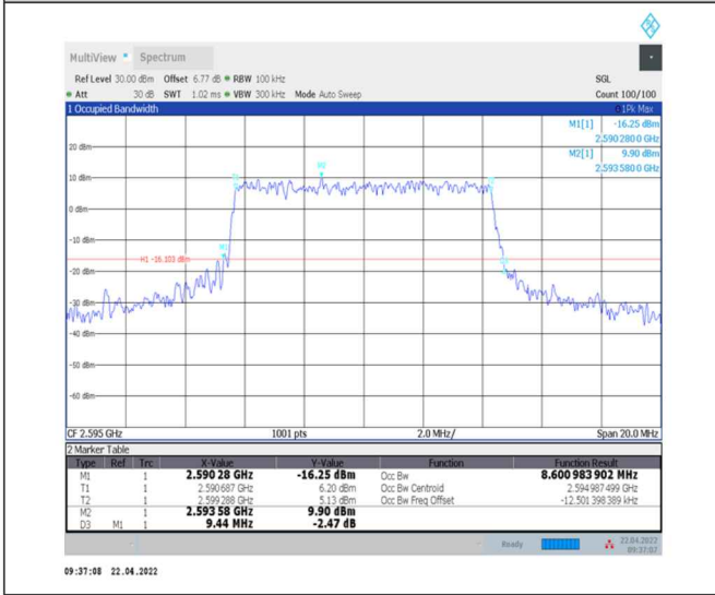
1-N38--30-10-M-6-CP-QPSK-Outer_Full-24@0-Ant0-8.601-9.440-≤10-PASS
