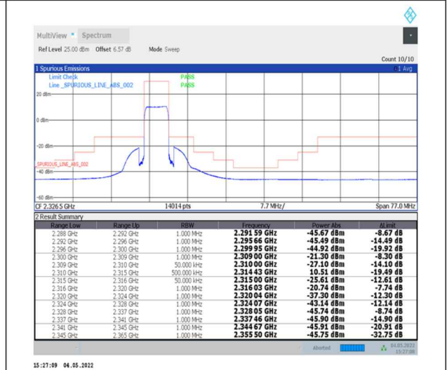
1-N30--15-5-H-6-CP-QPSK-Outer_Full-25@0-Ant0-PASS-see graph
