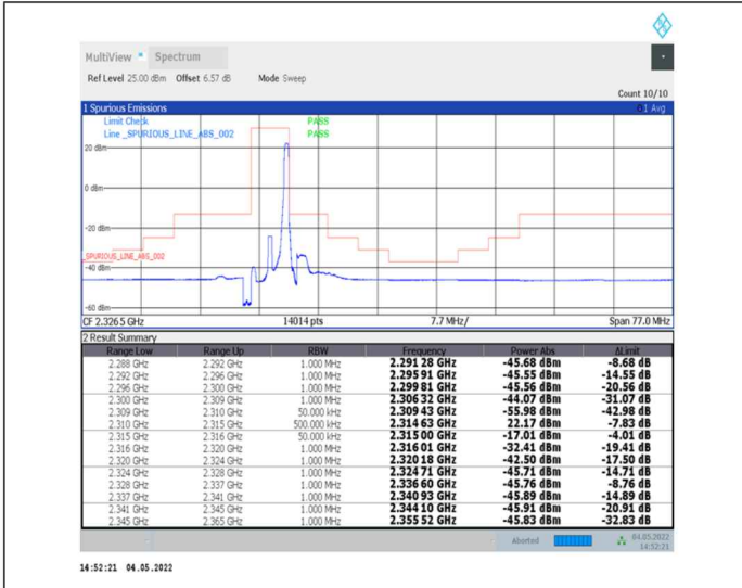
1-N30--15-5-H-2-DFT-PI2BPSK-Edge_1RB_Right-1@24-Ant0-PASS-see graph
