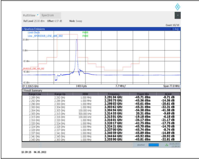
1-N30--15-10-H-5-CP-QPSK-Edge_1RB_Right-1@51-Ant0-PASS-see graph
