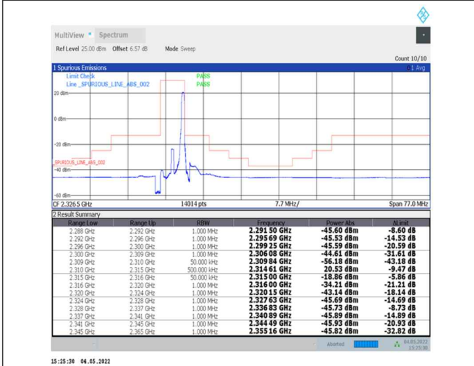
1-N30--15-5-H-5-CP-QPSK-Edge_1RB_Right-1@24-Ant0-PASS-see graph
