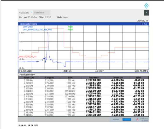
1-N30--30-10-L-1-DFT-PI2BPSK-Edge_1RB_Left-1@0-Ant0-PASS-see graph
