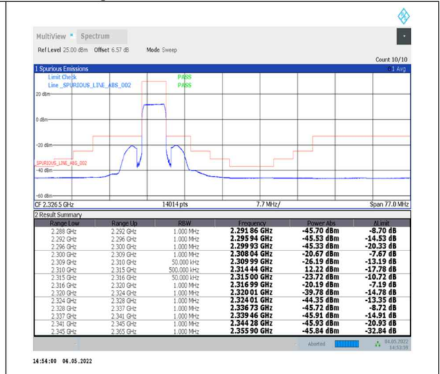
1-N30--15-5-H-3-DFT-PI2BPSK-Outer_Full-25@0-Ant0-PASS-see graph
