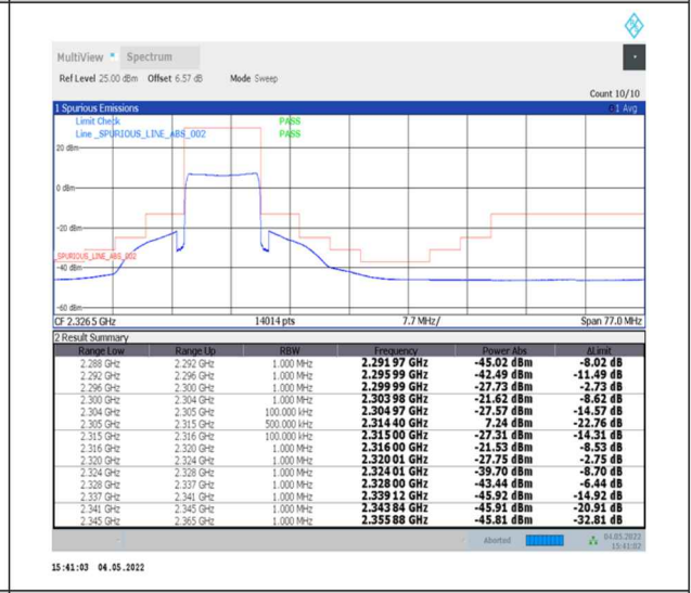
1-N30--15-10-H-6-CP-QPSK-Outer_Full-52@0-Ant0-PASS-see graph
