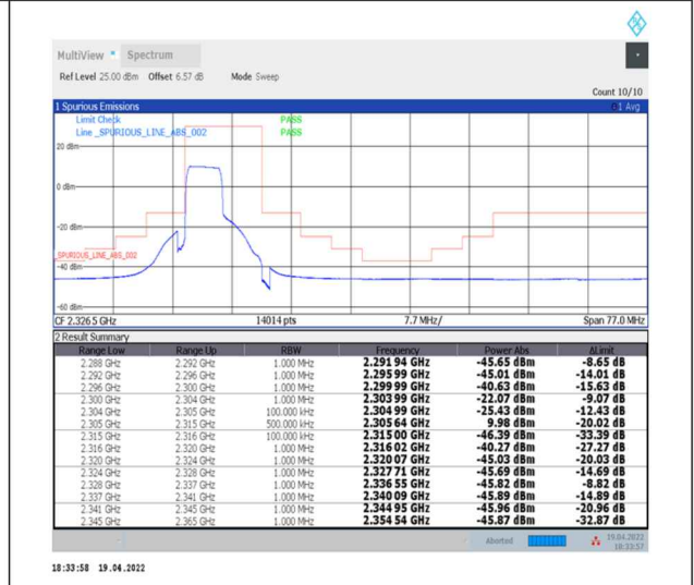
1-N30--30-10-L-6-CP-QPSK-Outer_Full-24@0-Ant0-PASS-see graph
