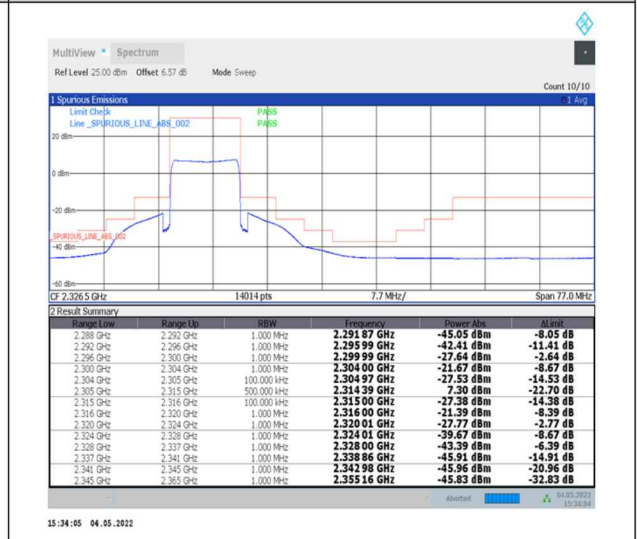
1-N30--15-10-L-6-CP-QPSK-Outer_Full-52@0-Ant0-PASS-see graph
