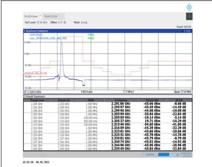
1-N30--15-10-L-4-CP-QPSK-Edge_1RB_Left-1@0-Ant0-PASS-see graph
