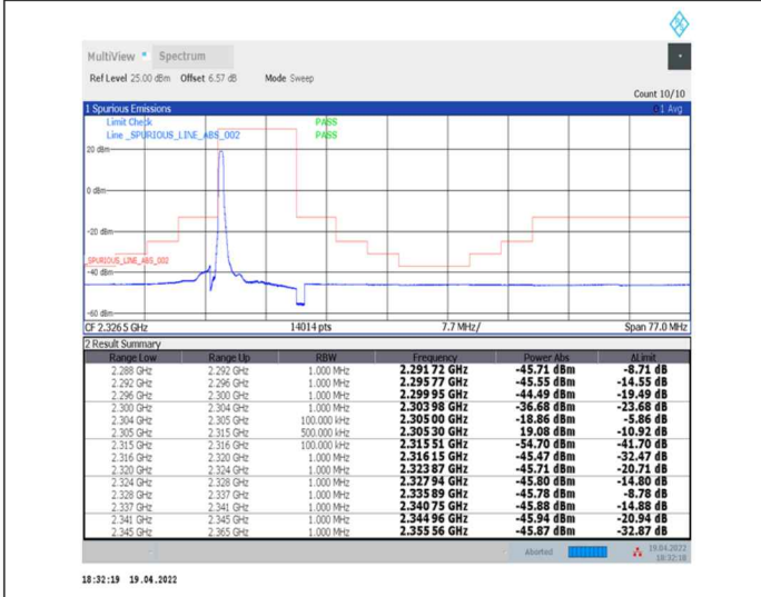
1-N30--30-10-L-4-CP-QPSK-Edge_1RB_Left-1@0-Ant0-PASS-see graph
