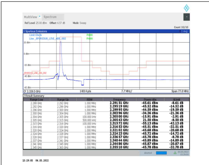
1-N30--15-10-L-1-DFT-PI2BPSK-Edge_1RB_Left-1@0-Ant0-PASS-see graph
