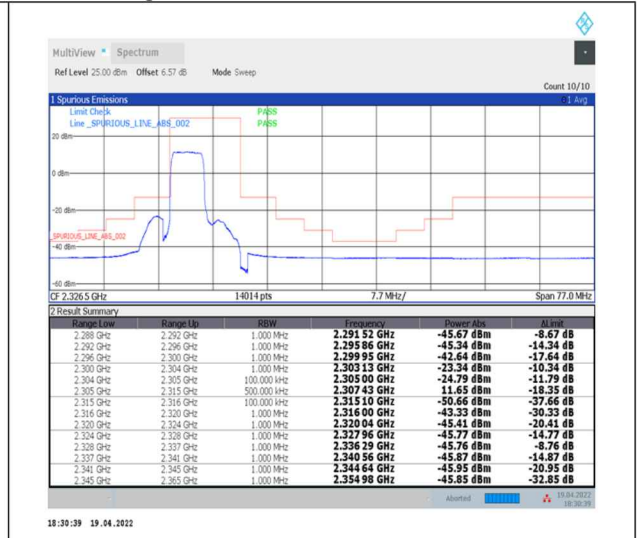
1-N30--30-10-L-3-DFT-PI2BPSK-Outer_Full-24@0-Ant0-PASS-see graph
