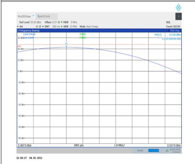
1-N30-PC3-15-5-H-1-DFT-PI2BPSK- Inner_1RB_Left-1@1-2307.5-2317.5-Ant0-21.50- 23.98-PASS
