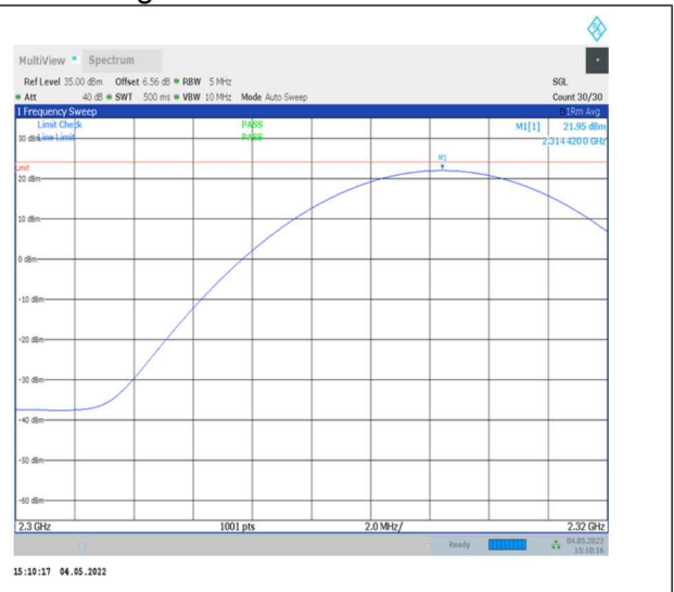
1-N30-PC3-15-10-M-2-DFT-PI2BPSK- Inner_1RB_Right-1@50-2300-2320-Ant0-21.95- 23.98-PASS
