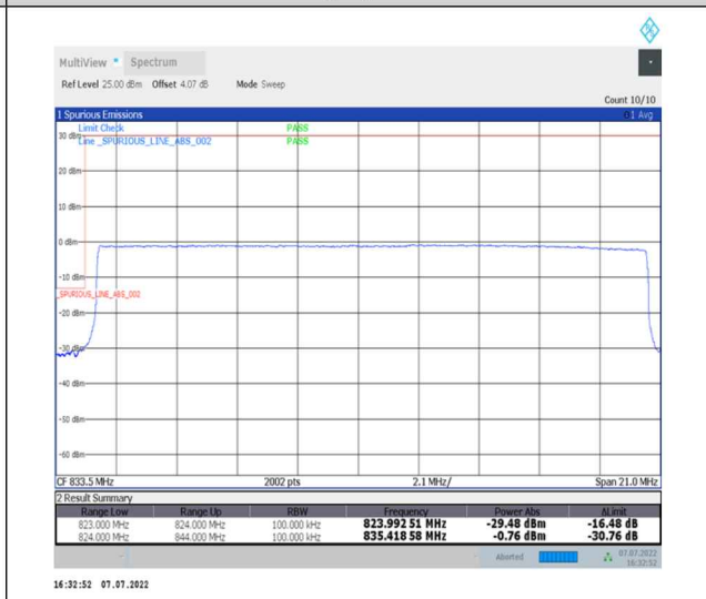
1-N26-824-849--15-20-L-6-CP-QPSK-Outer_Full-106@0-Ant0-seegraph-PASS-see graph
