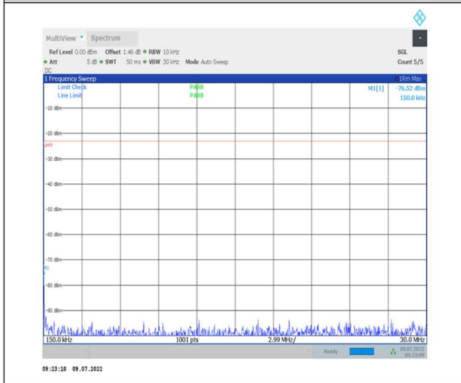
1-N26-824-849-PC3-15-20-M-1-DFT-PI2BPSK- Inner_1RB_Left-1@1-0.15-30-Ant0--76.52--33-PASS
