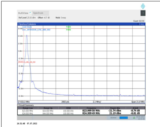
1-N26-824-849--15-20-L-1-DFT-PI2BPSK-Edge_1RB_Left-1@0-Ant0-seegraph-PASS-see graph
