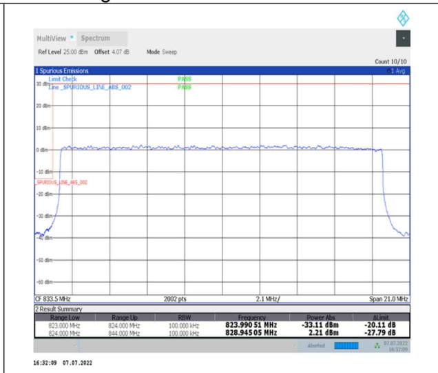
1-N26-824-849--15-20-L-3-DFT-PI2BPSK-Outer_Full-100@0-Ant0-seegraph-PASS-see graph
