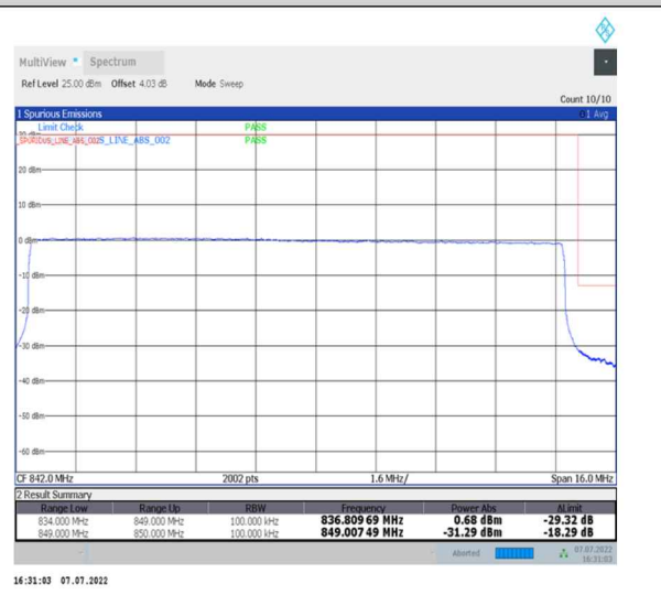
1-N26-824-849--15-15-H-6-CP-QPSK-Outer_Full-79@0-Ant0-seegraph-PASS-see graph
