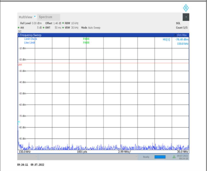
1-N26-824-849-PC3-15-20-H-1-DFT-PI2BPSK- Inner_1RB_Left-1@1-0.15-30-Ant0--78.48--33-PASS
