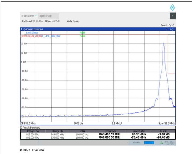
1-N26-824-849--15-20-H-2-DFT-PI2BPSK-Edge_1RB_Right-1@105-Ant0-seegraph-PASS-see graph
