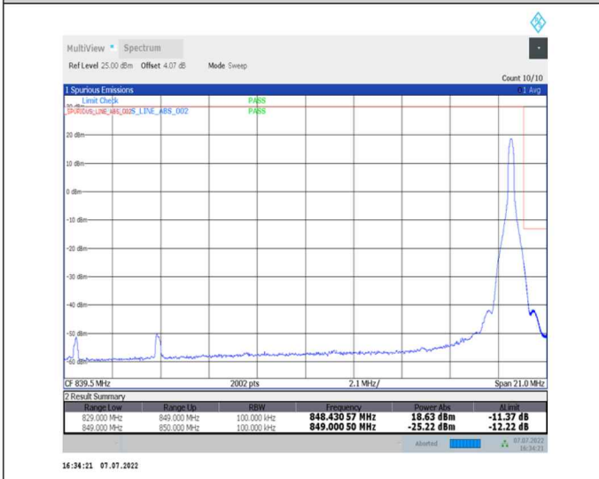
1-N26-824-849--15-20-H-5-CP-QPSK-Edge_1RB_Right-1@105-Ant0-seegraph-PASS-see graph
