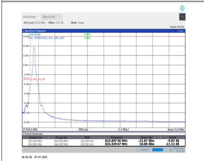
1-N26-824-849--15-20-L-4-CP-QPSK-Edge_1RB_Left-1@0-Ant0-seegraph-PASS-see graph
