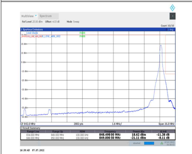
1-N26-824-849--15-15-H-5-CP-QPSK-Edge_1RB_Right-1@78-Ant0-seegraph-PASS-see graph
