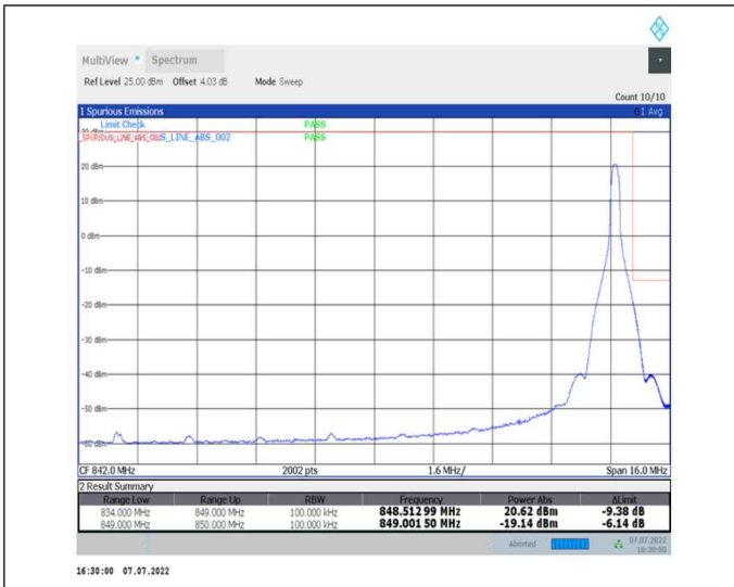
1-N26-824-849--15-15-H-2-DFT-PI2BPSK-Edge_1RB_Right-1@78-Ant0-seegraph-PASS-see graph
