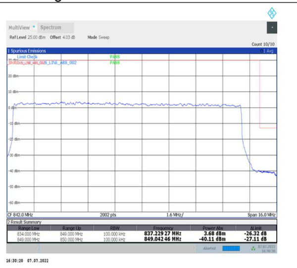
1-N26-824-849--15-15-H-3-DFT-PI2BPSK-Outer_Full-75@0-Ant0-seegraph-PASS-see graph
