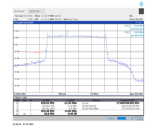
1-N26-824-849--15-20-H-1-DFT-QPSK-Outer_Full-100@0-Ant0-17.848-18.800-<=20-PASS
