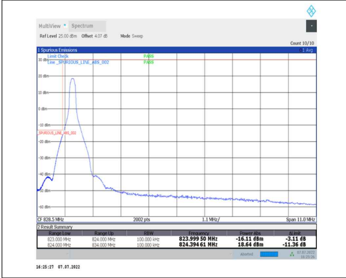
1-N26-824-849--15-10-L-4-CP-QPSK-Edge_1RB_Left-1@0-Ant0-seegraph-PASS-see graph
