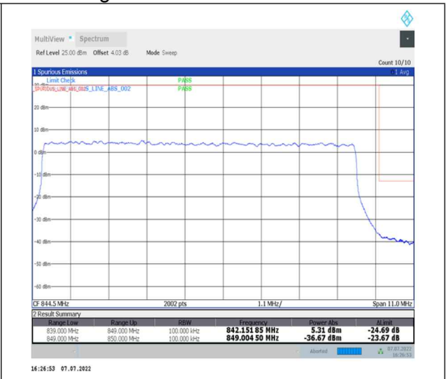
1-N26-824-849--15-10-H-3-DFT-PI2BPSK-Outer_Full-50@0-Ant0-seegraph-PASS-see graph
