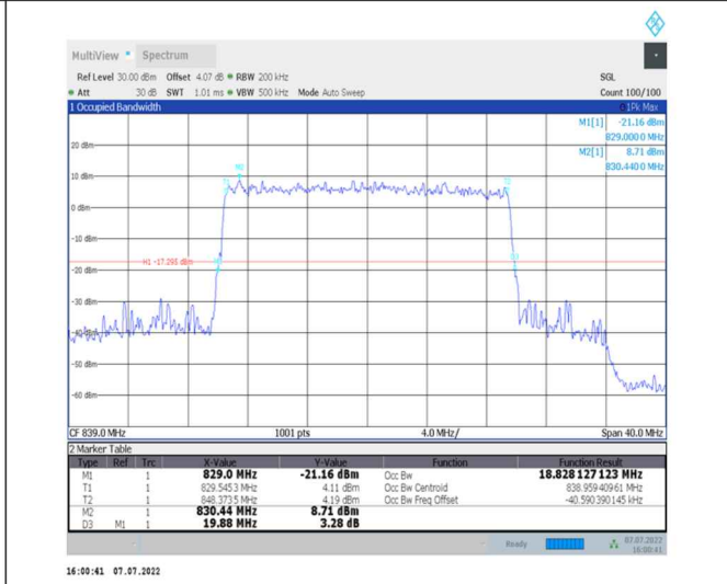
1-N26-824-849--15-20-H-9-CP-256QAM-Outer_Full-106@0-Ant0-18.828-19.880-<=20-PASS
