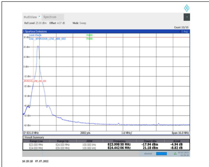
1-N26-824-849--15-15-L-1-DFT-PI2BPSK-Edge_1RB_Left-1@0-Ant0-seegraph-PASS-see graph
