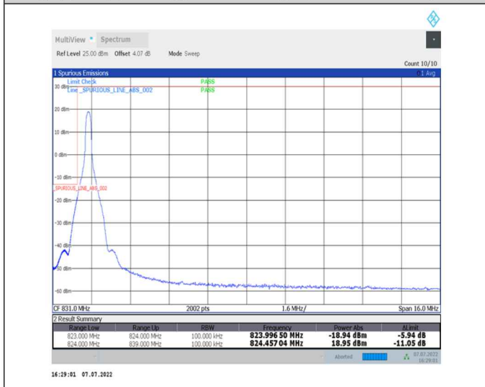
1-N26-824-849--15-15-L-4-CP-QPSK-Edge_1RB_Left-1@0-Ant0-seegraph-PASS-see graph
