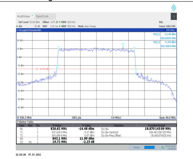
1-N26-824-849--15-20-M-8-CP-64QAM-Outer_Full-106@0-Ant0-18.87-19.720-<=20-PASS
