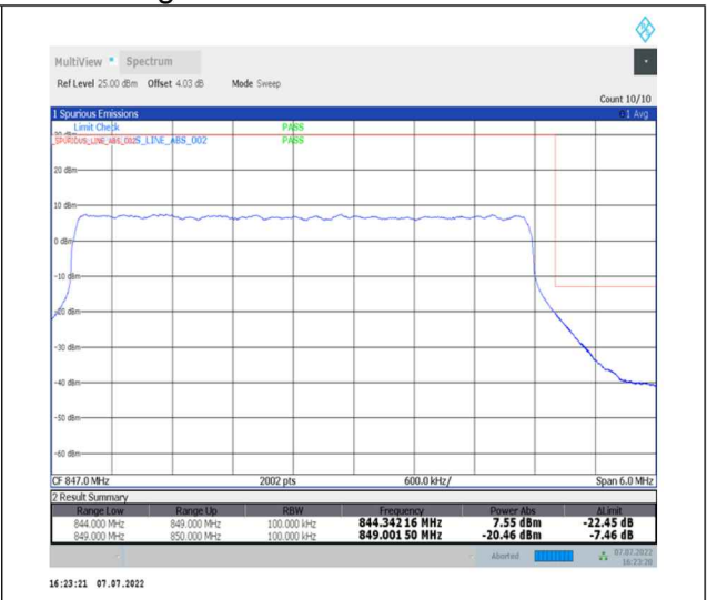
1-N26-824-849--15-5-H-3-DFT-PI2BPSK-Outer_Full-25@0-Ant0-seegraph-PASS-see graph
