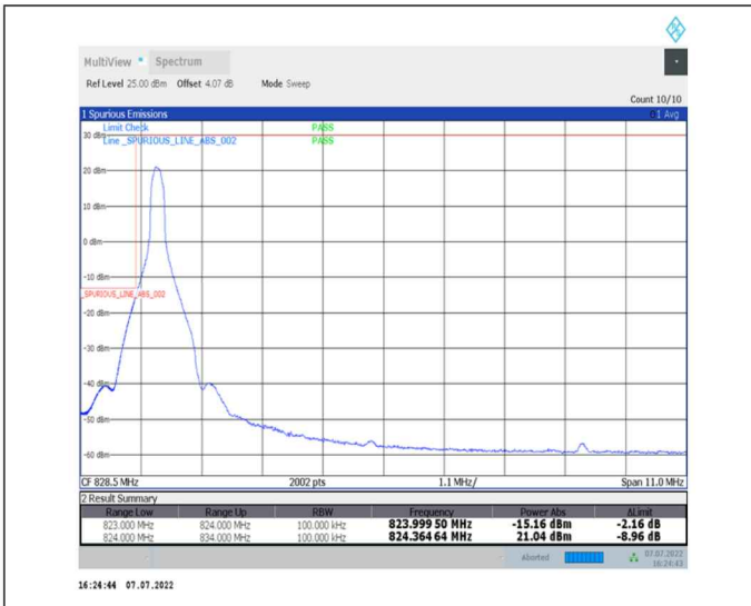
1-N26-824-849--15-10-L-1-DFT-PI2BPSK-Edge_1RB_Left-1@0-Ant0-seegraph-PASS-see graph
