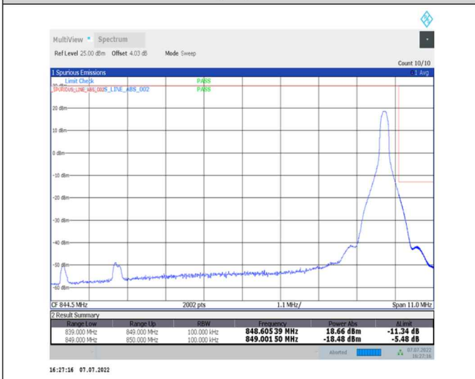
1-N26-824-849--15-10-H-5-CP-QPSK-Edge_1RB_Right-1@51-Ant0-seegraph-PASS-see graph
