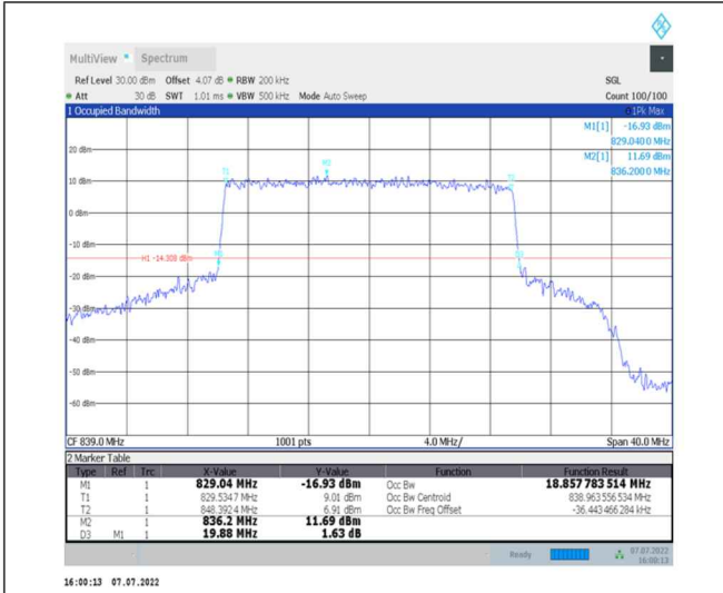
1-N26-824-849--15-20-H-6-CP-QPSK-Outer_Full-106@0-Ant0-18.858-19.880-<=20-PASS
