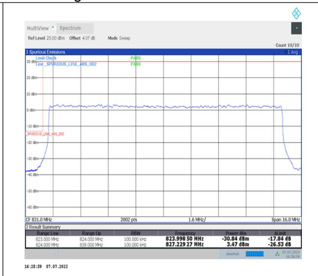
1-N26-824-849--15-15-L-3-DFT-PI2BPSK-Outer_Full-75@0-Ant0-seegraph-PASS-see graph
