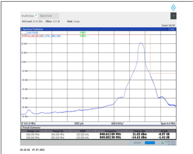
1-N26-824-849--15-5-H-2-DFT-PI2BPSK-Edge_1RB_Right-1@24-Ant0-seegraph-PASS-see graph
