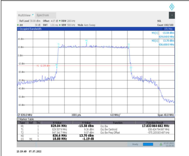
1-N26-824-849--15-20-H-4-DFT-64QAM-Outer_Full-100@0-Ant0-17.834-18.880-≤20-PASS
