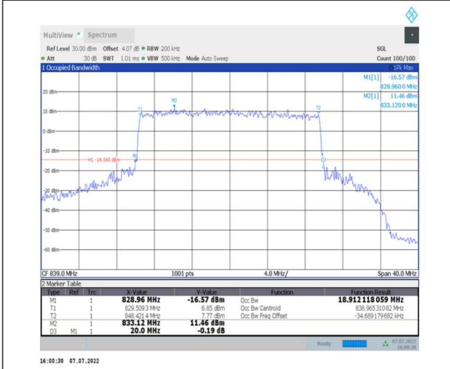
1-N26-824-849--15-20-H-8-CP-64QAM-Outer_Full-106@0-Ant0-18.912-20.000-<=20-PASS
