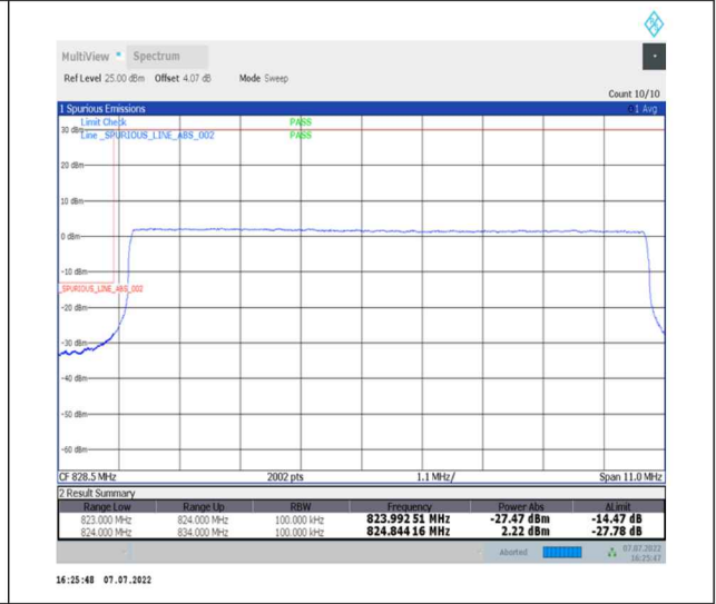
1-N26-824-849--15-10-L-6-CP-QPSK-Outer_Full-52@0-Ant0-seegraph-PASS-see graph
