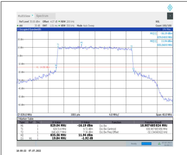
1-N26-824-849--15-20-H-2-DFT-PI2BPSK-Outer_Full-100@0-Ant0-39.671-40.000-≤20-FAIL
