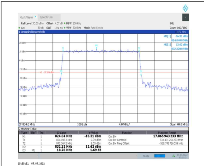
1-N26-824-849--15-20-L-4-DFT-64QAM-Outer_Full-100@0-Ant0-17.866-18.760-<20-PASS
