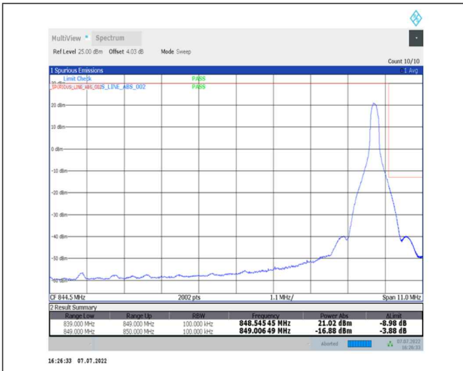
1-N26-824-849--15-10-H-2-DFT-PI2BPSK-Edge_1RB_Right-1@51-Ant0-seegraph-PASS-see graph
