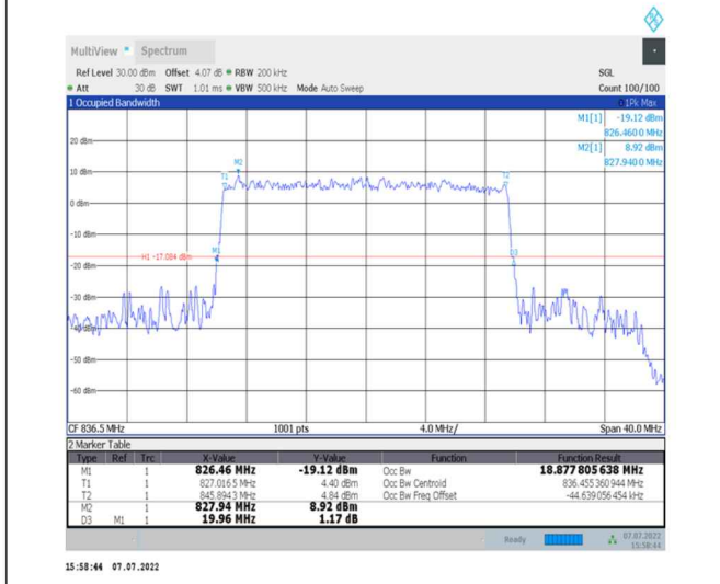
1-N26-824-849--15-20-M-9-CP-256QAM-Outer_Full-106@0-Ant0-18.878-19.960-<=20-PASS
