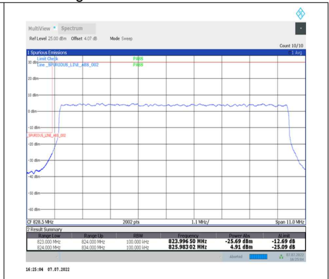
1-N26-824-849--15-10-L-3-DFT-PI2BPSK-Outer_Full-50@0-Ant0-seegraph-PASS-see graph
