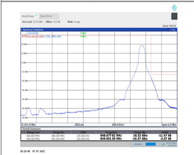
1-N26-824-849--15-5-H-5-CP-QPSK-Edge_1RB_Right-1@24-Ant0-seegraph-PASS-see graph
