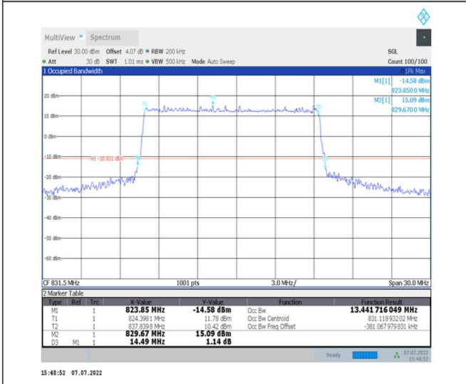
1-N26-824-849--15-15-L-1-DFT-QPSK-Outer_Full-75@0-Ant0-13.442-14.490-≤15-PASS
