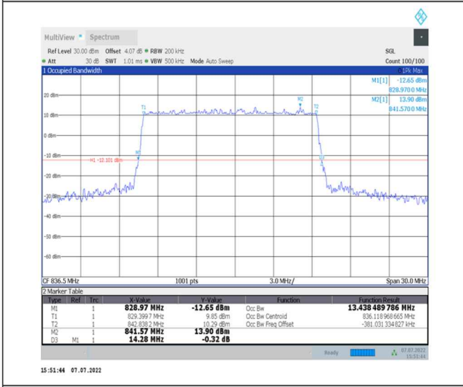
1-N26-824-849--15-15-M-4-DFT-64QAM-Outer_Full-75@0-Ant0-13.438-14.280-≤15-PASS
