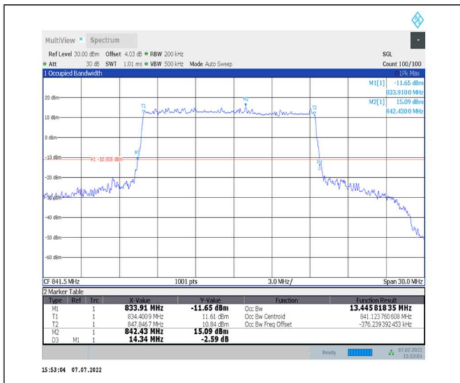
1-N26-824-849--15-15-H-1-DFT-QPSK-Outer_Full-75@0-Ant0-13.446-14.340-≤15-PASS
