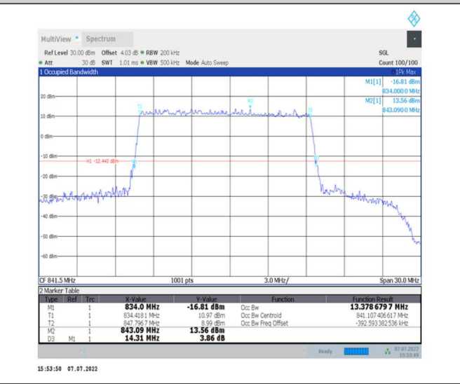
1-N26-824-849--15-15-H-4-DFT-64QAM-Outer_Full-75@0-Ant0-13.379-14.310-≤15-PASS
