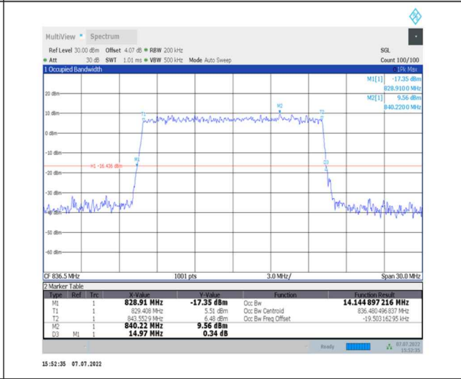
1-N26-824-849--15-15-M-9-CP-256QAM-Outer_Full-79@0-Ant0-14.145-14.970-≤15-PASS
