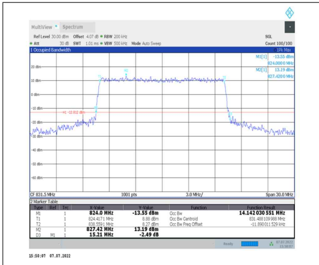
1-N26-824-849--15-15-L-7-CP-16QAM-Outer_Full-79@0-Ant0-14.142-15.210-≤15-PASS
