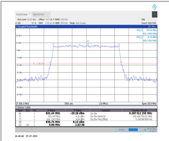
1-N26-824-849--15-10-M-9-CP-256QAM-Outer_Full-52@0-Ant0-9.288-9.980-≤10-PASS
