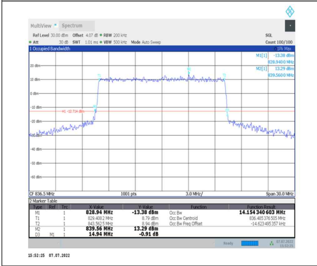
1-N26-824-849--15-15-M-8-CP-64QAM-Outer_Full-79@0-Ant0-14.154-14.940-≤15-PASS
