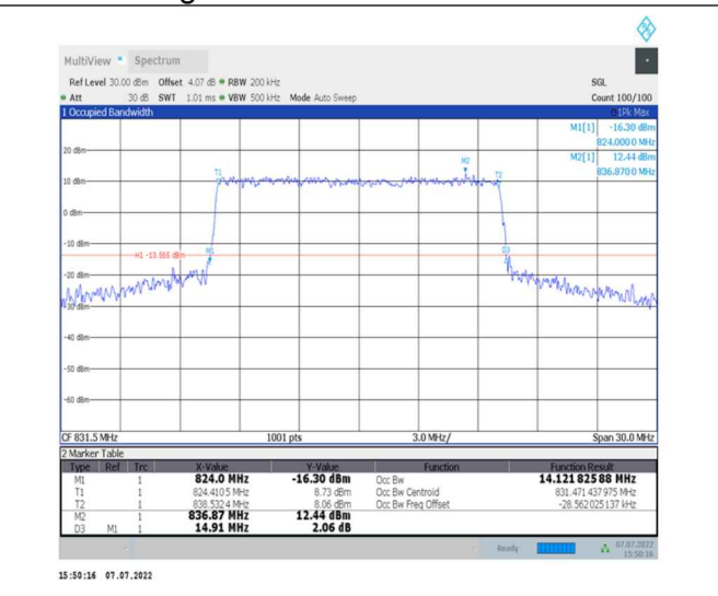
1-N26-824-849--15-15-L-8-CP-64QAM-Outer_Full-79@0-Ant0-14.122-14.910-≤15-PASS
