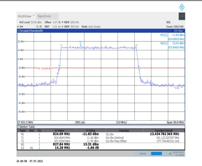
1-N26-824-849--15-15-L-2-DFT-PI2BPSK-Outer_Full-75@0-Ant0-13.435-14.280-≤15-PASS
