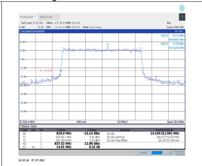
1-N26-824-849--15-15-M-7-CP-16QAM-Outer_Full-79@0-Ant0-14.105-14.910-≤15-PASS
