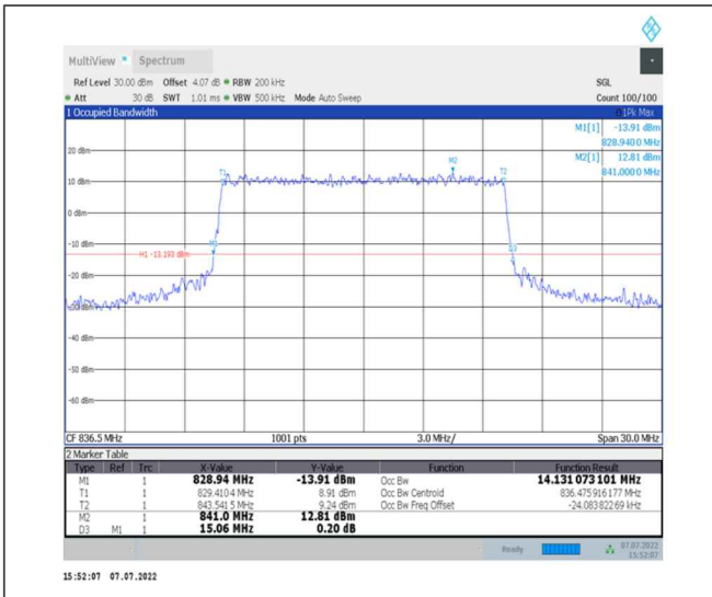
1-N26-824-849--15-15-M-6-CP-QPSK-Outer_Full-79@0-Ant0-14.131-15.060-≤15-PASS
