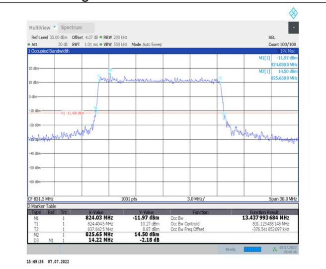
1-N26-824-849--15-15-L-4-DFT-64QAM-Outer_Full-75@0-Ant0-13.438-14.220-≤15-PASS
