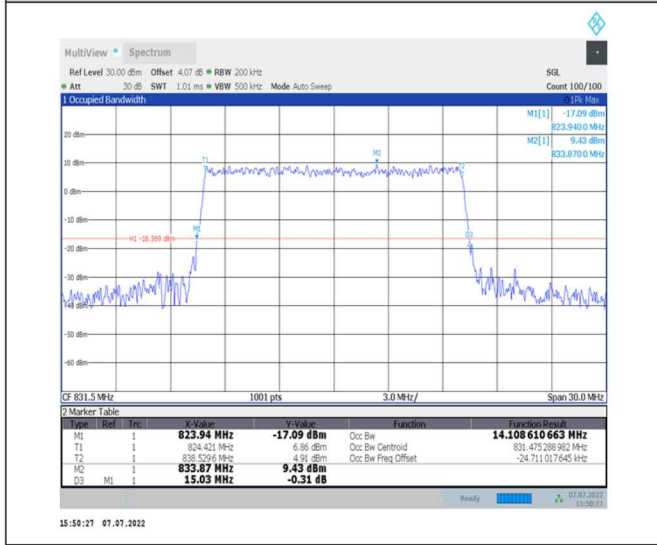
1-N26-824-849--15-15-L-9-CP-256QAM-Outer_Full-79@0-Ant0-14.109-15.030-≤15-PASS
