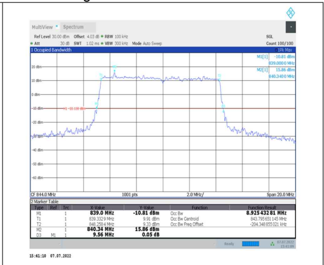
1-N26-824-849--15-10-H-1-DFT-QPSK-Outer_Full-50@0-Ant0-8.925-9.560-≤10-PASS
