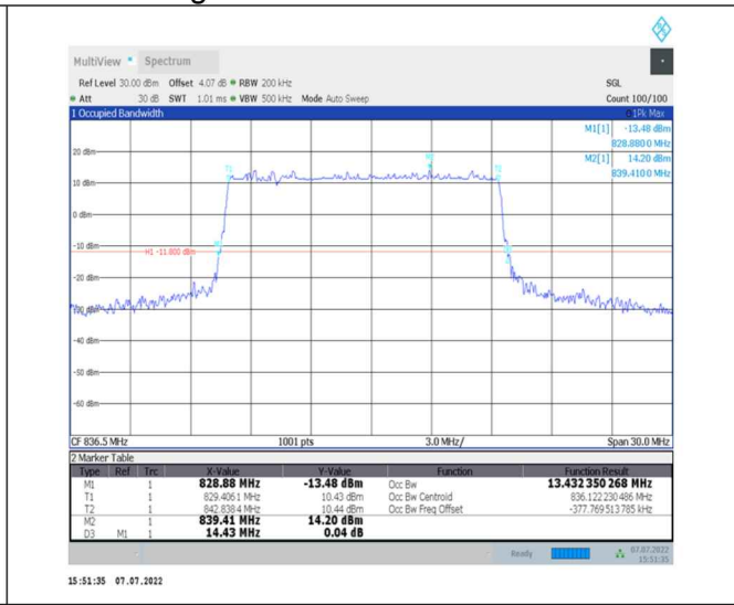
1-N26-824-849--15-15-M-3-DFT-16QAM-Outer_Full-75@0-Ant0-13.432-14.430-≤15-PASS
