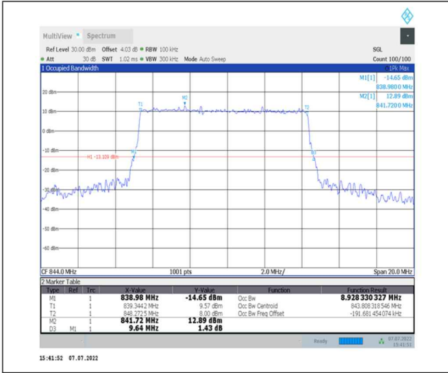
1-N26-824-849--15-10-H-4-DFT-64QAM-Outer_Full-50@0-Ant0-8.928-9.640-≤10-PASS
