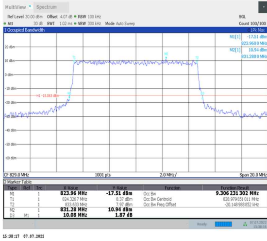
1-N26-824-849--15-10-L-6-CP-QPSK-Outer_Full-52@0-Ant0-9.306-10.080-≤10-PASS
