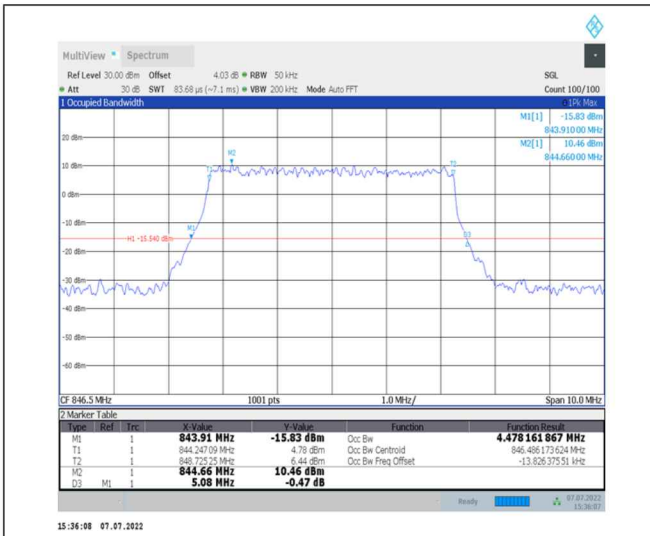
1-N26-824-849--15-5-H-7-CP-16QAM-Outer_Full-25@0-Ant0-4.478-5.080-≤5-PASS
