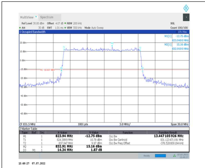
1-N26-824-849--15-15-L-3-DFT-16QAM-Outer_Full-75@0-Ant0-13.447-14.340-≤15-PASS
