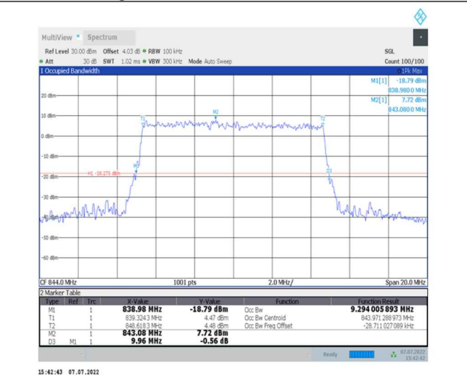
1-N26-824-849--15-10-H-9-CP-256QAM-Outer_Full-52@0-Ant0-9.294-9.960-≤10-PASS
