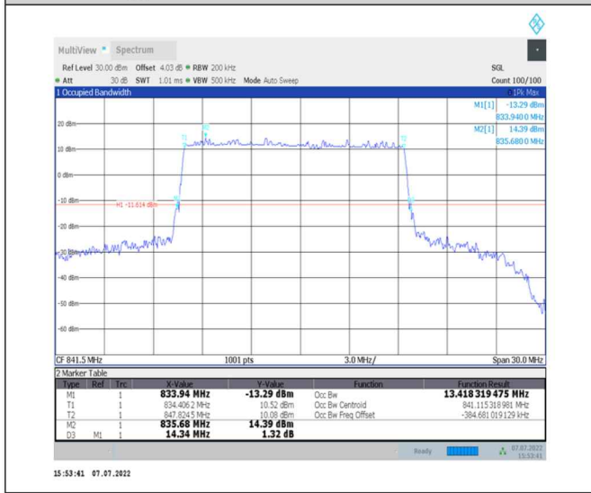
1-N26-824-849--15-15-H-3-DFT-16QAM-Outer_Full-75@0-Ant0-13.418-14.340-≤15-PASS
