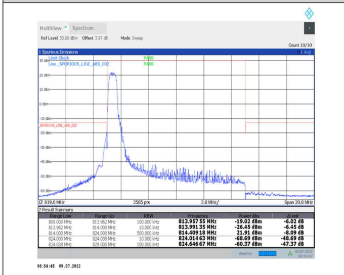
1-N26-814-824--15-10-M-4-CP-QPSK-Edge_1RB_Left-1@0-Ant0-PASS-see graph
