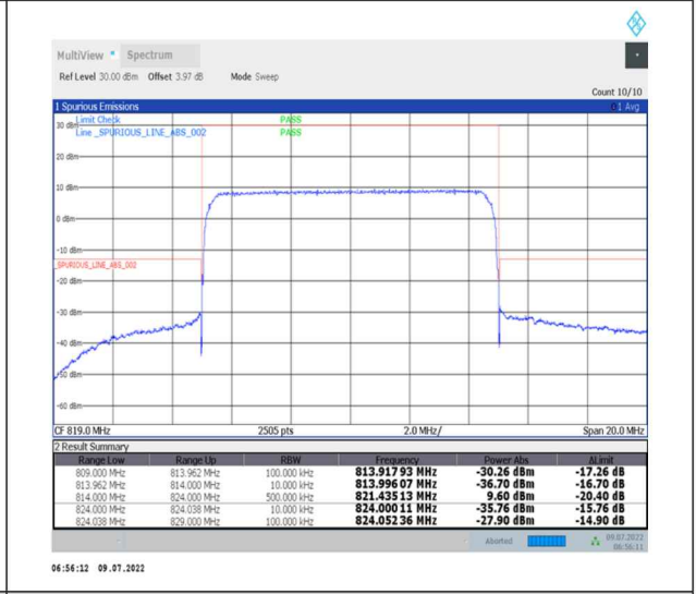
1-N26-814-824--15-10-M-6-CP-QPSK-Outer_Full-52@0-Ant0-PASS-see graph
