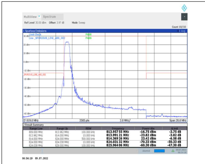
1-N26-814-824--15-10-M-1-DFT-PI2BPSK-Edge_1RB_Left-1@0-Ant0-PASS-see graph
