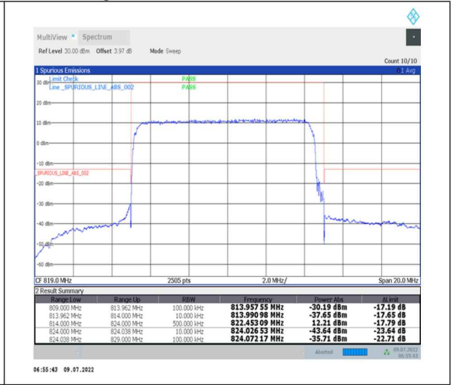
1-N26-814-824--15-10-M-3-DFT-PI2BPSK-Outer_Full-50@0-Ant0-PASS-see graph
