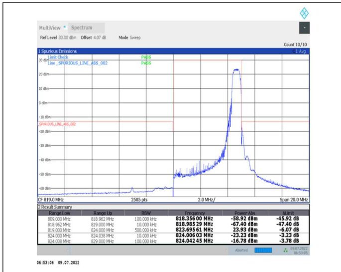
1-N26-814-824--15-5-H-2-DFT-PI2BPSK-Edge_1RB_Right-1@24-Ant0-PASS-see graph
