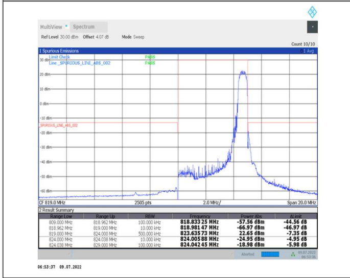
1-N26-814-824--15-5-H-5-CP-QPSK-Edge_1RB_Right-1@24-Ant0-PASS-see graph
