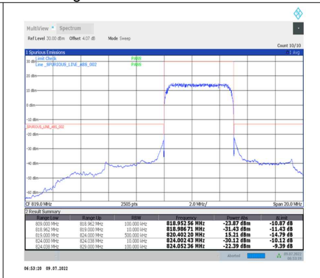
1-N26-814-824--15-5-H-3-DFT-PI2BPSK-Outer_Full-25@0-Ant0-PASS-see graph
