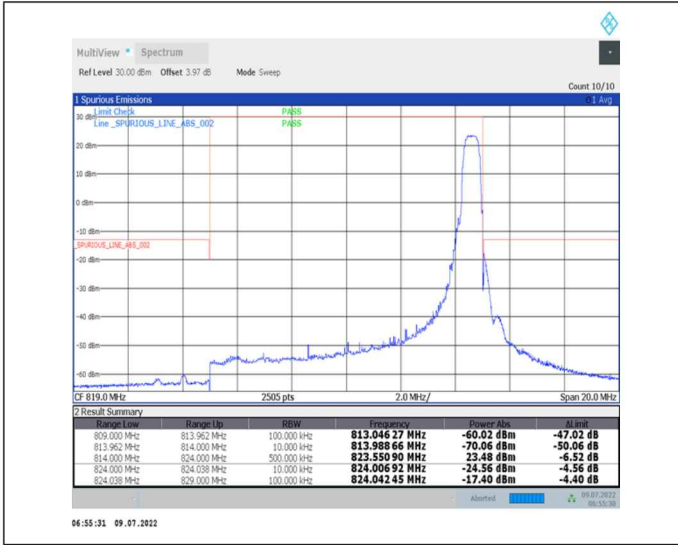
1-N26-814-824--15-10-M-2-DFT-PI2BPSK-Edge_1RB_Right-1@51-Ant0-PASS-see graph
