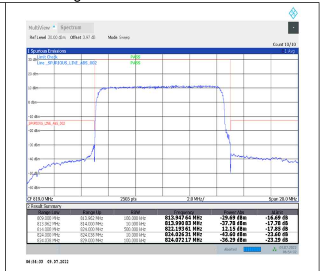
1-N26-814-824--15-10-M-3-DFT-PI2BPSK-Outer_Full-50@0-Ant0-PASS-see graph
