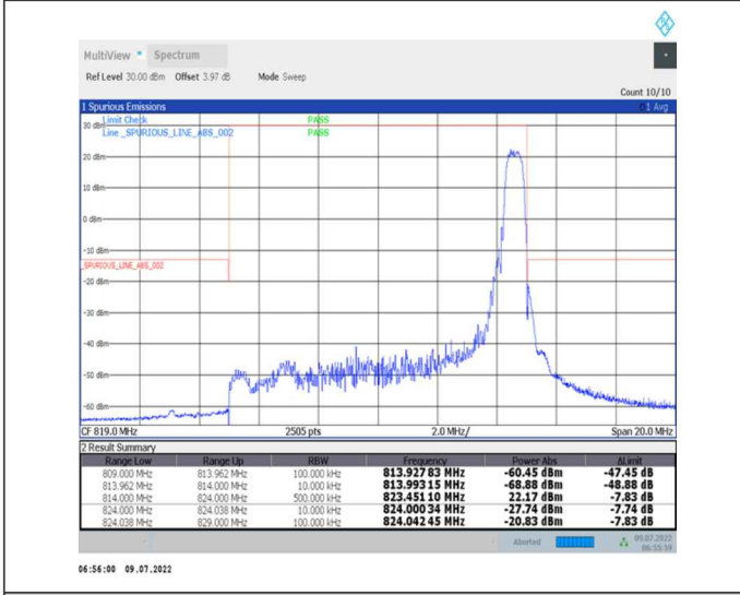
1-N26-814-824--15-10-M-5-CP-QPSK-Edge_1RB_Right-1@51-Ant0-PASS-see graph
