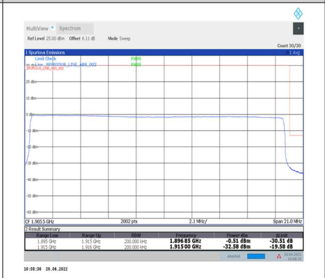
1-N25--15-20-H-6-CP-QPSK-Outer_Full-106@0-Ant0-seegraph-PASS-see graph
