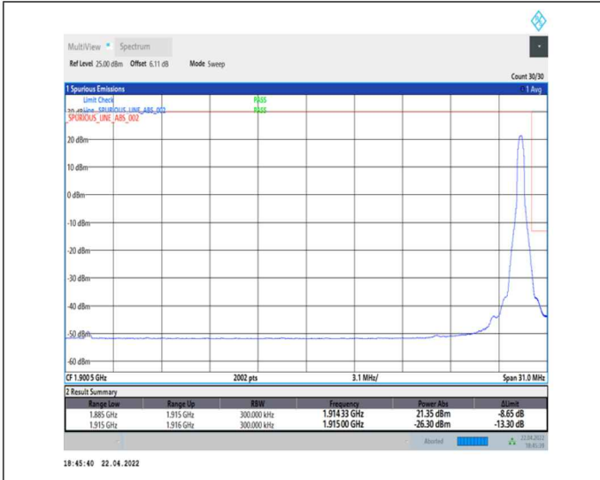
1-N25--15-30-H-2-DFT-PI2BPSK-Edge_1RB_Right-1@159-Ant0-seegraph-PASS-see graph
