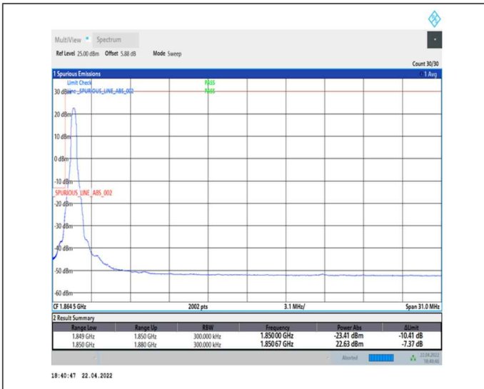
1-N25--15-30-L-1-DFT-PI2BPSK-Edge_1RB_Left-1@0-Ant0-seegraph-PASS-see graph
