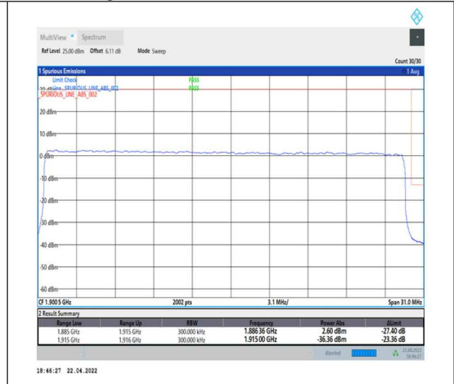
1-N25--15-30-H-3-DFT-PI2BPSK-Outer_Full-160@0-Ant0-seegraph-PASS-see graph
