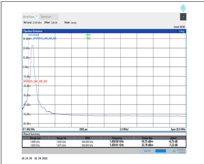
1-N25--15-25-L-1-DFT-PI2BPSK-Edge_1RB_Left-1@0-Ant0-seegraph-PASS-see graph
