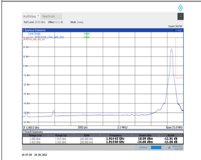
1-N25--15-20-H-5-CP-QPSK-Edge_1RB_Right-1@105-Ant0-seegraph-PASS-see graph
