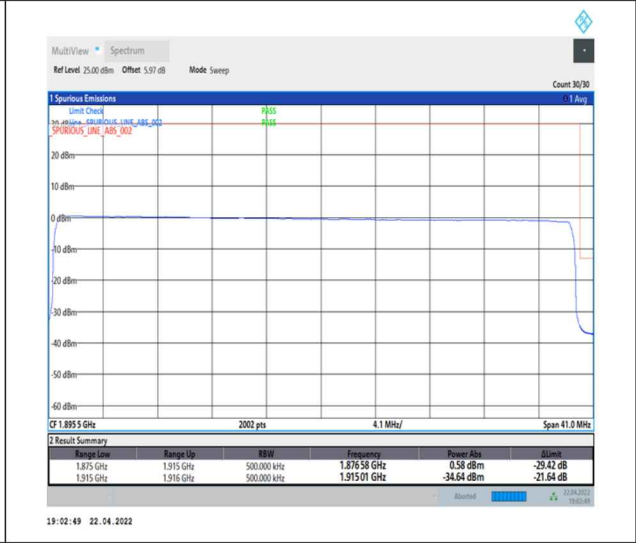
1-N25--15-40-H-6-CP-QPSK-Outer_Full-216@0-Ant0-seegraph-PASS-see graph
