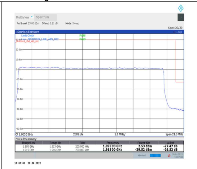
1-N25--15-20-H-3-DFT-PI2BPSK-Outer_Full-100@0-Ant0-seegraph-PASS-see graph
