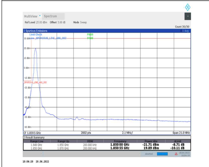
1-N25--15-20-L-4-CP-QPSK-Edge_1RB_Left-1@0-Ant0-seegraph-PASS-see graph
