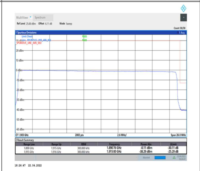
1-N25--15-25-H-6-CP-QPSK-Outer_Full-133@0-Ant0-seegraph-PASS-see graph
