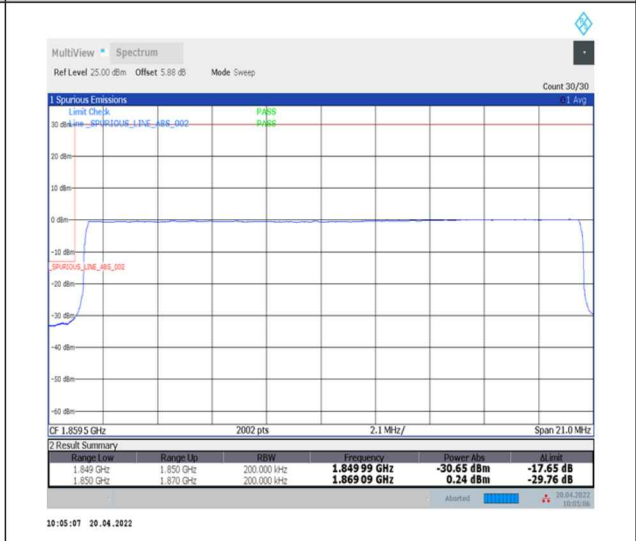
1-N25--15-20-L-6-CP-QPSK-Outer_Full-106@0-Ant0-seegraph-PASS-see graph
