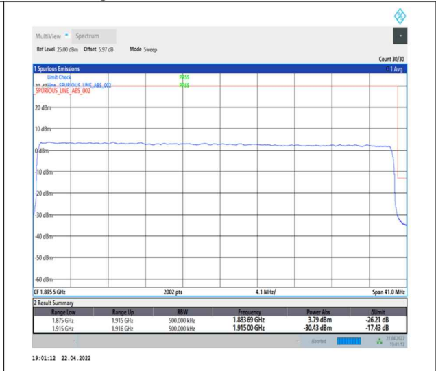
1-N25--15-40-H-3-DFT-PI2BPSK-Outer_Full-216@0-Ant0-seegraph-PASS-see graph
