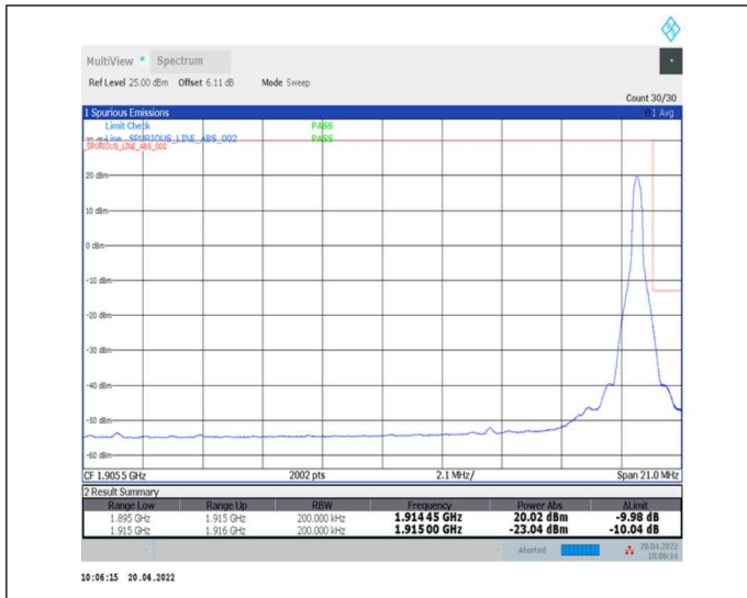
1-N25--15-20-H-2-DFT-PI2BPSK-Edge_1RB_Right-1@105-Ant0-seegraph-PASS-see graph
