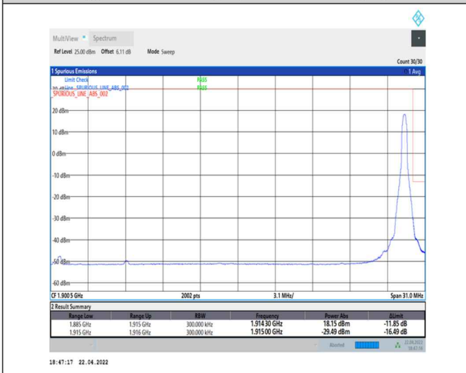
1-N25--15-30-H-5-CP-QPSK-Edge_1RB_Right-1@159-Ant0-seegraph-PASS-see graph
