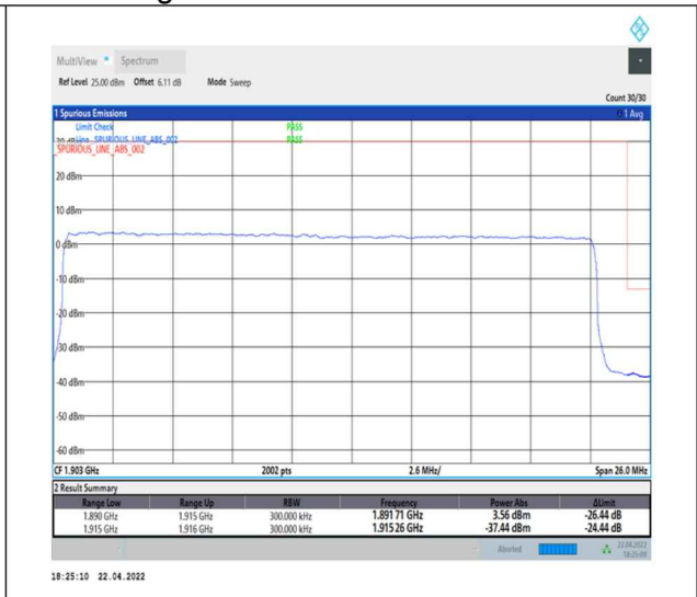
1-N25--15-25-H-3-DFT-PI2BPSK-Outer_Full-128@0-Ant0-seegraph-PASS-see graph
