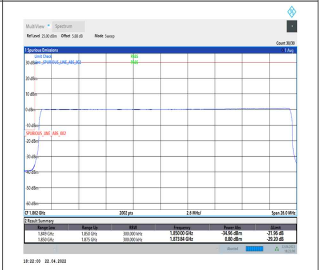
1-N25--15-25-L-6-CP-QPSK-Outer_Full-133@0-Ant0-seegraph-PASS-see graph
