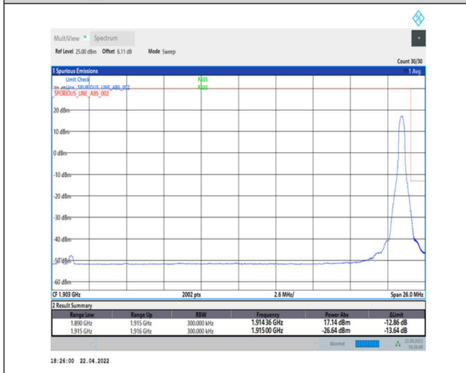
1-N25--15-25-H-5-CP-QPSK-Edge_1RB_Right-1@132-Ant0-seegraph-PASS-see graph
