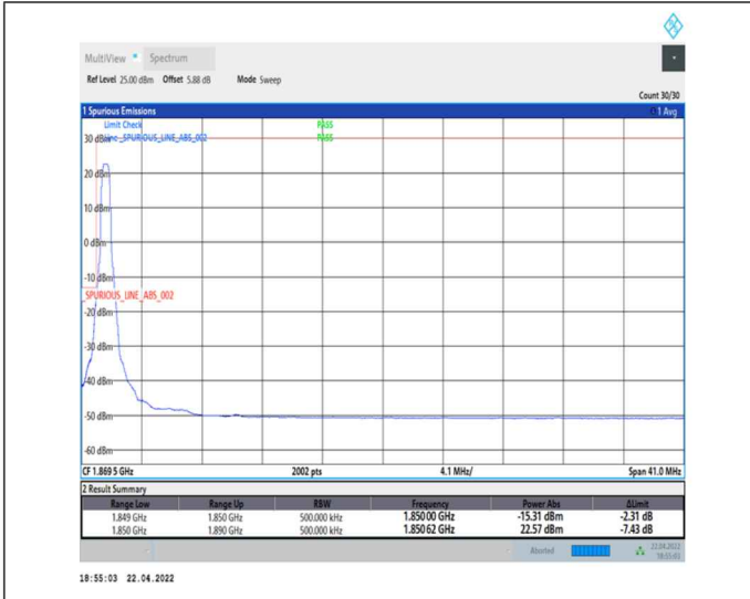
1-N25--15-40-L-1-DFT-PI2BPSK-Edge_1RB_Left-1@0-Ant0-seegraph-PASS-see graph
