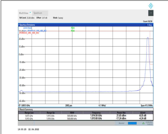
1-N25--15-40-H-2-DFT-PI2BPSK-Edge_1RB_Right-1@215-Ant0-seegraph-PASS-see graph
