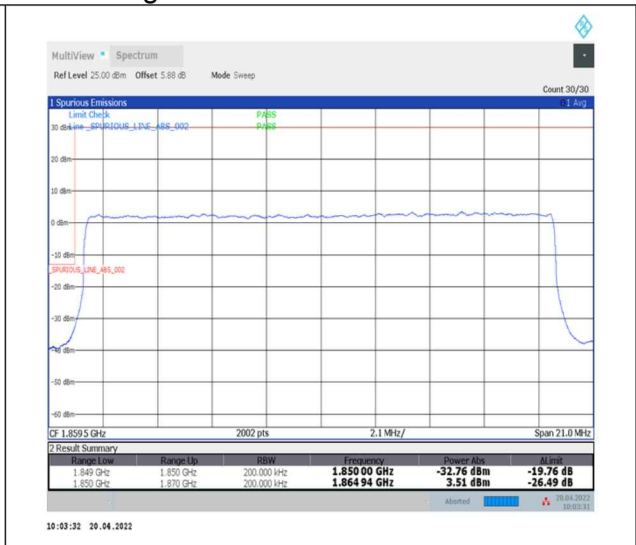
1-N25--15-20-L-3-DFT-PI2BPSK-Outer_Full-100@0-Ant0-seegraph-PASS-see graph
