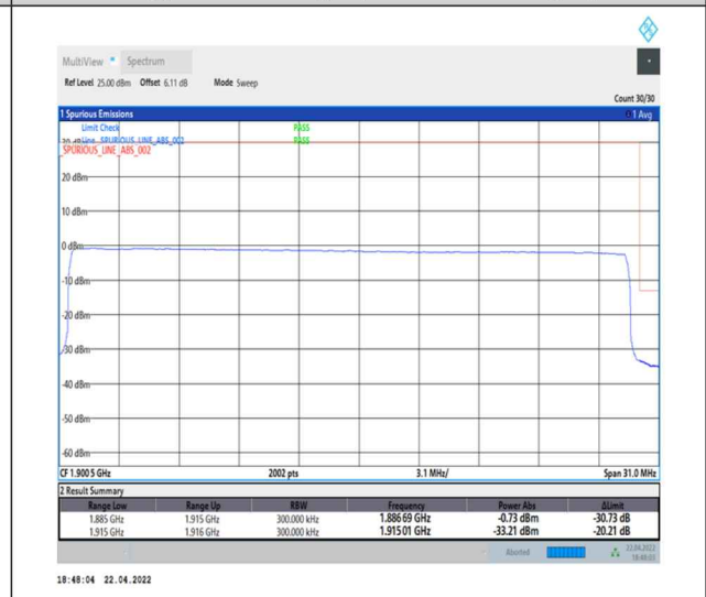
1-N25--15-30-H-6-CP-QPSK-Outer_Full-160@0-Ant0-seegraph-PASS-see graph
