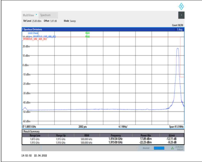
1-N25--15-40-H-5-CP-QPSK-Edge_1RB_Right-1@215-Ant0-seegraph-PASS-see graph
