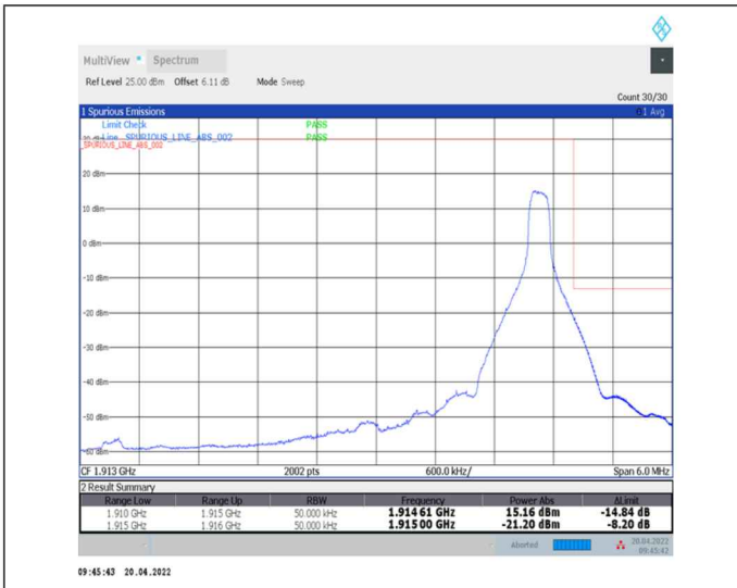
1-N25--15-5-H-2-DFT-PI2BPSK-Edge_1RB_Right-1@24-Ant0-seegraph-PASS-see graph
