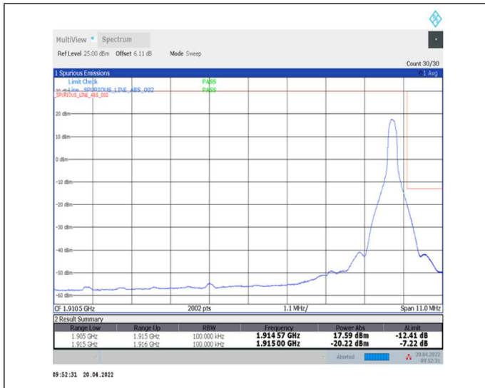
1-N25--15-10-H-2-DFT-PI2BPSK-Edge_1RB_Right-1@51-Ant0-seegraph-PASS-see graph
