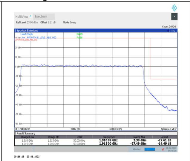
1-N25--15-5-H-3-DFT-PI2BPSK-Outer_Full-25@0-Ant0-seegraph-PASS-see graph
