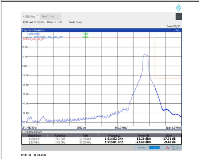
1-N25--15-5-H-5-CP-QPSK-Edge_1RB_Right-1@24-Ant0-seegraph-PASS-see graph
