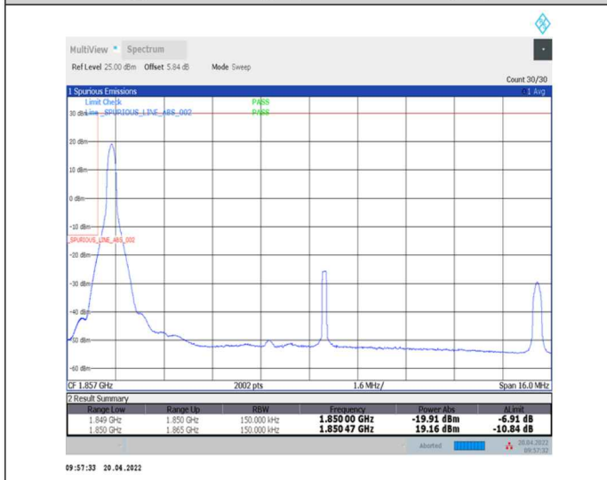
1-N25--15-15-L-4-CP-QPSK-Edge_1RB_Left-1@0-Ant0-seegraph-PASS-see graph
