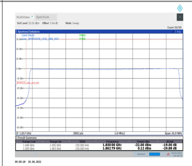
1-N25--15-15-L-6-CP-QPSK-Outer_Full-79@0-Ant0-seegraph-PASS-see graph
