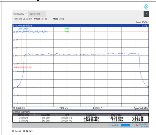
1-N25--15-15-L-3-DFT-PI2BPSK-Outer_Full-75@0-Ant0-seegraph-PASS-see graph
