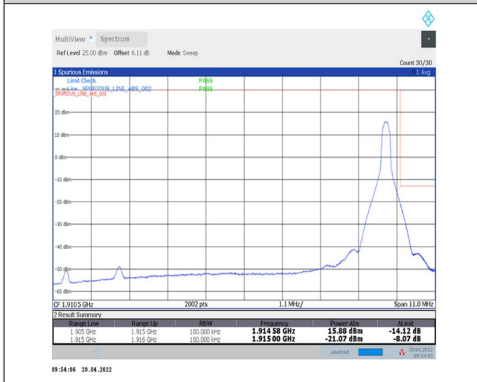
1-N25--15-10-H-5-CP-QPSK-Edge_1RB_Right-1@51-Ant0-seegraph-PASS-see graph
