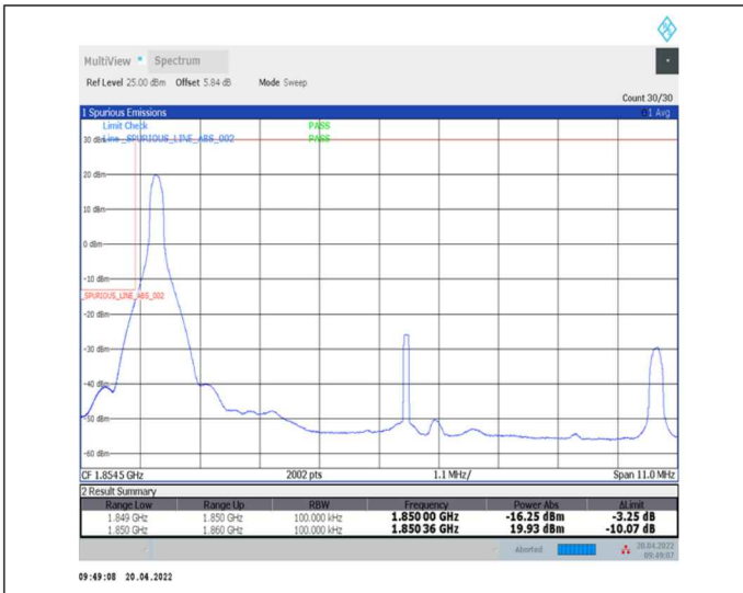
1-N25--15-10-L-1-DFT-PI2BPSK-Edge_1RB_Left-1@0-Ant0-seegraph-PASS-see graph
