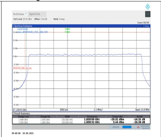
1-N25--15-10-L-3-DFT-PI2BPSK-Outer_Full-50@0-Ant0-seegraph-PASS-see graph
