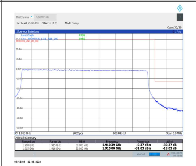
1-N25--15-5-H-6-CP-QPSK-Outer_Full-25@0-Ant0-seegraph-PASS-see graph
