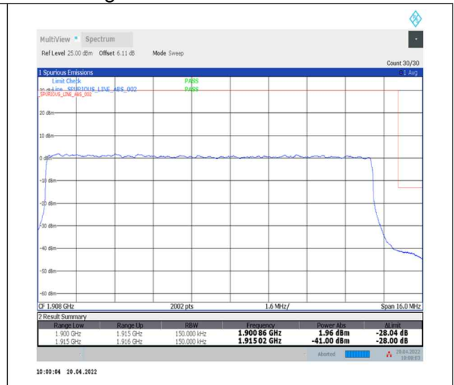
1-N25--15-15-H-3-DFT-PI2BPSK-Outer_Full-75@0-Ant0-seegraph-PASS-see graph
