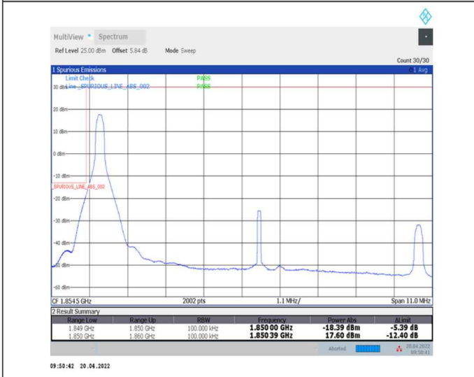
1-N25--15-10-L-4-CP-QPSK-Edge_1RB_Left-1@0-Ant0-seegraph-PASS-see graph
