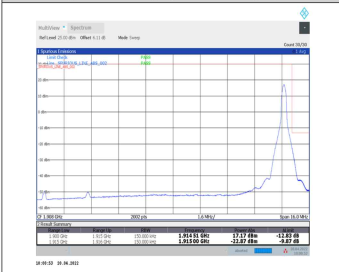
1-N25--15-15-H-5-CP-QPSK-Edge_1RB_Right-1@78-Ant0-seegraph-PASS-see graph
