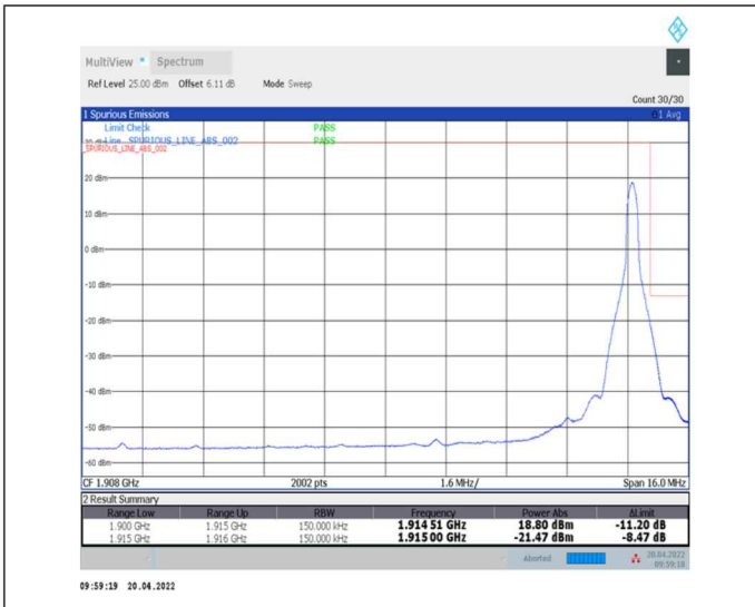
1-N25--15-15-H-2-DFT-PI2BPSK-Edge_1RB_Right-1@78-Ant0-seegraph-PASS-see graph
