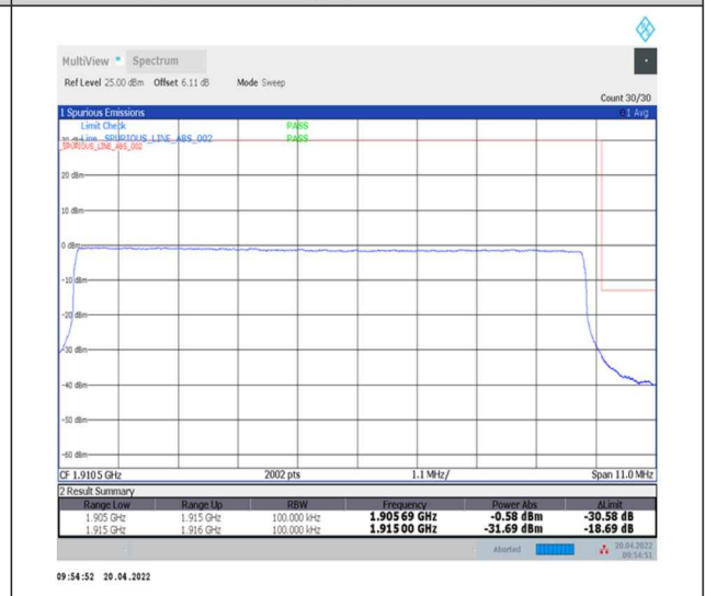
1-N25--15-10-H-6-CP-QPSK-Outer_Full-52@0-Ant0-seegraph-PASS-see graph
