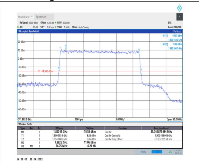
1-N25--15-25-H-8-CP-64QAM-Outer_Full-133@0-Ant0-23.745-24.750-≤25-PASS
