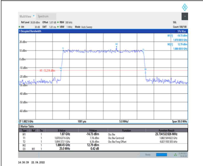
1-N25--15-25-M-6-CP-QPSK-Outer_Full-133@0-Ant0-23.735-25.000-<25-PASS
