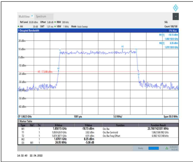
1-N25--15-25-L-9-CP-256QAM-Outer_Full-133@0-Ant0-23.76-24.950-<math>\leq 25</math>-PASS
