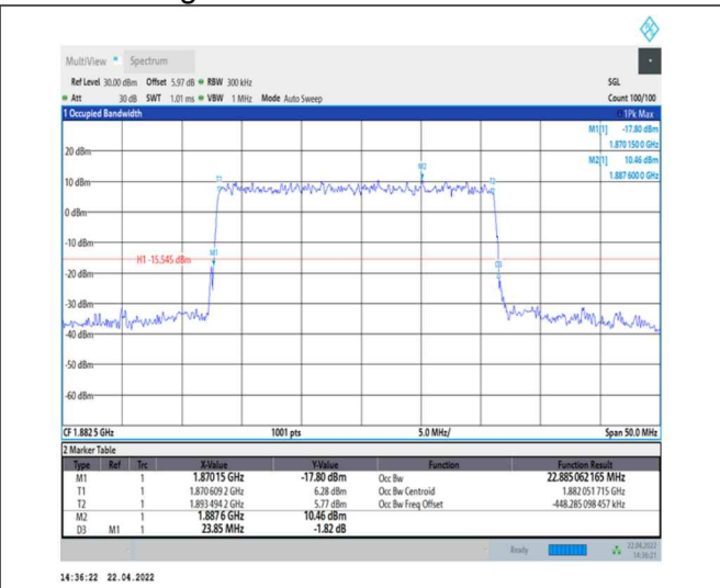
1-N25--15-25-M-5-DFT-256QAM-Outer_Full-128@0-Ant0-22.885-23.850-<25-PASS
