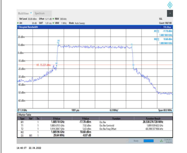
1-N25--15-30-H-6-CP-QPSK-Outer_Full-160@0-Ant0-28.538-29.640-≤30-PASS
