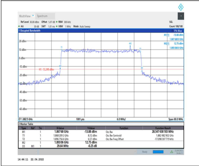
1-N25--15-30-M-7-CP-16QAM-Outer_Full-160@0-Ant0-28.547-29.640-≤30-PASS
