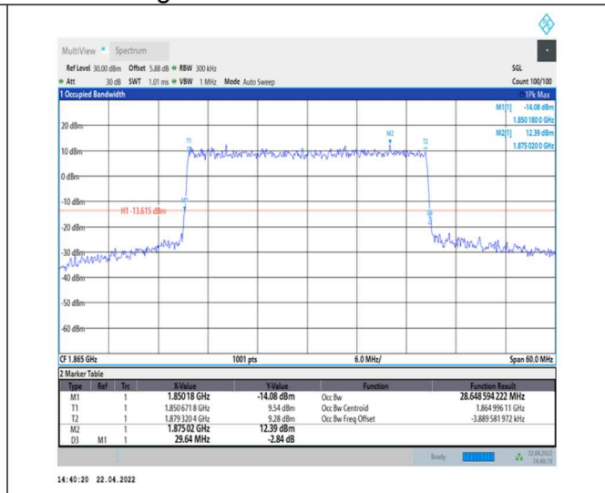
1-N25--15-30-L-3-DFT-16QAM-Outer_Full-160@0-Ant0-28.649-29.640-≤30-PASS
