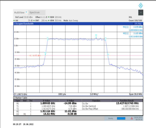
1-N25--15-15-H-4-DFT-64QAM-Outer_Full-75@0-Ant0-13.427-14.520-≤15-PASS
