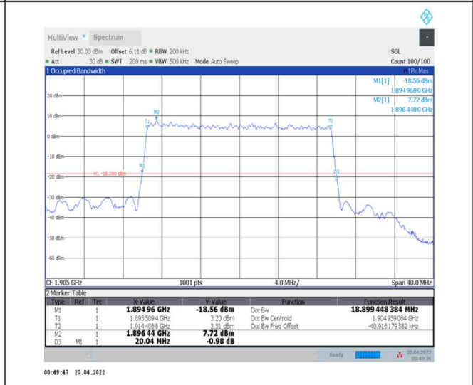
1-N25--15-20-H-9-CP-256QAM-Outer_Full-106@0-Ant0-18.899-20.040-<=20-PASS
