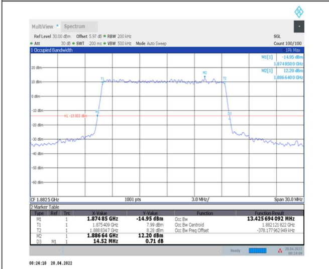
1-N25--15-15-M-4-DFT-64QAM-Outer_Full-75@0-Ant0-13.426-14.520-≤15-PASS
