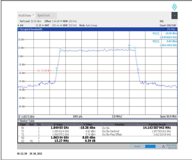
1-N25--15-15-L-9-CP-256QAM-Outer_Full-79@0-Ant0-14.144-15.270-≤15-PASS
