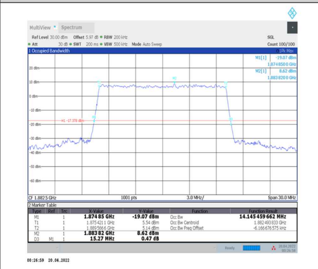
1-N25--15-15-M-9-CP-256QAM-Outer_Full-79@0-Ant0-14.145-15.270-≤15-PASS
