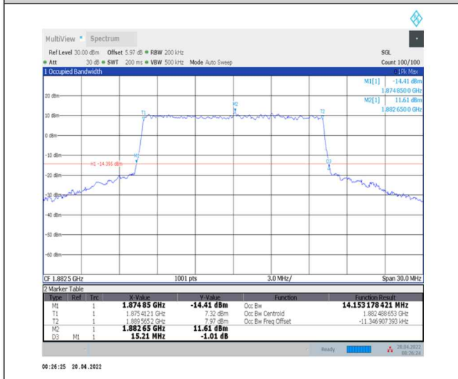
1-N25--15-15-M-8-CP-64QAM-Outer_Full-79@0-Ant0-14.153-15.210-≤15-PASS
