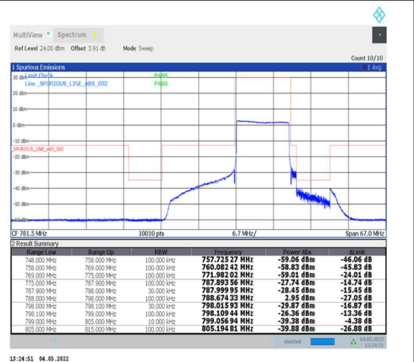
1-N14--15-10-H-6-CP-QPSK-Outer_Full-52@0-Ant0-PASS-see graph
