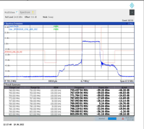
1-N14--15-10-H-3-DFT-PI2BPSK-Outer_Full-50@0-Ant0-PASS-see graph
