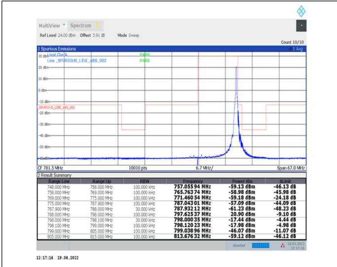
1-N14--15-10-H-2-DFT-PI2BPSK-Edge_1RB_Right-1@51-Ant0-PASS-see graph
