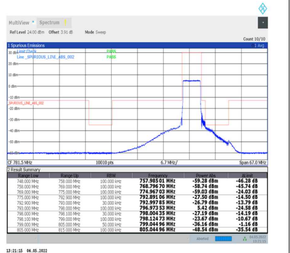
1-N14--15-5-H-6-CP-QPSK-Outer_Full-25@0-Ant0-PASS-see graph
