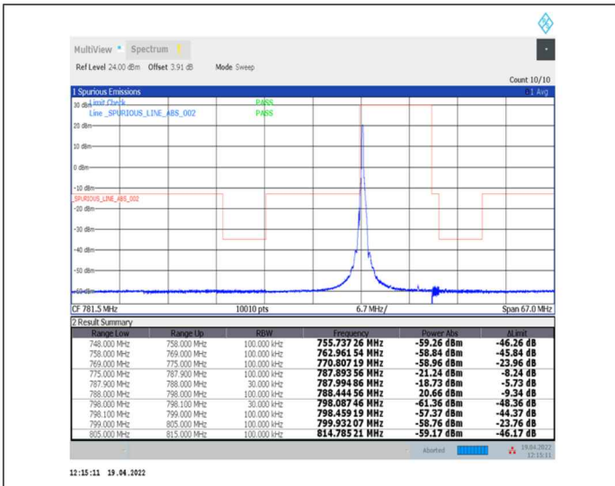
1-N14--15-10-L-1-DFT-PI2BPSK-Edge_1RB_Left-1@0-Ant0-PASS-see graph
