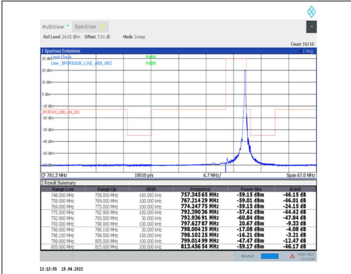
1-N14--15-5-H-2-DFT-PI2BPSK-Edge_1RB_Right-1@24-Ant0-PASS-see graph
