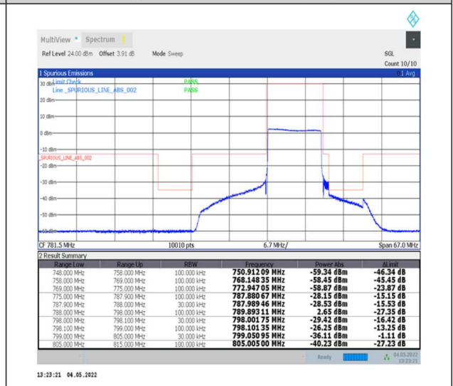
1-N14--15-10-L-6-CP-QPSK-Outer_Full-52@0-Ant0-PASS-see graph
