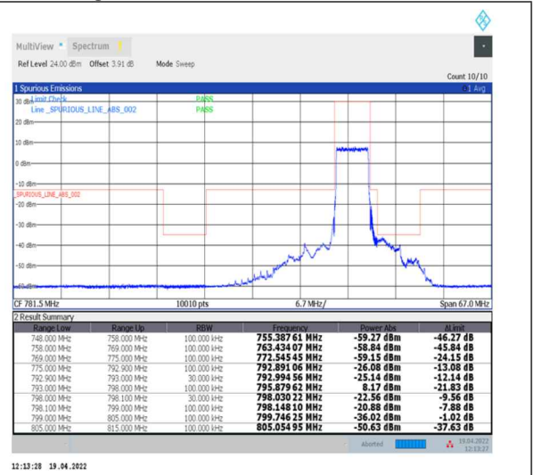
1-N14--15-5-H-3-DFT-PI2BPSK-Outer_Full-25@0-Ant0-PASS-see graph
