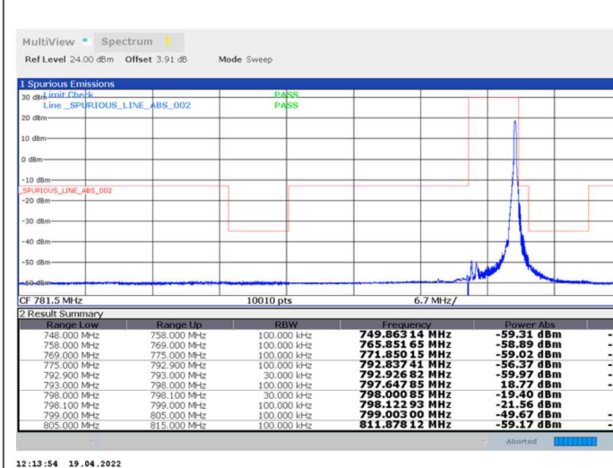
1-N14--15-5-H-5-CP-QPSK-Edge_1RB_Right-1@24-Ant0-PASS-see graph
