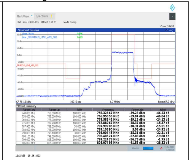
1-N14--15-10-L-3-DFT-PI2BPSK-Outer_Full-50@0-Ant0-PASS-see graph
