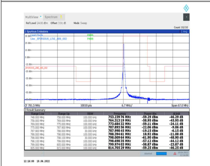
1-N14--15-10-L-4-CP-QPSK-Edge_1RB_Left-1@0-Ant0-PASS-see graph
