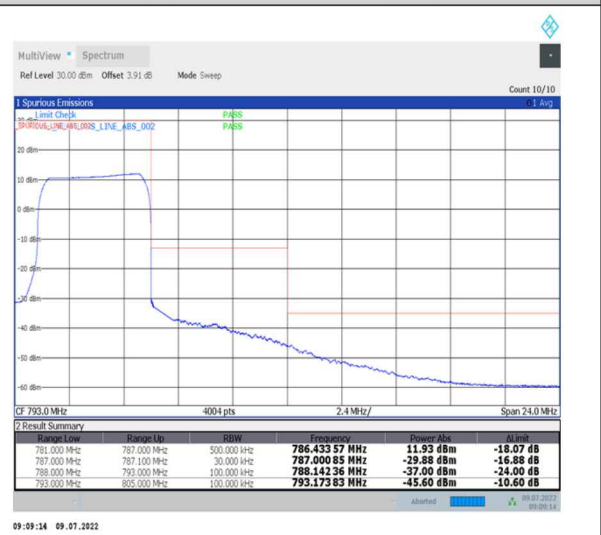
1-N13-PC3-15-5-H-6-CP-QPSK-Outer_Full-25@0-Ant0-PASS-see graph
