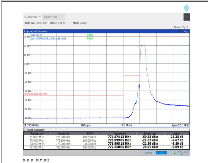
1-N13-PC3-15-10-L-4-CP-QPSK-Edge_1RB_Left-1@0-Ant0-PASS-see graph
