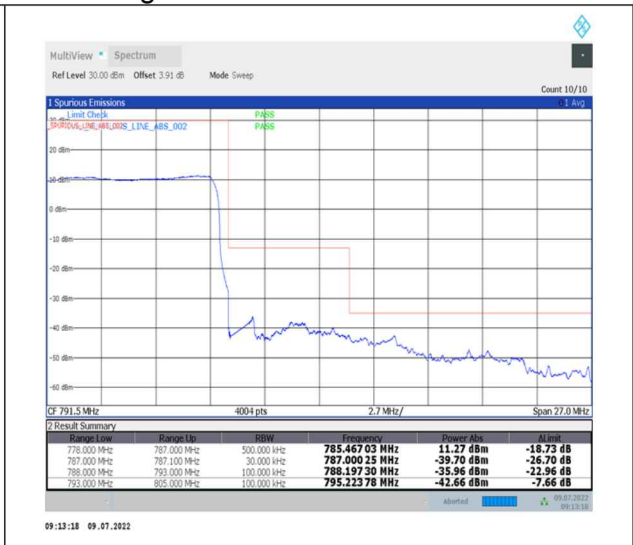
1-N13-PC3-15-10-H-3-DFT-PI2BPSK-Outer_Full-50@0-Ant0-PASS-see graph
