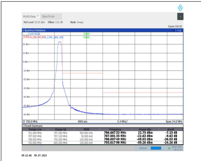
1-N13-PC3-15-10-H-2-DFT-PI2BPSK-Edge_1RB_Right-1@51-Ant0-PASS-see graph
