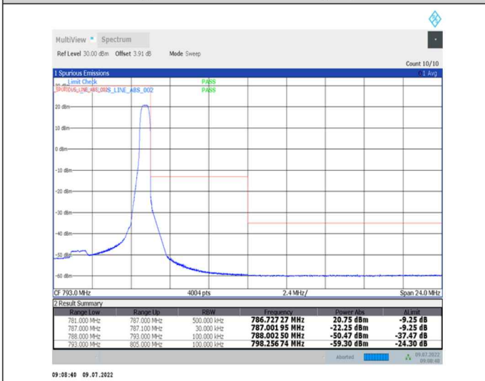
1-N13-PC3-15-5-H-5-CP-QPSK-Edge_1RB_Right-1@24-Ant0-PASS-see graph
