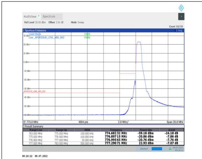
1-N13-PC3-15-10-L-1-DFT-PI2BPSK-Edge_1RB_Left-1@0-Ant0-PASS-see graph
