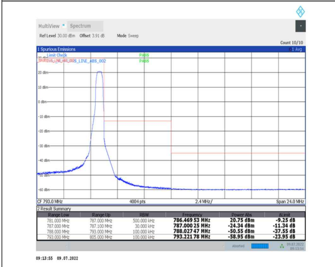
1-N13-PC3-15-10-H-5-CP-QPSK-Edge_1RB_Right-1@51-Ant0-PASS-see graph
