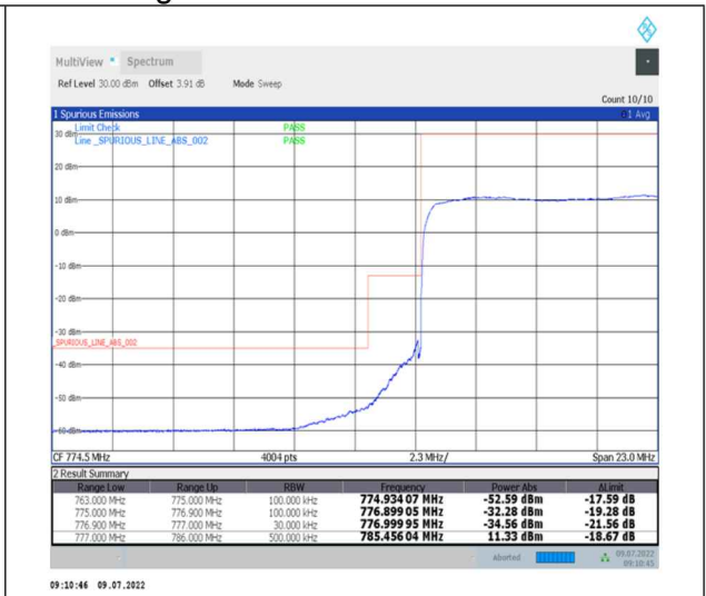
1-N13-PC3-15-10-L-3-DFT-PI2BPSK-Outer_Full-50@0-Ant0-PASS-see graph
