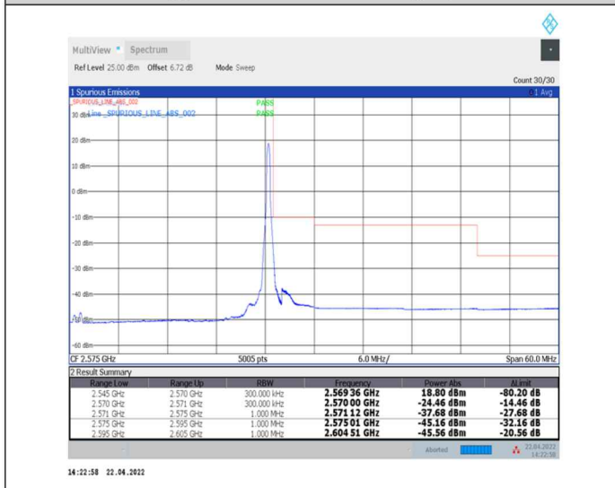
1-N7--15-25-H-5-CP-QPSK-Edge_1RB_Right-1@132-Ant0-PASS-see graph
