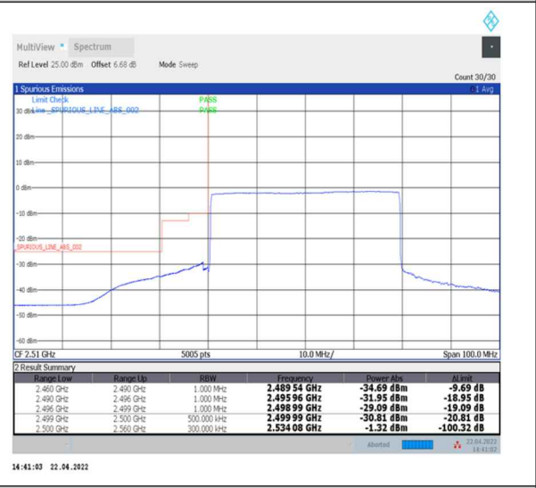
1-N7--15-40-L-6-CP-QPSK-Outer_Full-216@0-Ant0-PASS-see graph
