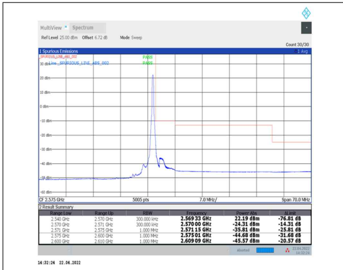
1-N7--15-30-H-2-DFT-PI2BPSK-Edge_1RB_Right-1@159-Ant0-PASS-see graph
