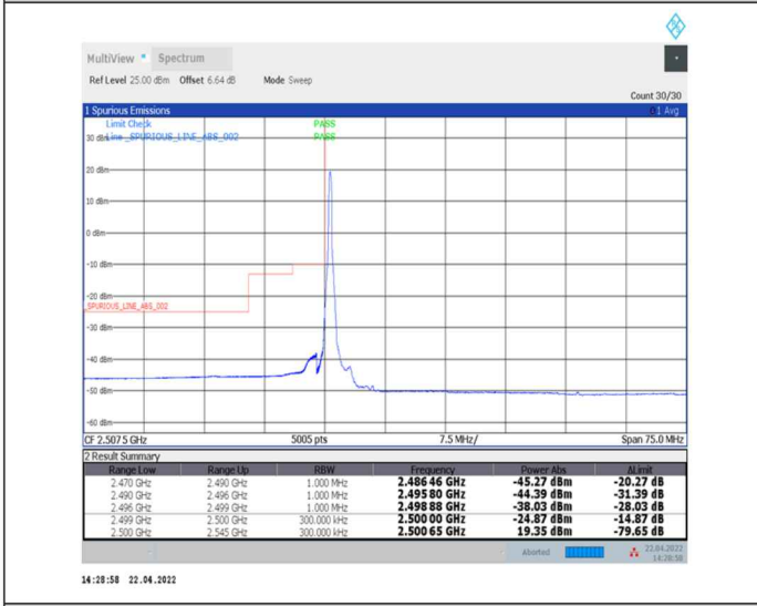
1-N7--15-30-L-4-CP-QPSK-Edge_1RB_Left-1@0-Ant0-PASS-see graph
