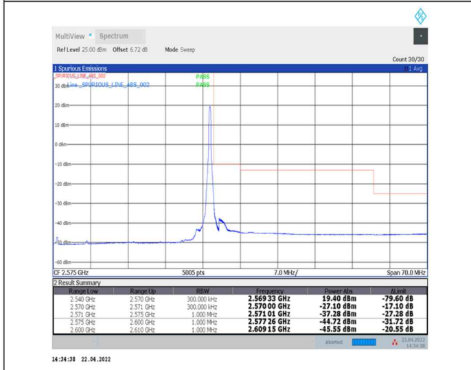
1-N7--15-30-H-5-CP-QPSK-Edge_1RB_Right-1@159-Ant0-PASS-see graph
