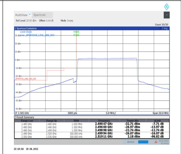
1-N7--15-20-L-6-CP-QPSK-Outer_Full-106@0-Ant0-PASS-see graph
