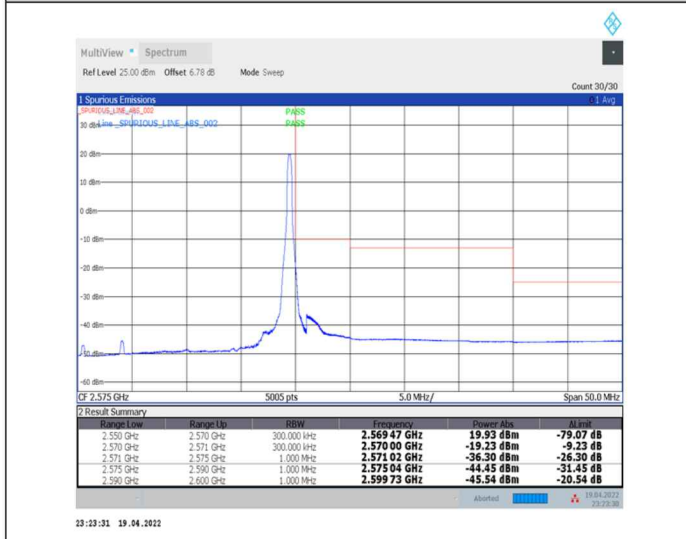
1-N7--15-20-H-5-CP-QPSK-Edge_1RB_Right-1@105-Ant0-PASS-see graph
