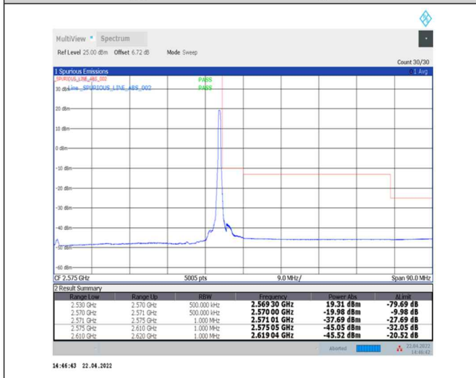
1-N7--15-40-H-5-CP-QPSK-Edge_1RB_Right-1@215-Ant0-PASS-see graph
