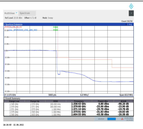
1-N7--15-25-H-6-CP-QPSK-Outer_Full-133@0-Ant0-PASS-see graph
