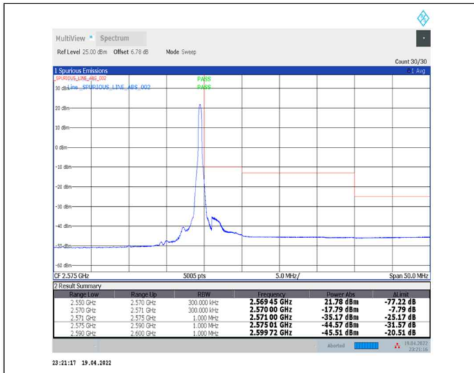
1-N7--15-20-H-2-DFT-PI2BPSK-Edge_1RB_Right-1@105-Ant0-PASS-see graph
