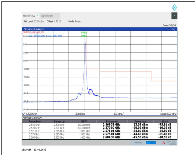
1-N7--15-25-H-2-DFT-PI2BPSK-Edge_1RB_Right-1@132-Ant0-PASS-see graph
