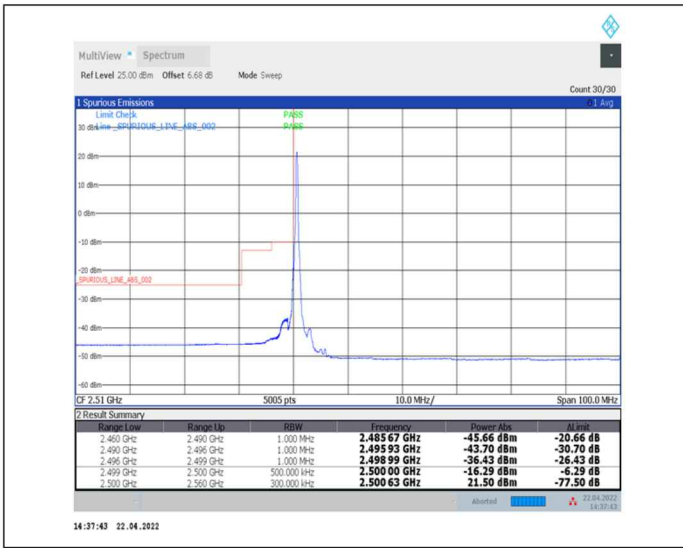
1-N7--15-40-L-1-DFT-PI2BPSK-Edge_1RB_Left-1@0-Ant0-PASS-see graph
