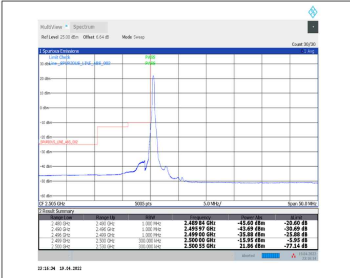
1-N7--15-20-L-1-DFT-PI2BPSK-Edge_1RB_Left-1@0-Ant0-PASS-see graph
