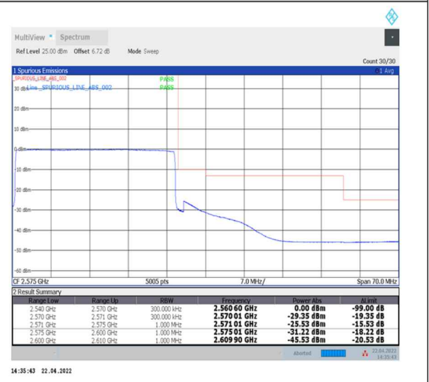
1-N7--15-30-H-6-CP-QPSK-Outer_Full-160@0-Ant0-PASS-see graph
