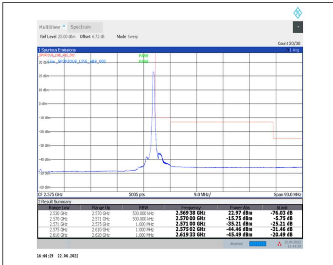
1-N7--15-40-H-2-DFT-PI2BPSK-Edge_1RB_Right-1@215-Ant0-PASS-see graph
