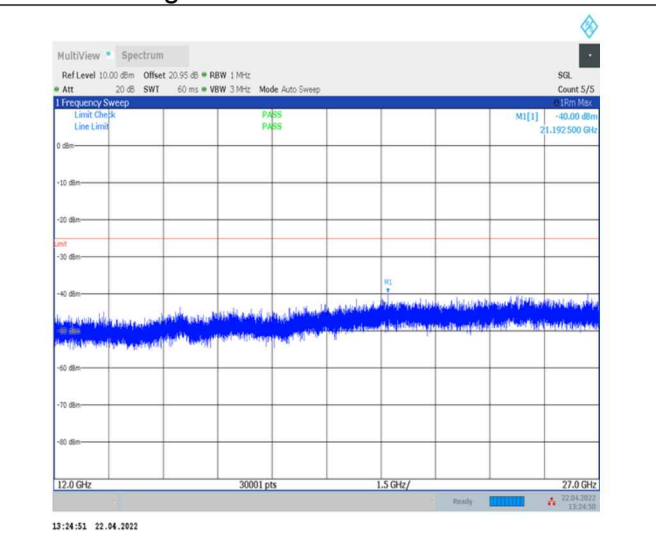
1-N7--15-40-H-1-DFT-PI2BPSK-Inner_1RB_Left- 1@1-12000-27000-Ant0--40.00--25-PASS
