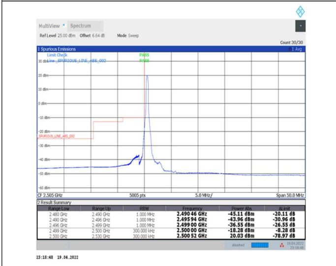
1-N7--15-20-L-4-CP-QPSK-Edge_1RB_Left-1@0-Ant0-PASS-see graph
