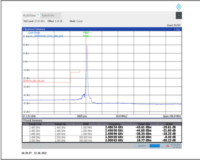
1-N7--15-40-L-4-CP-QPSK-Edge_1RB_Left-1@0-Ant0-PASS-see graph
