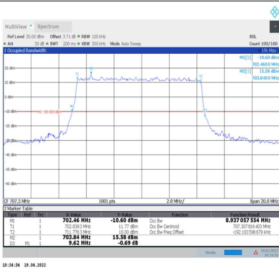
1-N12--15-10-M-1-DFT-QPSK-Outer_Full-50@0-Ant0-8.937-9.620-≤10-PASS
