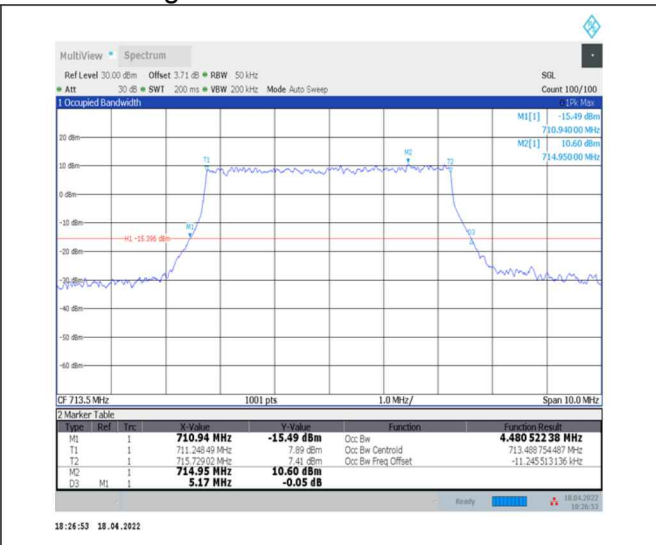
1-N12--15-5-H-8-CP-64QAM-Outer_Full-25@0-Ant0-4.481-5.170-≤5-PASS
