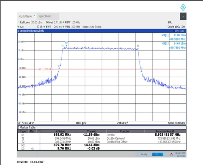
1-N12--15-10-L-3-DFT-16QAM-Outer_Full-50@0-Ant0-8.928-9.760-≤10-PASS
