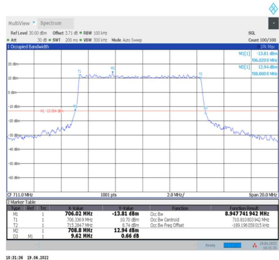
1-N12--15-10-H-3-DFT-16QAM-Outer_Full-50@0-Ant0-8.948-9.620-≤10-PASS
