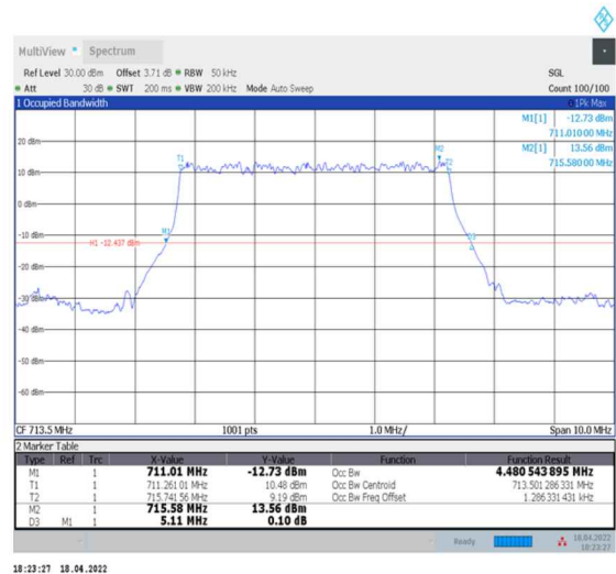
1-N12--15-5-H-2-DFT-PI2BPSK-Outer_Full-25@0-Ant0-4.481-5.110-<math>\leq</math>5-PASS
