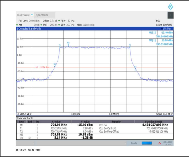
1-N12--15-5-M-7-CP-16QAM-Outer_Full-25@0-Ant0-4.474-5.140-<math>\leq</math>5-PASS
