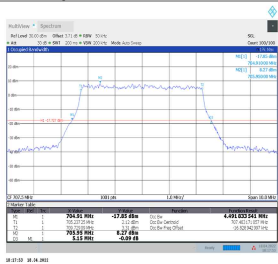
1-N12--15-5-M-9-CP-256QAM-Outer_Full-25@0-Ant0-4.492-5.150-<math>\leq</math>5-PASS
