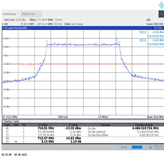
1-N12--15-5-H-1-DFT-QPSK-Outer_Full-25@0-Ant0-4.486-5.130-<math>\leq</math>5-PASS
