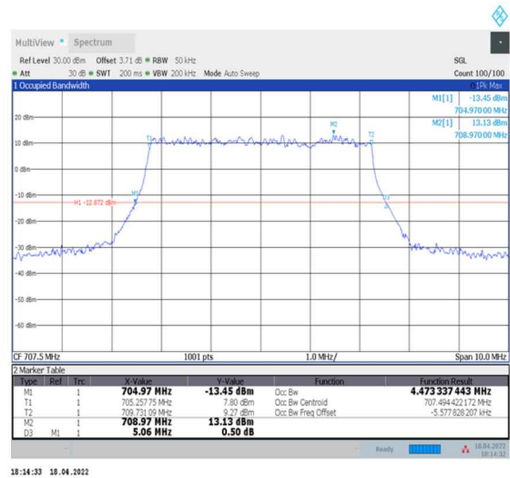
1-N12--15-5-M-3-DFT-16QAM-Outer_Full-25@0-Ant0-4.473-5.060-≤5-PASS
