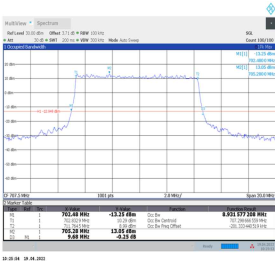
1-N12--15-10-M-3-DFT-16QAM-Outer_Full-50@0-Ant0-8.932-9.680-≤10-PASS
