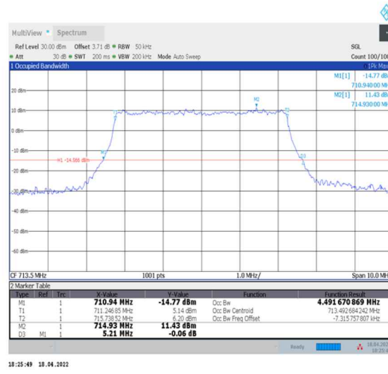
1-N12--15-5-H-6-CP-QPSK-Outer_Full-25@0-Ant0-4.492-5.210-≤5-PASS
