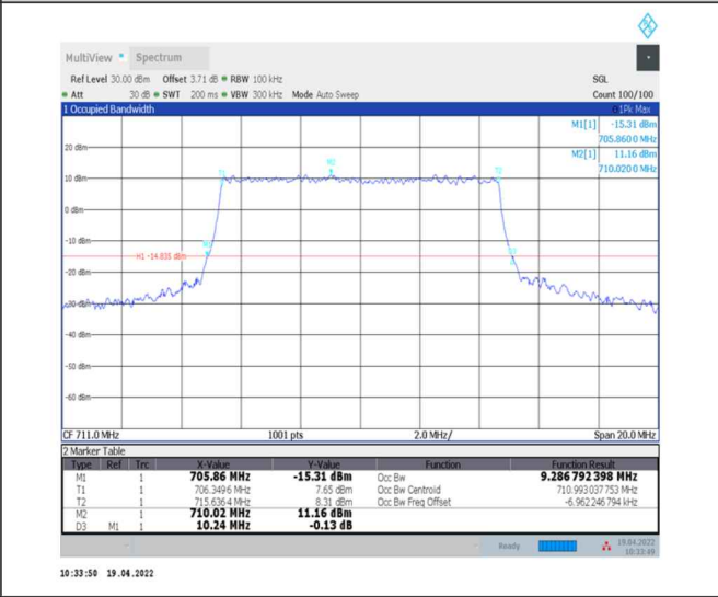
1-N12--15-10-H-7-CP-16QAM-Outer_Full-52@0-Ant0-9.287-10.240-≤10-PASS
