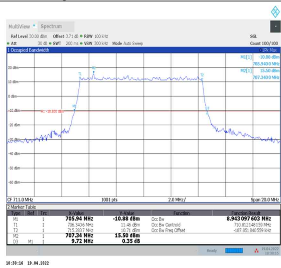
1-N12--15-10-H-1-DFT-QPSK-Outer_Full-50@0-Ant0-8.943-9.720-≤10-PASS
