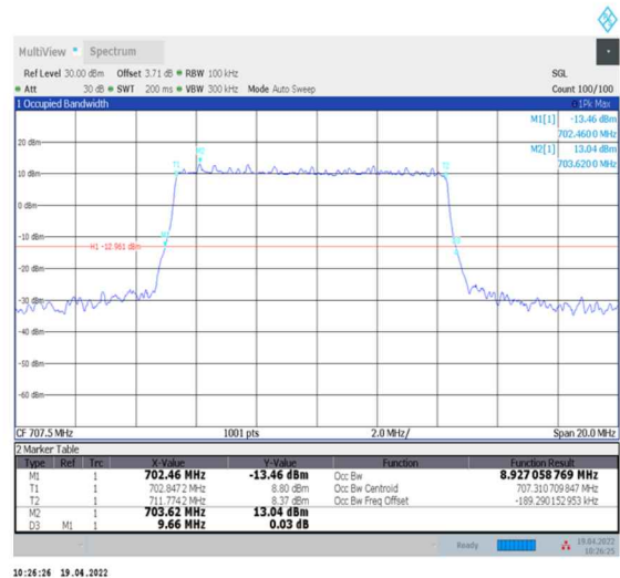
1-N12--15-10-M-4-DFT-64QAM-Outer_Full-50@0-Ant0-8.927-9.660-≤10-PASS
