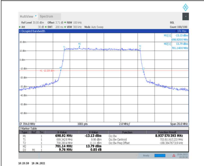
1-N12--15-10-L-4-DFT-64QAM-Outer_Full-50@0-Ant0-8.938-9.760-≤10-PASS
