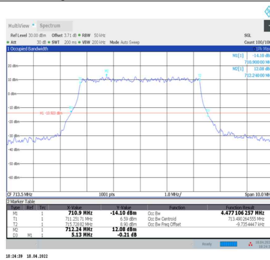
1-N12--15-5-H-4-DFT-64QAM-Outer_Full-25@0-Ant0-4.477-5.130-≤5-PASS
