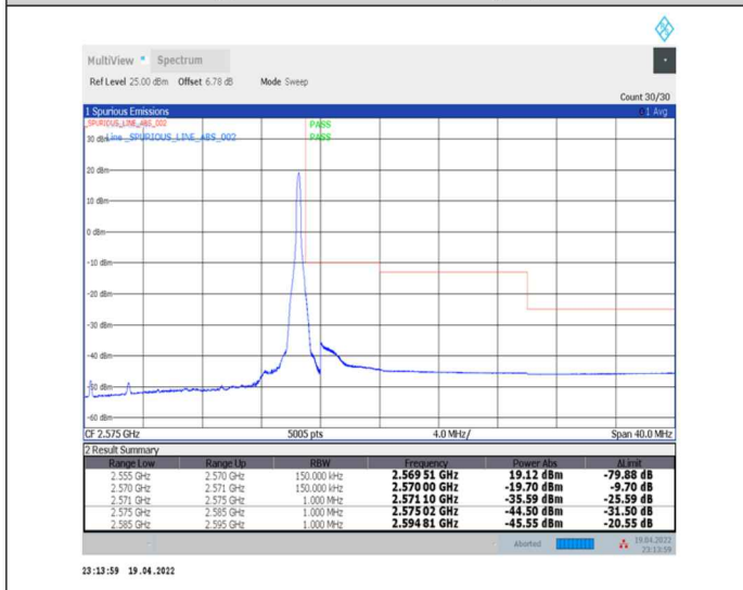
1-N7--15-15-H-5-CP-QPSK-Edge_1RB_Right-1@78-Ant0-PASS-see graph
