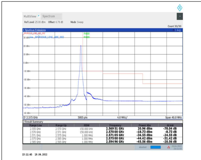
1-N7--15-15-H-2-DFT-PI2BPSK-Edge_1RB_Right-1@78-Ant0-PASS-see graph
