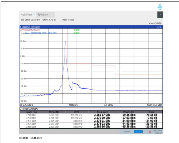
1-N7--15-10-H-2-DFT-PI2BPSK-Edge_1RB_Right-1@51-Ant0-PASS-see graph
