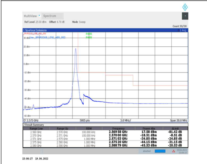
1-N7--15-10-H-5-CP-QPSK-Edge_1RB_Right-1@51-Ant0-PASS-see graph
