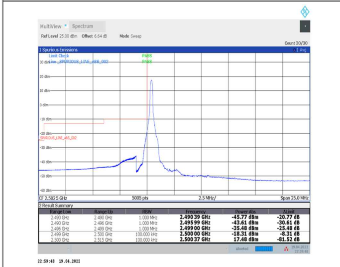
1-N7--15-10-L-4-CP-QPSK-Edge_1RB_Left-1@0-Ant0-PASS-see graph
