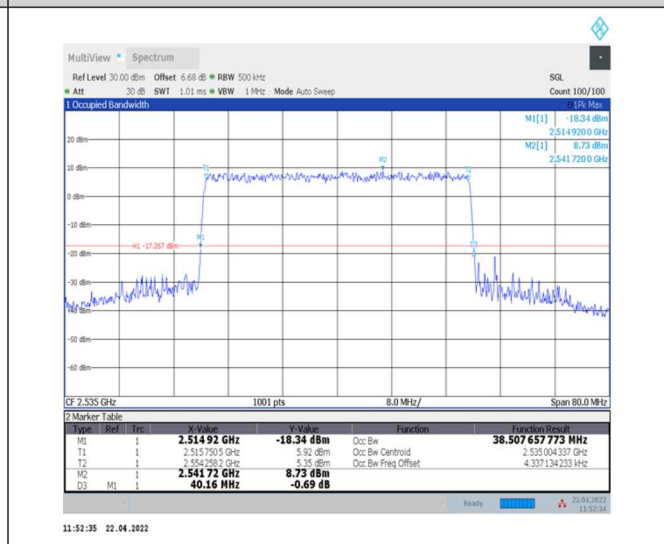
1-N7--15-40-M-9-CP-256QAM-Outer_Full-216@0-Ant0-38.491-40.160-<math>\leq 40</math>-PASS
