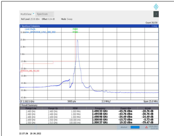
1-N7--15-10-L-1-DFT-PI2BPSK-Edge_1RB_Left-1@0-Ant0-PASS-see graph
