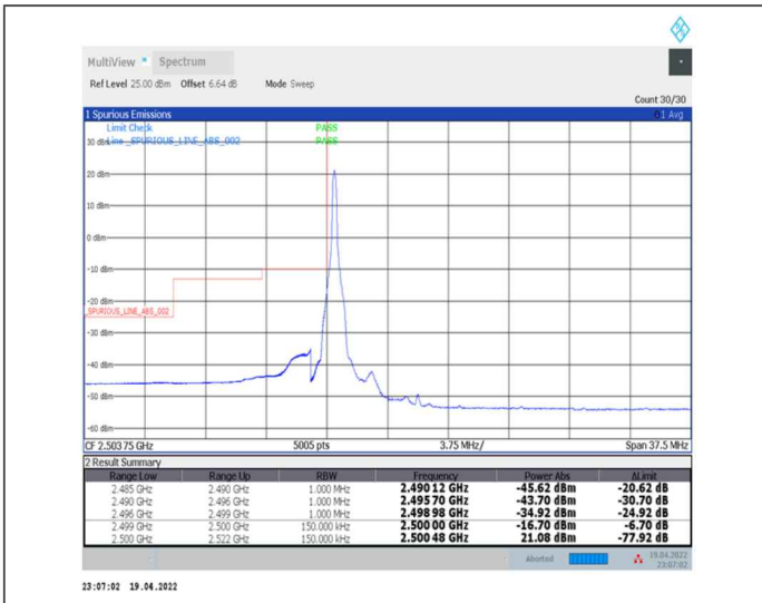
1-N7--15-15-L-1-DFT-PI2BPSK-Edge_1RB_Left-1@0-Ant0-PASS-see graph
