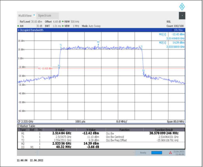
1-N7--15-40-M-1-DFT-QPSK-Outer_Full-216@0-Ant0-38.595-40.320-<math>\leq</math>40-PASS
