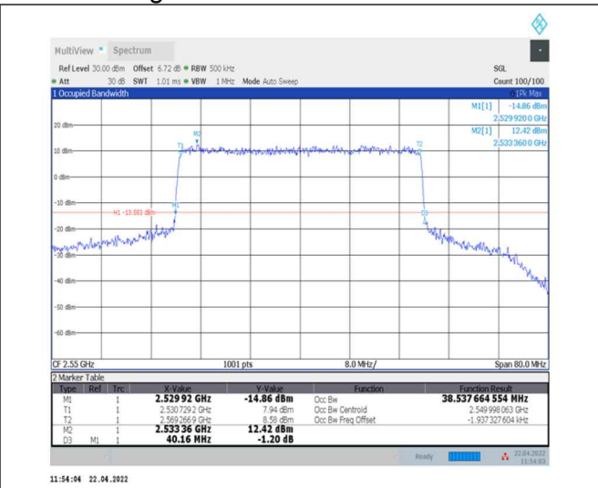
1-N7--15-40-H-6-CP-QPSK-Outer_Full-216@0-Ant0-38.55-40.160-<=40-PASS
