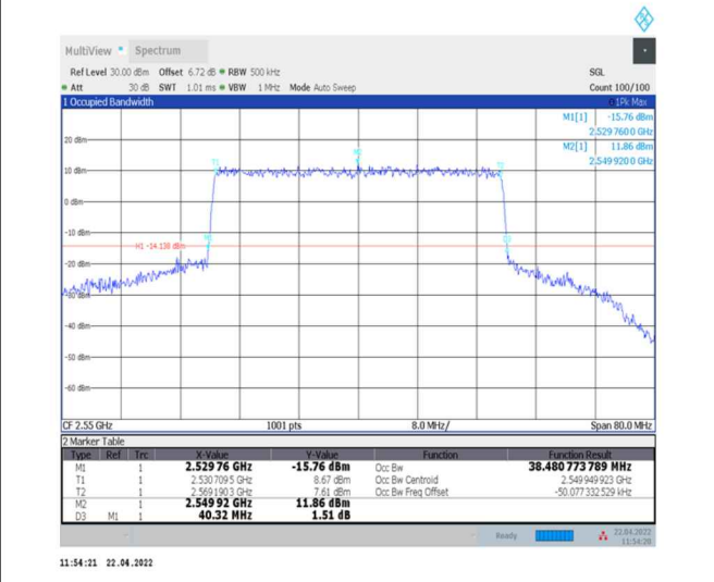
1-N7--15-40-H-8-CP-64QAM-Outer_Full-216@0-Ant0-38.405-40.320-<=40-PASS
