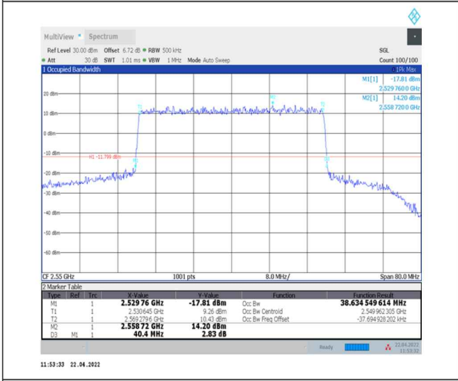
1-N7--15-40-H-3-DFT-16QAM-Outer_Full-216@0-Ant0-38.648-40.400-<math>\leq 40</math>-PASS
