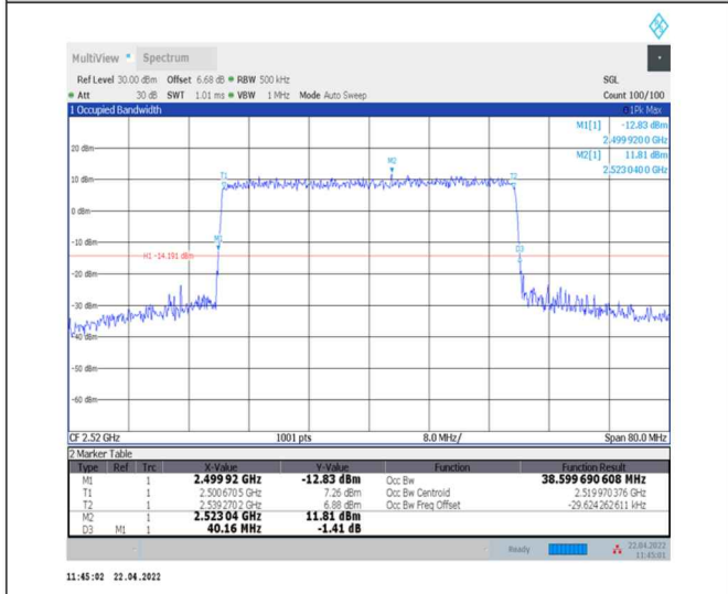
1-N7--15-40-L-5-DFT-256QAM-Outer_Full-216@0-Ant0-38.621-40.160-<math>\leq 40</math>-PASS
