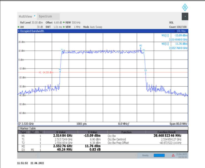
1-N7--15-40-M-5-DFT-256QAM-Outer_Full-216@0-Ant0-38.487-40.240-≤40-PASS
