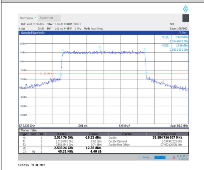
1-N7--15-40-M-8-CP-64QAM-Outer_Full-216@0-Ant0-38.585-40.320-<math>\leq 40</math>-PASS
