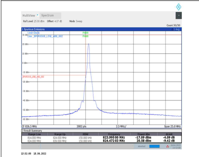
1-N5--15-15-L-4-CP-QPSK-Edge_1RB_Left-1@0-Ant0-seegraph-PASS-see graph
