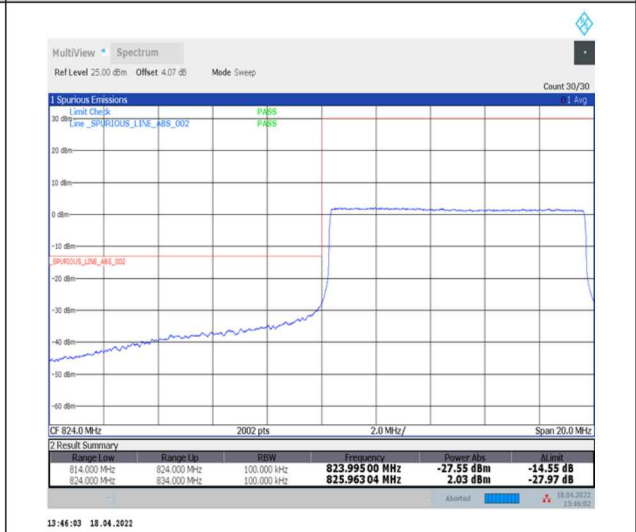
1-N5--15-10-L-6-CP-QPSK-Outer_Full-52@0-Ant0-seegraph-PASS-see graph
