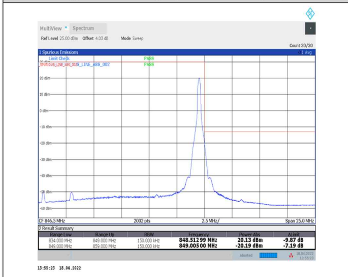
1-N5--15-15-H-5-CP-QPSK-Edge_1RB_Right-1@78-Ant0-seegraph-PASS-see graph
