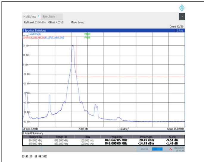
1-N5--15-5-H-2-DFT-PI2BPSK-Edge_1RB_Right-1@24-Ant0-seegraph-PASS-see graph
