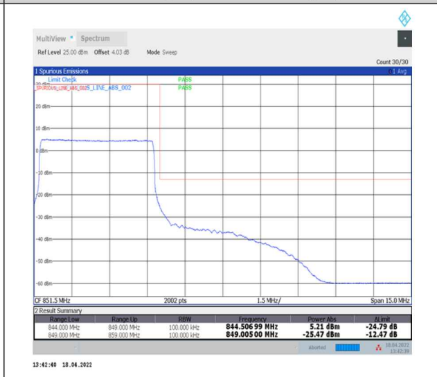
1-N5--15-5-H-6-CP-QPSK-Outer_Full-25@0-Ant0-seegraph-PASS-see graph
