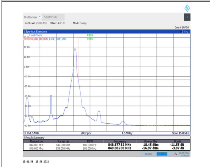
1-N5--15-5-H-5-CP-QPSK-Edge_1RB_Right-1@24-Ant0-seegraph-PASS-see graph
