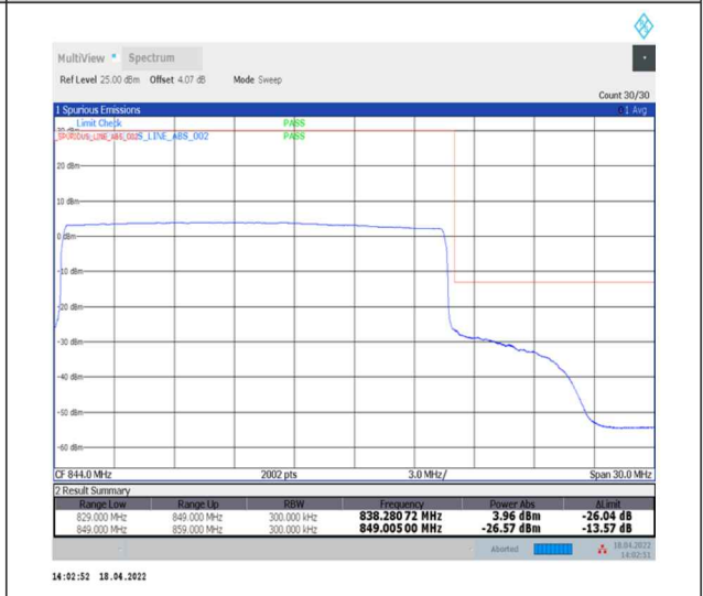
1-N5--15-20-H-6-CP-QPSK-Outer_Full-106@0-Ant0-seegraph-PASS-see graph
