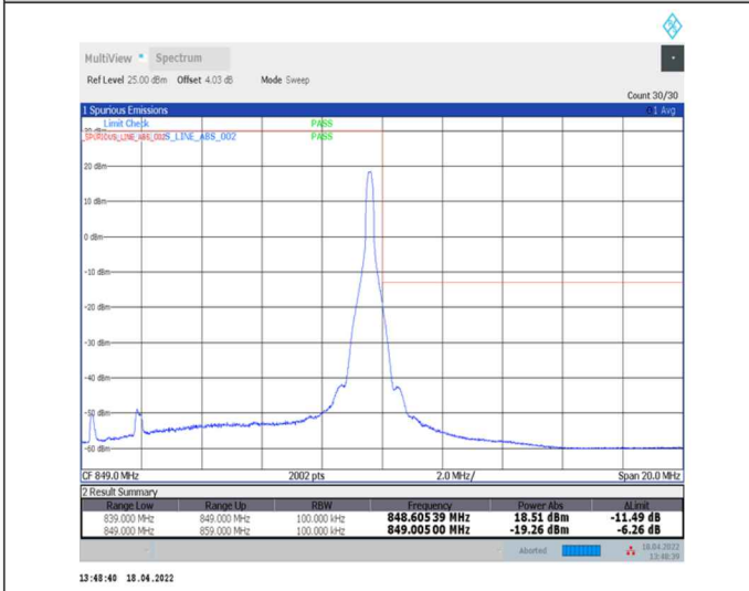
1-N5--15-10-H-5-CP-QPSK-Edge_1RB_Right-1@51-Ant0-seegraph-PASS-see graph
