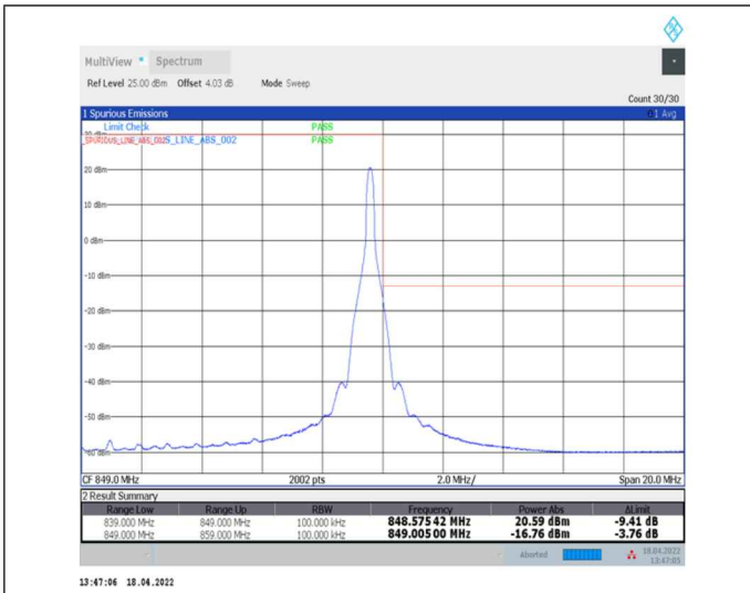
1-N5--15-10-H-2-DFT-PI2BPSK-Edge_1RB_Right-1@51-Ant0-seegraph-PASS-see graph
