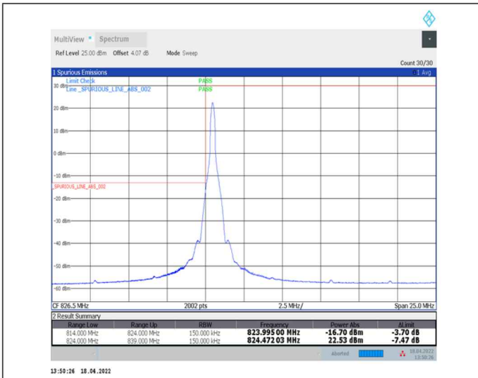
1-N5--15-15-L-1-DFT-PI2BPSK-Edge_1RB_Left-1@0-Ant0-seegraph-PASS-see graph
