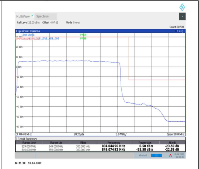
1-N5--15-20-H-3-DFT-PI2BPSK-Outer_Full-100@0-Ant0-seegraph-PASS-see graph
