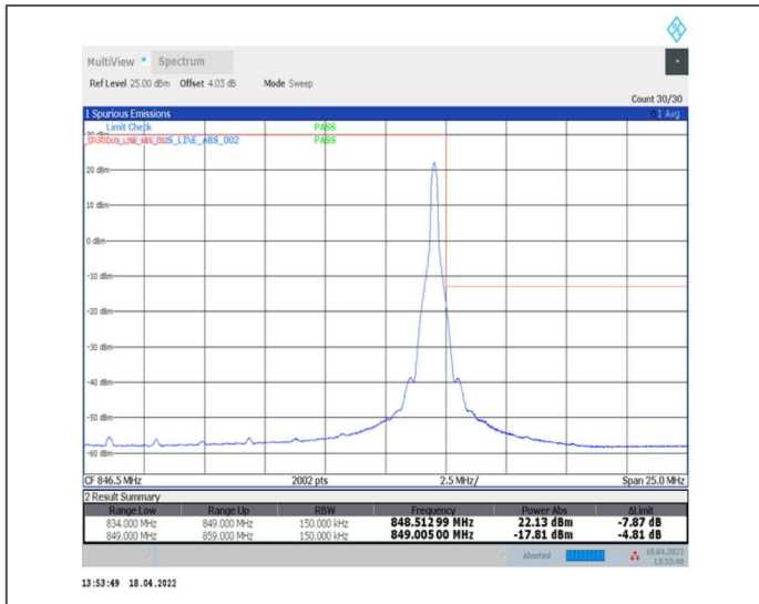
1-N5--15-15-H-2-DFT-PI2BPSK-Edge_1RB_Right-1@78-Ant0-seegraph-PASS-see graph
