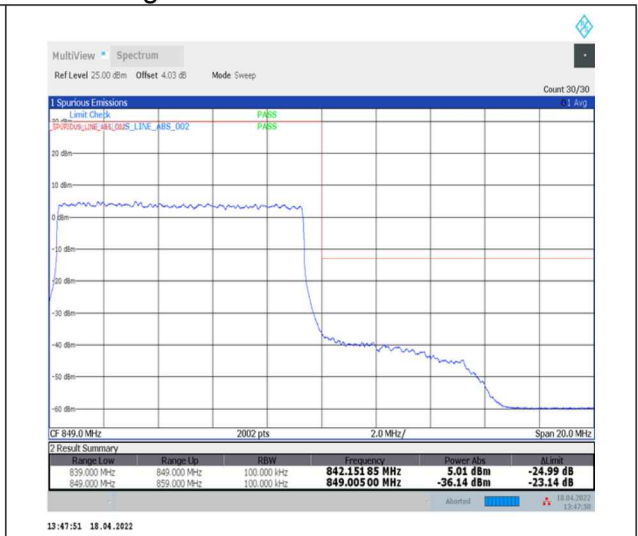
1-N5--15-10-H-3-DFT-PI2BPSK-Outer_Full-50@0-Ant0-seegraph-PASS-see graph
