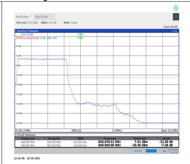
1-N5--15-5-H-3-DFT-PI2BPSK-Outer_Full-25@0-Ant0-seegraph-PASS-see graph
