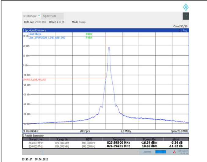
1-N5--15-10-L-4-CP-QPSK-Edge_1RB_Left-1@0-Ant0-seegraph-PASS-see graph
