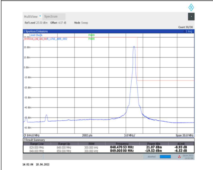
1-N5--15-20-H-5-CP-QPSK-Edge_1RB_Right-1@105-Ant0-seegraph-PASS-see graph
