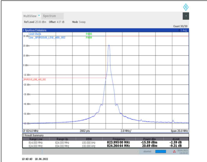
1-N5--15-10-L-1-DFT-PI2BPSK-Edge_1RB_Left-1@0-Ant0-seegraph-PASS-see graph
