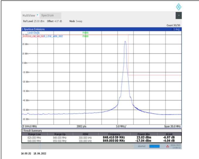
1-N5--15-20-H-2-DFT-PI2BPSK-Edge_1RB_Right-1@105-Ant0-seegraph-PASS-see graph
