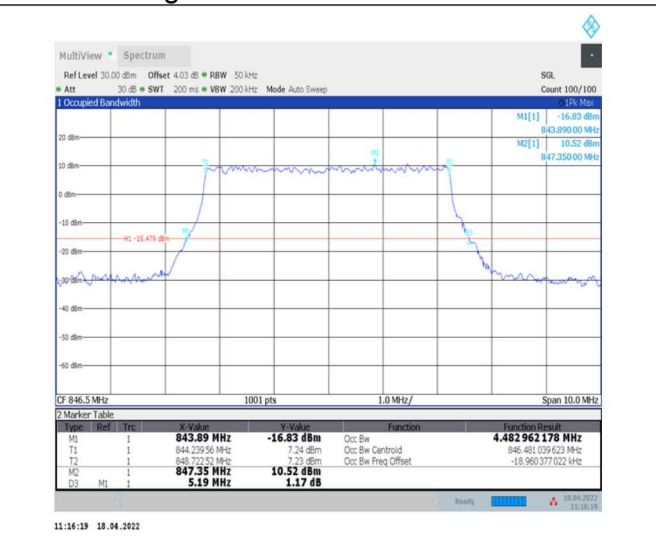
1-N5--15-5-H-8-CP-64QAM-Outer_Full-25@0-Ant0-4.483-5.190-≤5-PASS
