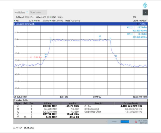
1-N5--15-5-L-8-CP-64QAM-Outer_Full-25@0-Ant0-4.486-5.260-≤5-PASS
