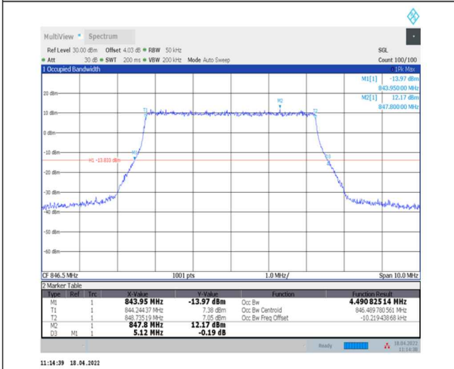
1-N5--15-5-H-5-DFT-256QAM-Outer_Full-25@0-Ant0-4.491-5.120-≤5-PASS
