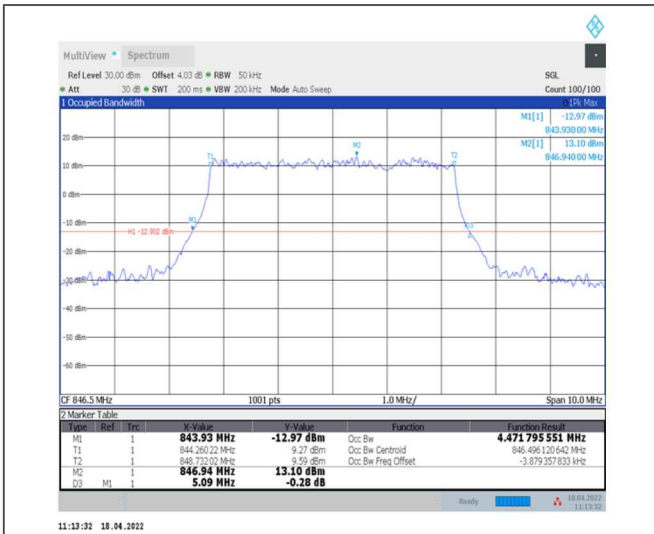
1-N5--15-5-H-3-DFT-16QAM-Outer_Full-25@0-Ant0-4.472-5.090-≤5-PASS
