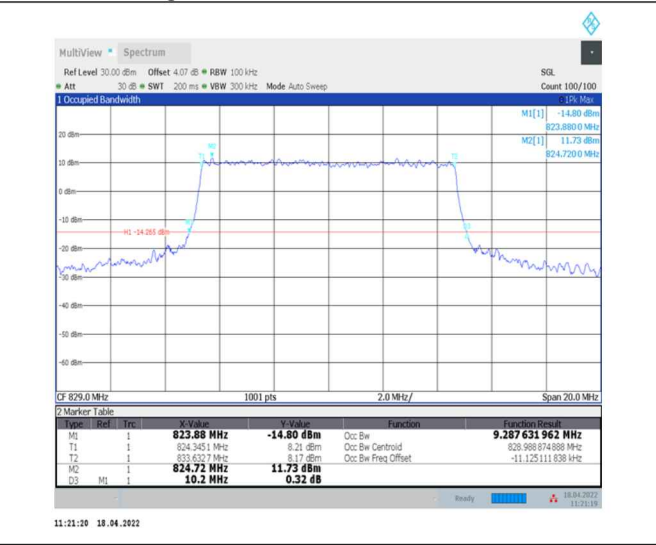
1-N5--15-10-L-7-CP-16QAM-Outer_Full-52@0-Ant0-9.288-10.200-≤10-PASS
