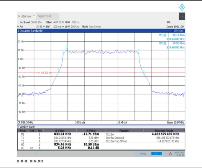
1-N5--15-5-M-5-DFT-256QAM-Outer_Full-25@0-Ant0-4.483-5.080-≤5-PASS
