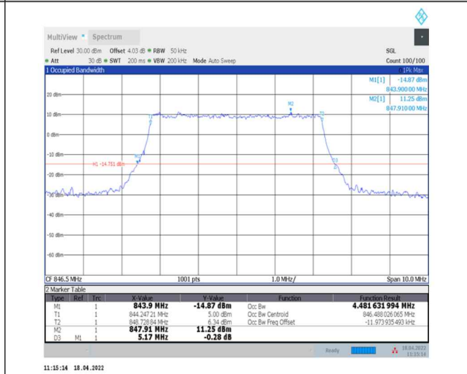
1-N5--15-5-H-6-CP-QPSK-Outer_Full-25@0-Ant0-4.482-5.170-≤5-PASS
