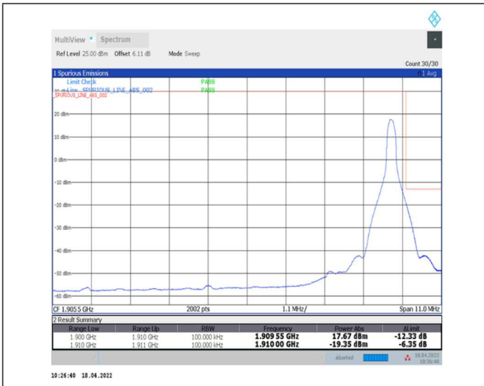
1-N2--15-10-H-2-DFT-PI2BPSK-Edge_1RB_Right-1@51-Ant0-seegraph-PASS-see graph
