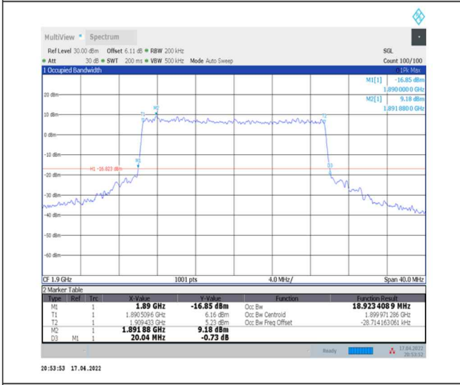
1-N2--15-20-H-8-CP-64QAM-Outer_Full-106@0-Ant0-18.923-20.040-<=20-PASS
