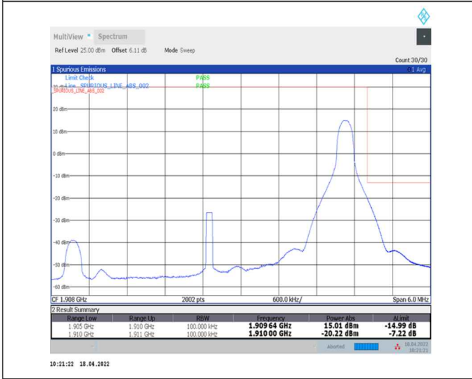
1-N2--15-5-H-5-CP-QPSK-Edge_1RB_Right-1@24-Ant0-seegraph-PASS-see graph
