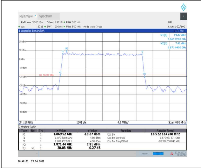
1-N2--15-20-M-9-CP-256QAM-Outer_Full-106@0-Ant0-18.922-20.080-<=20-PASS
