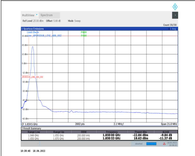
1-N2--15-20-L-4-CP-QPSK-Edge_1RB_Left-1@0-Ant0-seegraph-PASS-see graph
