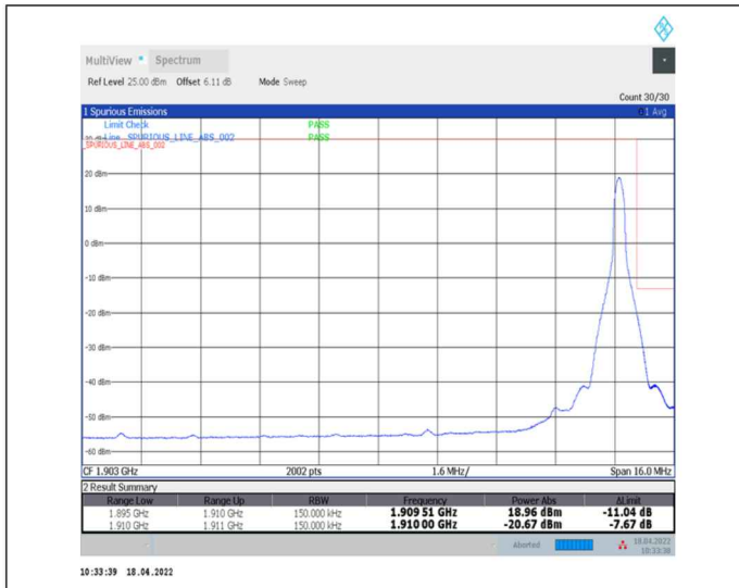
1-N2--15-15-H-2-DFT-PI2BPSK-Edge_1RB_Right-1@78-Ant0-seegraph-PASS-see graph
