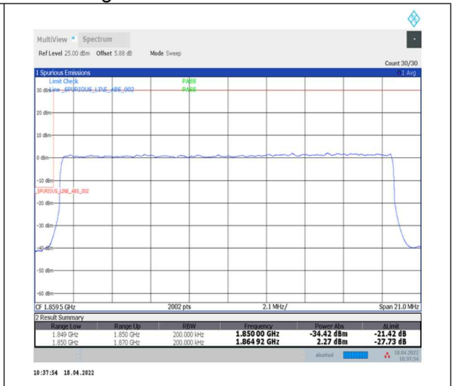
1-N2--15-20-L-3-DFT-PI2BPSK-Outer_Full-100@0-Ant0-seegraph-PASS-see graph
