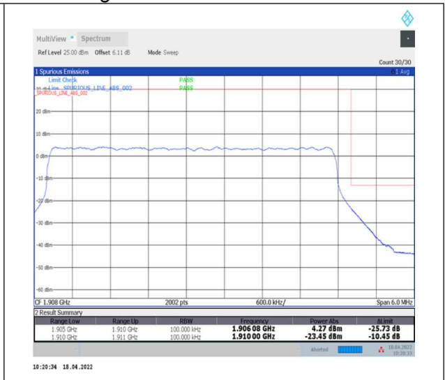
1-N2--15-5-H-3-DFT-PI2BPSK-Outer_Full-25@0-Ant0-seegraph-PASS-see graph
