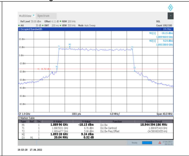
1-N2--15-20-H-7-CP-16QAM-Outer_Full-106@0-Ant0-18.945-20.040-<=20-PASS
