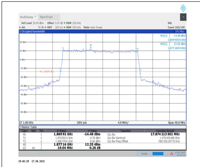
1-N2--15-20-M-3-DFT-16QAM-Outer_Full-100@0-Ant0-17.874-19.040-<=20-PASS
