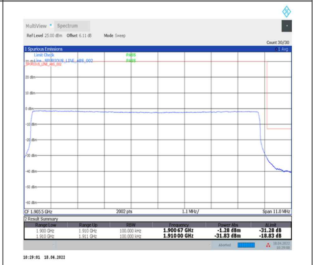
1-N2--15-10-H-6-CP-QPSK-Outer_Full-52@0-Ant0-seegraph-PASS-see graph
