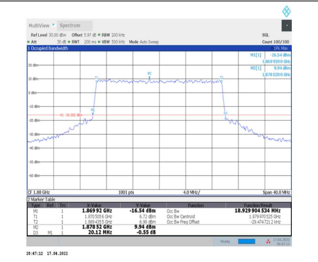
1-N2--15-20-M-6-CP-QPSK-Outer_Full-106@0-Ant0-18.93-20.120-<=20-PASS
