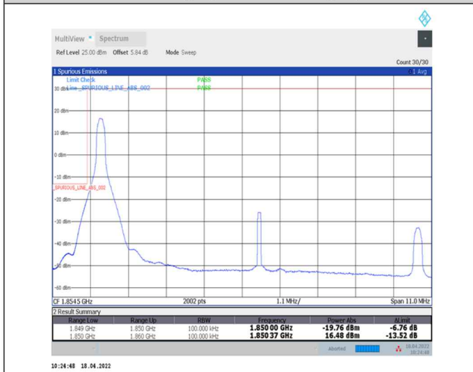
1-N2--15-10-L-4-CP-QPSK-Edge_1RB_Left-1@0-Ant0-seegraph-PASS-see graph
