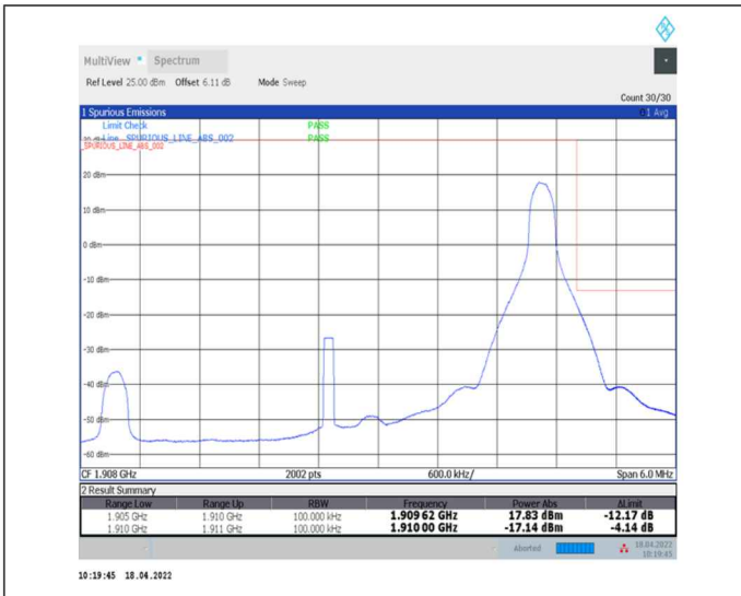
1-N2--15-5-H-2-DFT-PI2BPSK-Edge_1RB_Right-1@24-Ant0-seegraph-PASS-see graph
