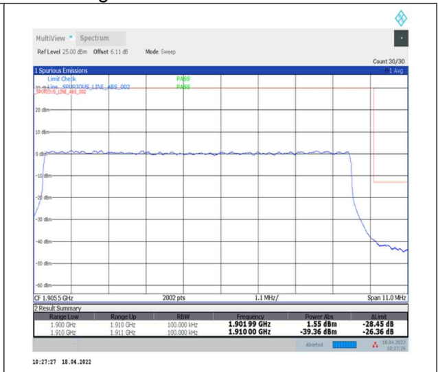
1-N2--15-10-H-3-DFT-PI2BPSK-Outer_Full-50@0-Ant0-seegraph-PASS-see graph
