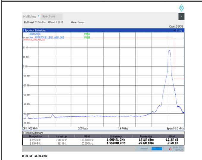
1-N2--15-15-H-5-CP-QPSK-Edge_1RB_Right-1@78-Ant0-seegraph-PASS-see graph
