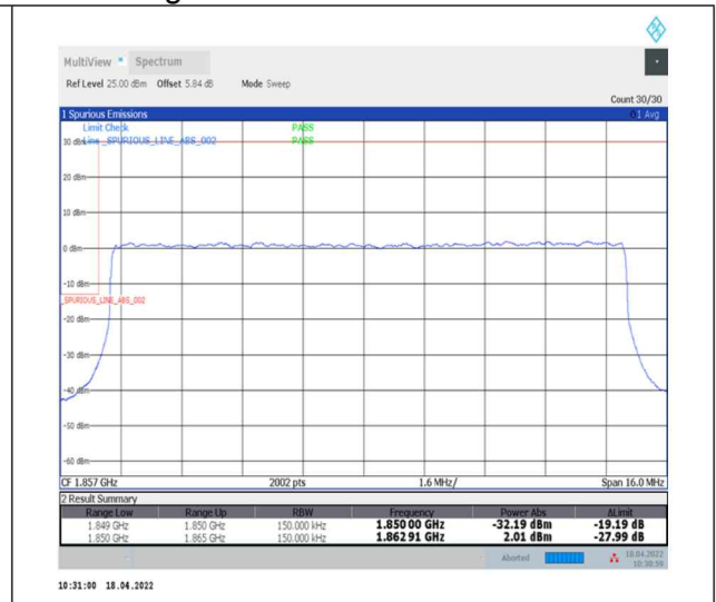
1-N2--15-15-L-3-DFT-PI2BPSK-Outer_Full-75@0-Ant0-seegraph-PASS-see graph
