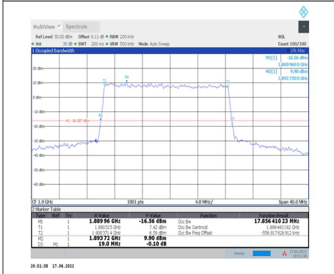
1-N2--15-20-H-4-DFT-64QAM-Outer_Full-100@0-Ant0-17.856-19.000-<20-PASS
