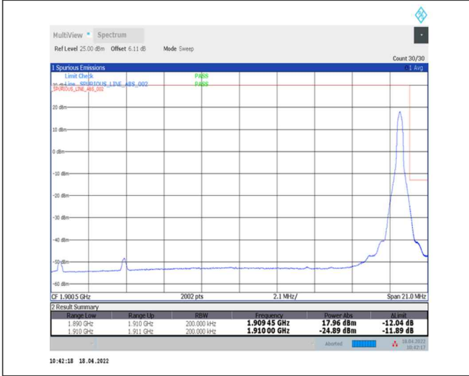
1-N2--15-20-H-5-CP-QPSK-Edge_1RB_Right-1@105-Ant0-seegraph-PASS-see graph
