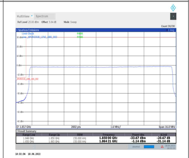
1-N2--15-15-L-6-CP-QPSK-Outer_Full-79@0-Ant0-seegraph-PASS-see graph
