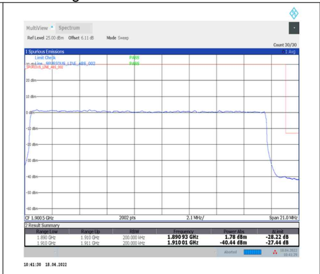
1-N2--15-20-H-3-DFT-PI2BPSK-Outer_Full-100@0-Ant0-seegraph-PASS-see graph
