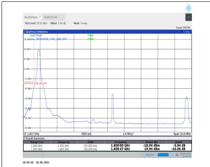
1-N2--15-15-L-1-DFT-PI2BPSK-Edge_1RB_Left-1@0-Ant0-seegraph-PASS-see graph
