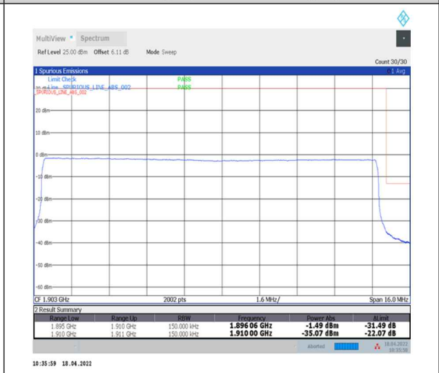
1-N2--15-15-H-6-CP-QPSK-Outer_Full-79@0-Ant0-seegraph-PASS-see graph
