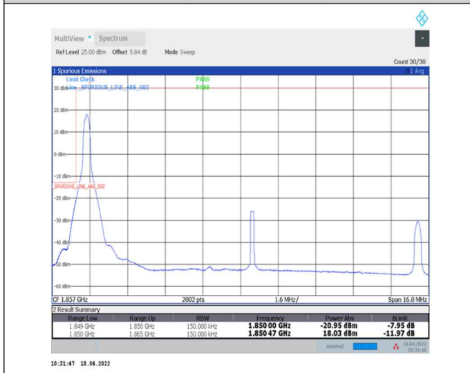
1-N2--15-15-L-4-CP-QPSK-Edge_1RB_Left-1@0-Ant0-seegraph-PASS-see graph
