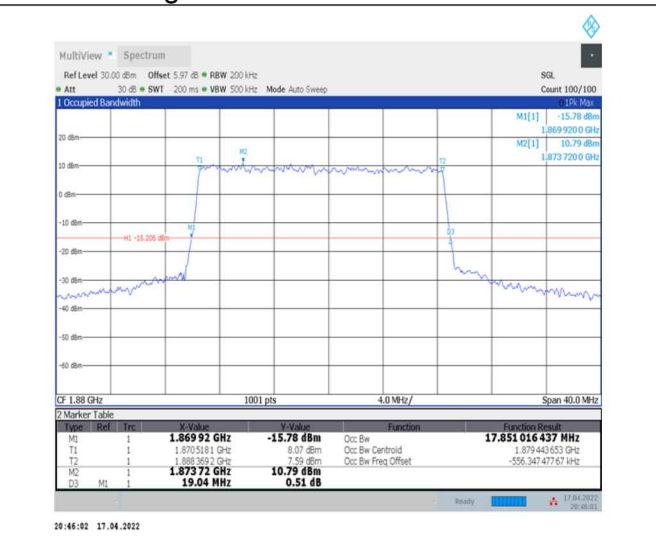
1-N2--15-20-M-4-DFT-64QAM-Outer_Full-100@0-Ant0-17.851-19.040-<=20-PASS
