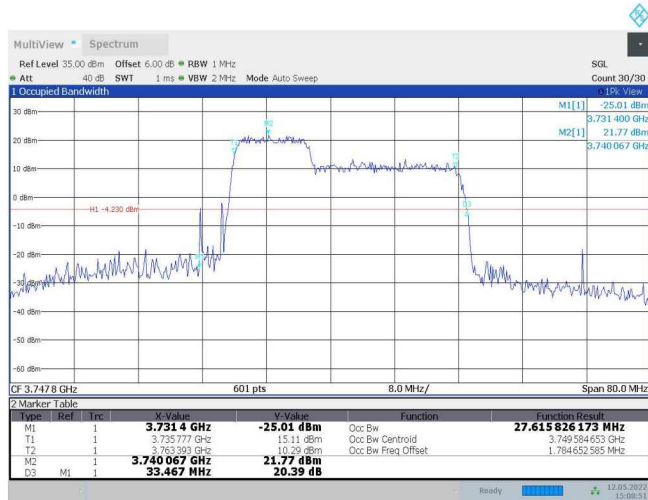
43-43-10MHz-20MHz-QPSK-QPSK-44996-45140-50RB#0-100RB#0
