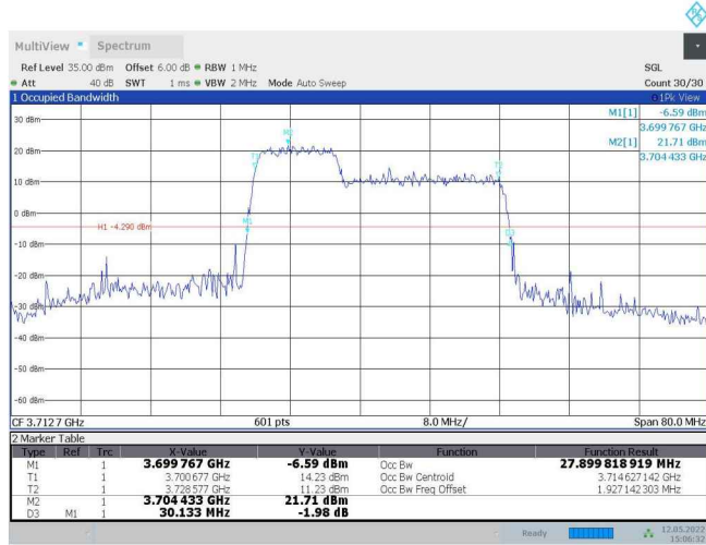
43-43-10MHz-20MHz-QPSK-QPSK-44645-44789-50RB#0-100RB#0
