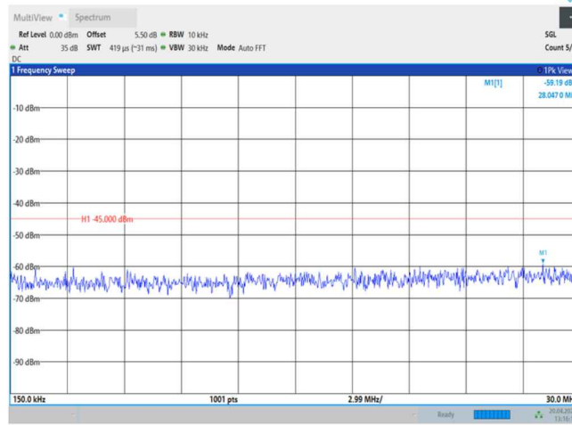
7-7-20MHz-20MHz-QPSK-QPSK-20850-21048-1RB#0-0RB#0-0.15~30MHz
