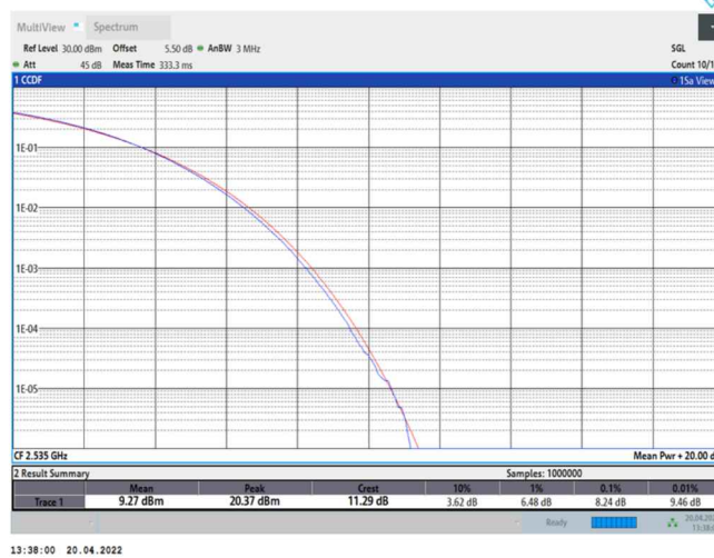
7-7-20MHz-20MHz-QPSK-QPSK-21001-21199-100RB#0-100RB#0
