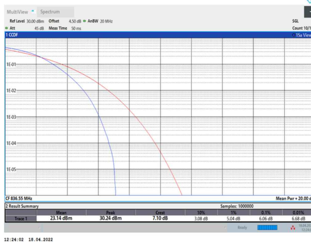
5-5-10MHz-10MHz-QPSK-QPSK-20476-20575-50RB#0-50RB#0
